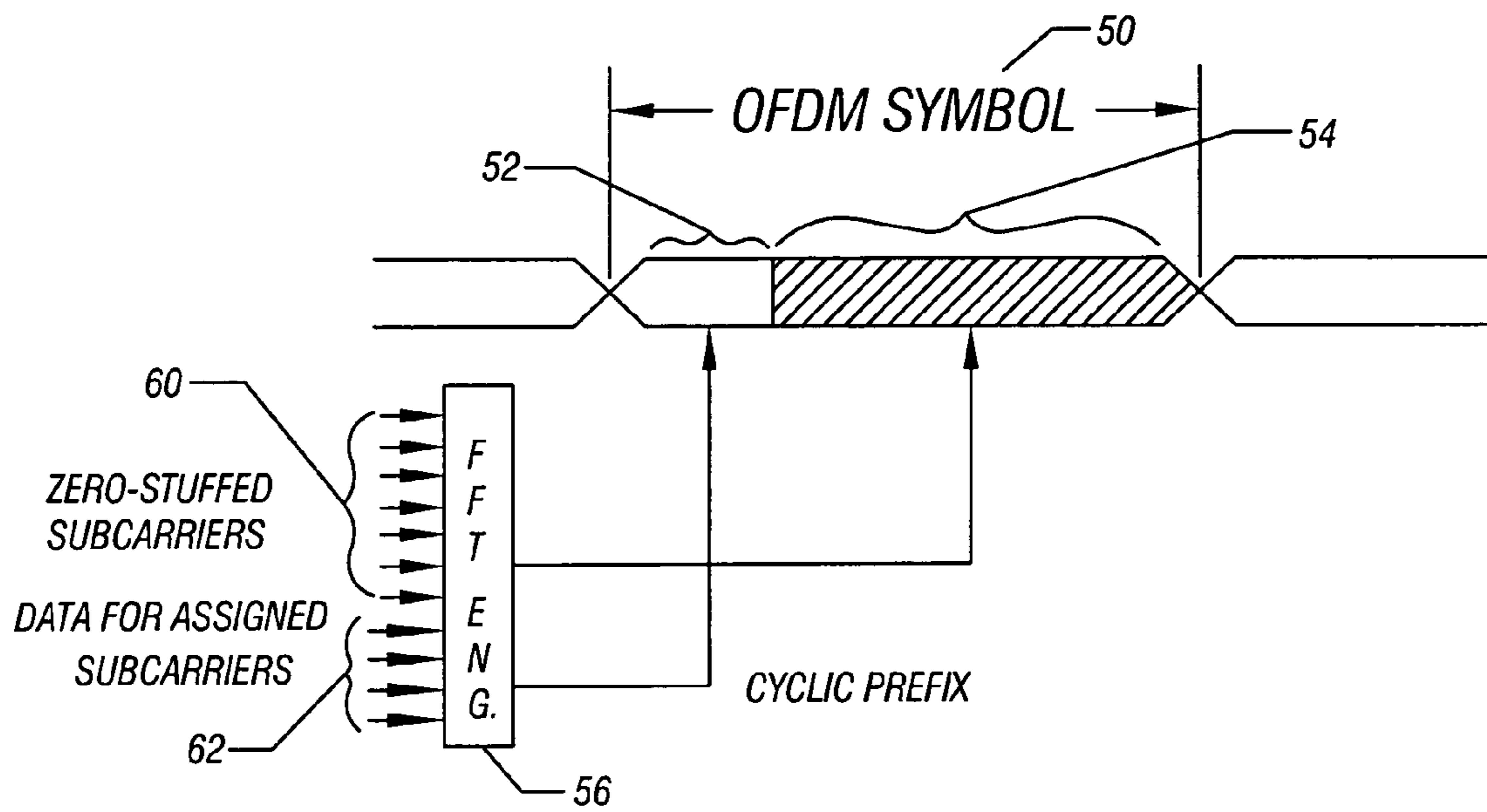
FIG. 2 (PRIOR ART)
