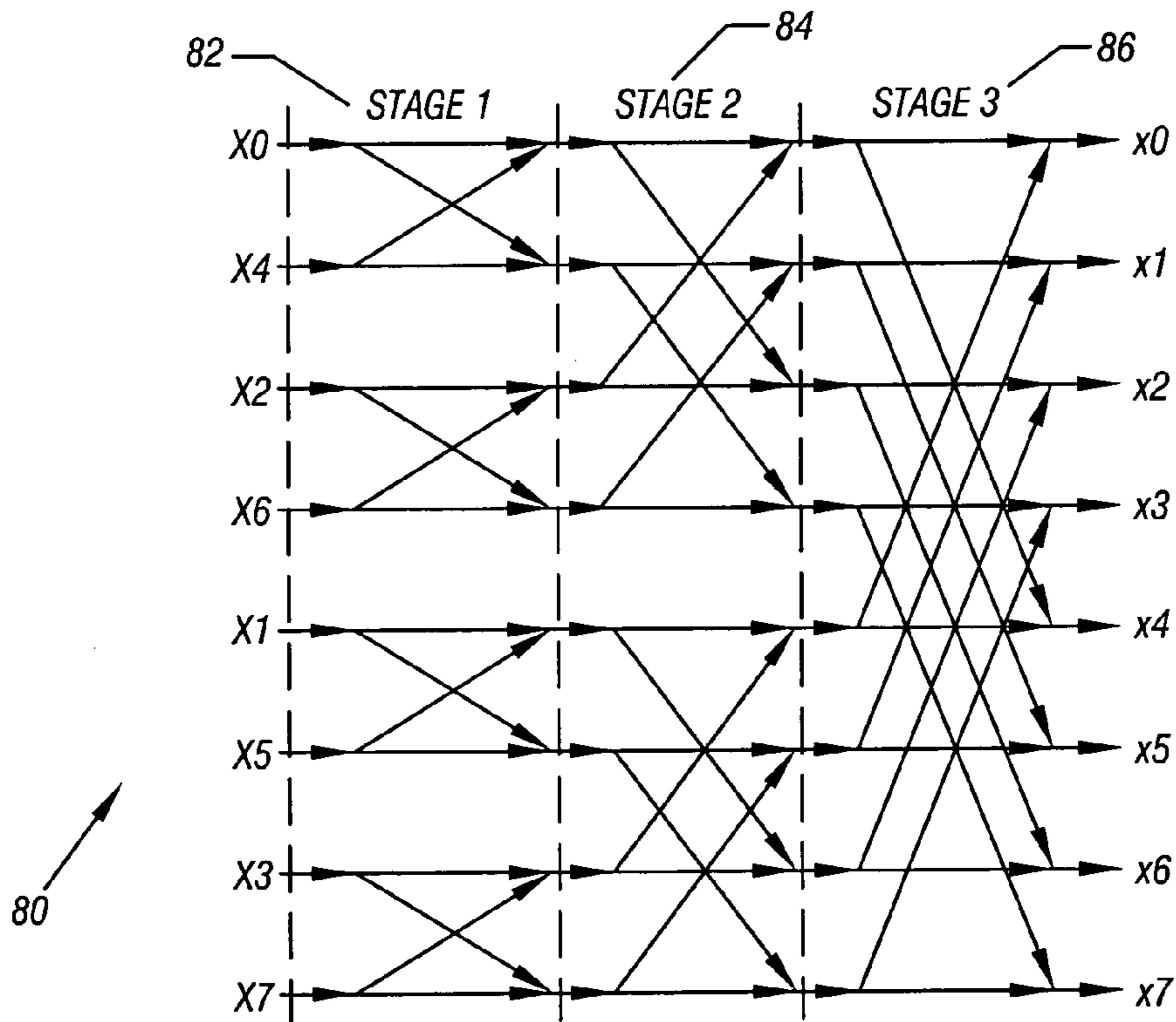
FIG. 3 (PRIOR ART)
