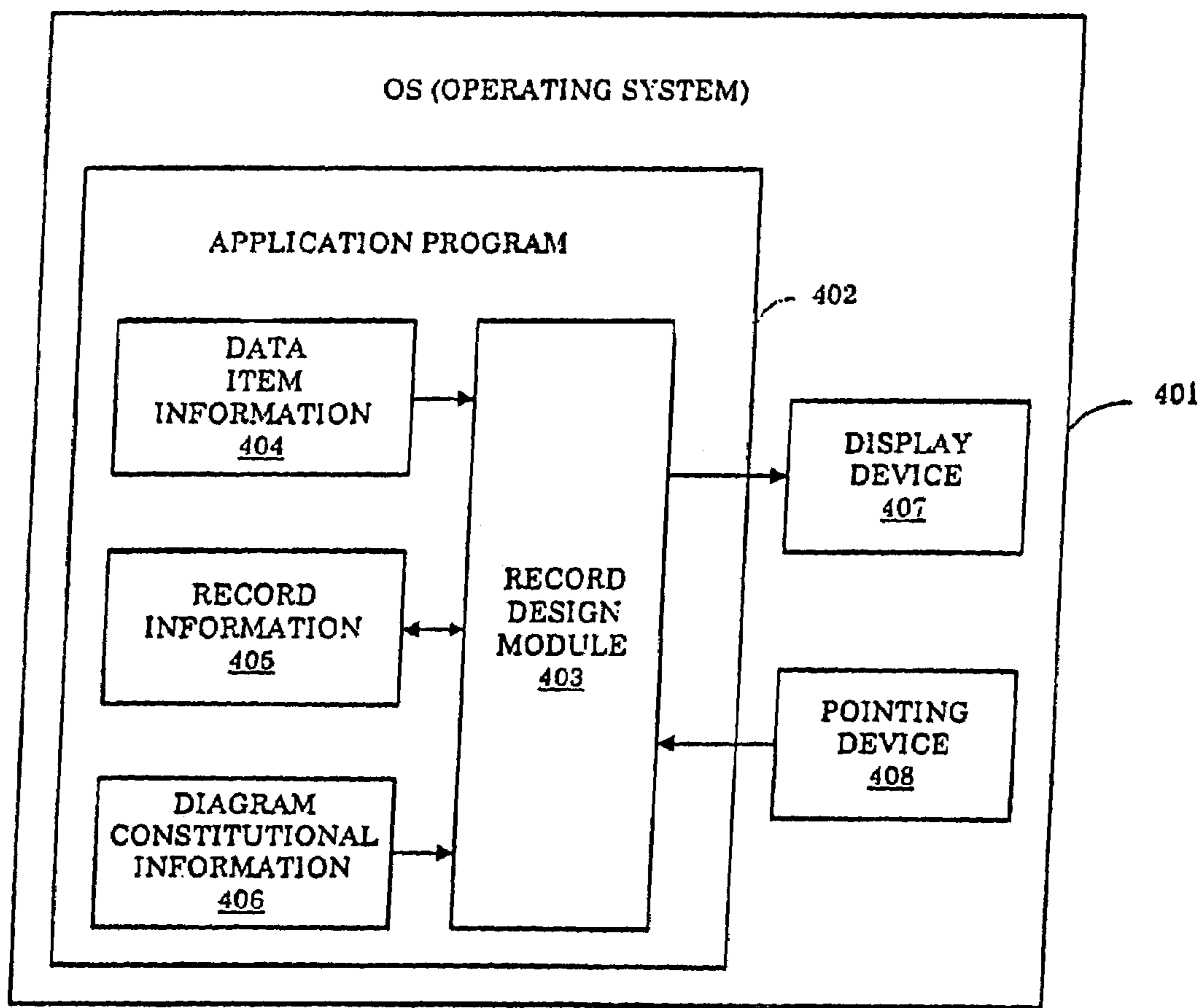
CONSTITUTIONAL VIEW OF SOFTWARE
