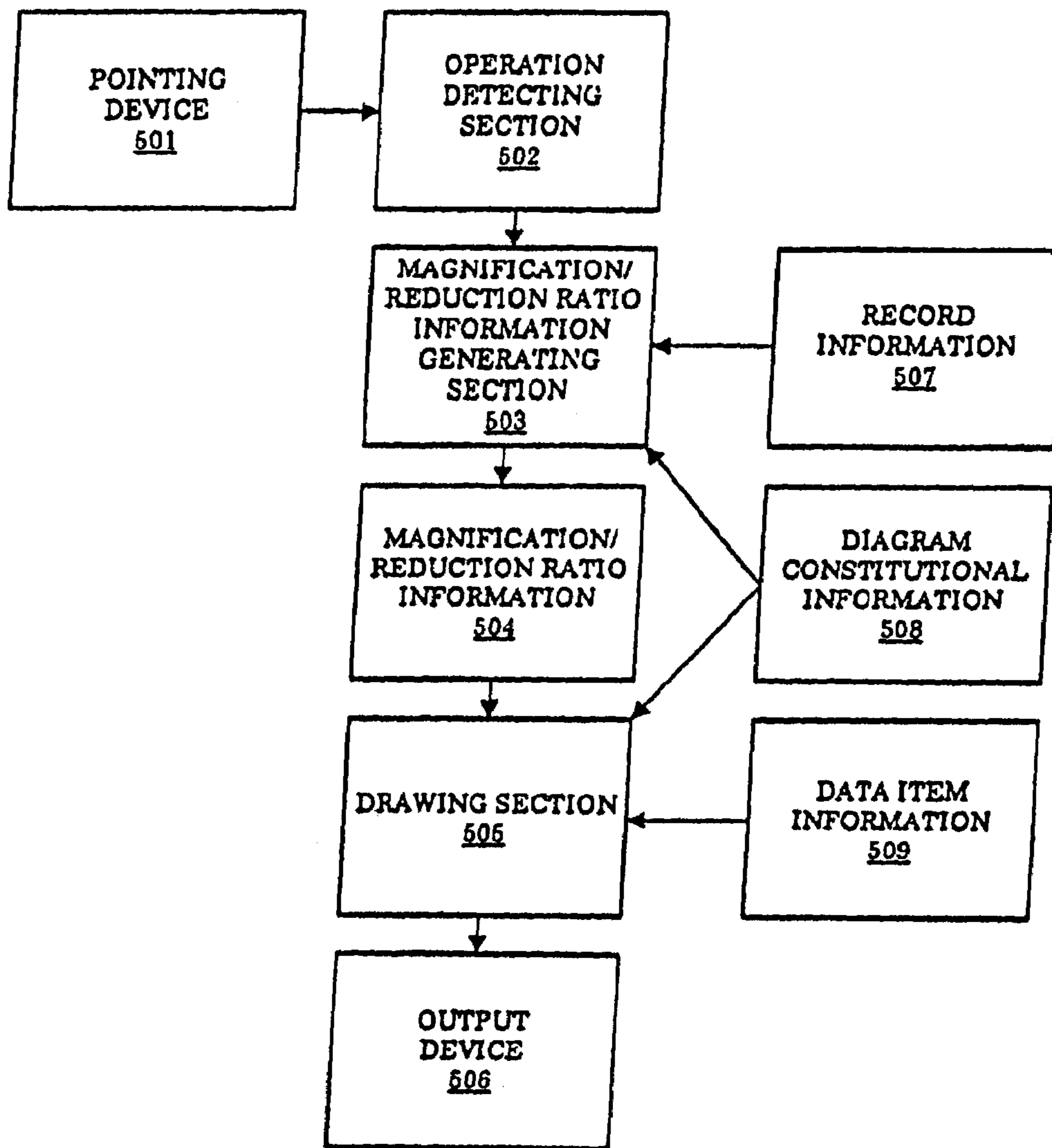
CONSTITUTIONAL VIEW OF RECORD DESIGN MODULE
