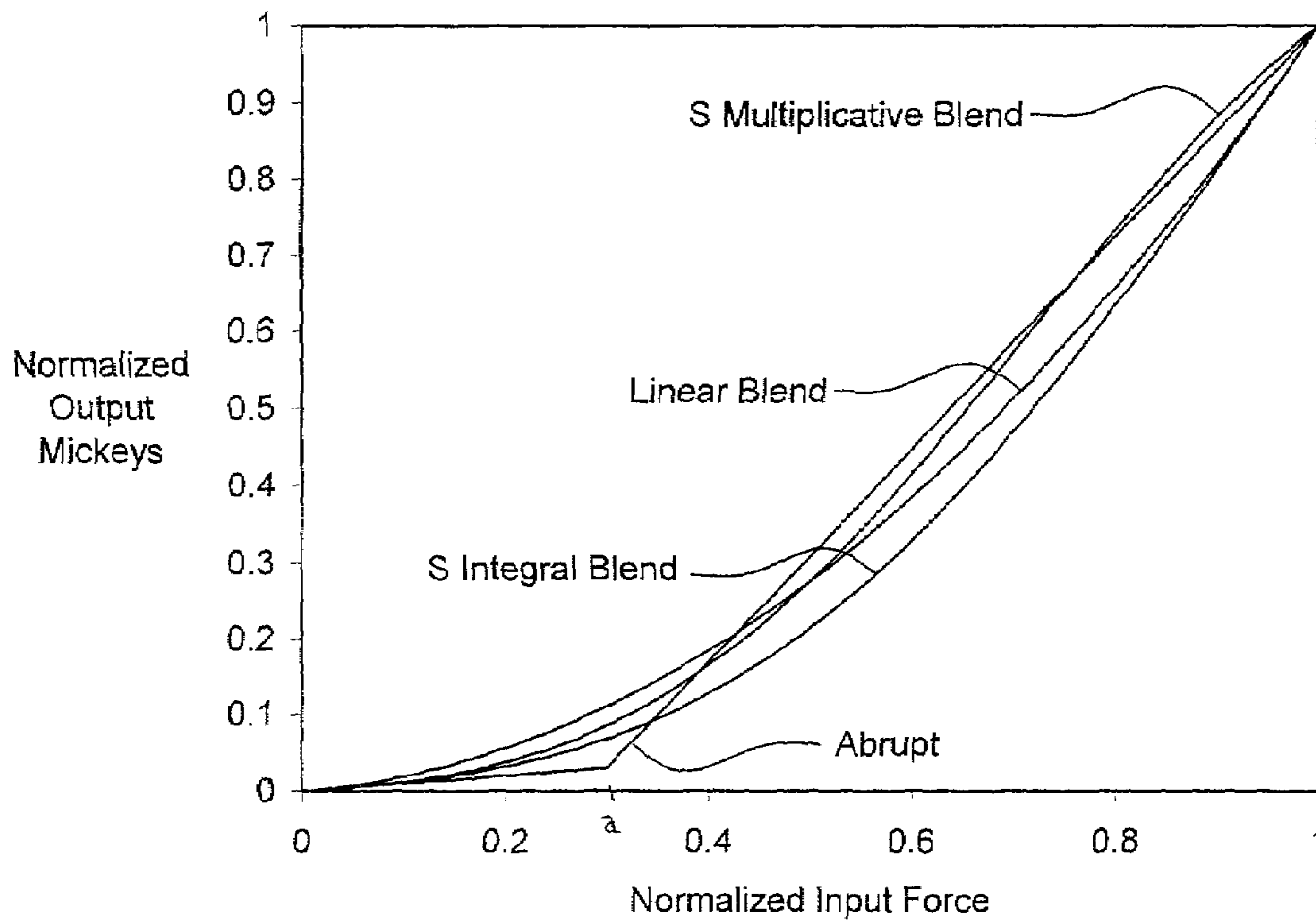
Dual-Gain Transfer Functions
