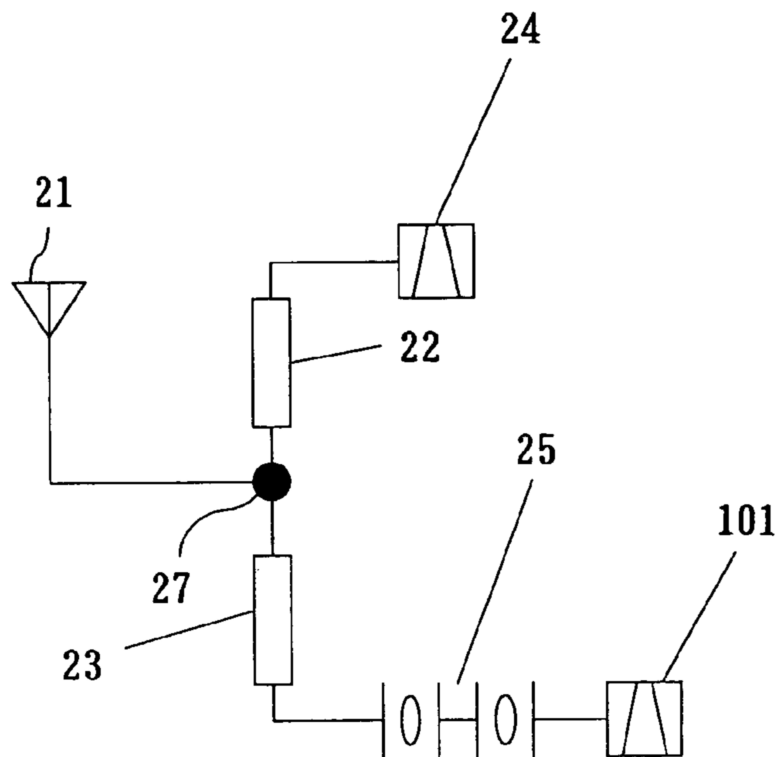
Fig. 17 (a)
