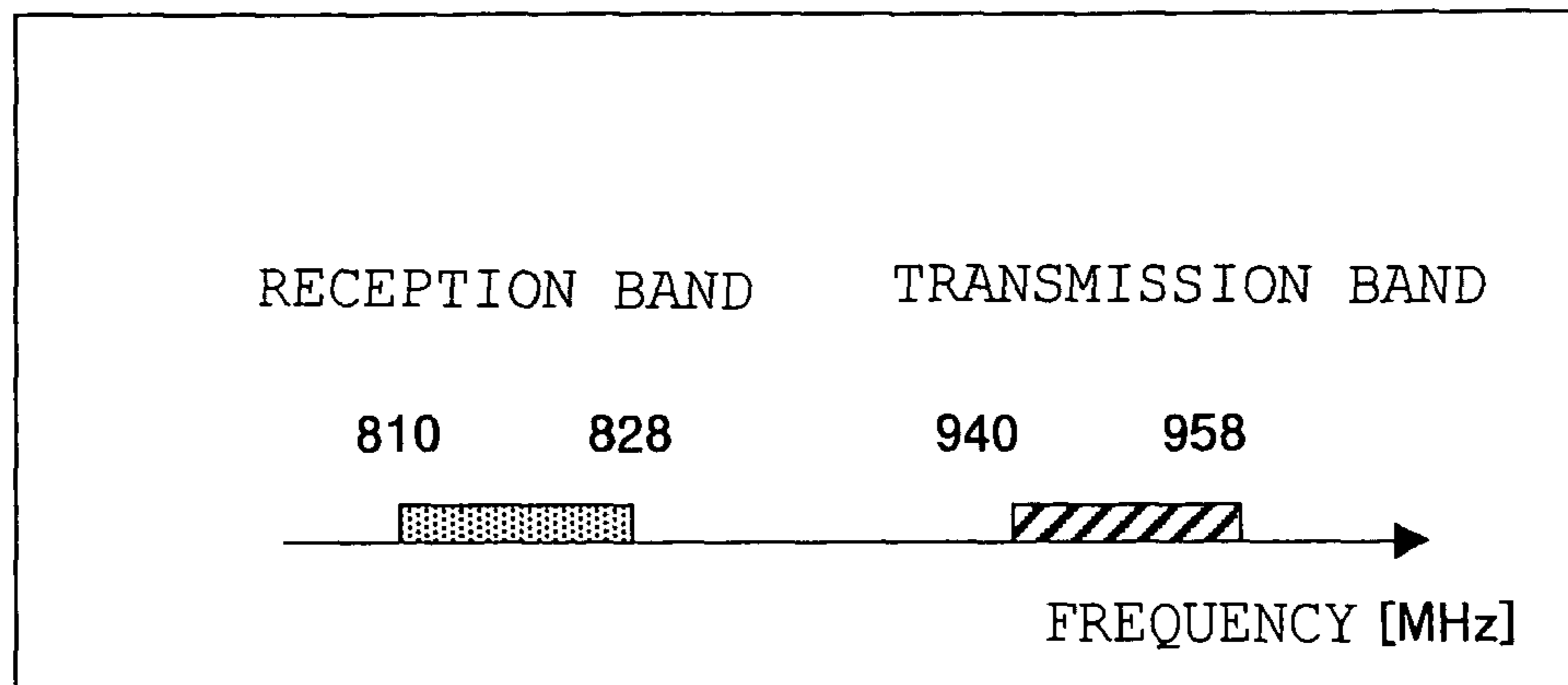
Fig. 23 PRIOR ART
