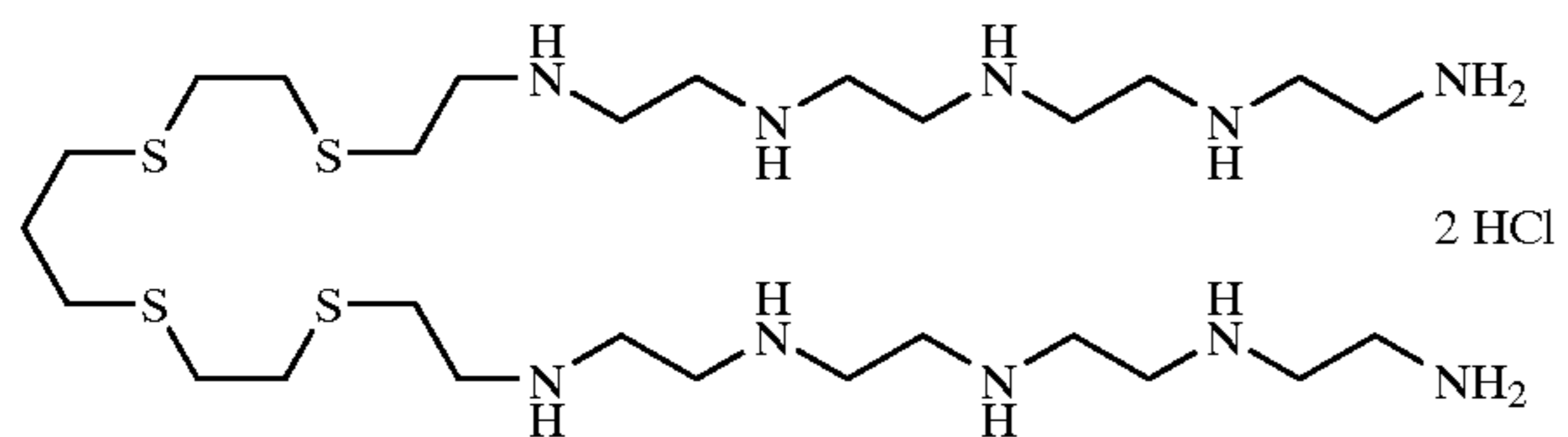
Formula IV
