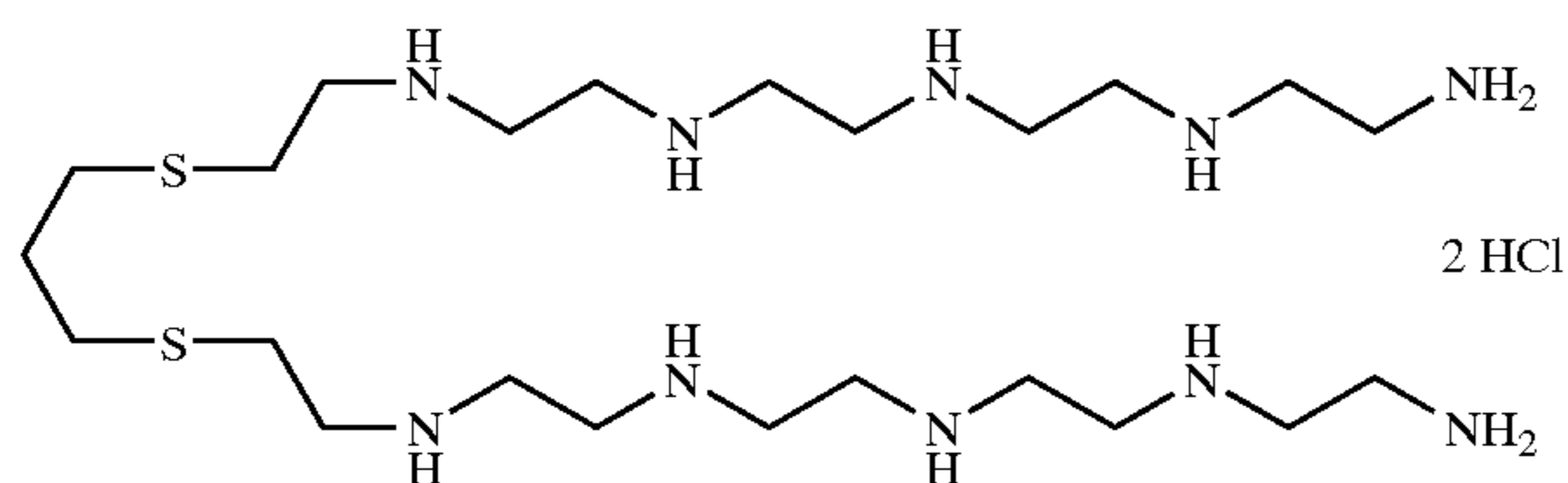
Formula V
