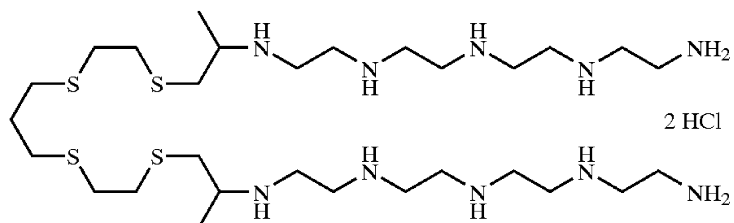
Formula II
