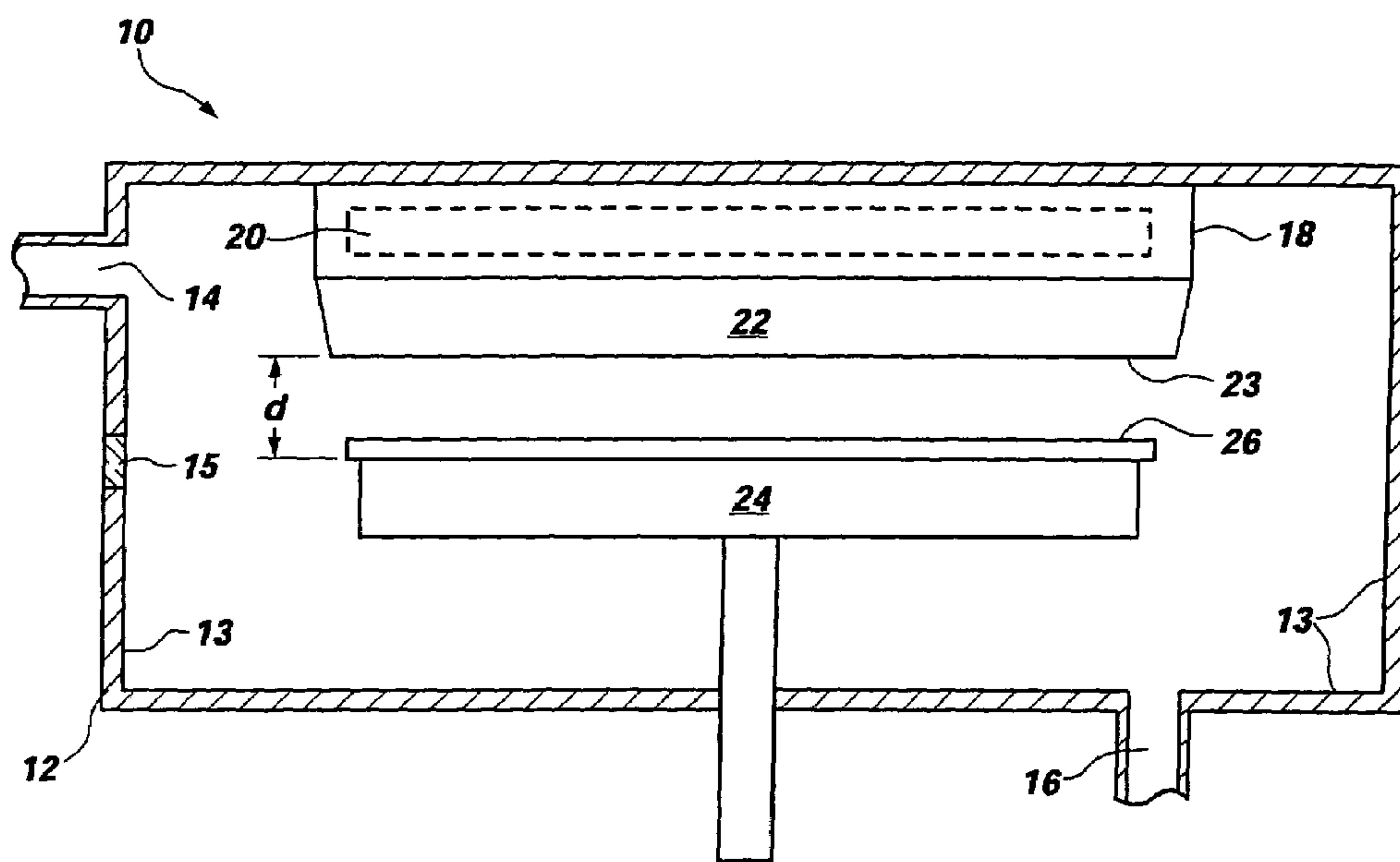
FIG. 1 (PRIOR ART)
