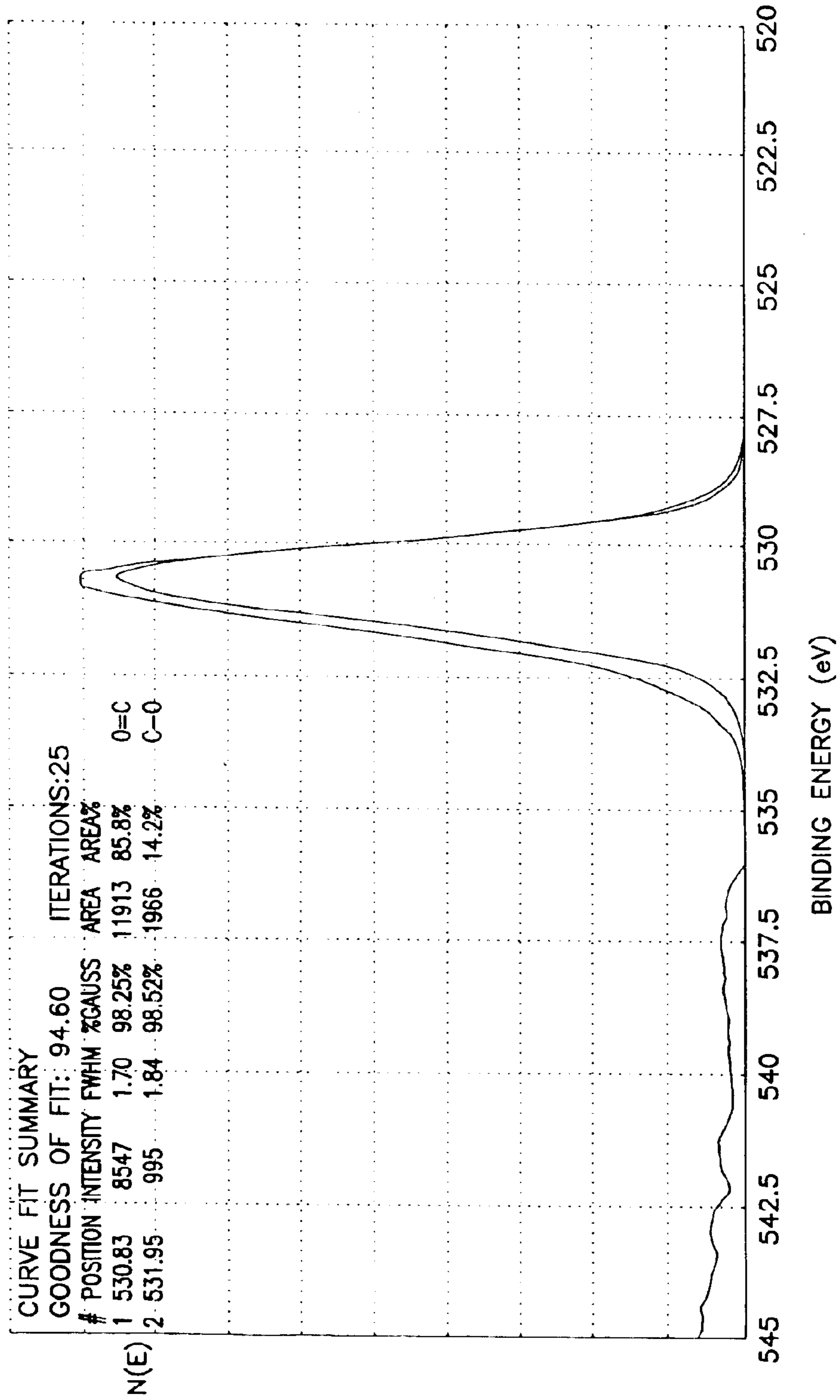
FIG. 5 ESCA O1s SPECTRA FOR HEAT-TREATED SAMPLE 6A
