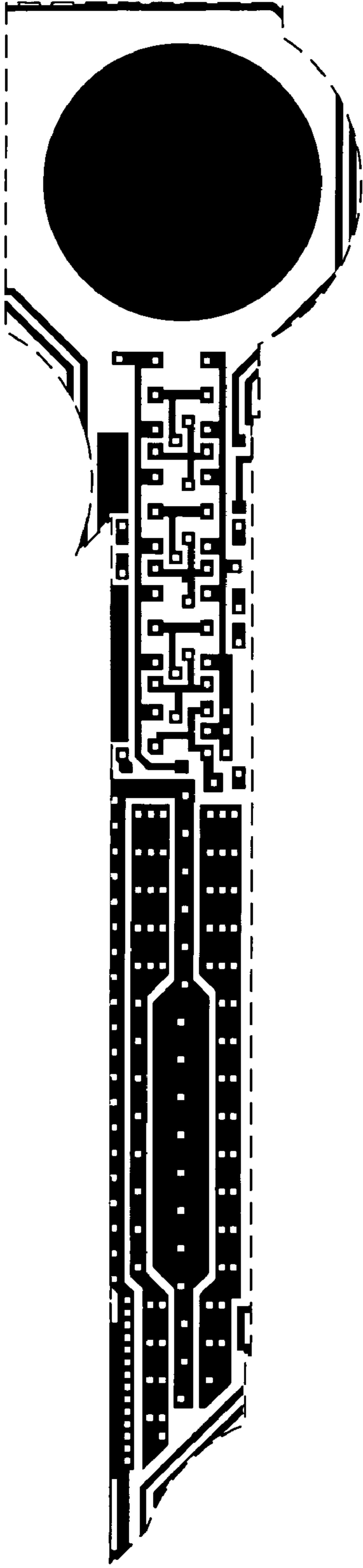
Metal 1 mask
