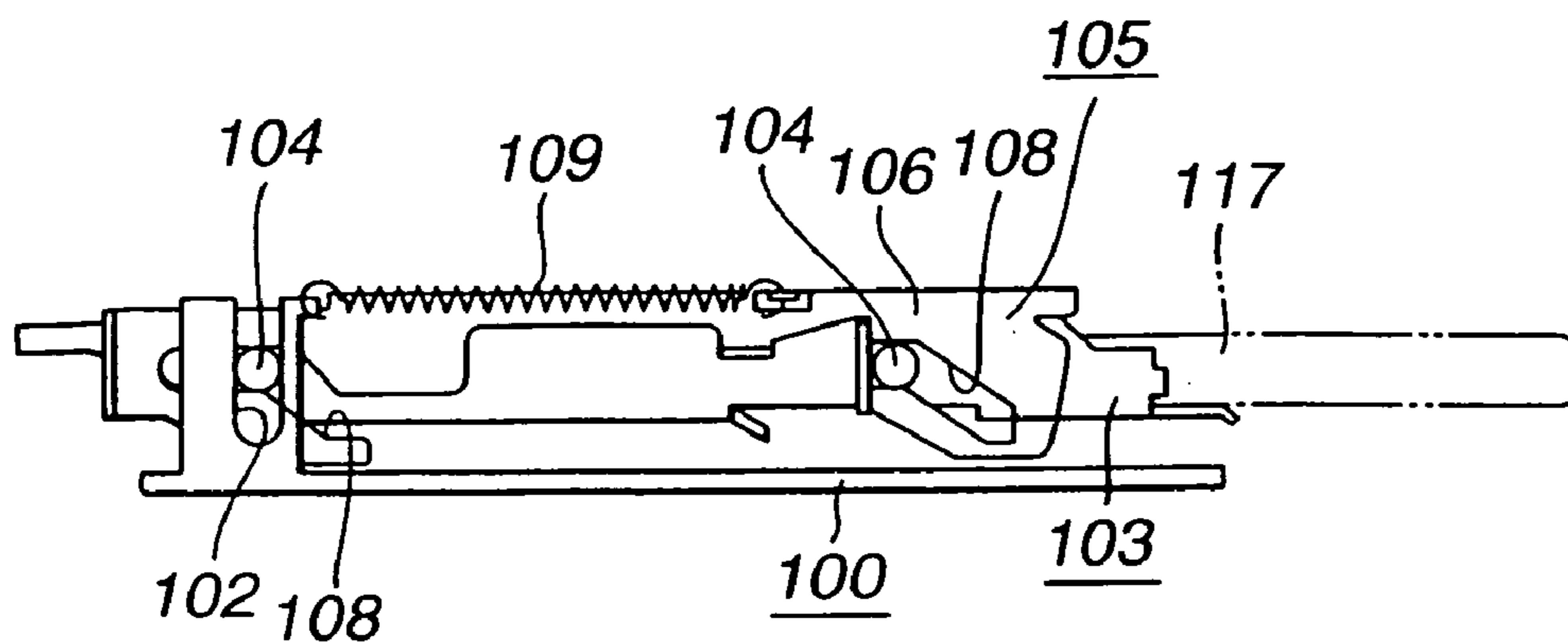
FIG. 2 (PRIOR ART)
