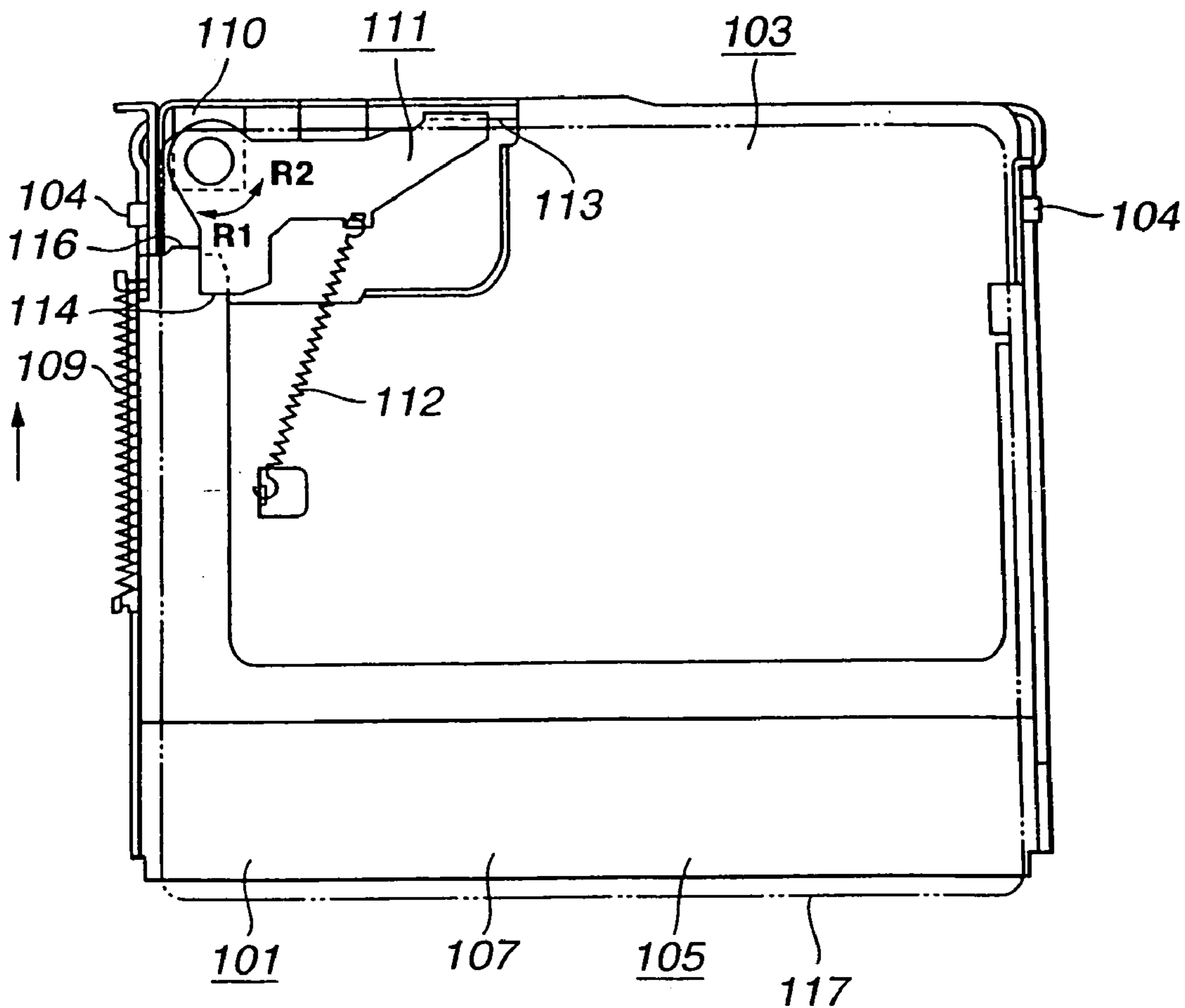
FIG. 4 (PRIOR ART)
