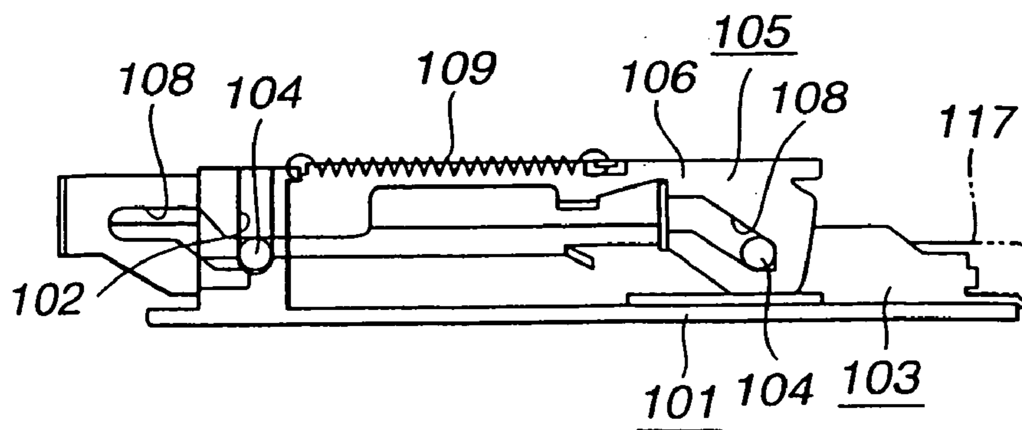
FIG. 5 (PRIOR ART)
