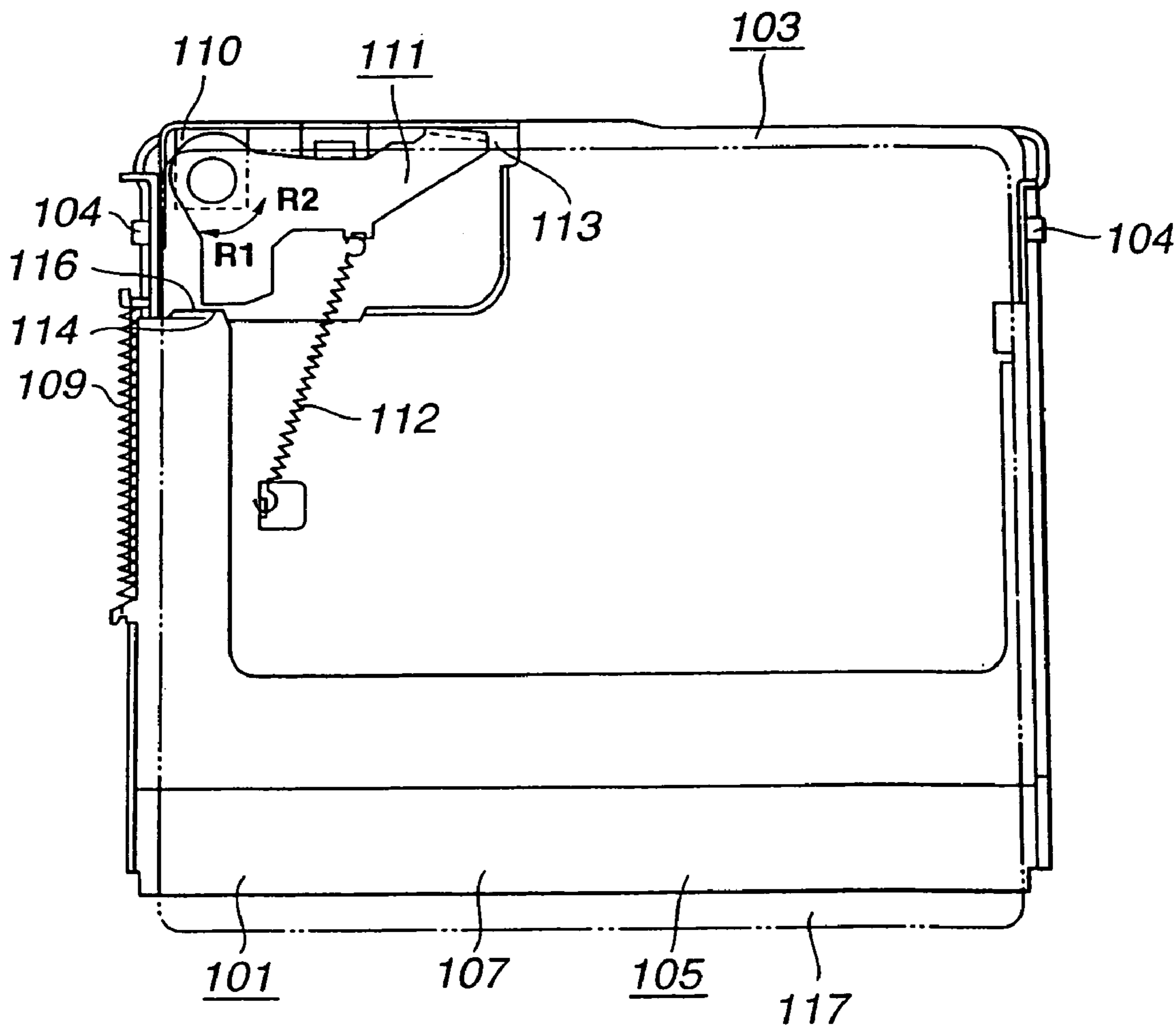
FIG. 3 (PRIOR ART)
