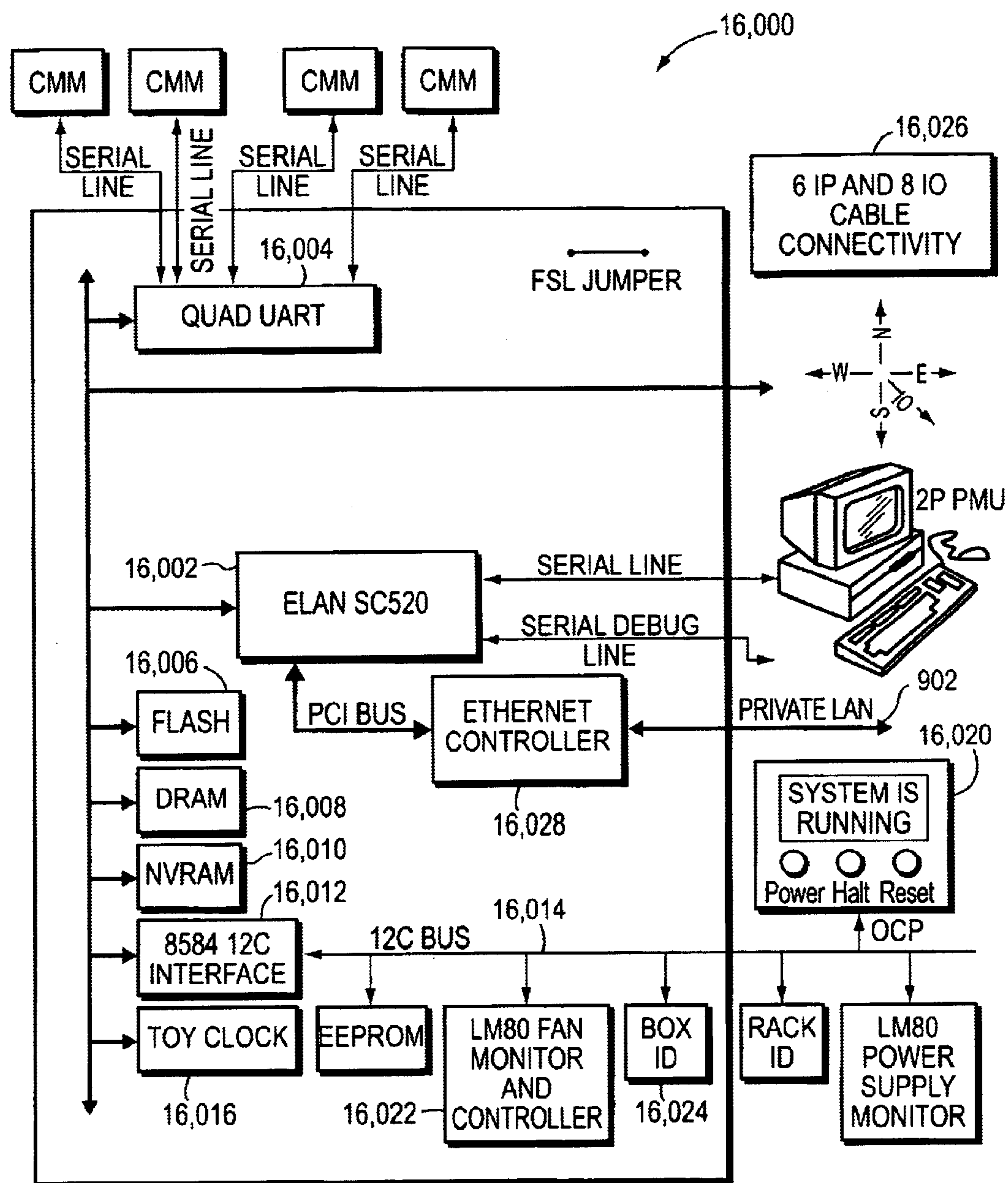
MBM HARDWARE OVERVIEW
