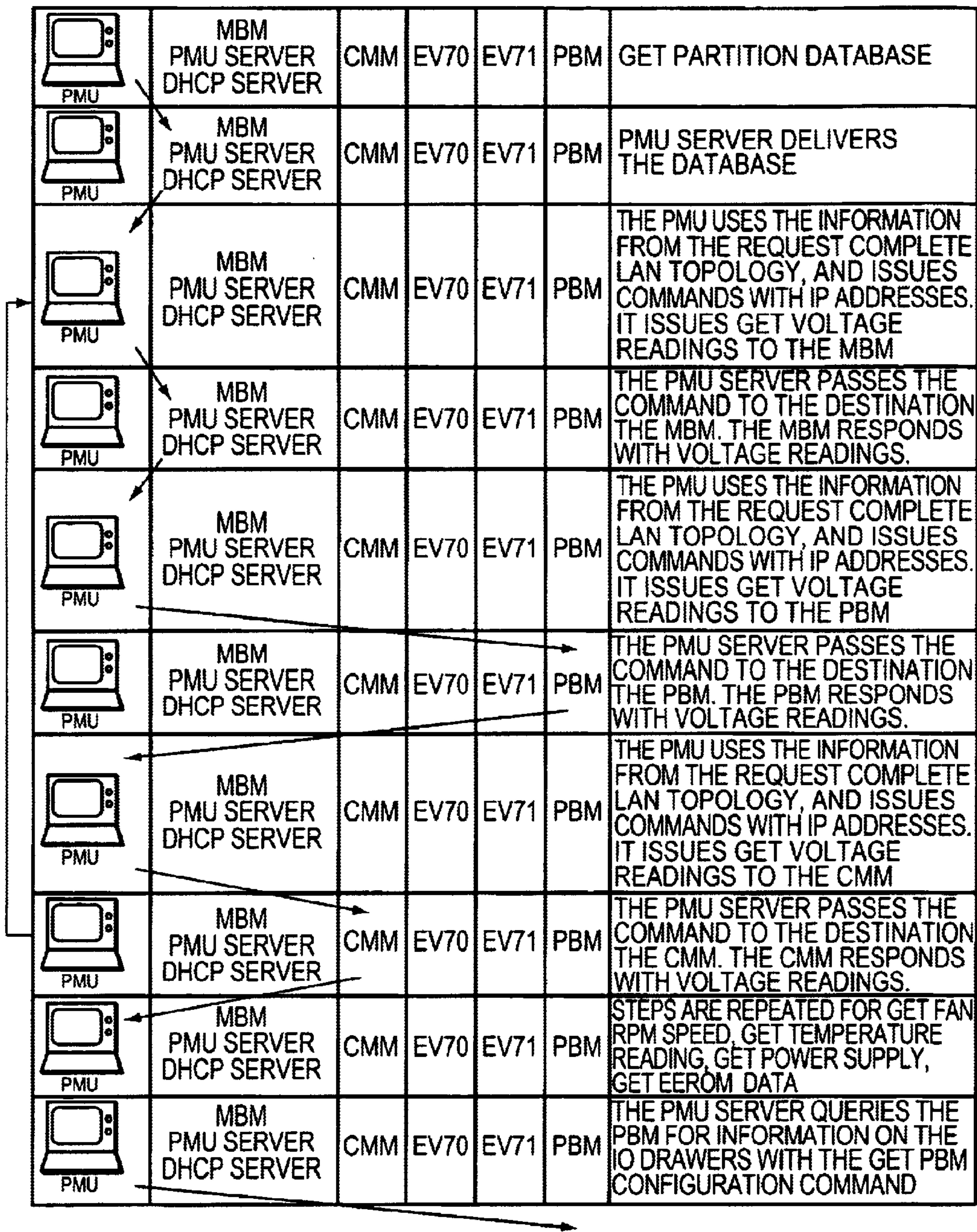
SHOW CONFIGURATION FLOW DIAGRAM (PART 3)
