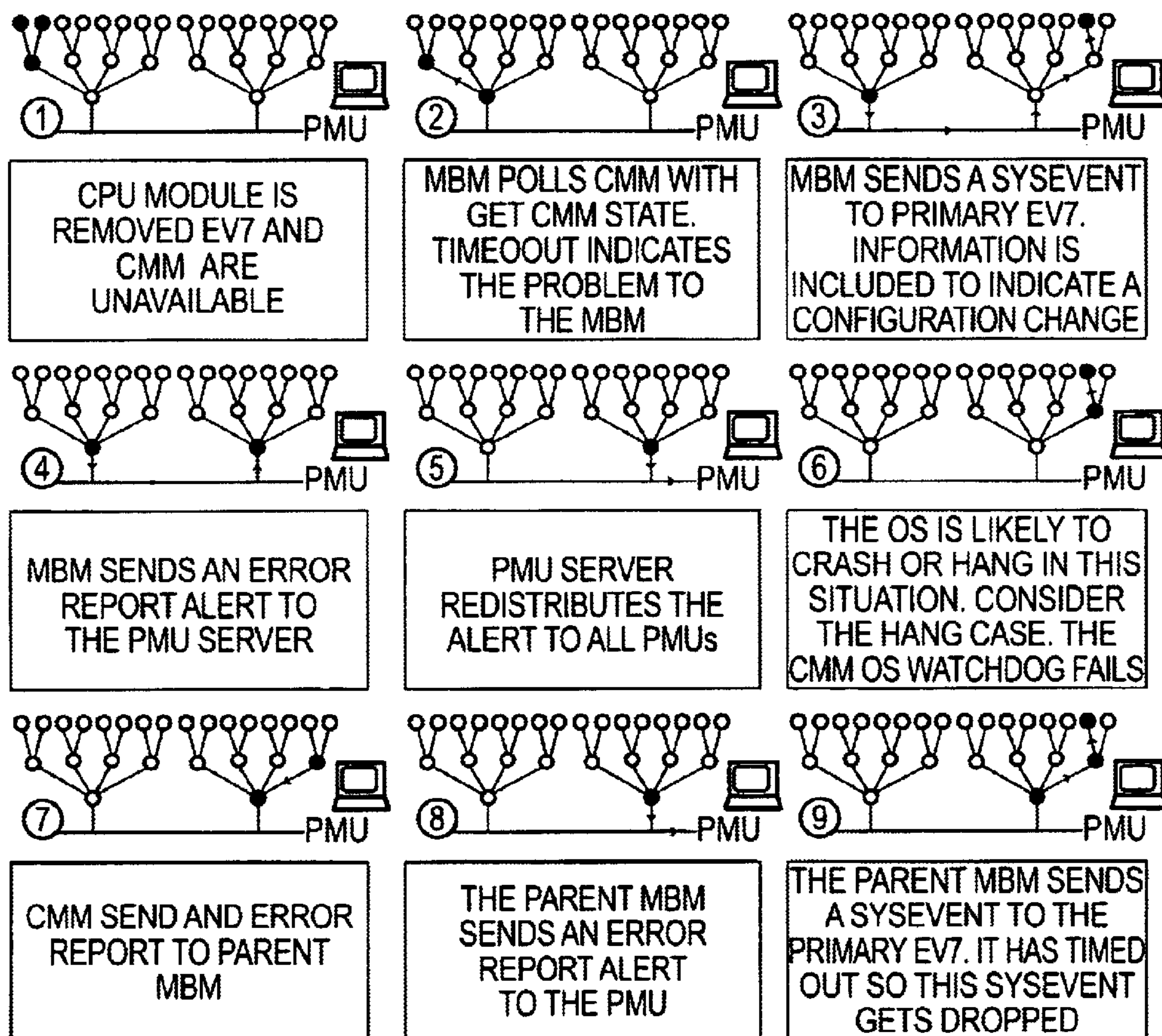
EV7 FAILYRE/REPLACE FLOW DIAGRAM (PART 1)
