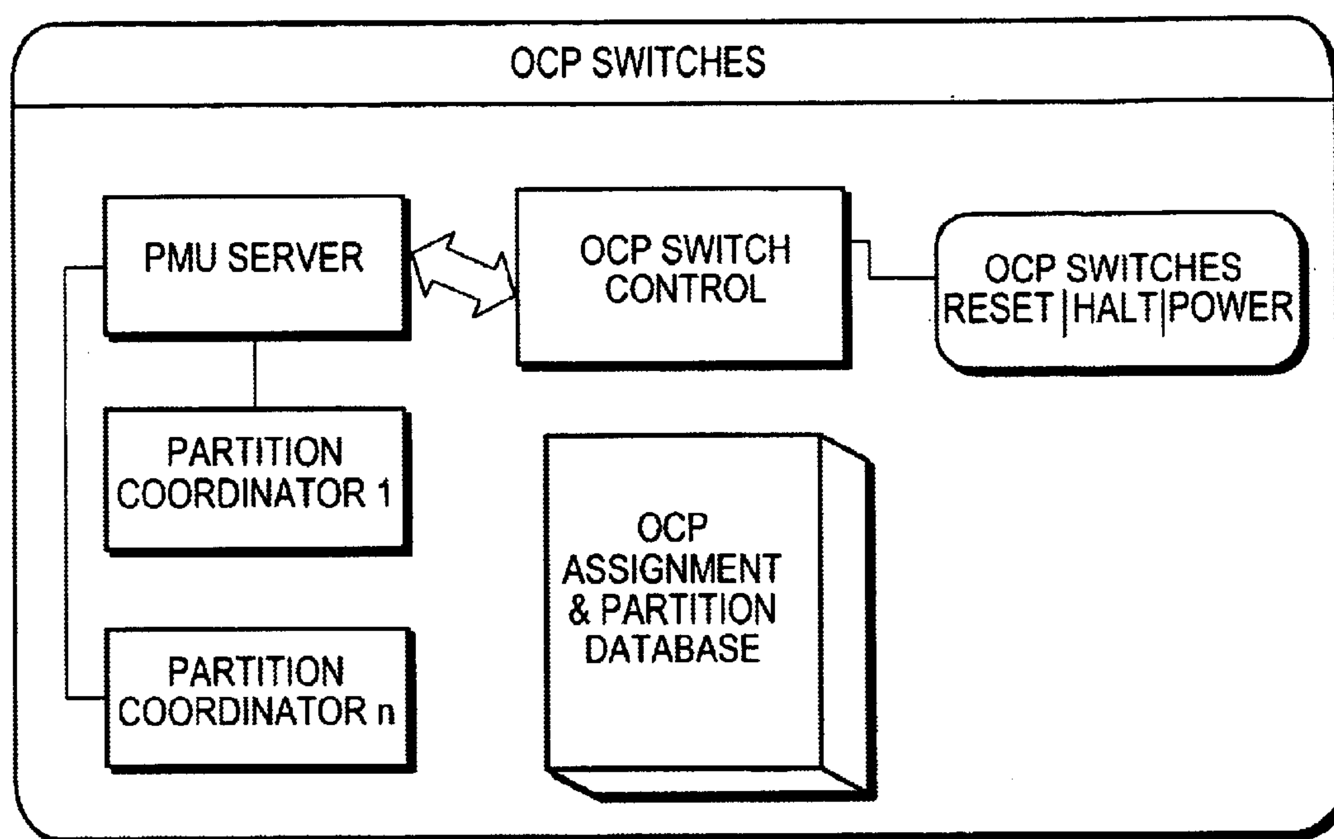
OCP SWITCHES BLOCK DIAGRAM
