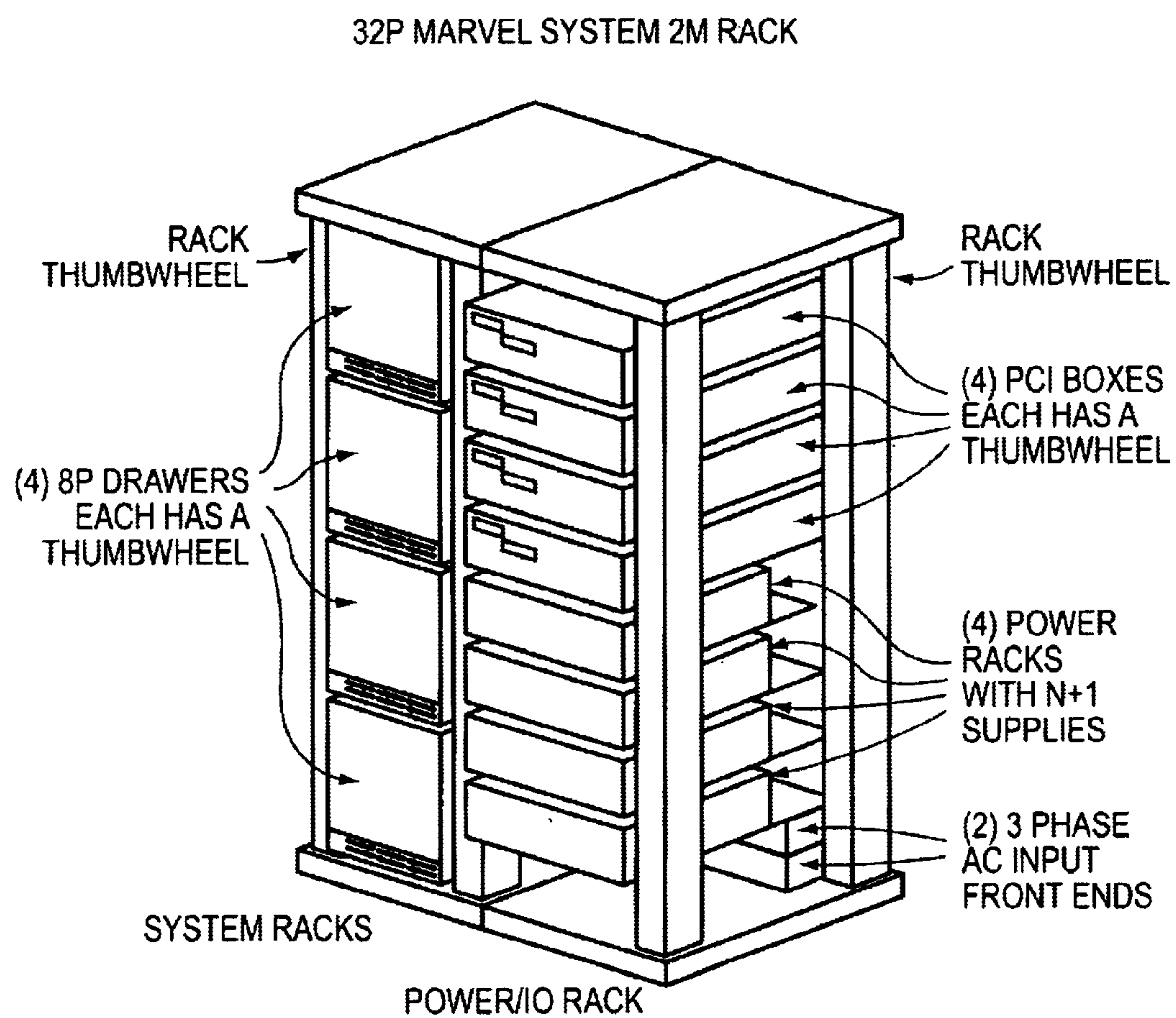
RACK AND BOX THUMBWHEEL SCHEME
