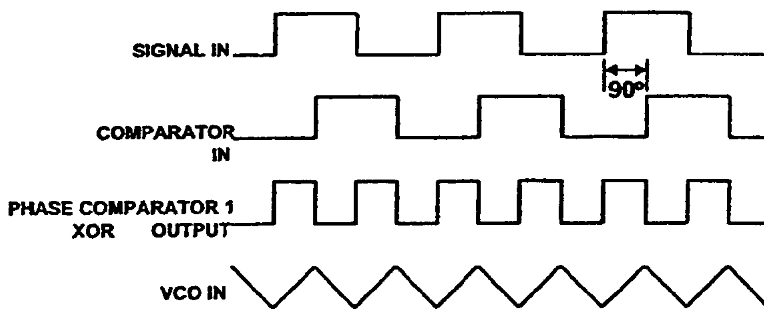
(C) TYPICAL XOR DETECTOR WAVEFORMS
