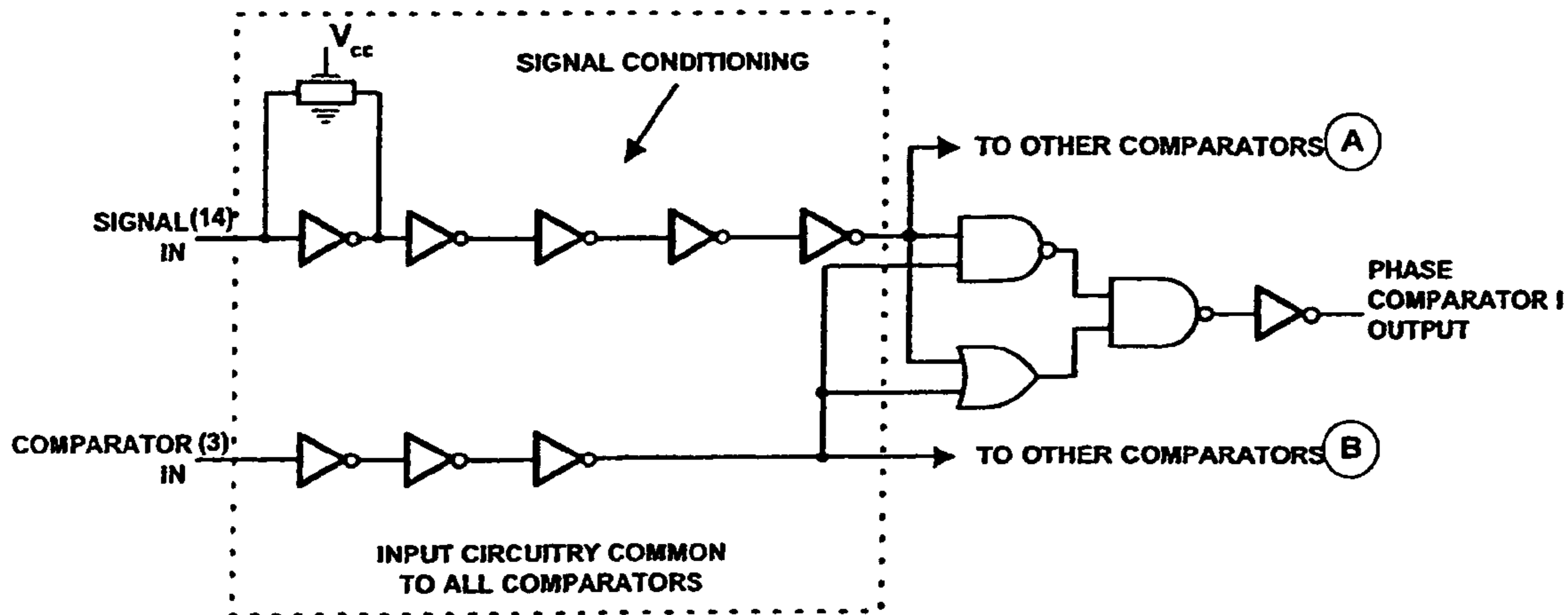
(B) DETAILED ON-CHIP IC CIRCUITRY IN 74HC4046
