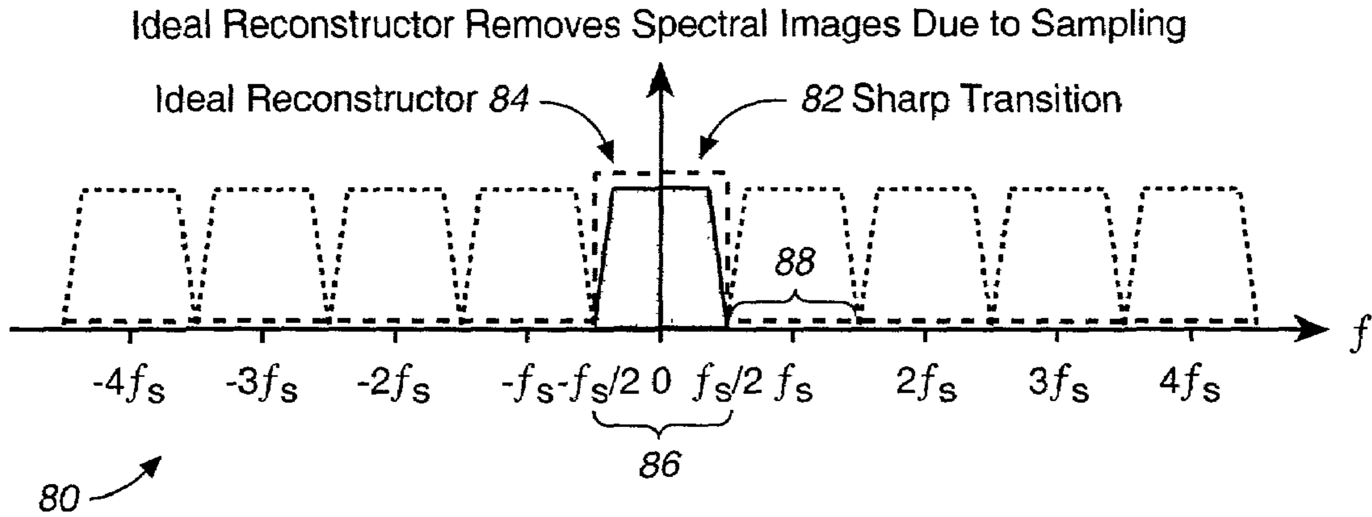
FIG. 5 (PRIOR ART)
