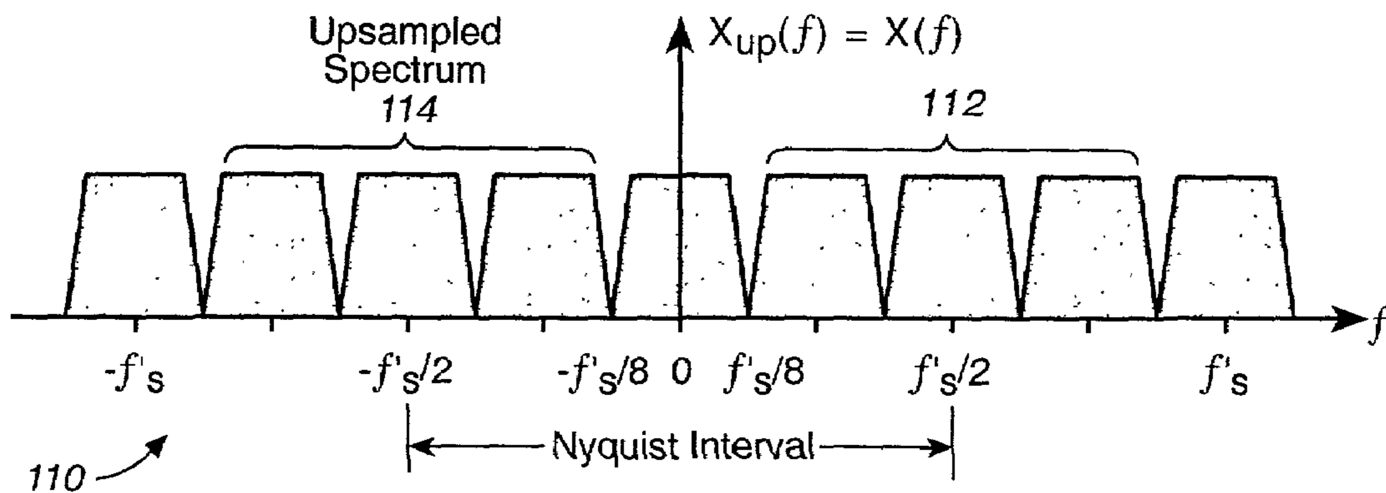
FIG. 7 (PRIOR ART)
