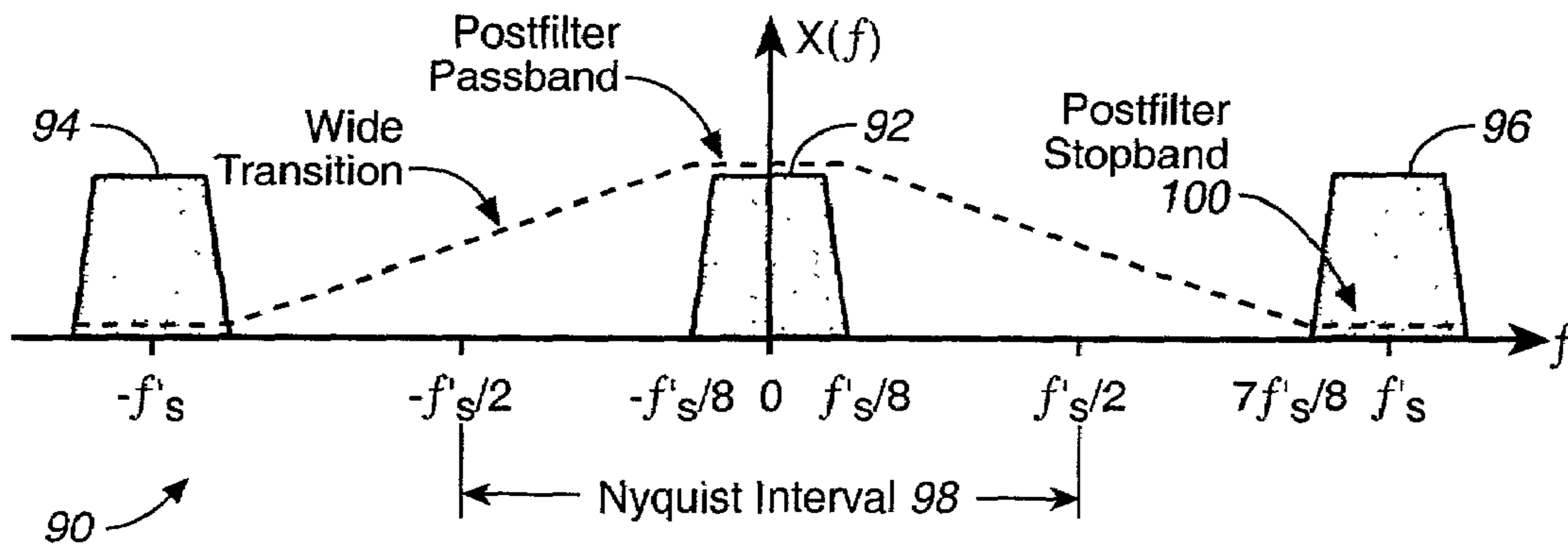
FIG. 6 (PRIOR ART)
