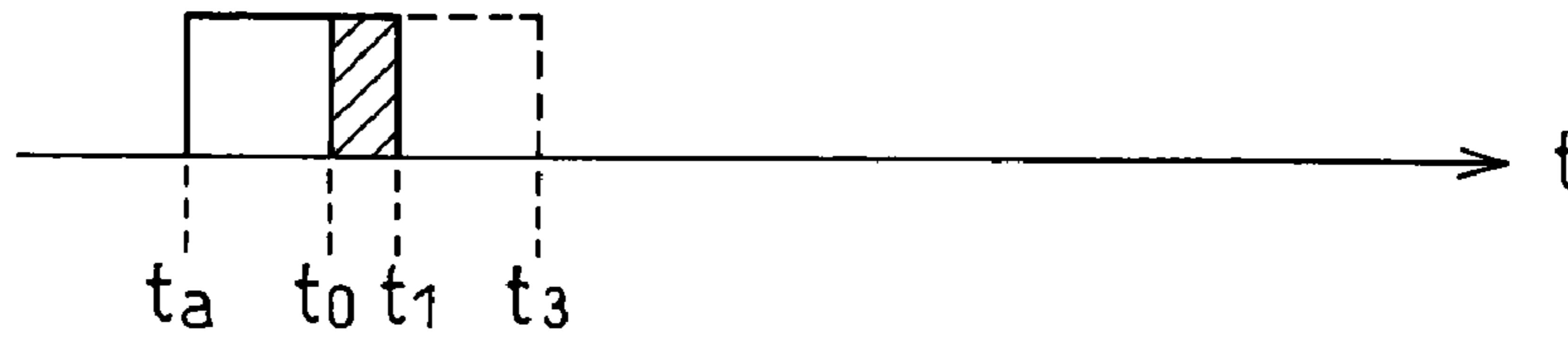
RETURN TIMING OF REFLECTED WAVE FROM SHORT-RANGE TARGET
