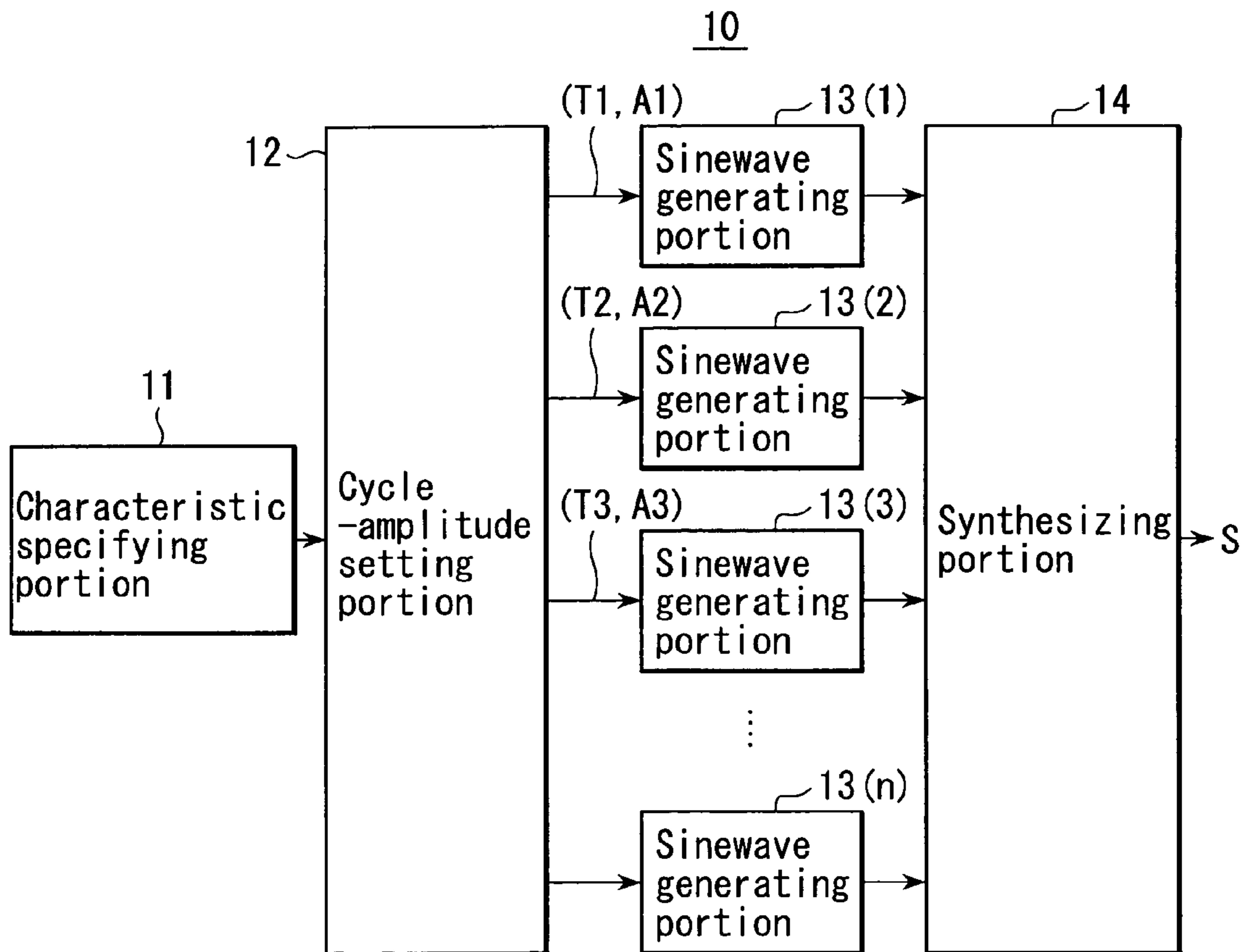
FIG. 8 (PRIOR ART)
