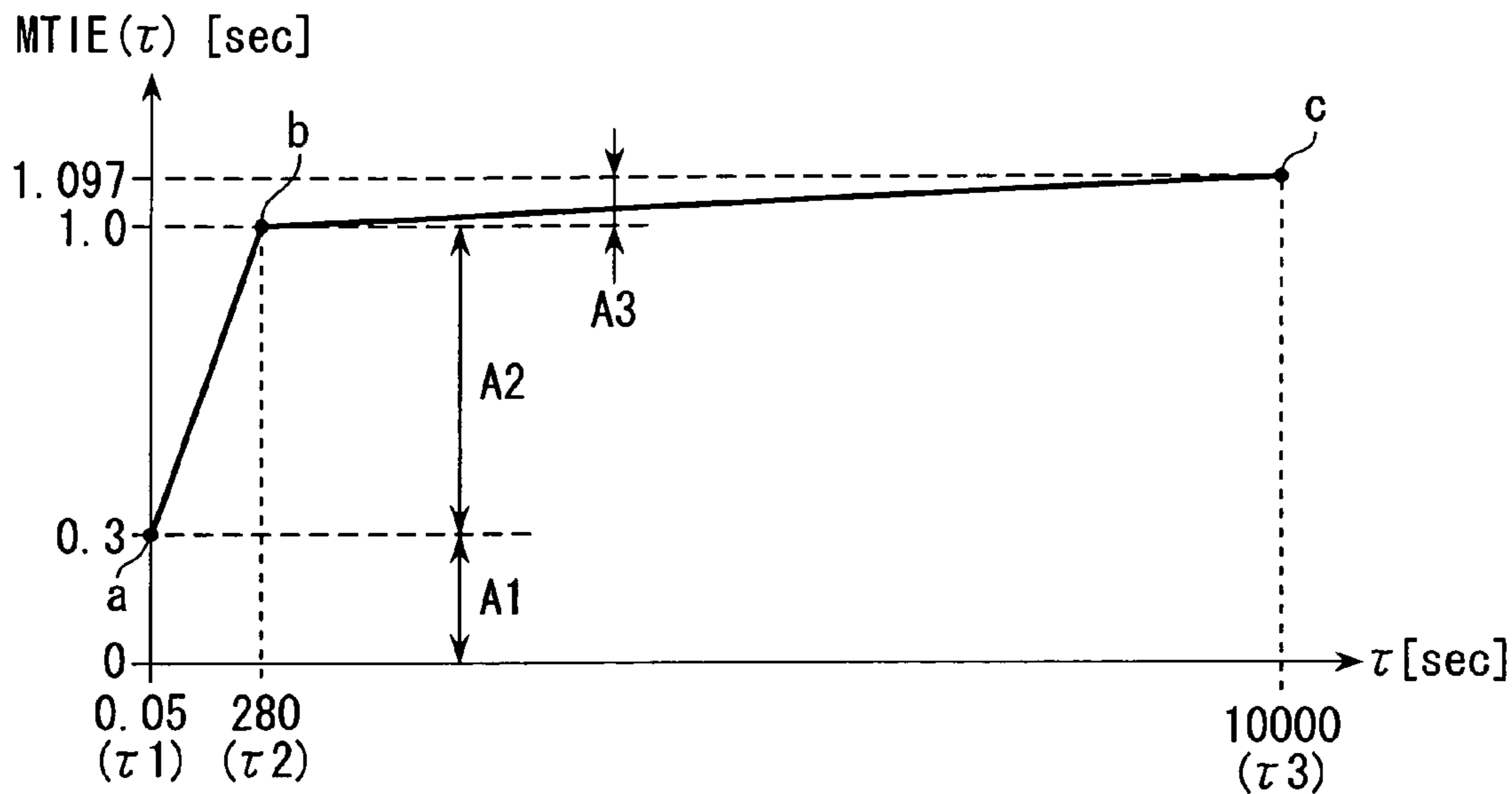
FIG. 7 (PRIOR ART)
