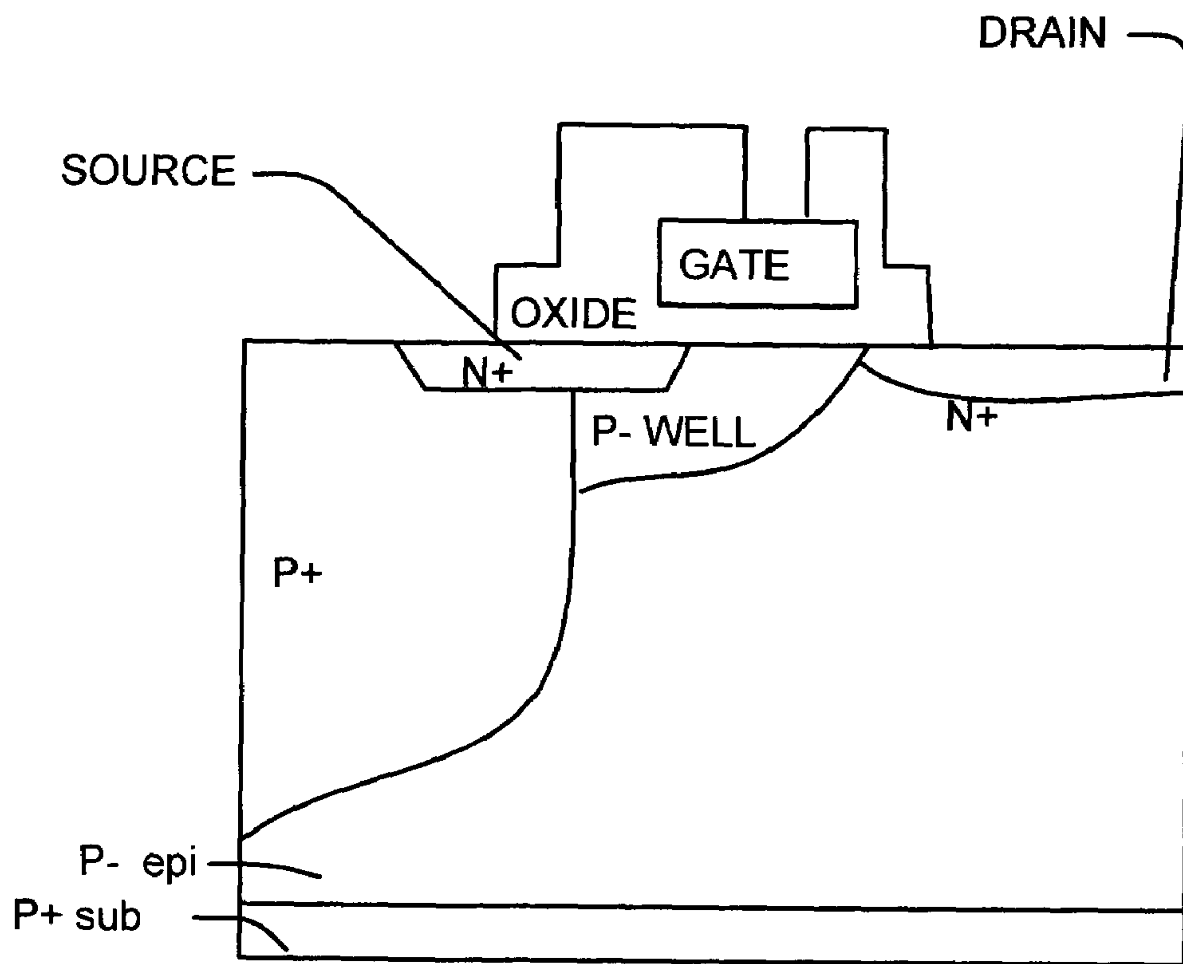
NON-OFFSET LDMOS
