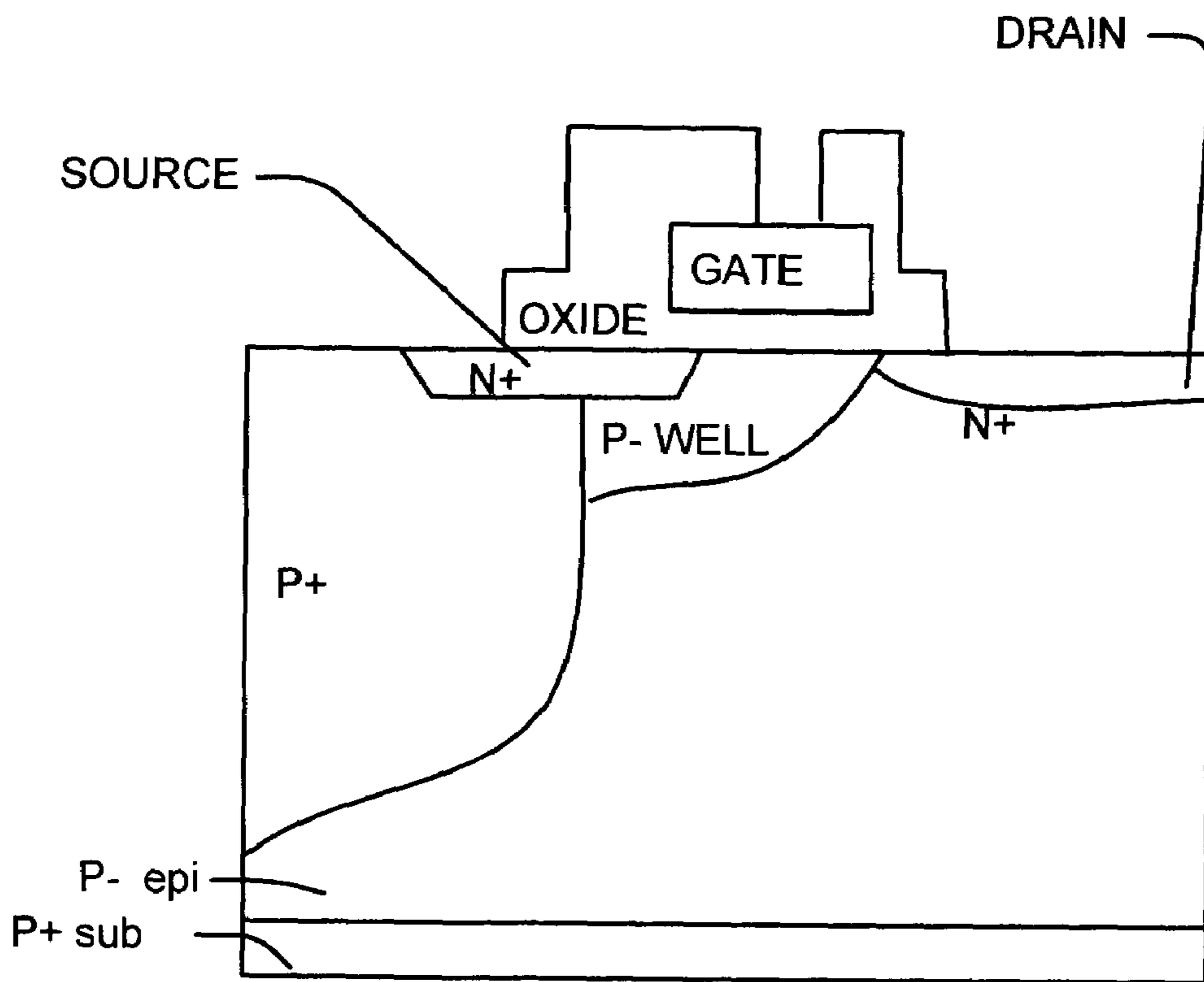
NON-OFFSET LDMOS
