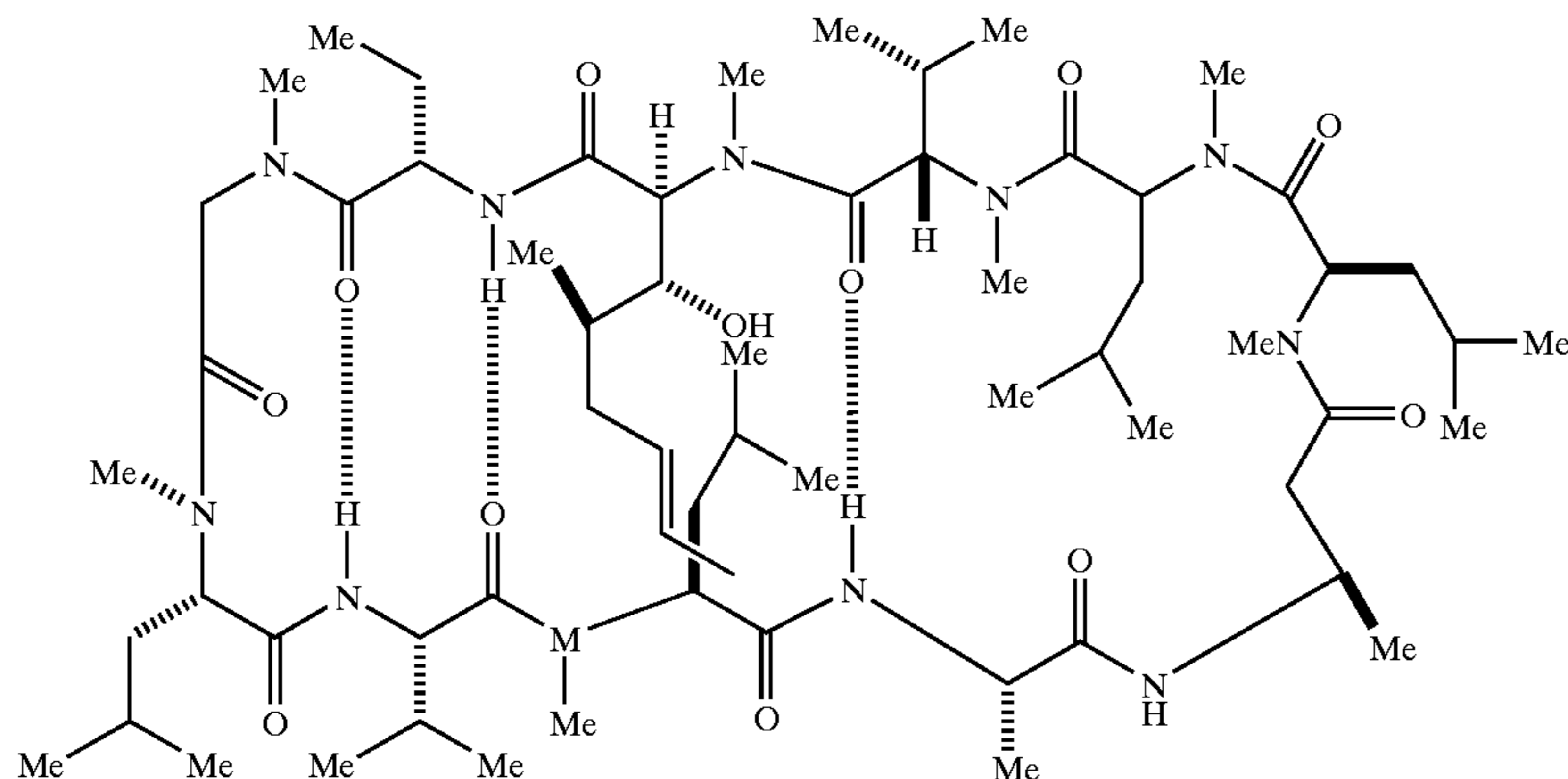
1 (R = Me): CsA 2 (R ≠ Me): Modified [MeVal 11 ]CsA
