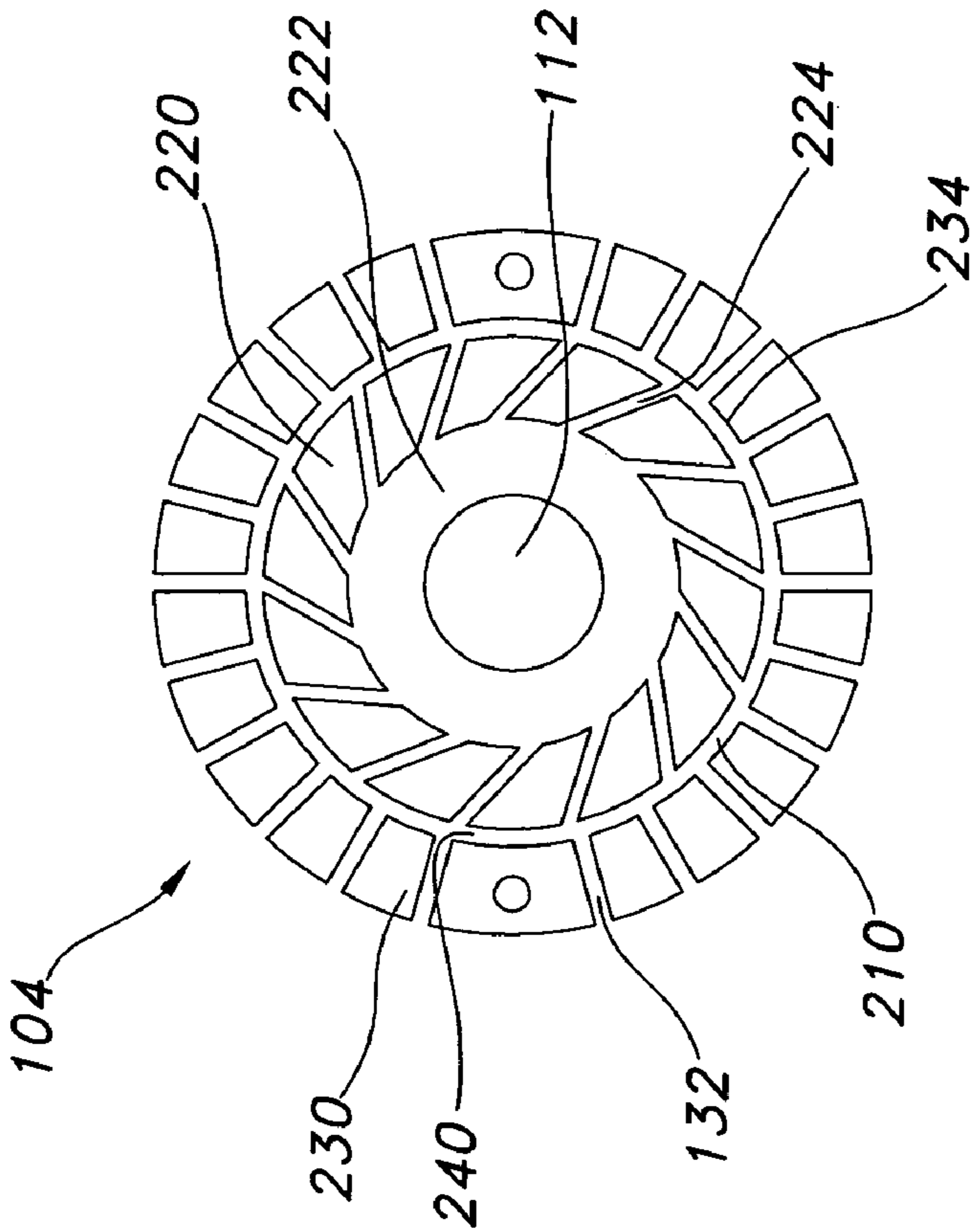
FIG. 2 (PRIOR ART)
