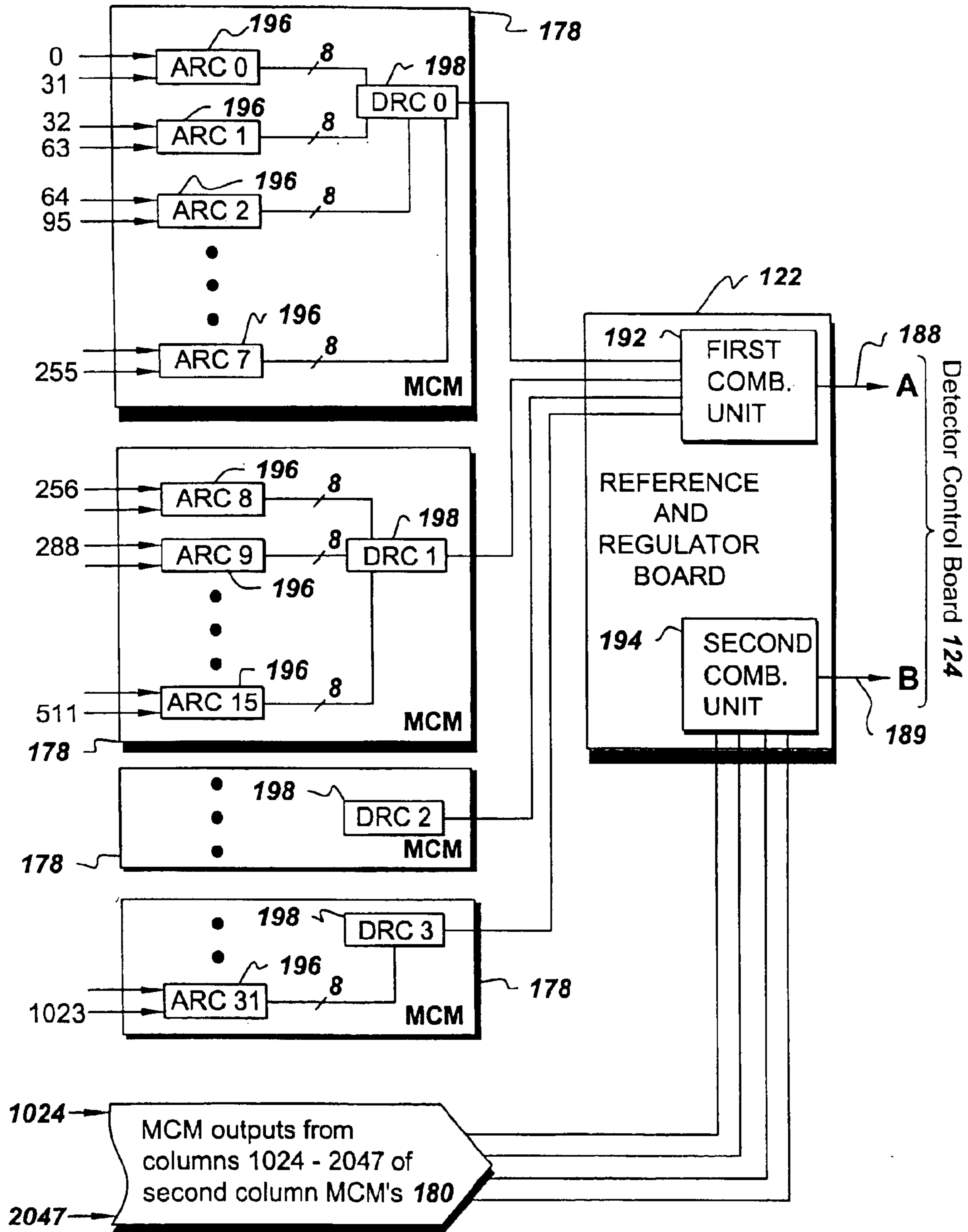
fig. 9 (PRIOR ART)
