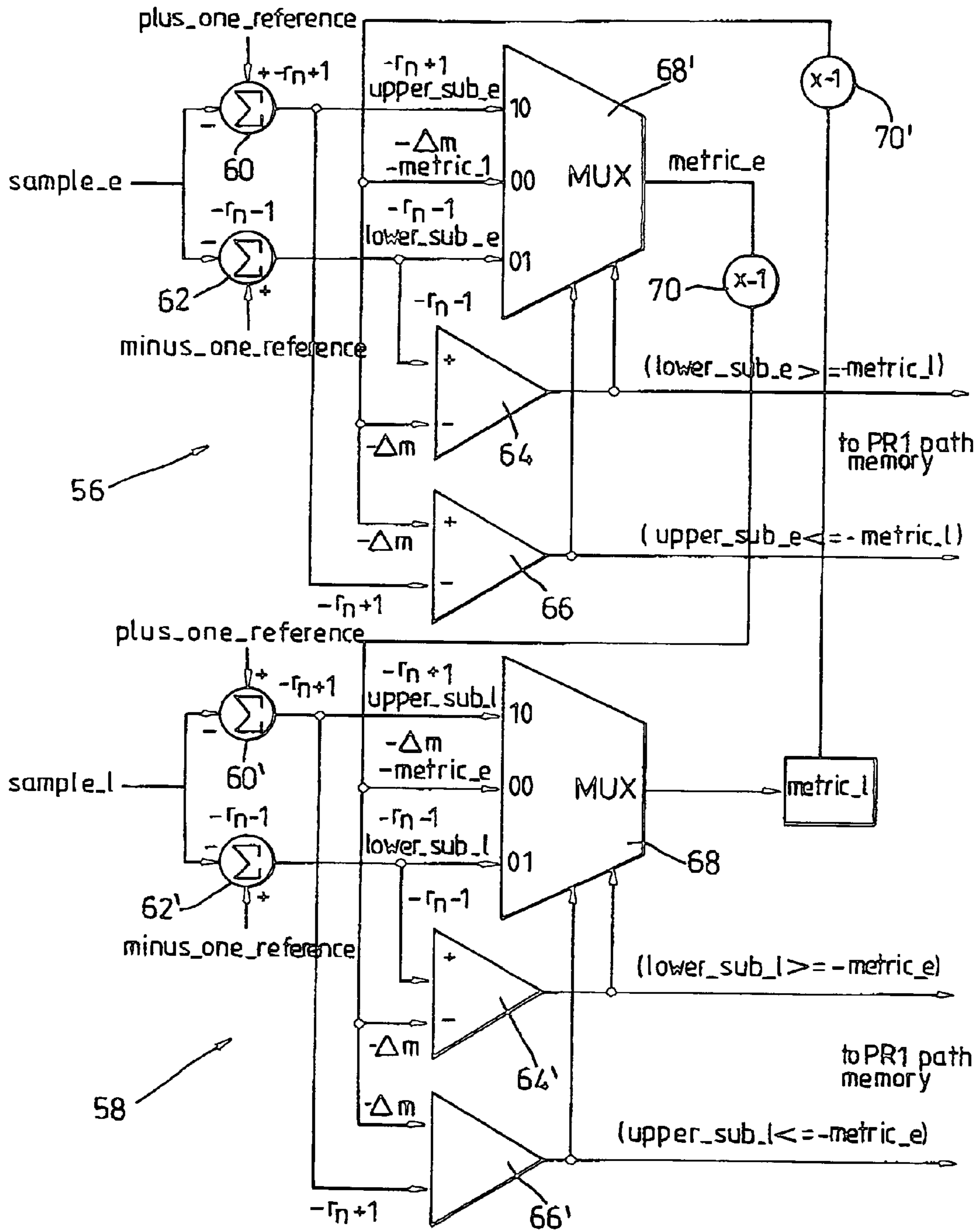
Half Rate PR1 Viterbi Engine
