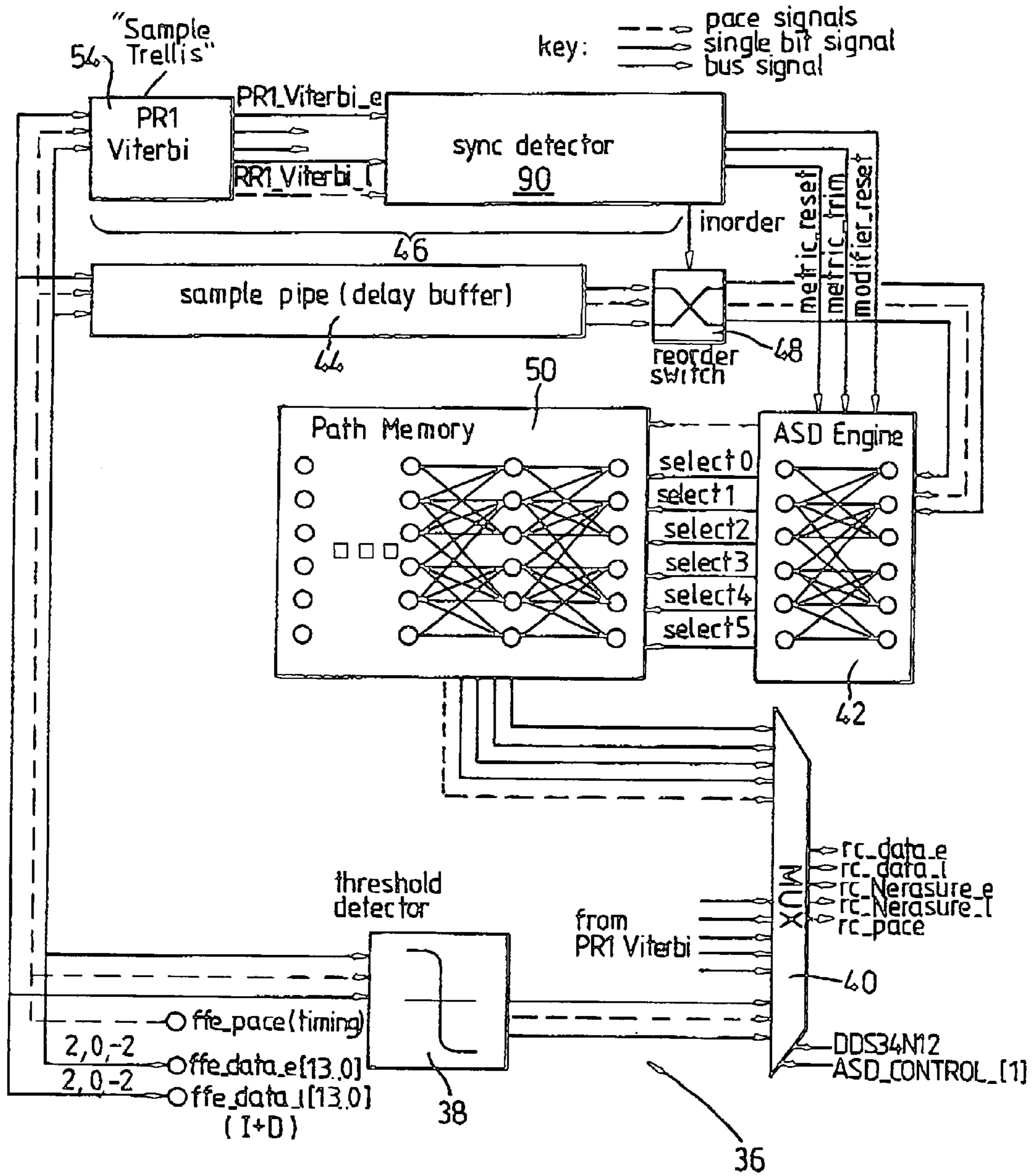
Sequence Detector top level
