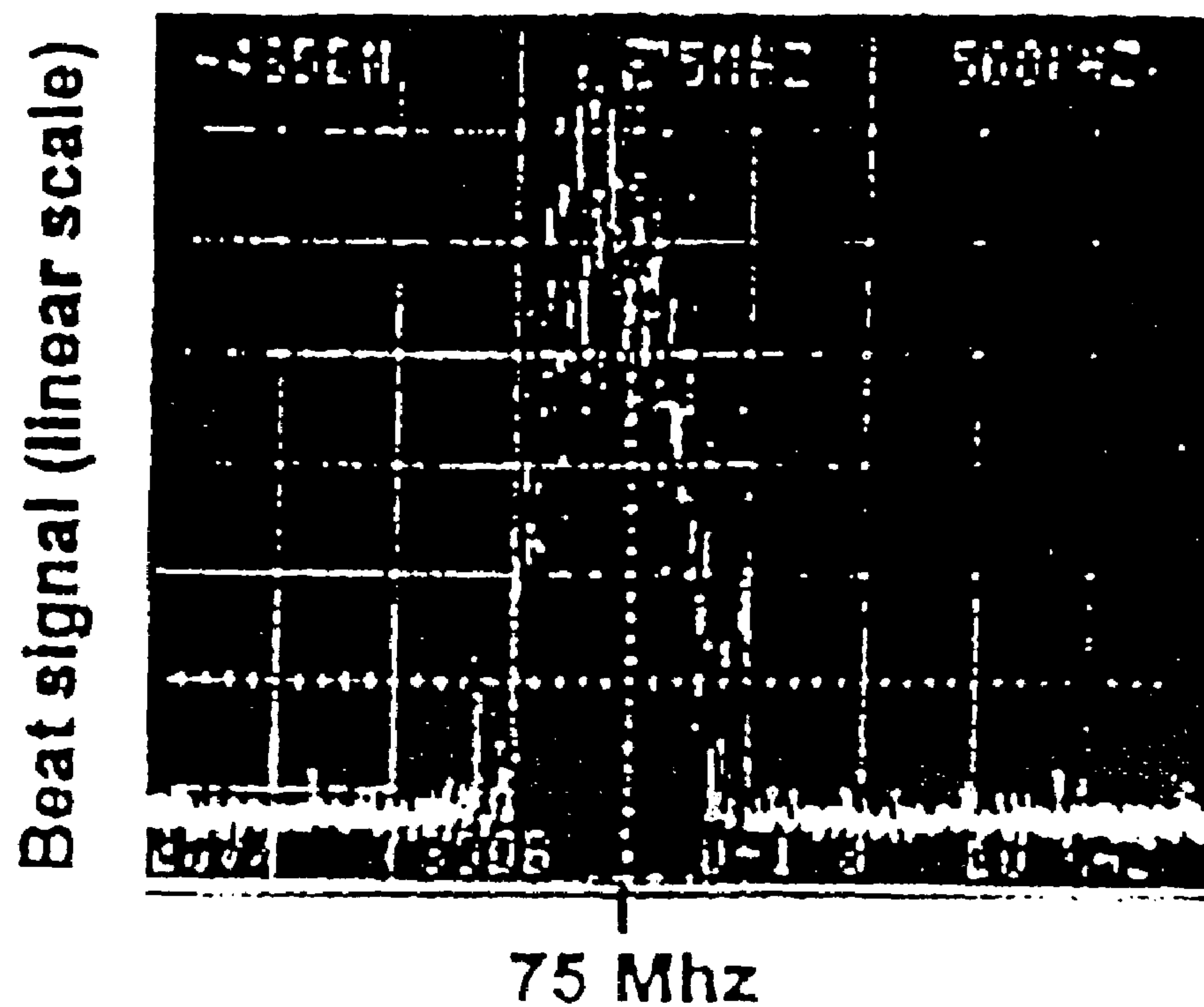
FIG. 1-A4 Frequency (500 kHz/div.)
