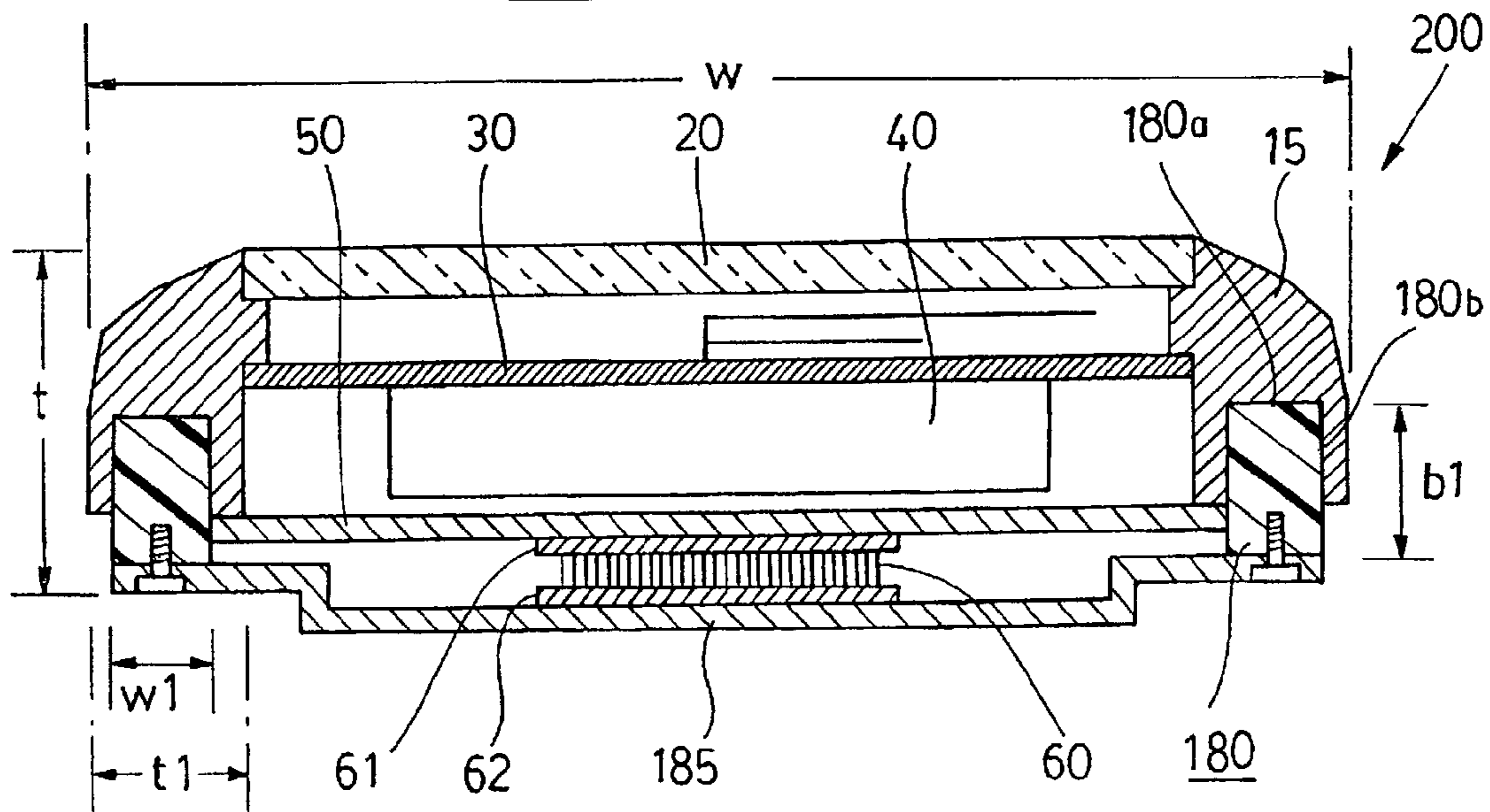
FIG. 20 PRIOR ART
