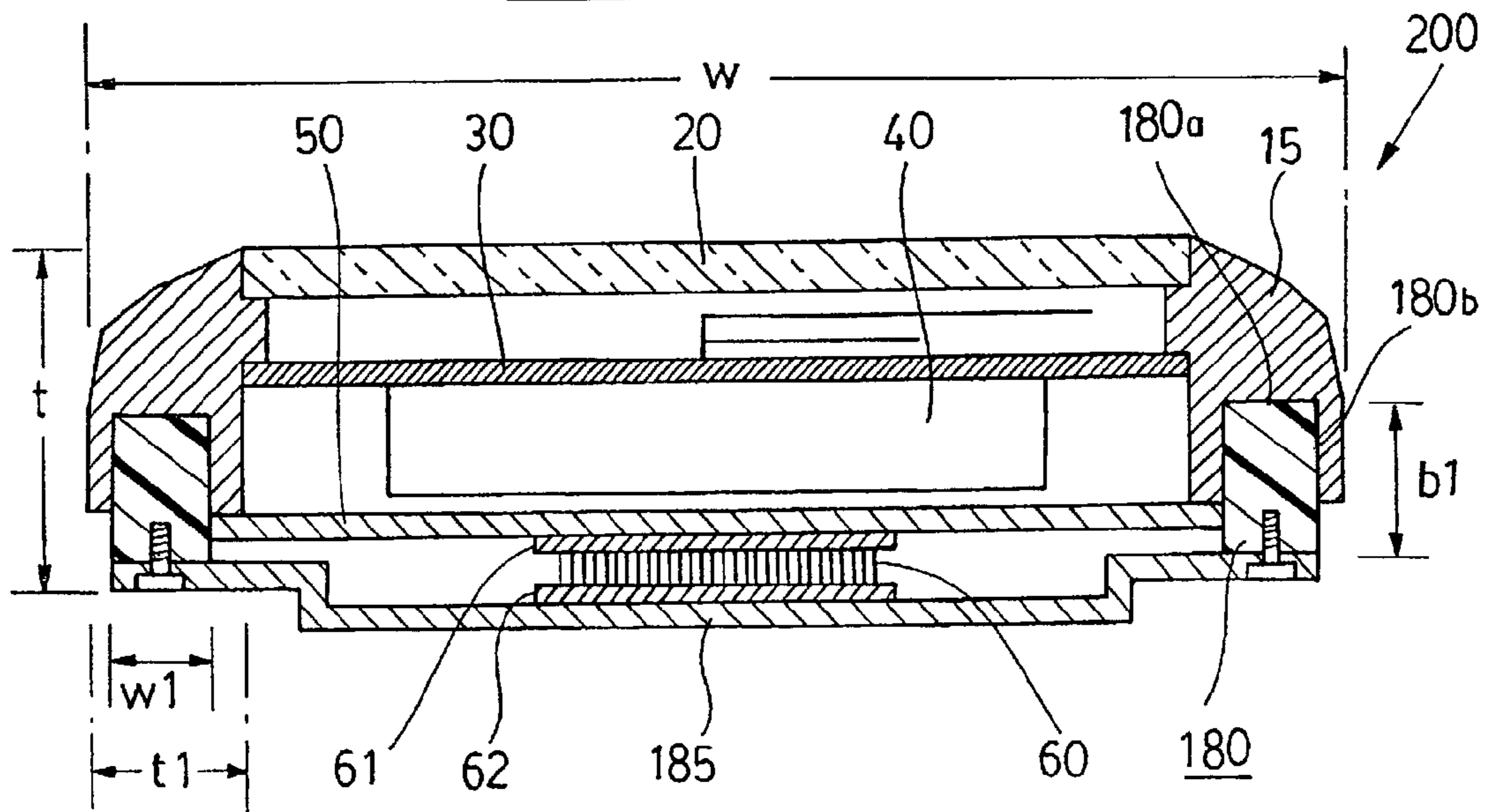
FIG. 20 PRIOR ART
