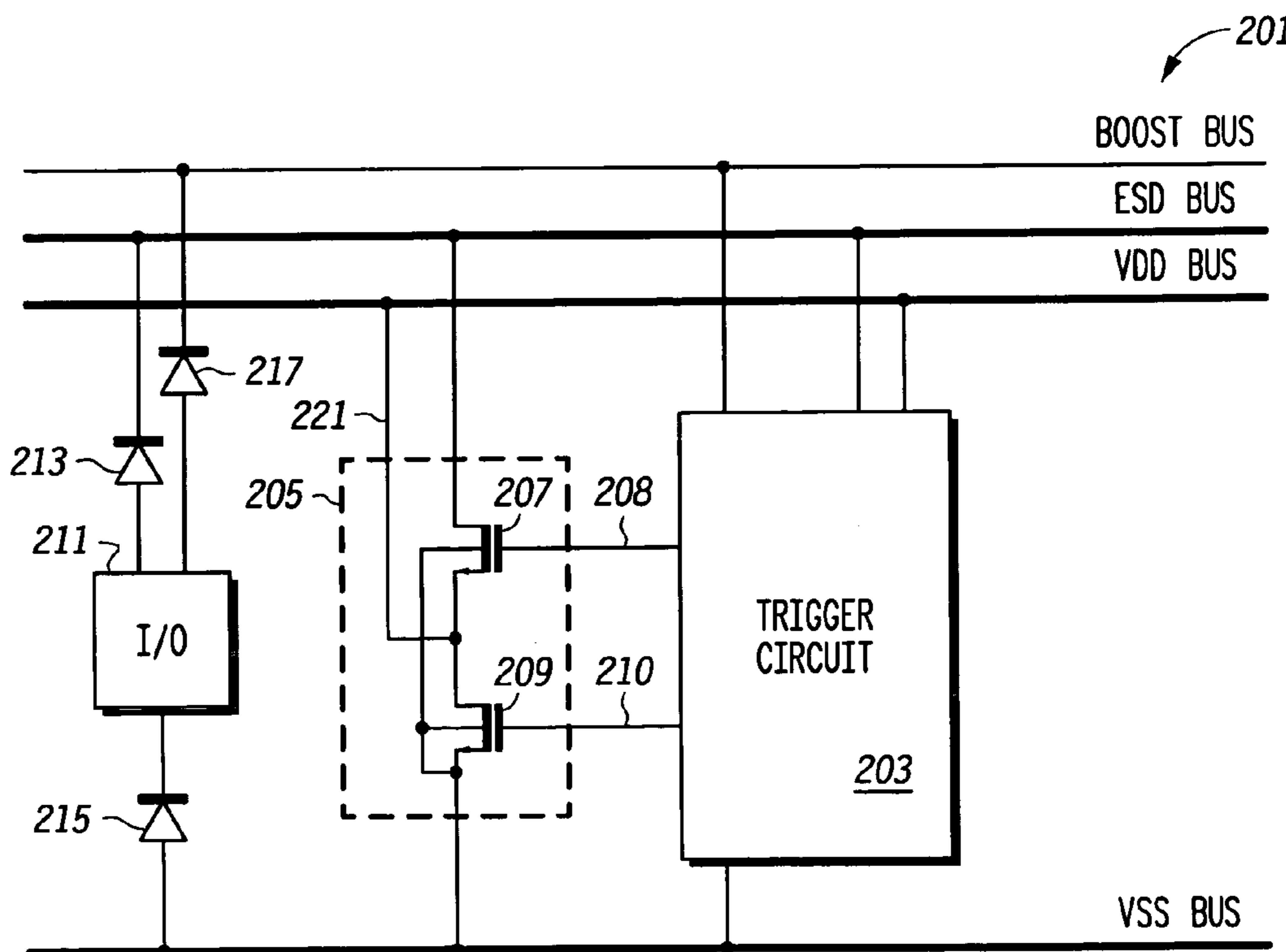
FIG. 1 -PRIOR ART-
