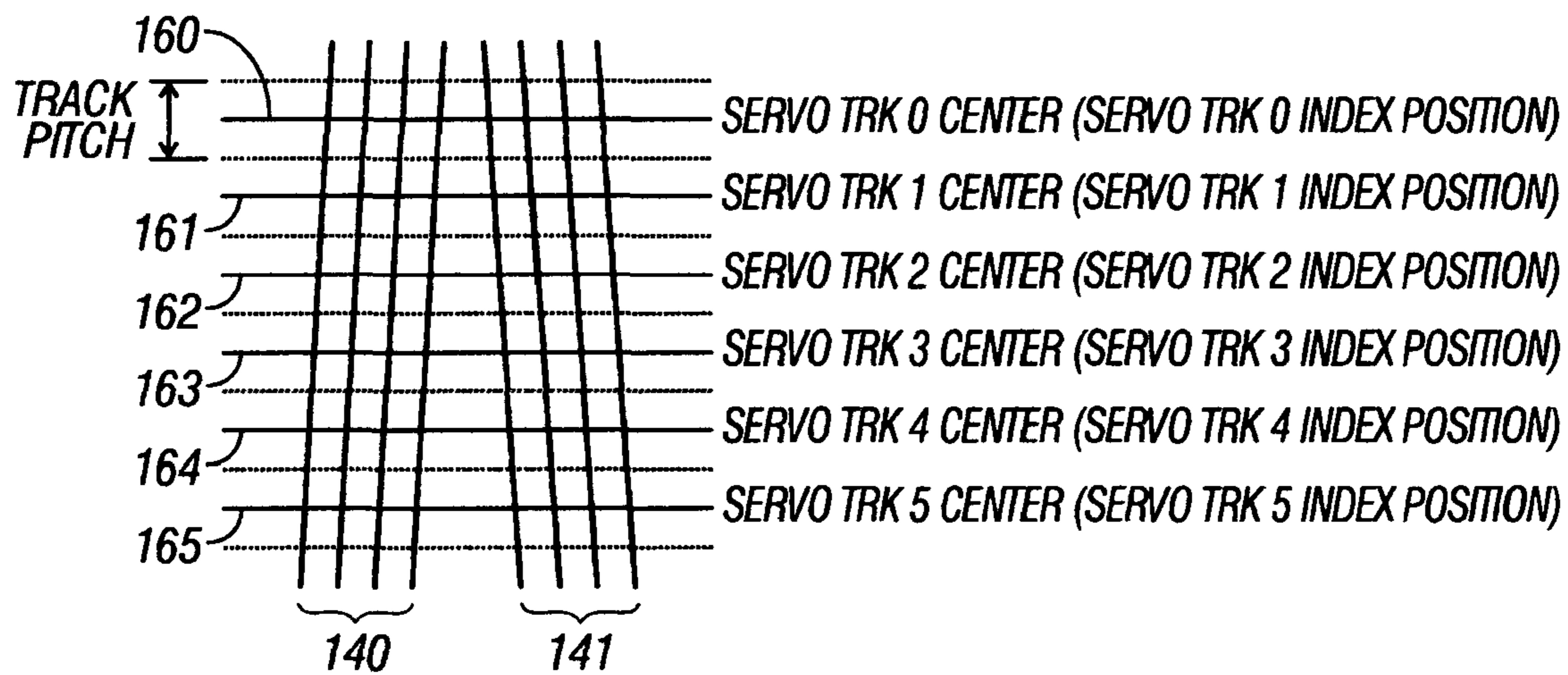
FIG. 5 (PRIOR ART)
