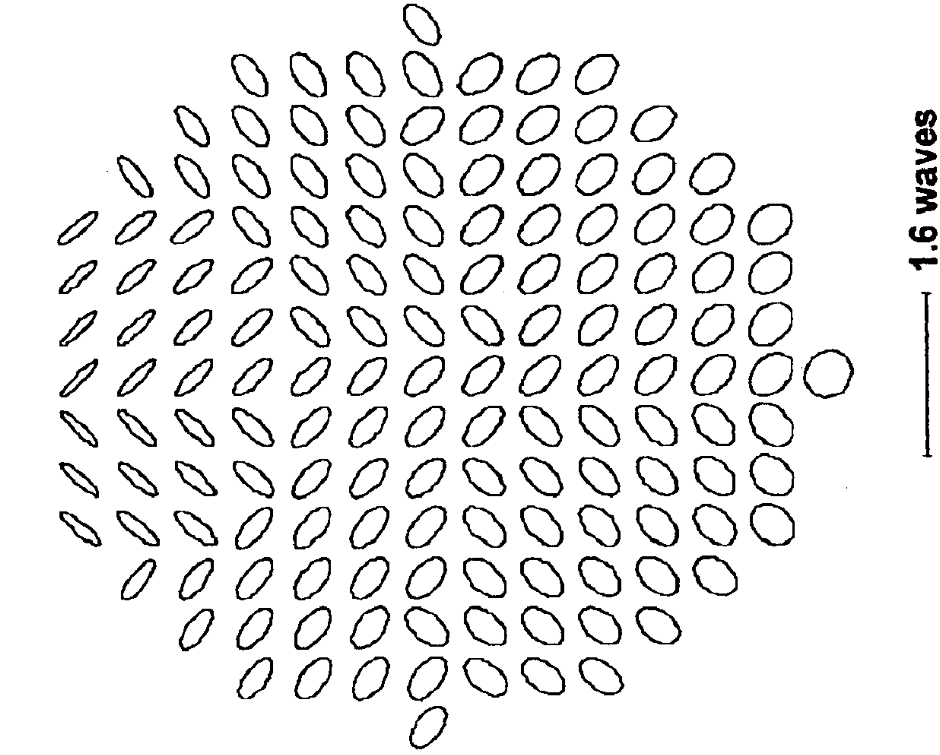
Net Retardance All Elements Plus Rotator 1, Extreme Field
