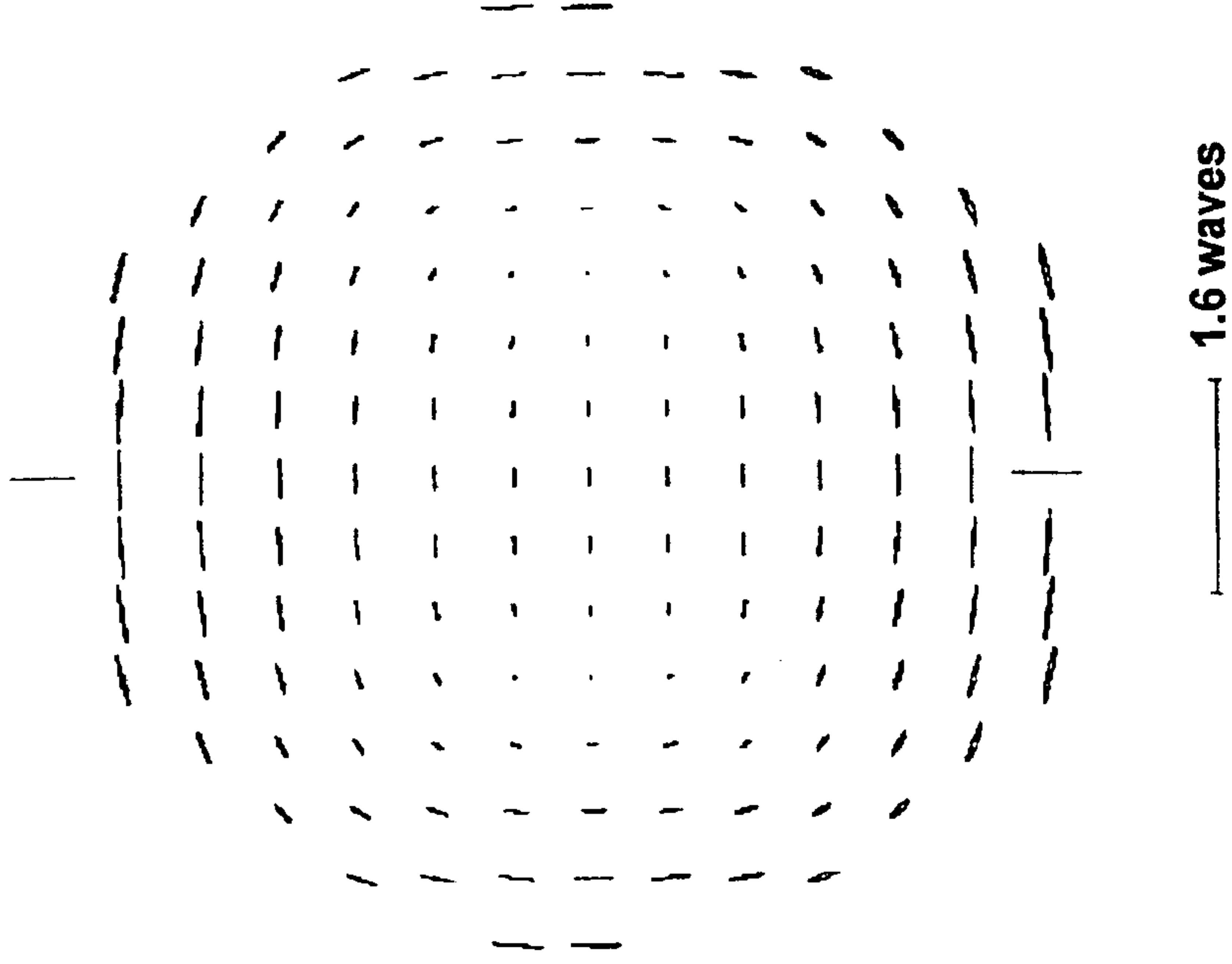
Retardance, Extreme Field
