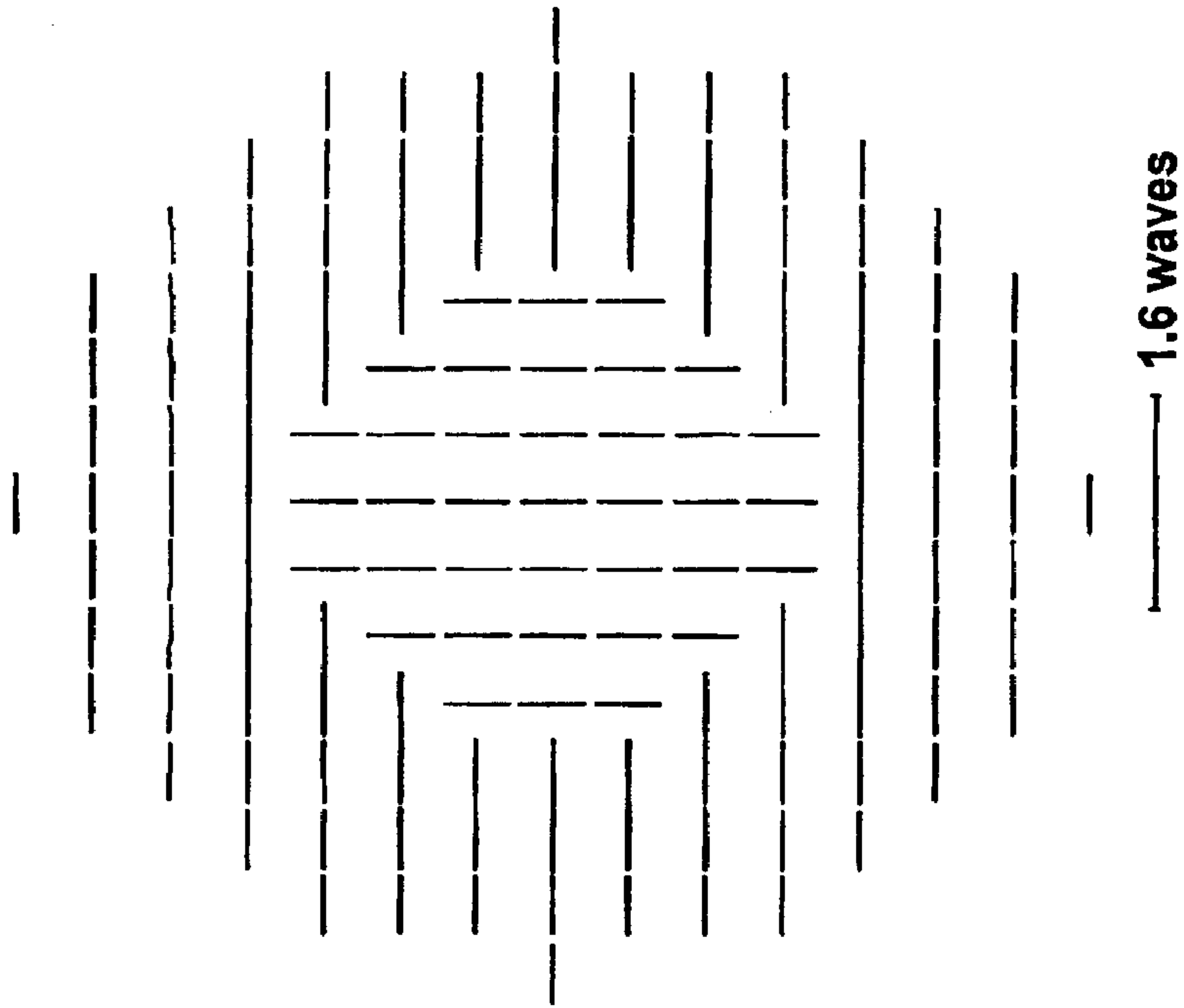
Net Retardance without Rotator, On-Axis Field
