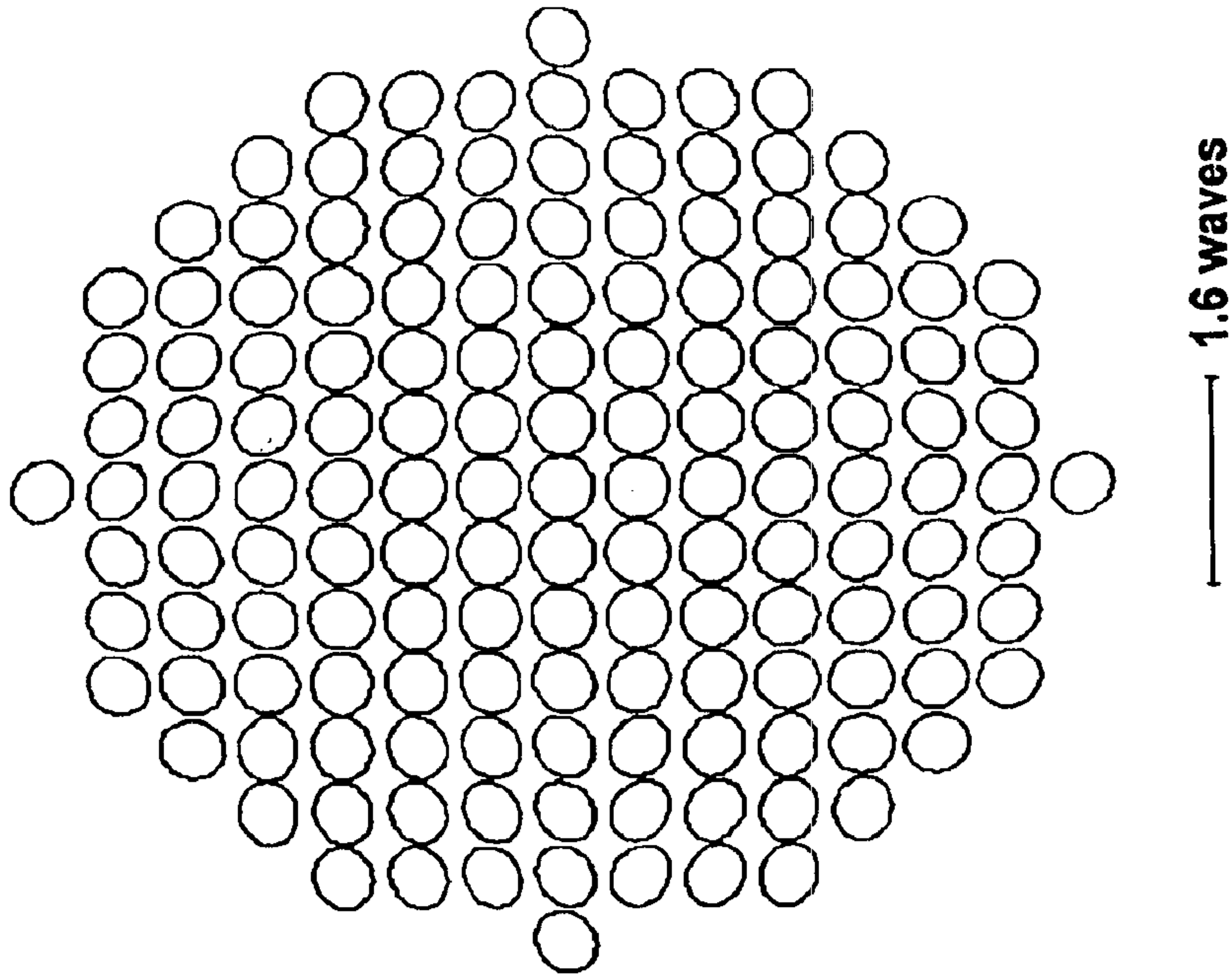
Net Retardance All Elements Plus Rotator 1, On-Axis Field
