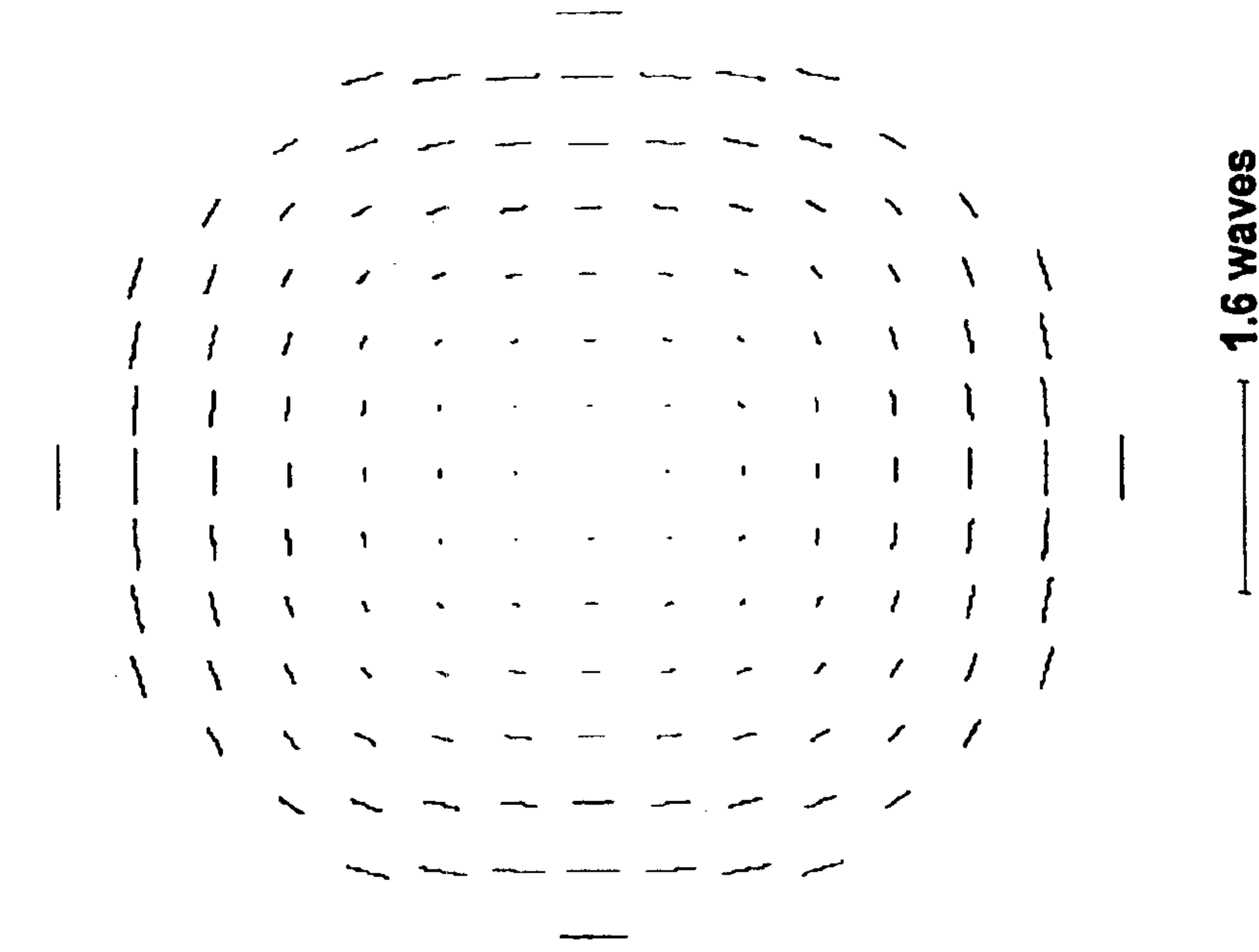
Retardance, On-Axis Field
