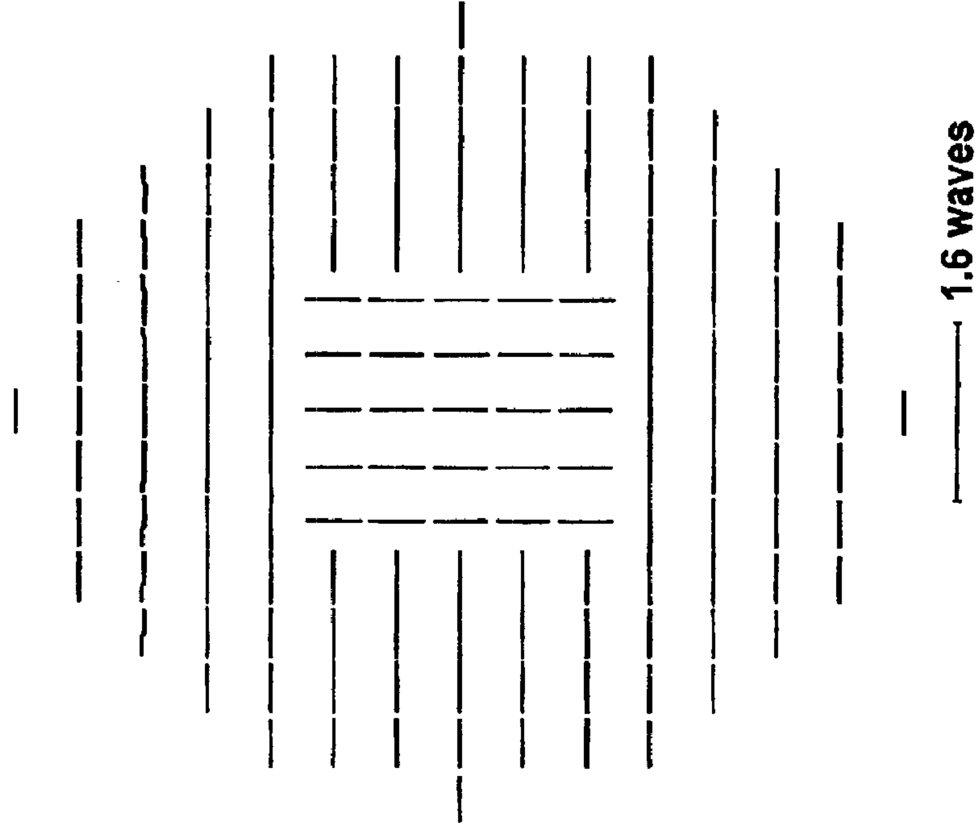
Net Retardance without Rotator, Extreme Field
