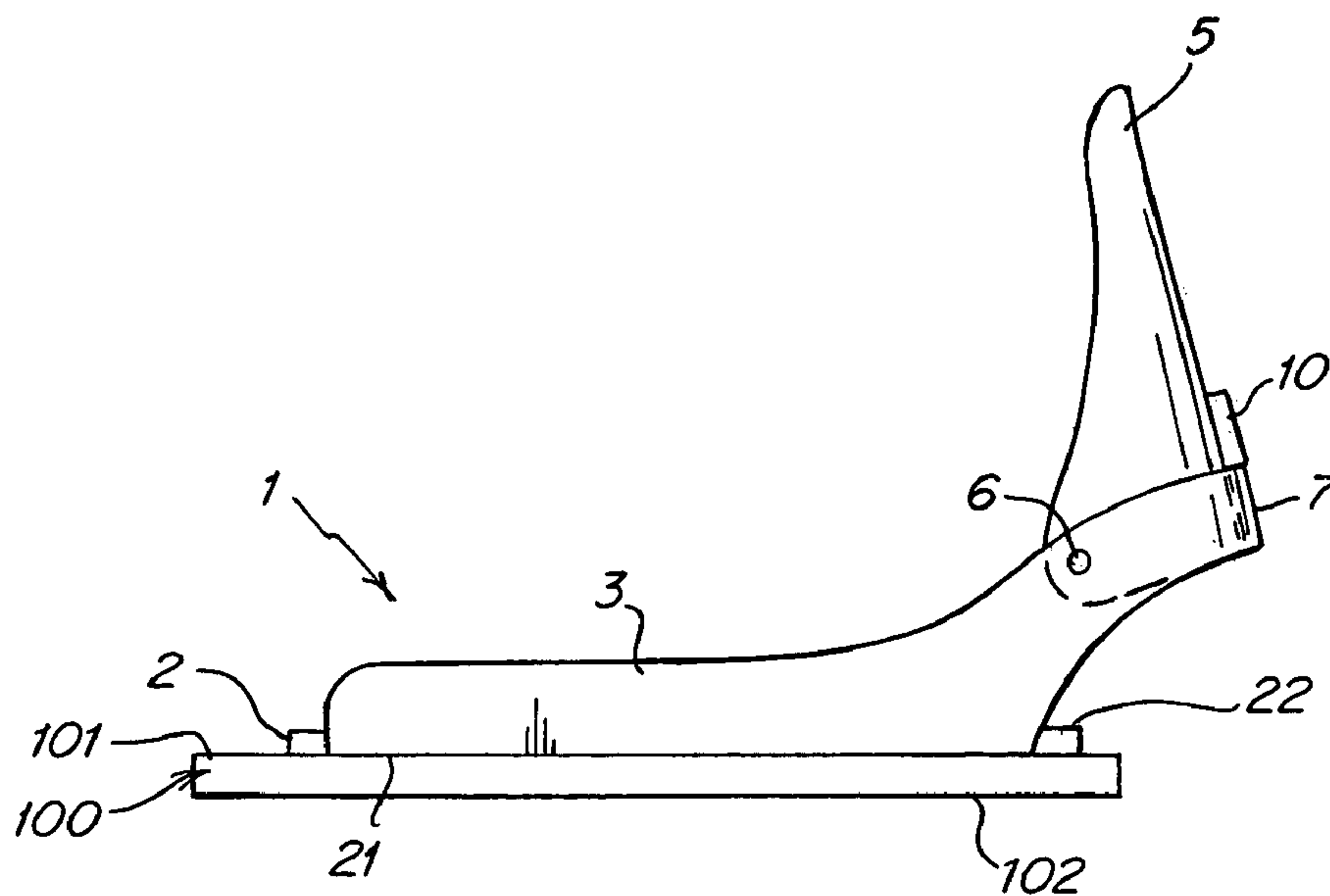
Fig. 16 PRIOR ART
