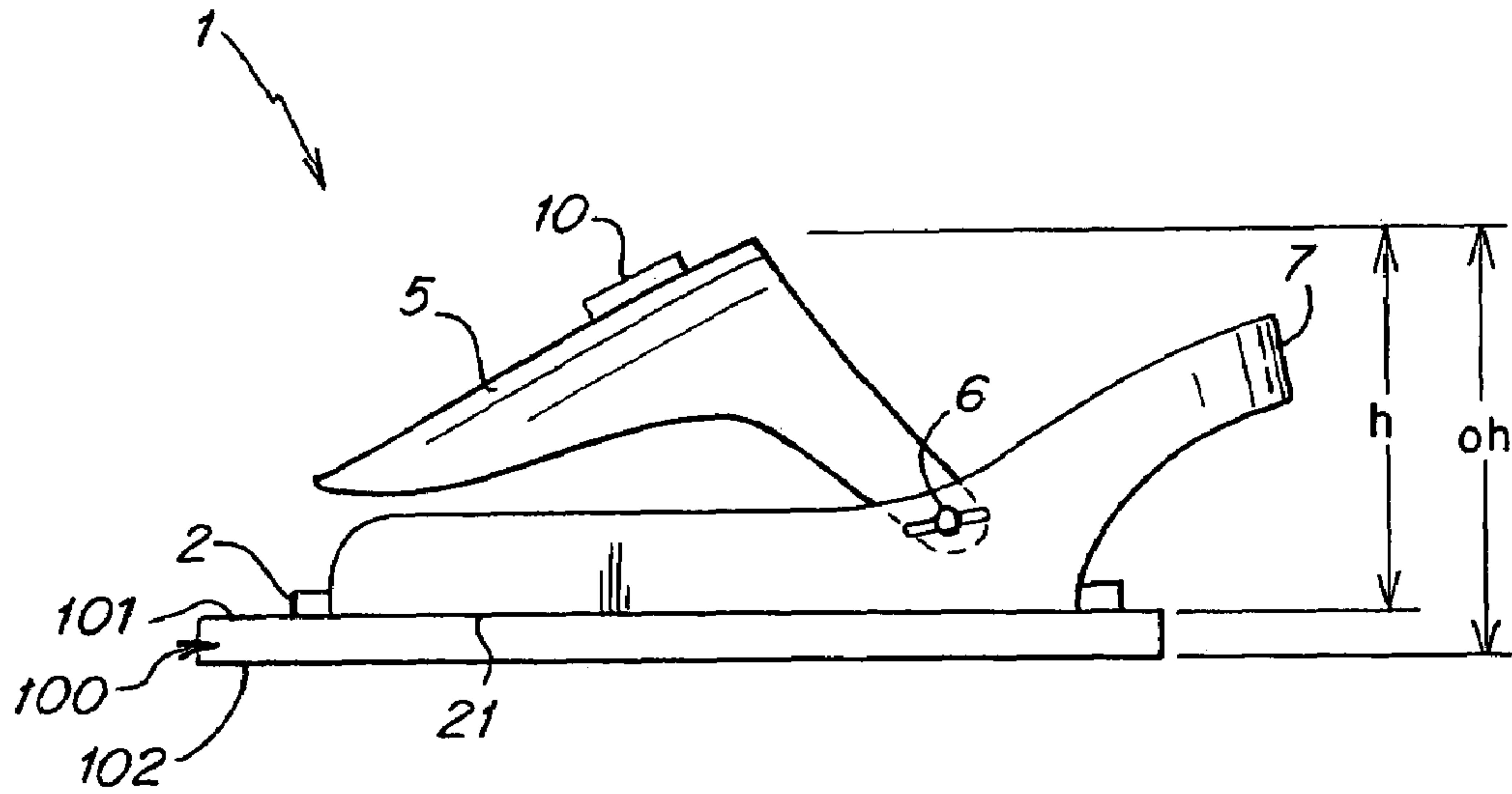
Fig. 17 PRIOR ART
