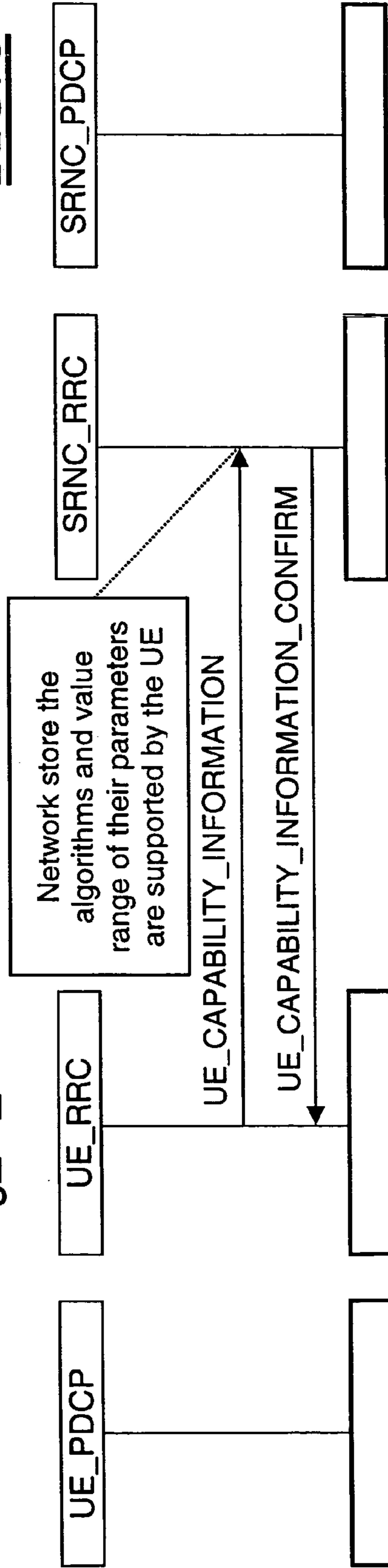
MSC Initialization
