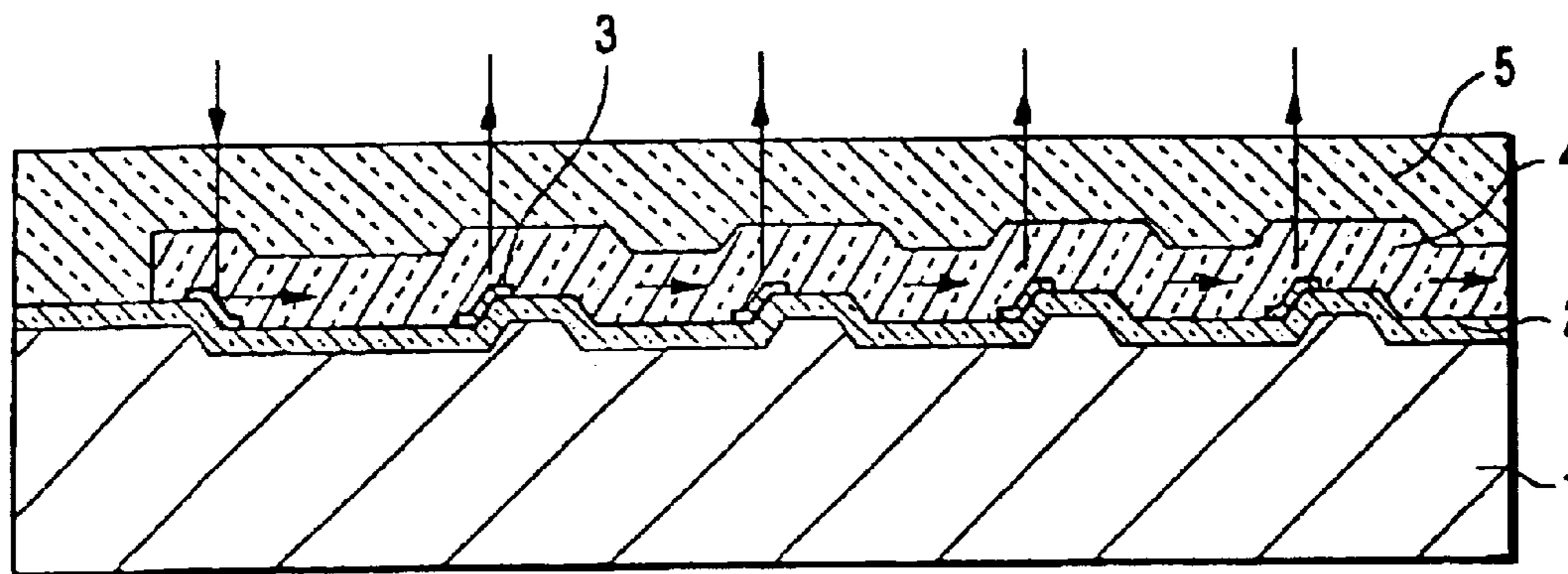
FIG. 2 PRIOR ART
