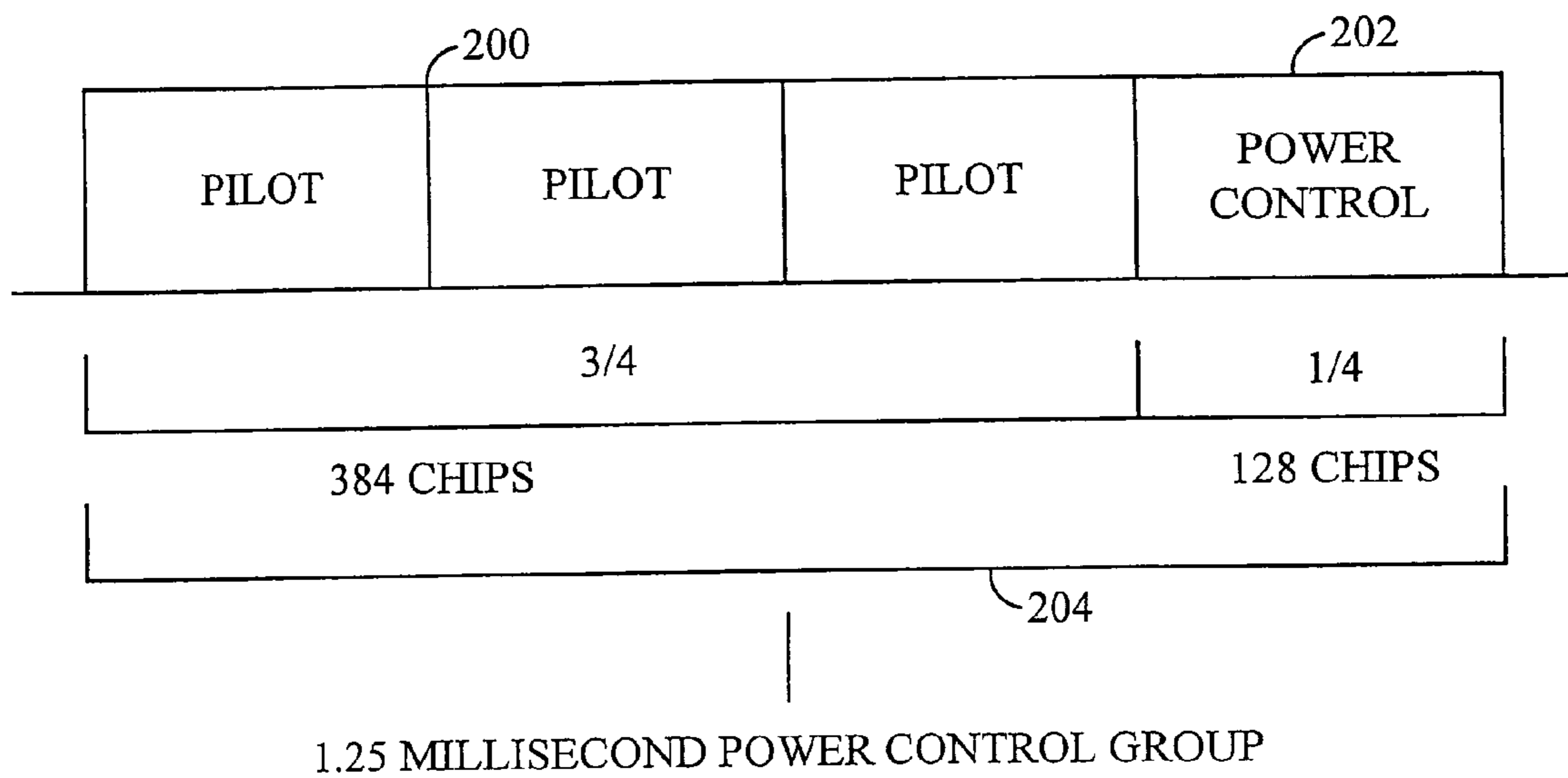
REVERSE LINK POWER CONTROL SUBCHANNEL STRUCTURE
