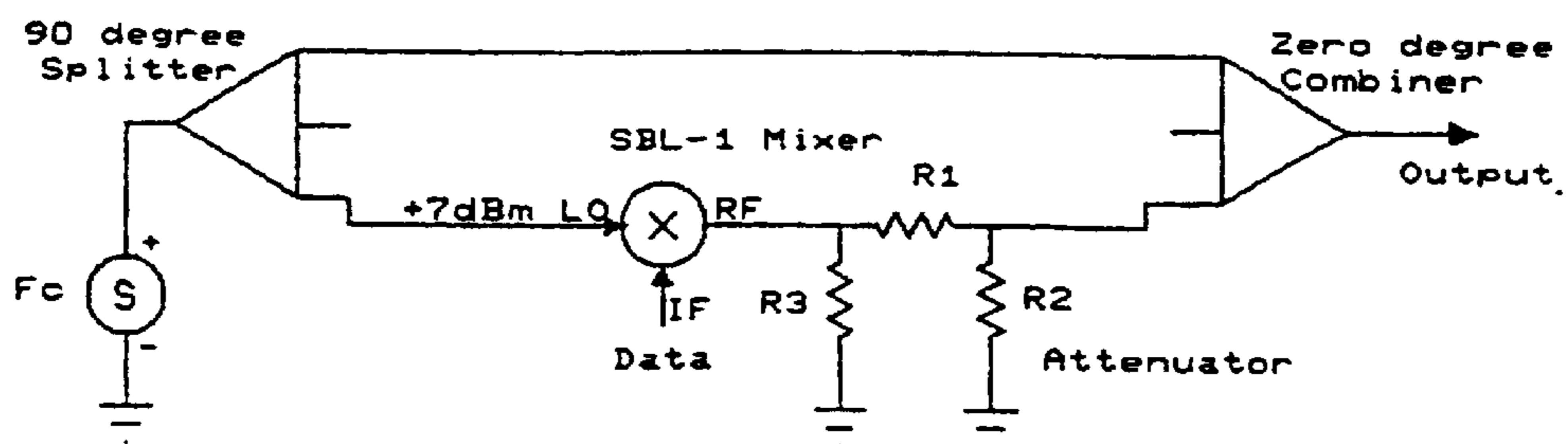
Figure 7 : Example Circuit for Modulating
