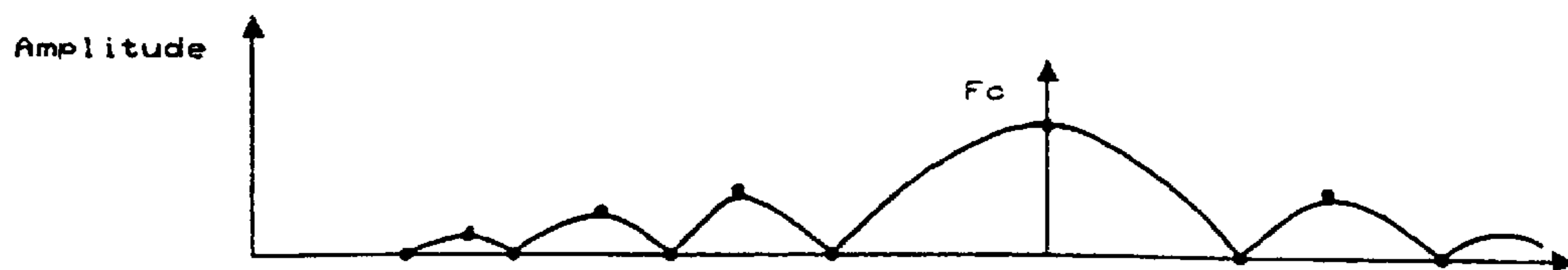
Figure 3(c) : Excitation Spectrum Modulated with PPM frequency
