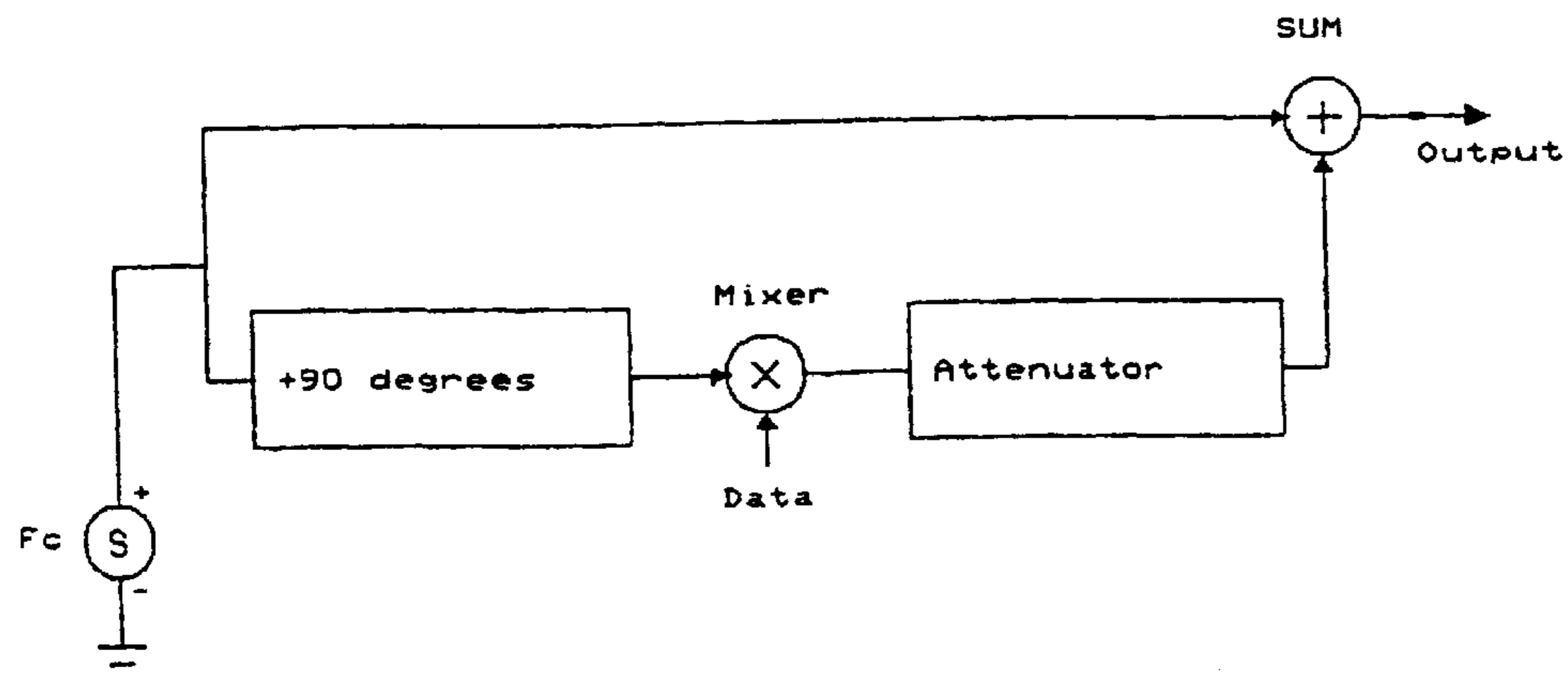
Figure 6(a) : Method of Modulating Excitation Signal
