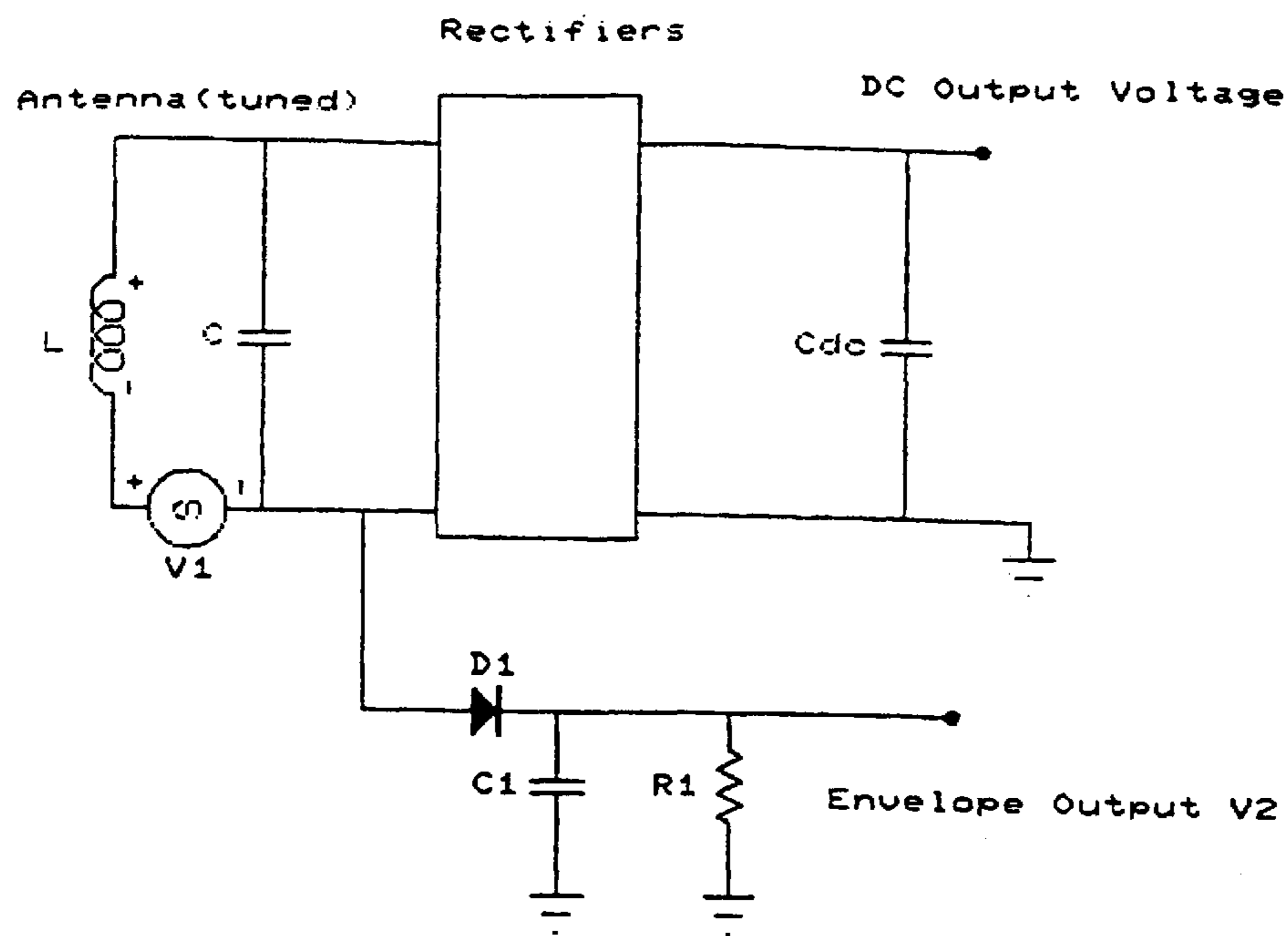
Figure 1 : Prior Art Transponder
