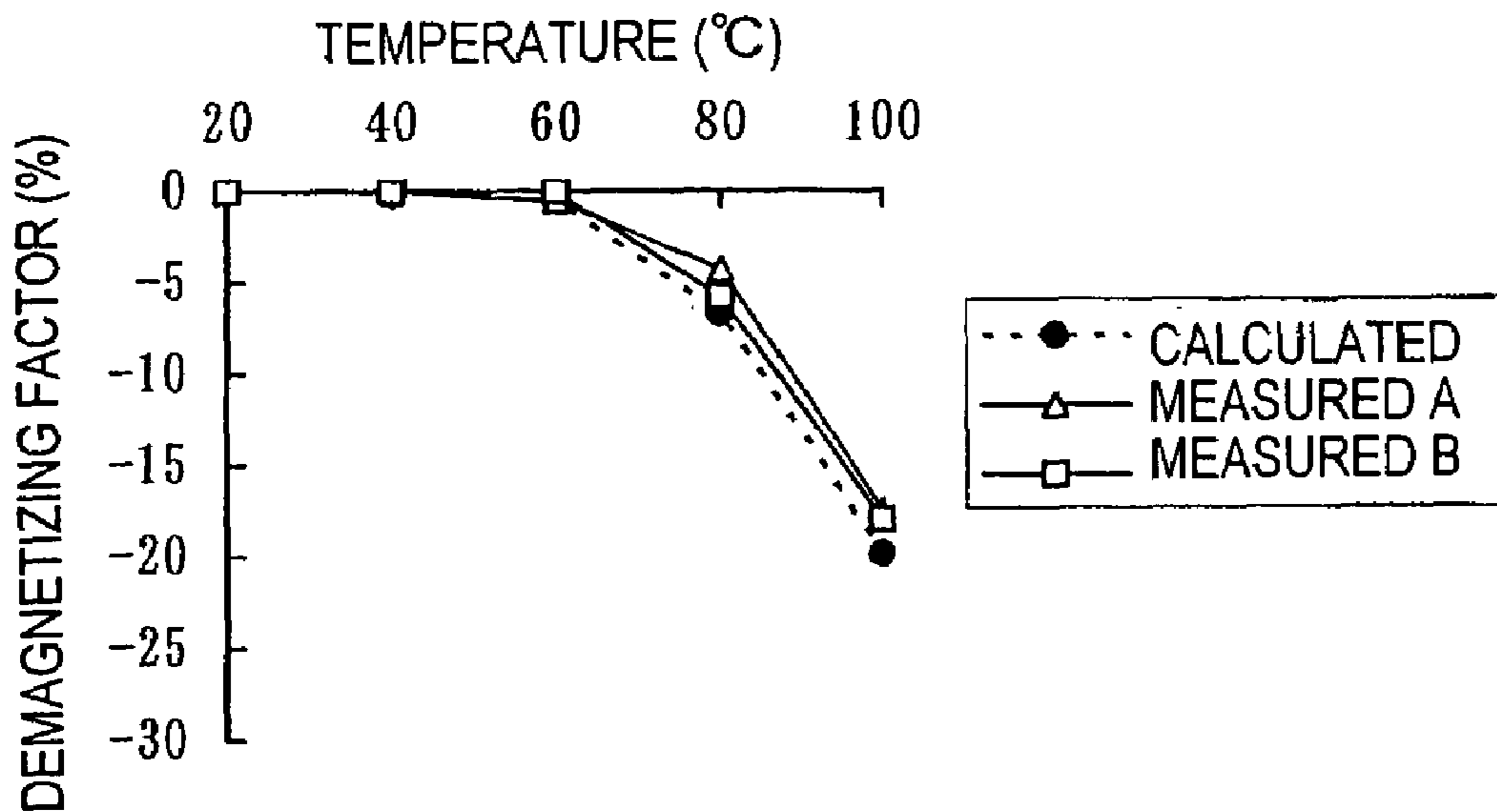
(b) COMPARE DEMAGNETIZING FACTORS
