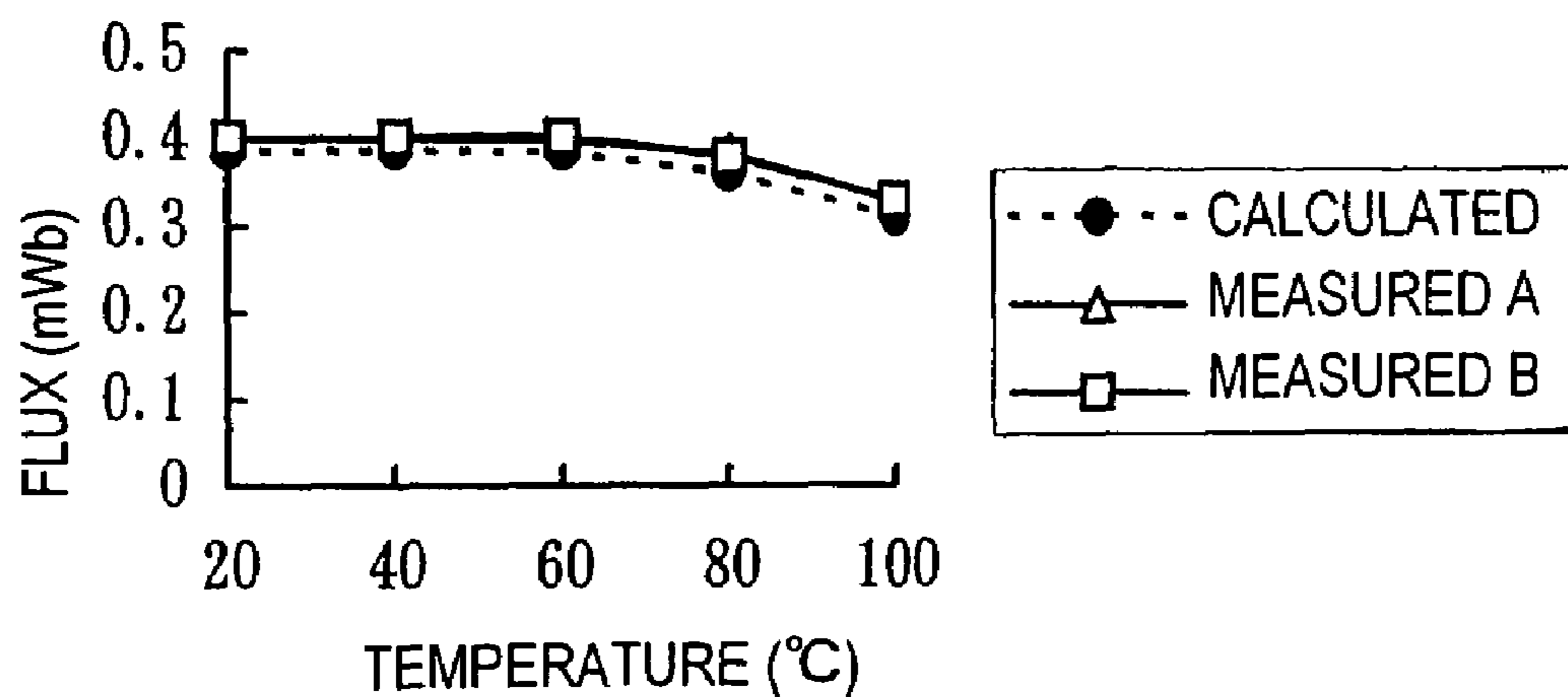
(a) COMPARE FLUXES
