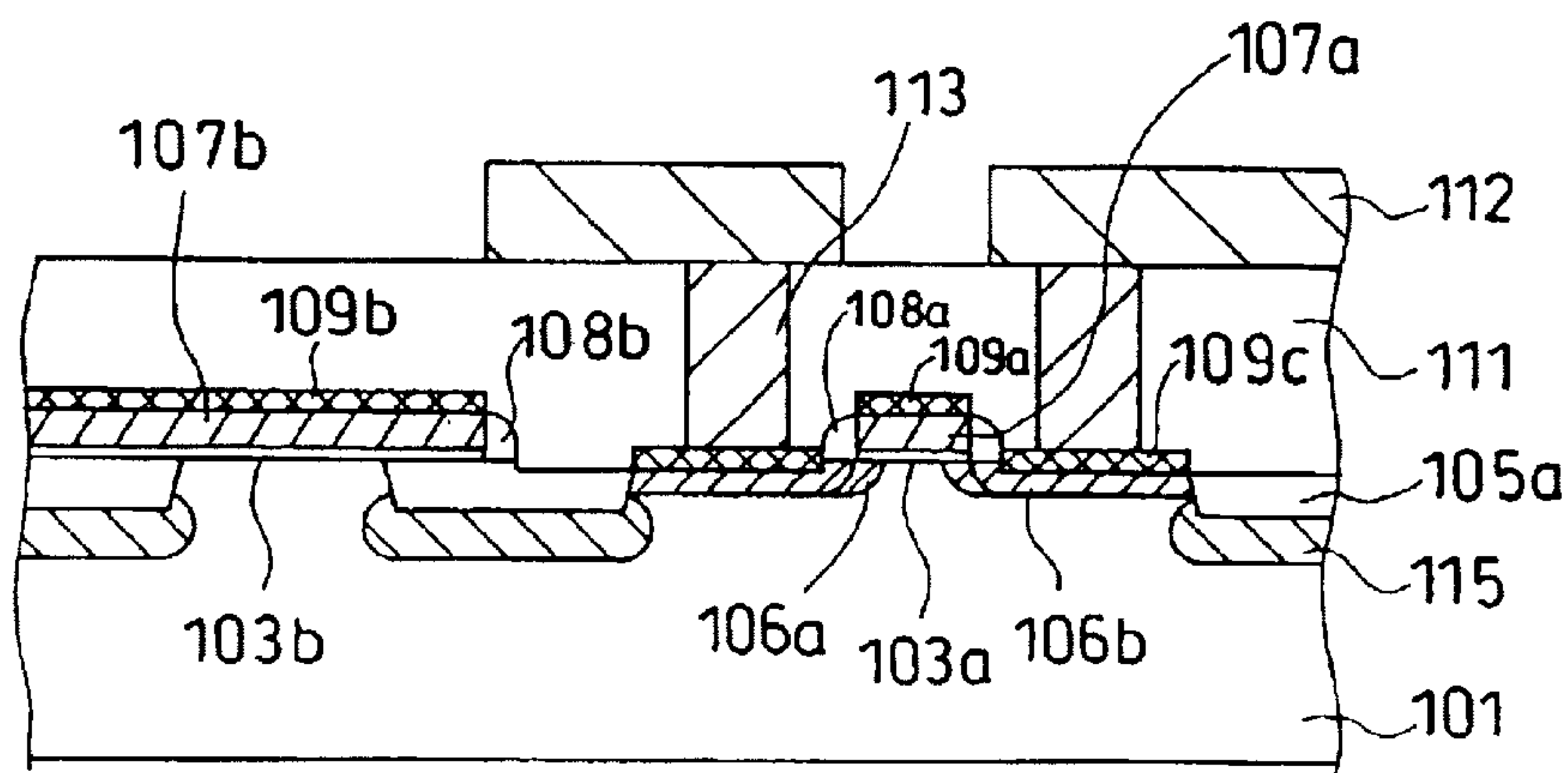
FIG. 19 PRIOR ART
