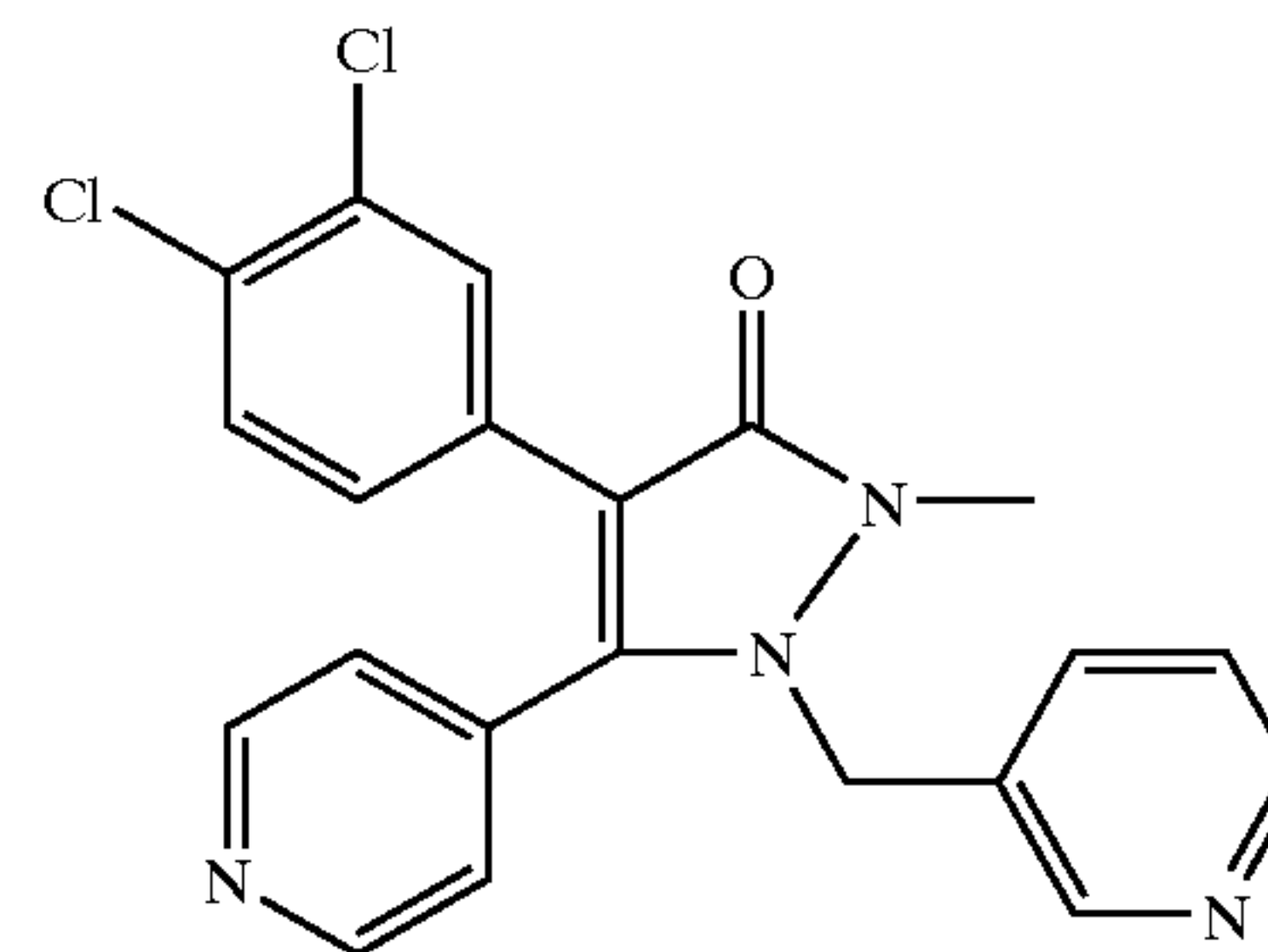
4-(3,4-Dichloro-phenyl)-2-methyl-5-pyridin-4-yl-1-pyridin-3-ylmethyl-1,2-dihydro-pyrazol-3-one
