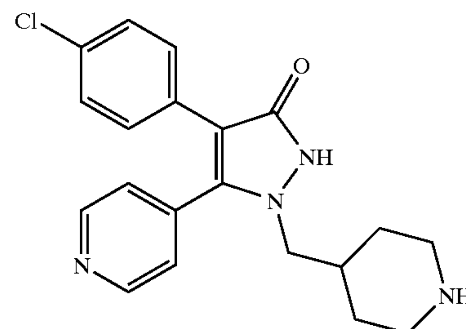
4-(4-Chloro-phenyl)-1-piperidin-4-ylmethyl-5-pyridin-4-yl-1,2-dihydro-pyrazol-3-one
