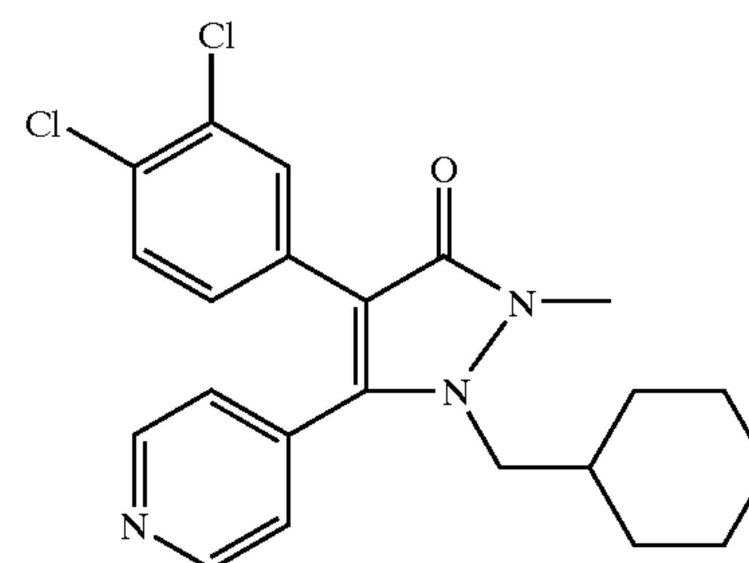
1-Cyclohexylmethyl-4-(3,4-dichloro-phenyl)-2-methyl-5-pyridin-4-yl-1,2-dihydro-pyrazol-3-one
