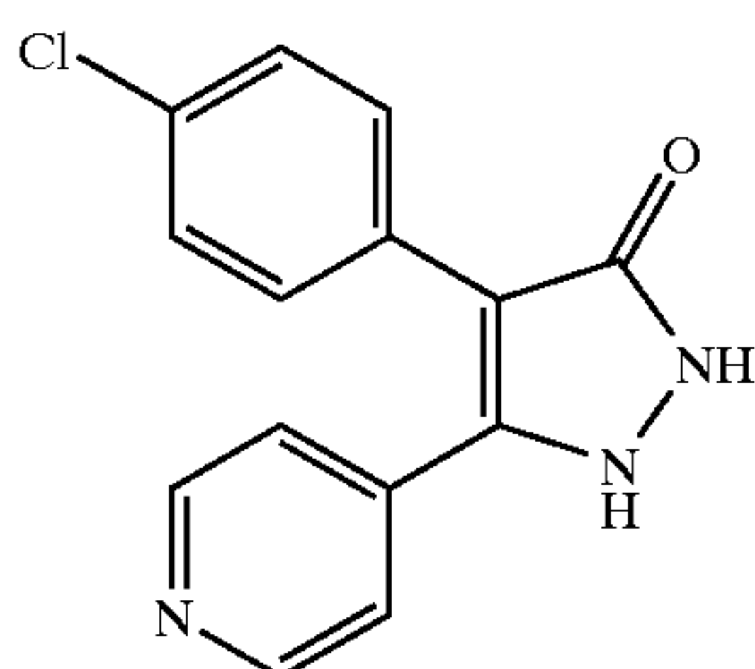
4-(4-Chloro-phenyl)-5-pyridin-4-yl-1,2-dihydro-pyrazol-3-one
