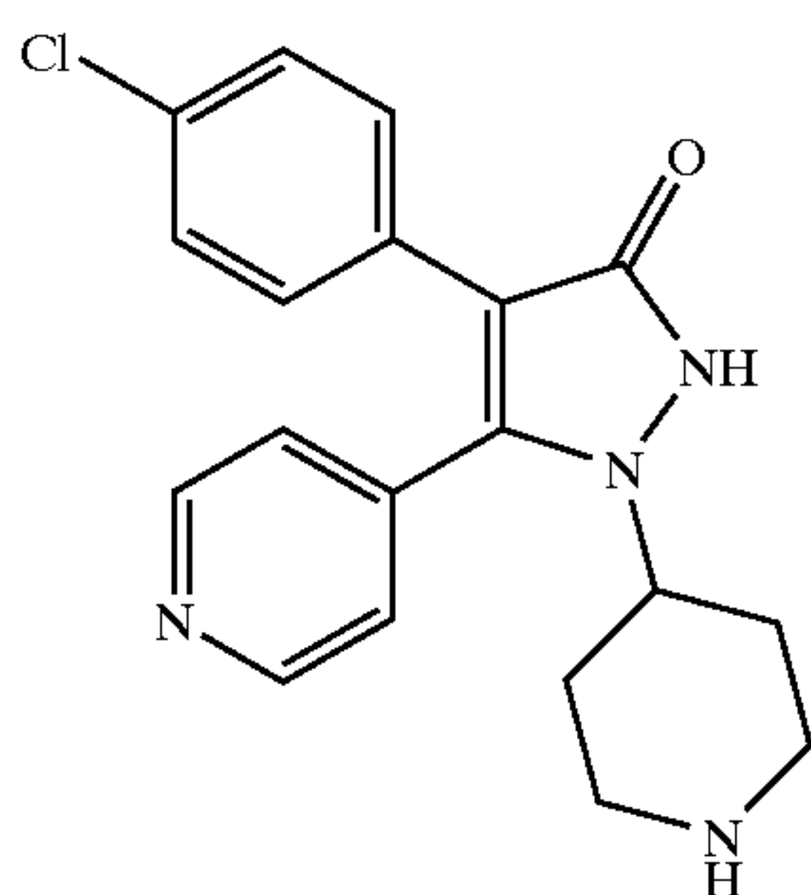
4-(4-Chloro-phenyl)-1-piperidin-4-yl-5-pyridin-4-yl-1,2-dihydro-pyrazol-3-one
