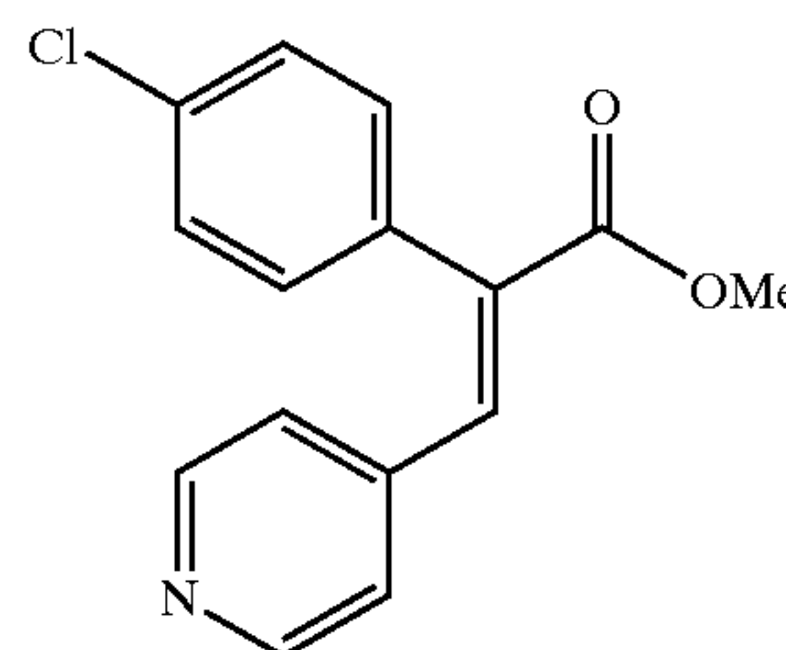
2-(4-Chloro-phenyl)-3-pyridin-4-yl-acrylic acid methyl ester
