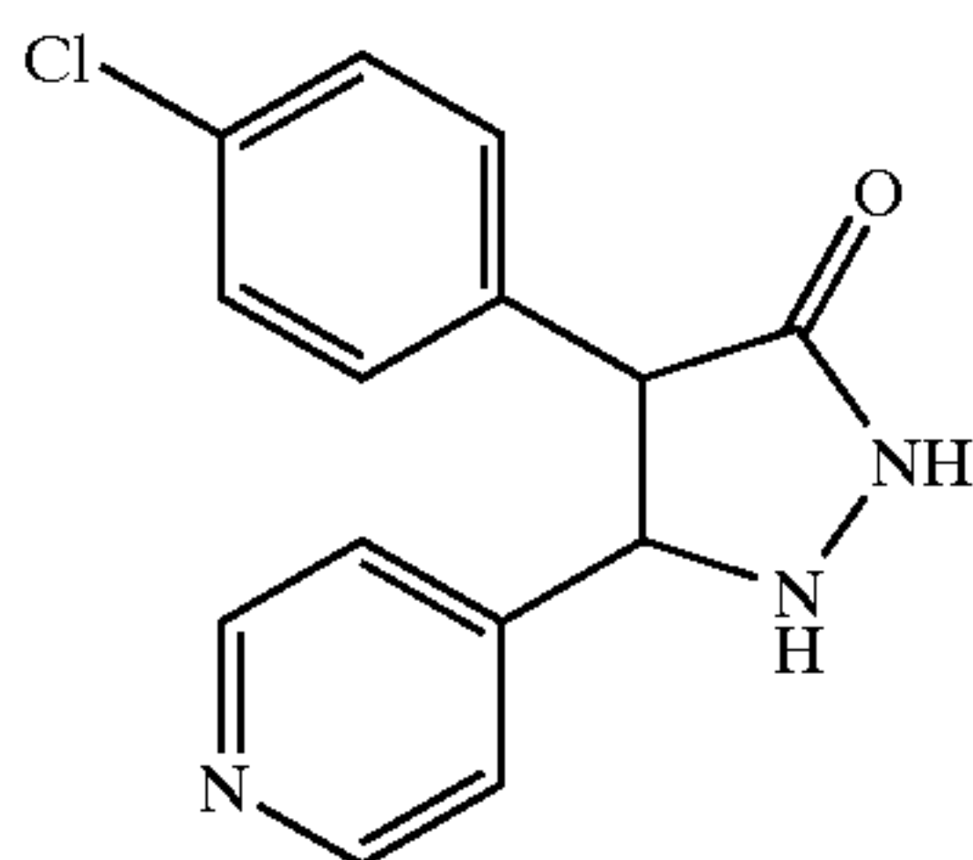
4-(4-Chloro-phenyl)-5-pyridin-4-yl-pyrazolidin-3-one
