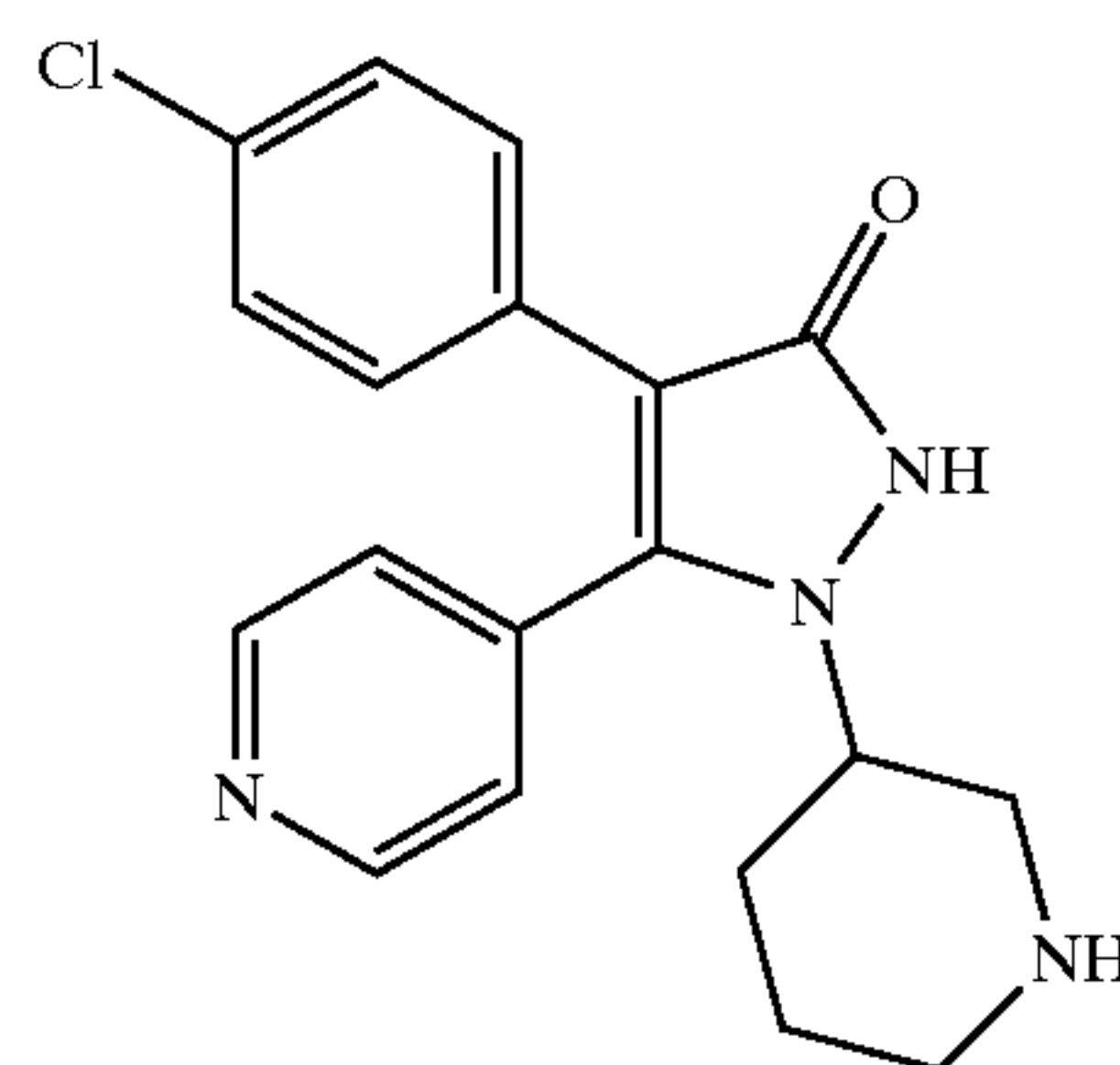
4-(4-Chloro-phenyl)-1-piperidin-3-yl-5-pyridin-4-yl-1,2-dihydro-pyrazol-3-one
