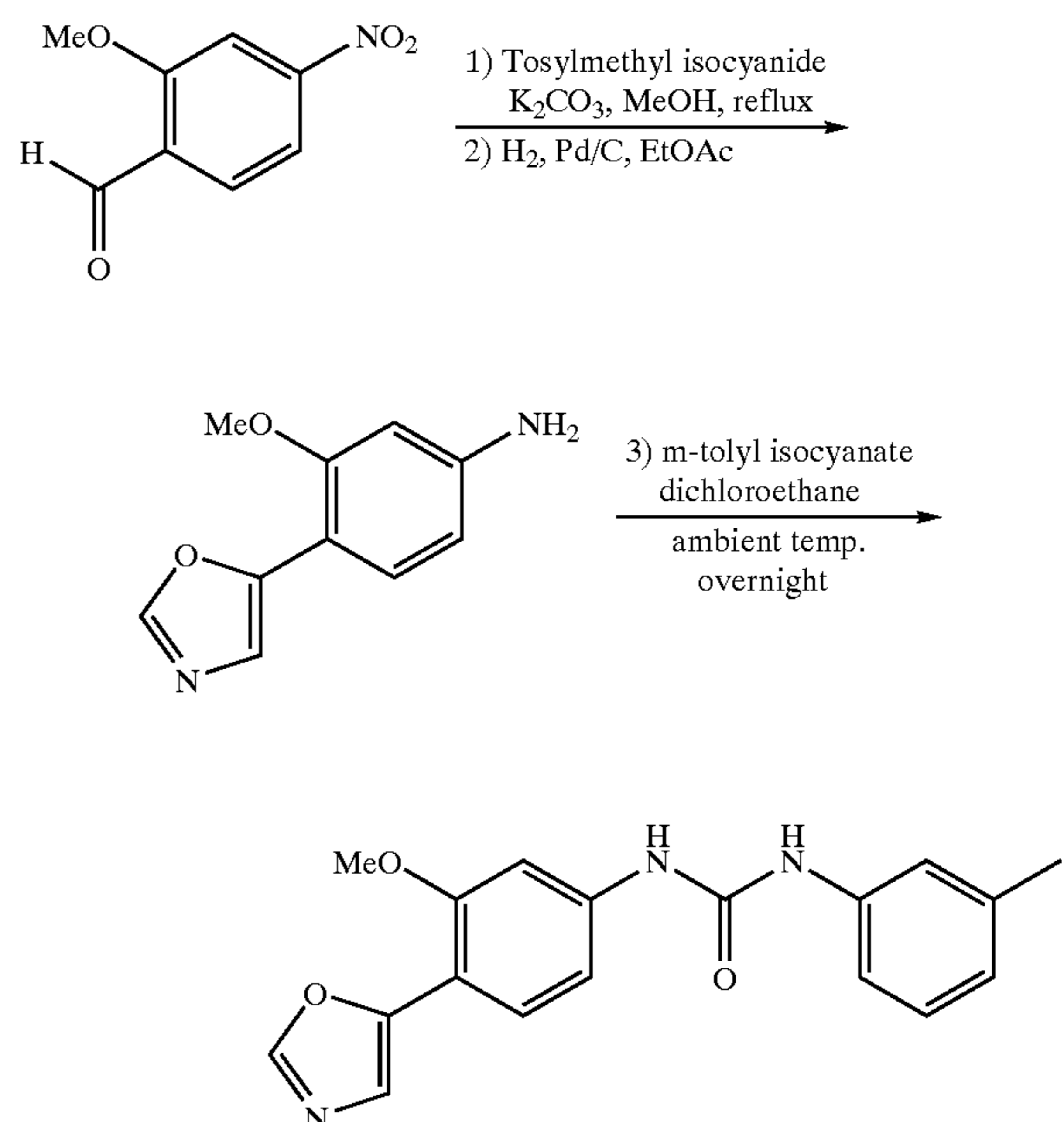
General Synthetic Scheme 2:
