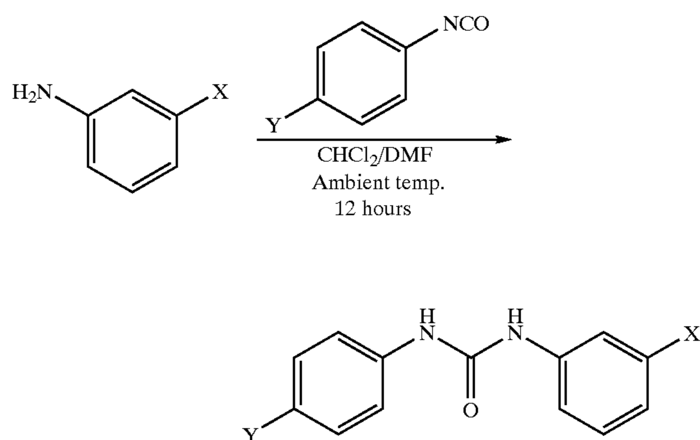
General Synthetic Scheme 1:
