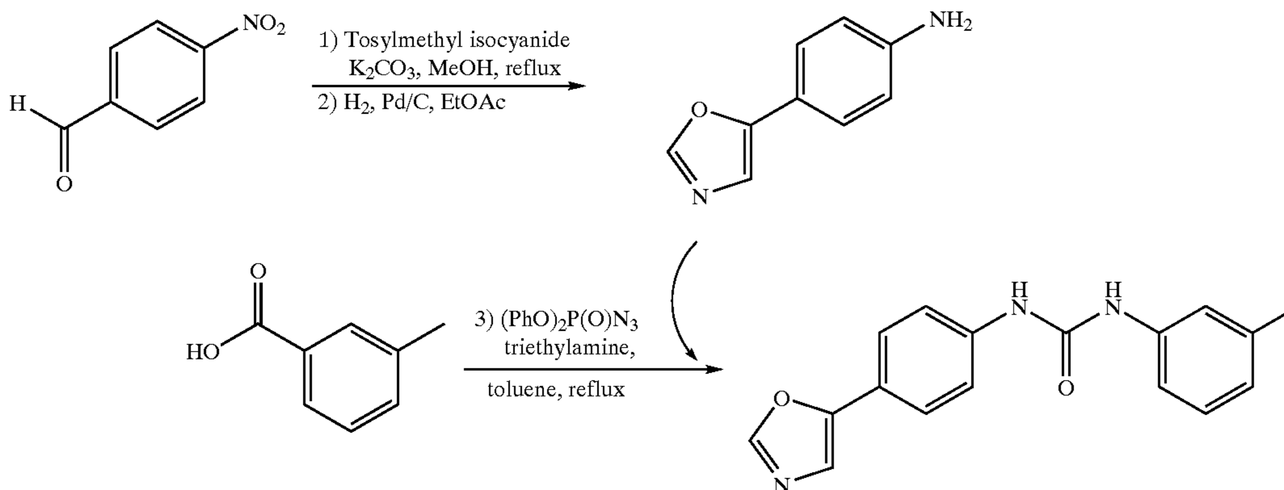
General Synthetic Scheme 3:
