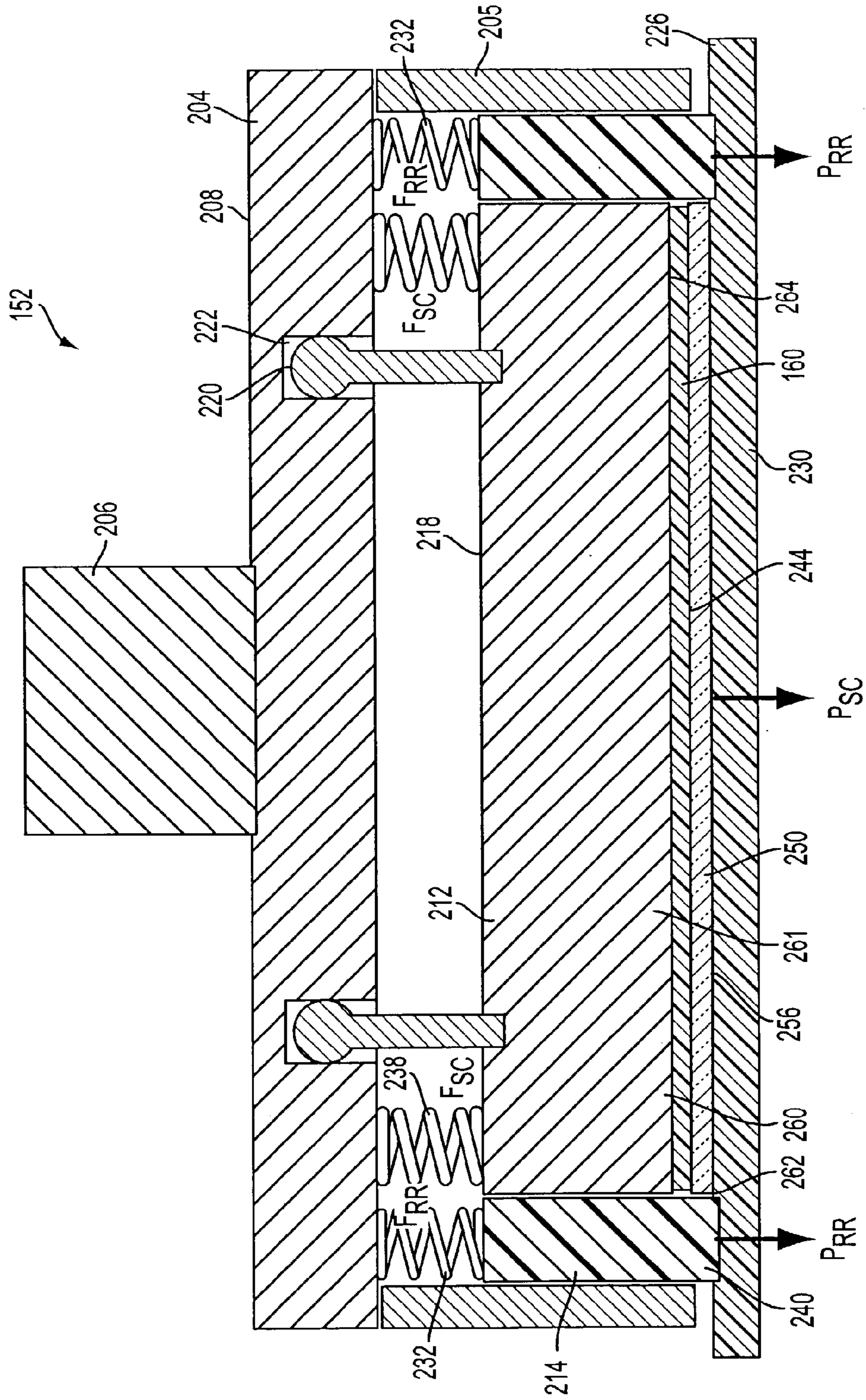
FIG. 2 (PRIOR ART)
