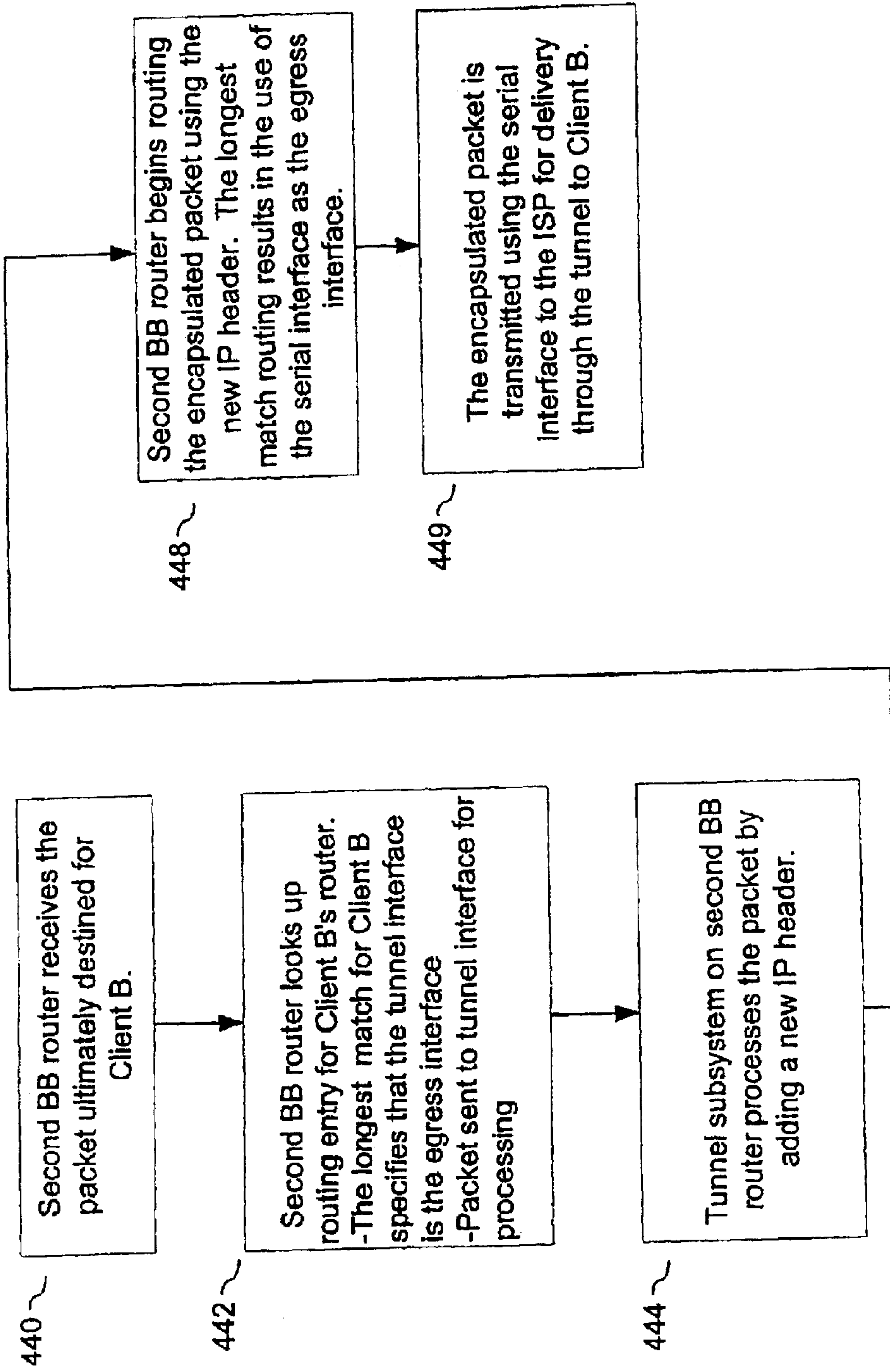
Fig. 4(d) Routing on Second Client Router
