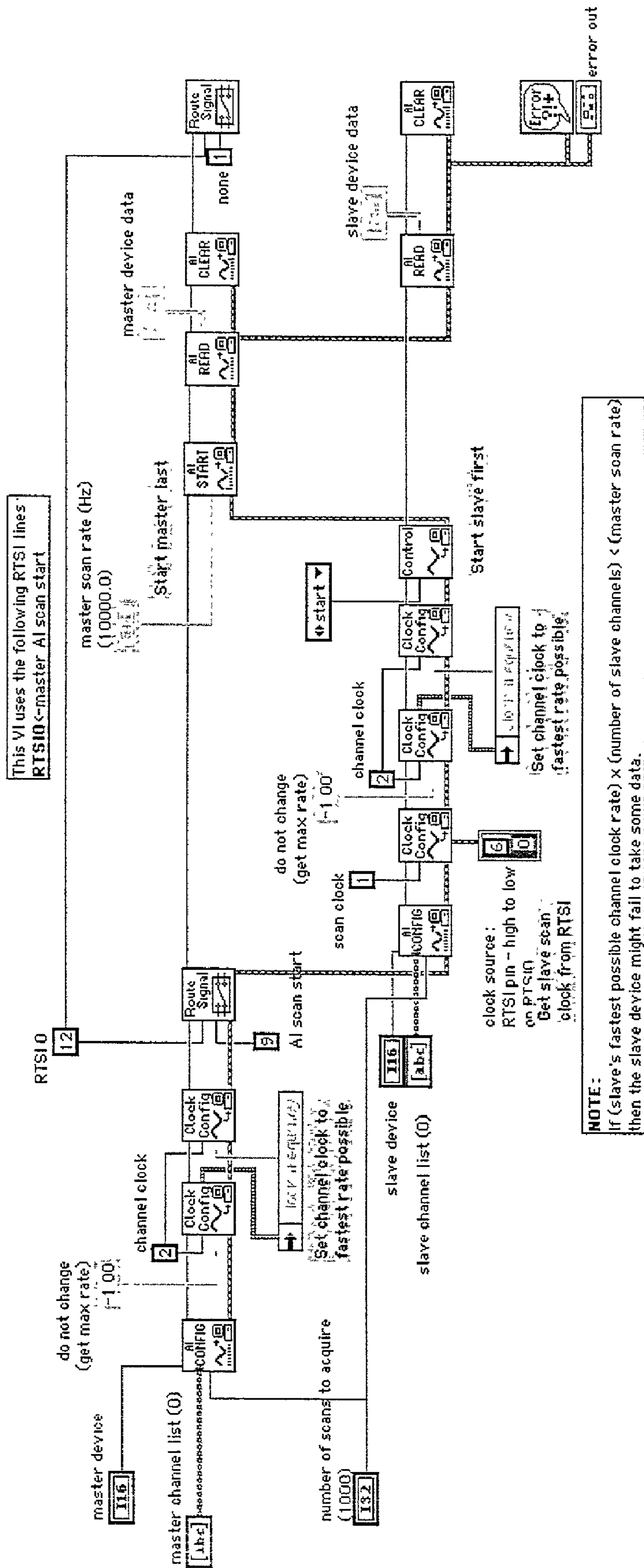
Sharing Scan Clock Across Two E-Series Devices (Prior Art)
