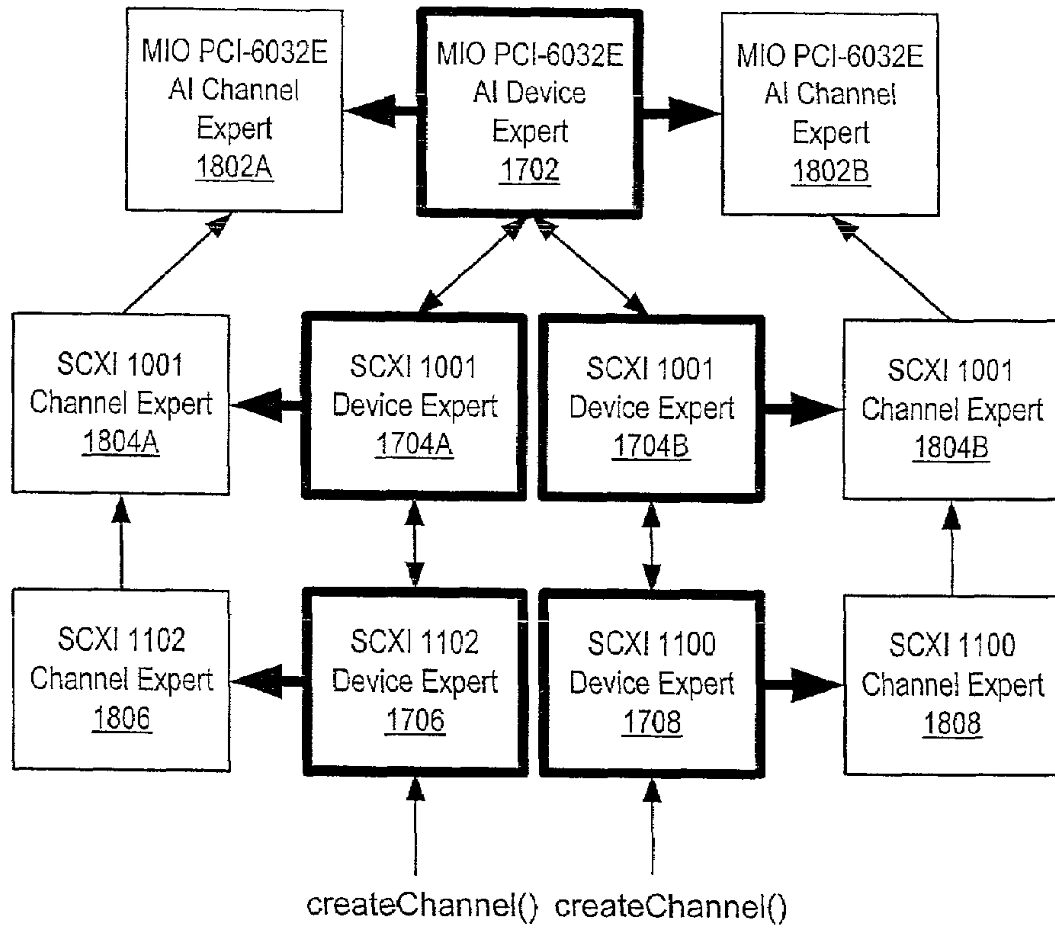
Create Channel Experts
