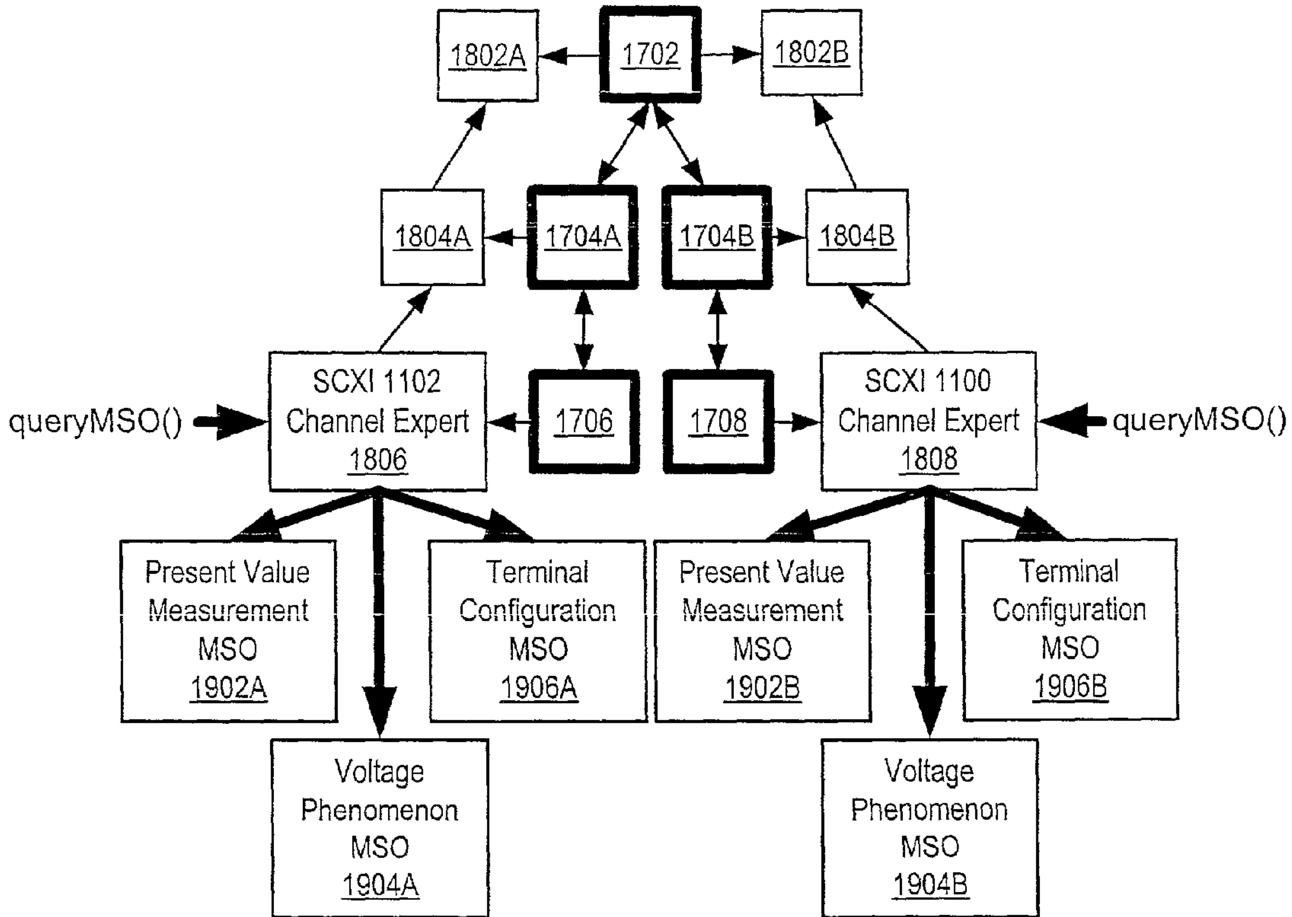
Deserialize Named Channel MSOs
