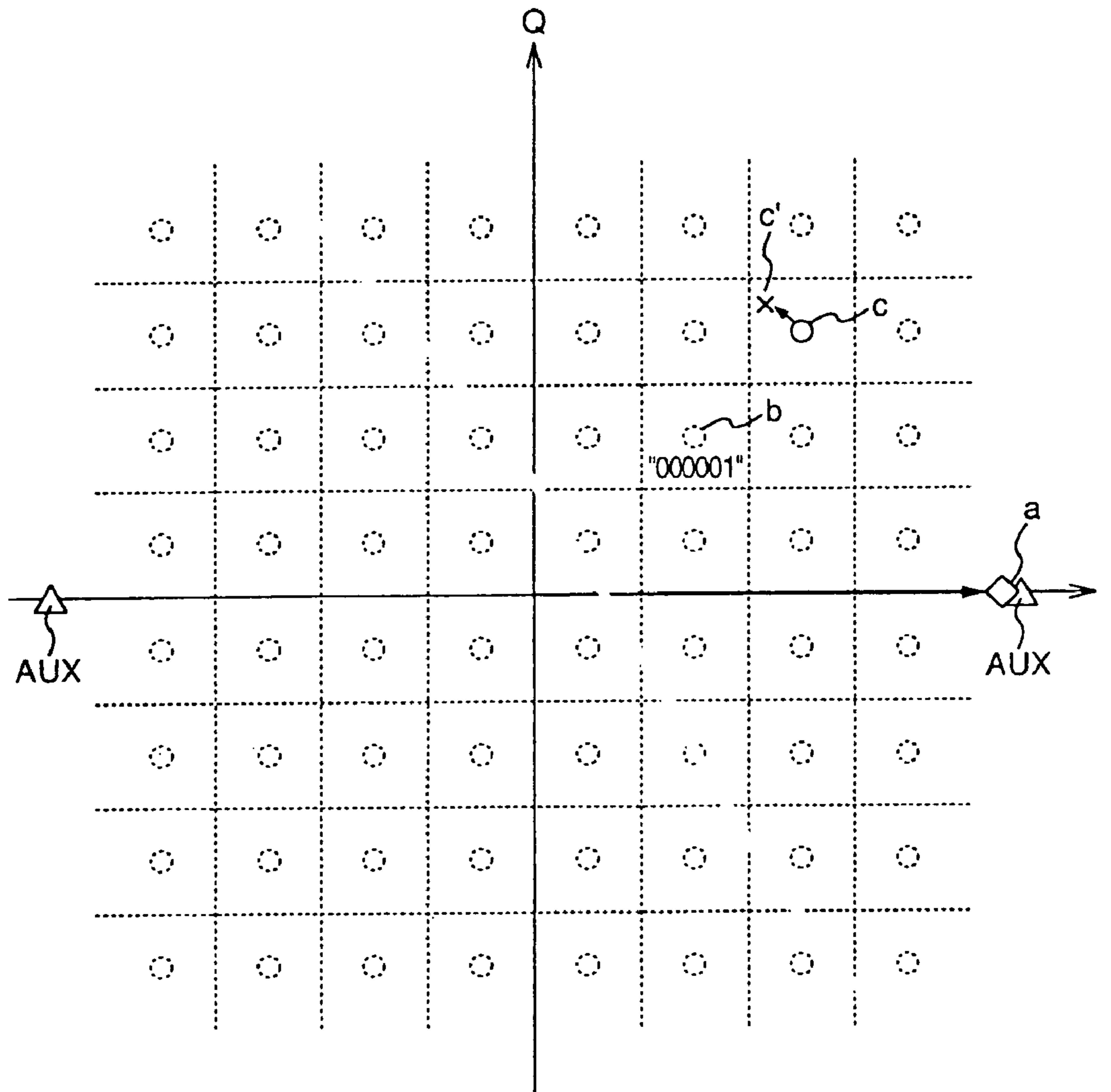
FIG.6 PRIOR ART
