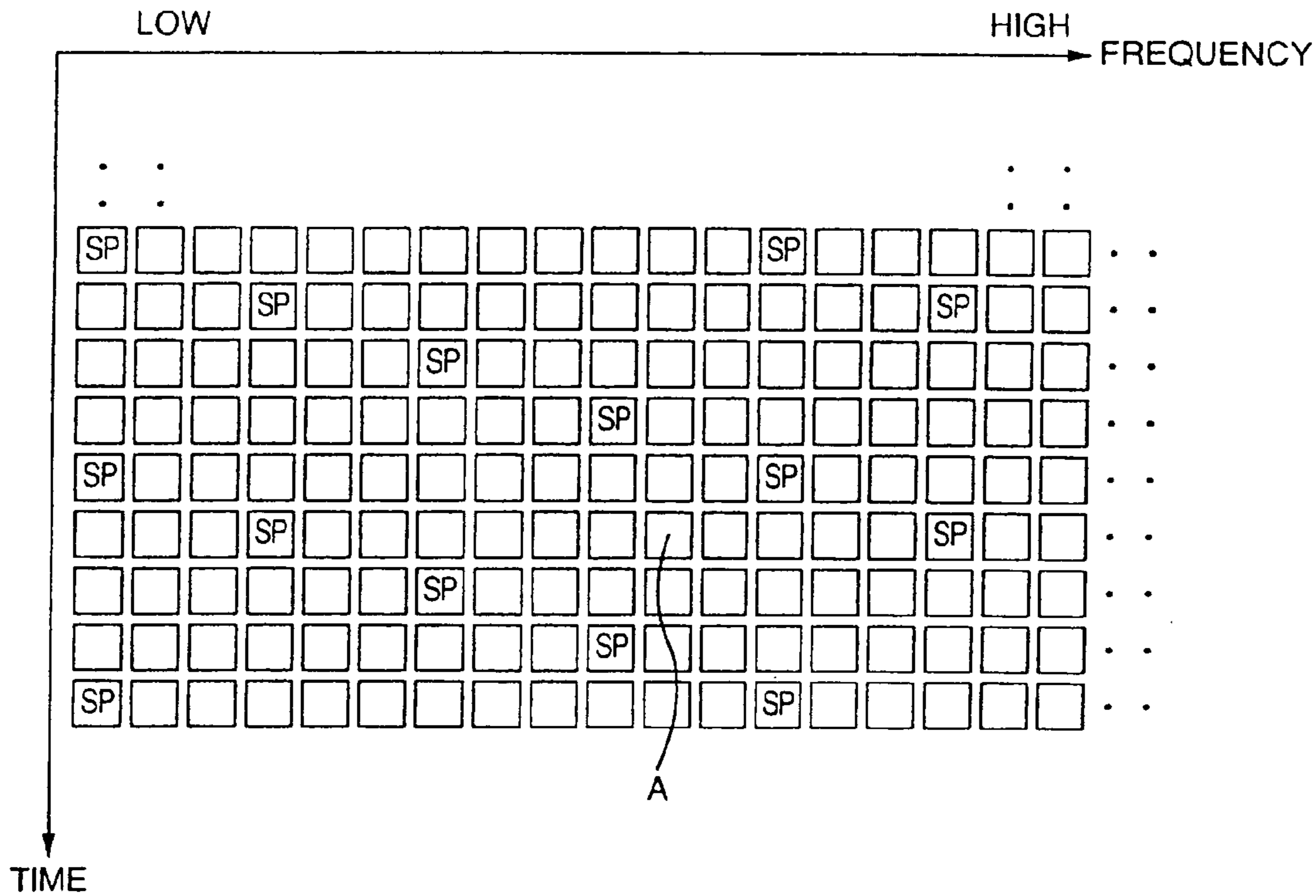
FIG.5 PRIOR ART
