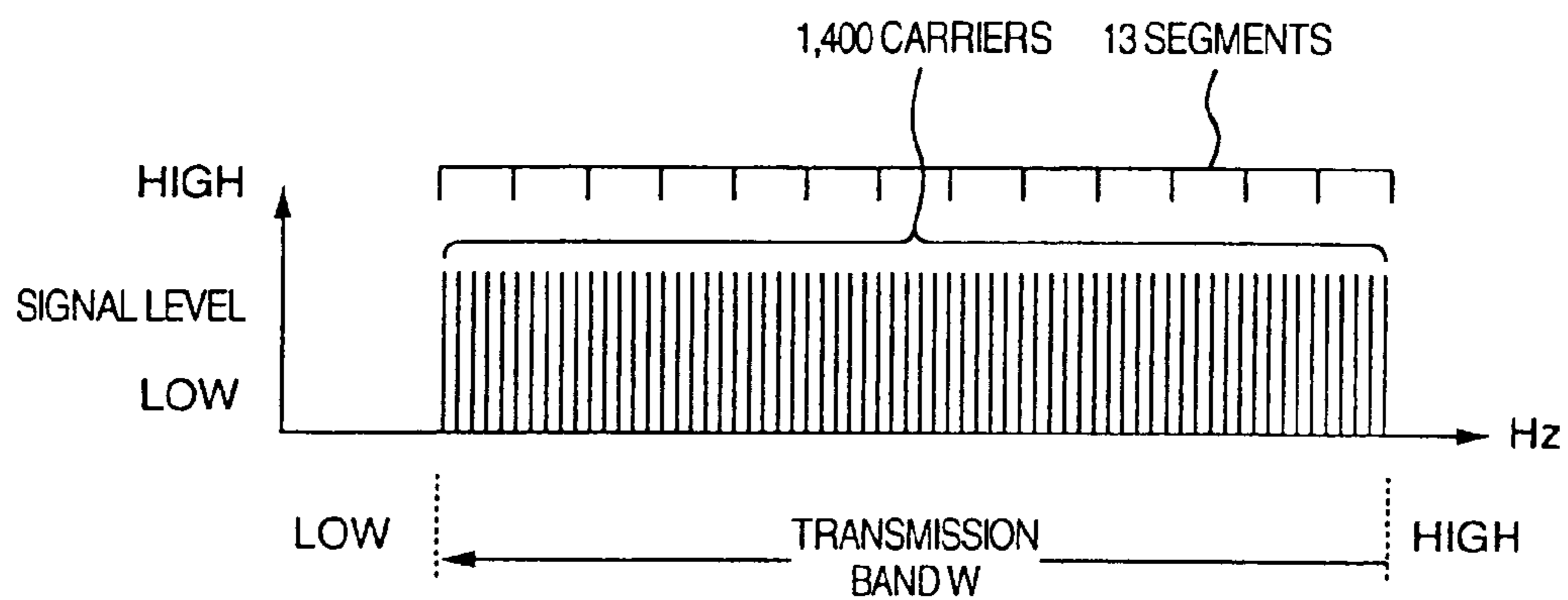
FIG.5 PRIOR ART
