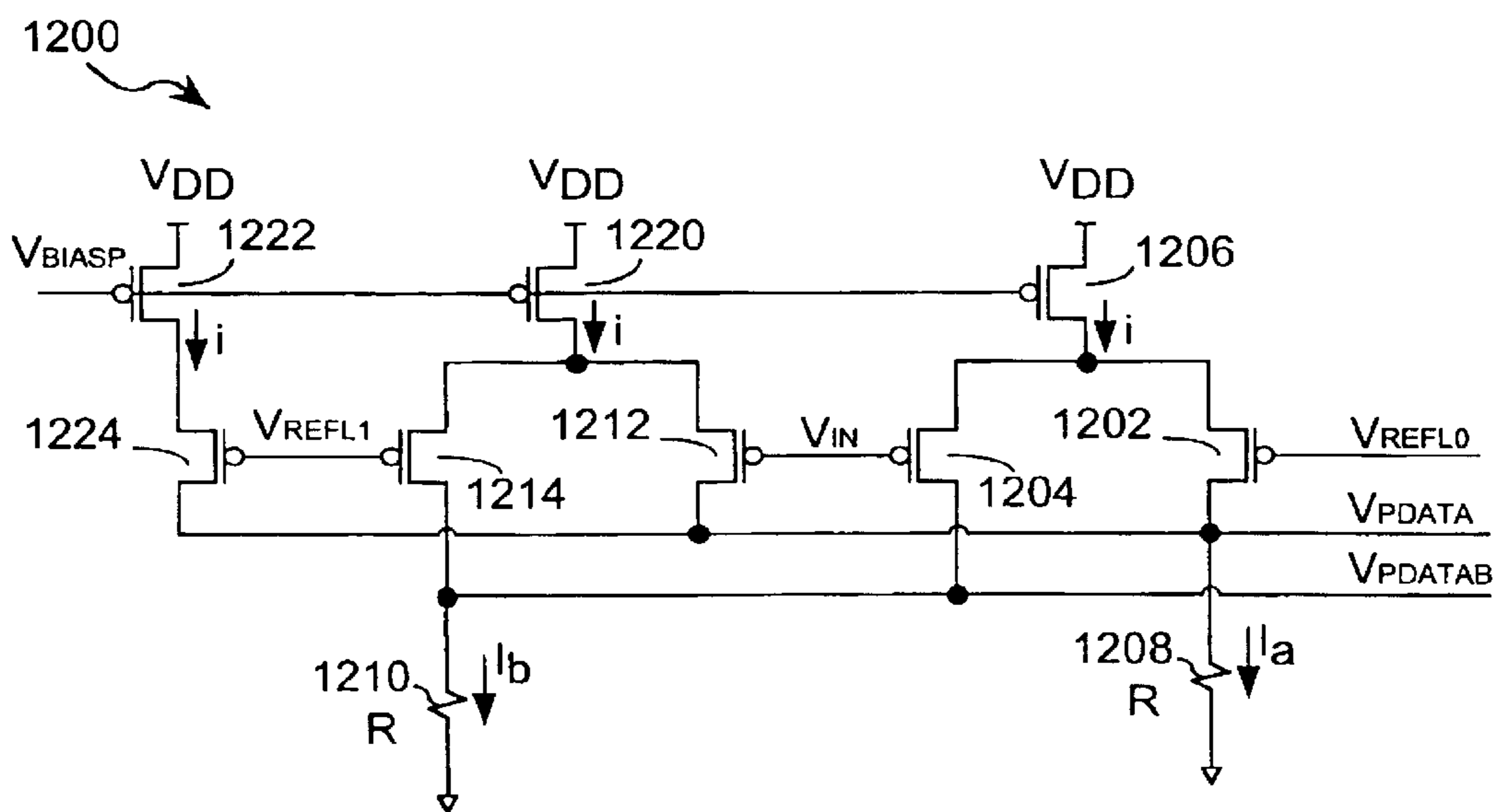
Multi-PAM Pre-Amplifier FIG. 45B
