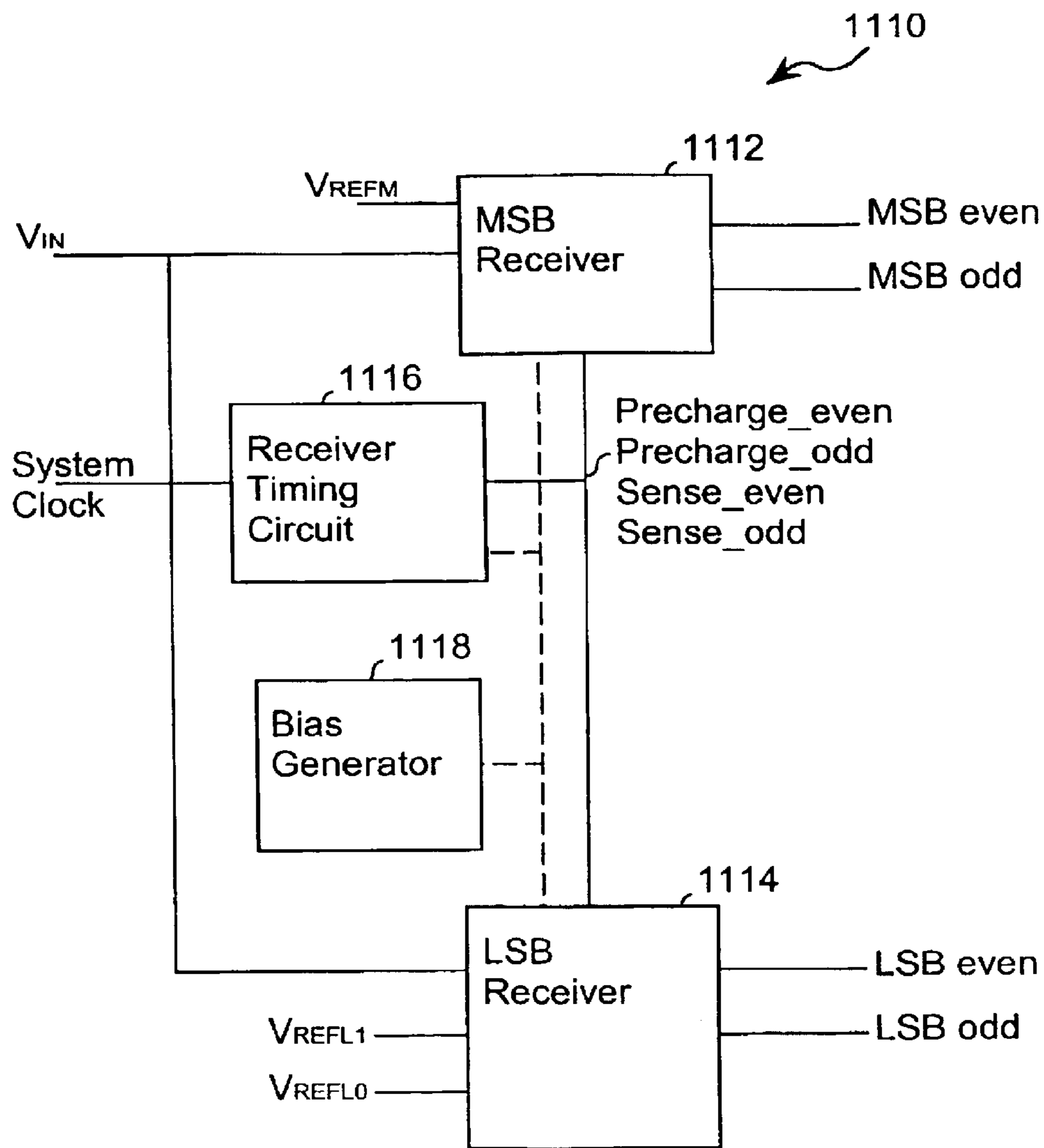
Multi-PAM Receiver FIG. 40
