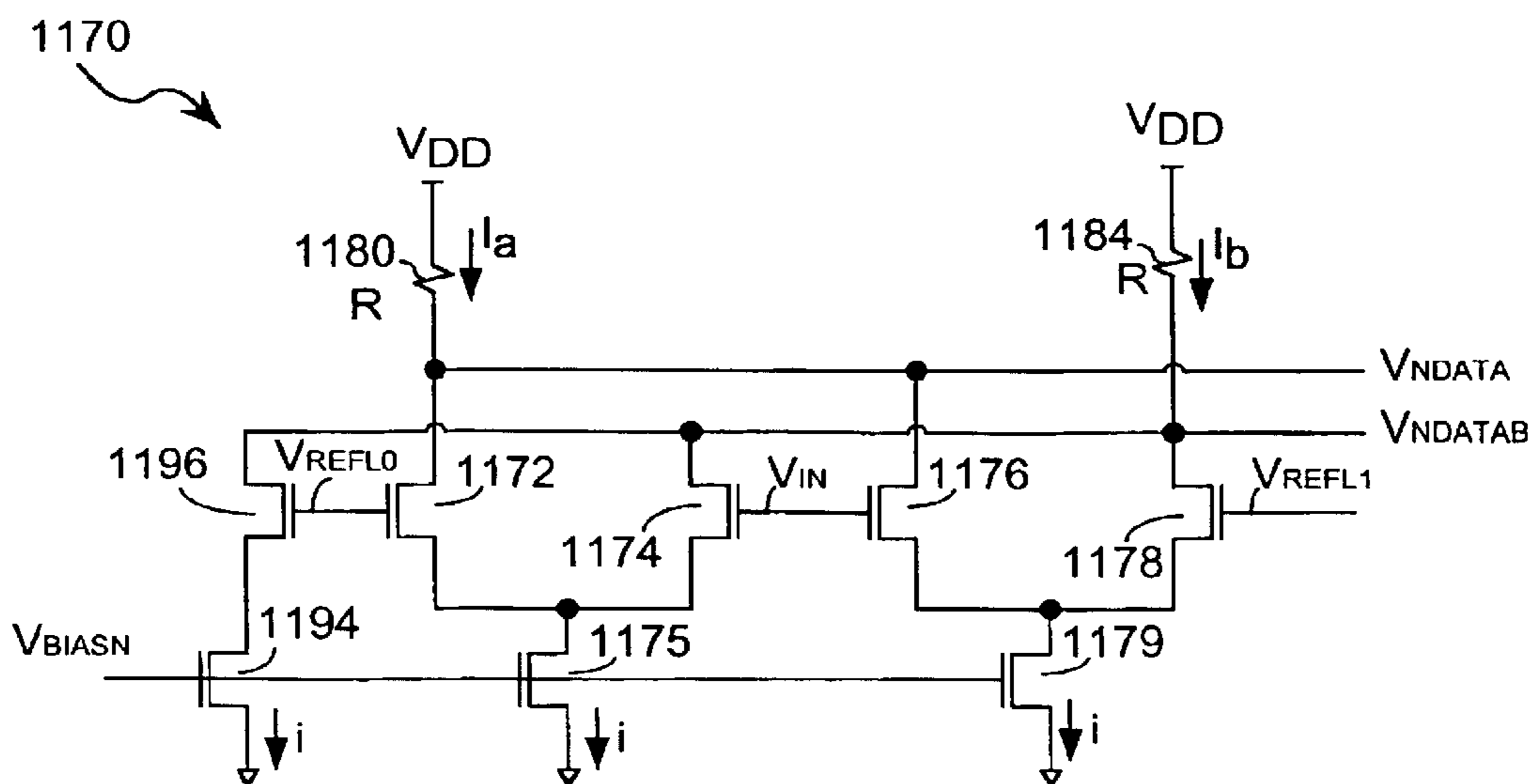
Multi-PAM Pre-Amplifier FIG. 45A
