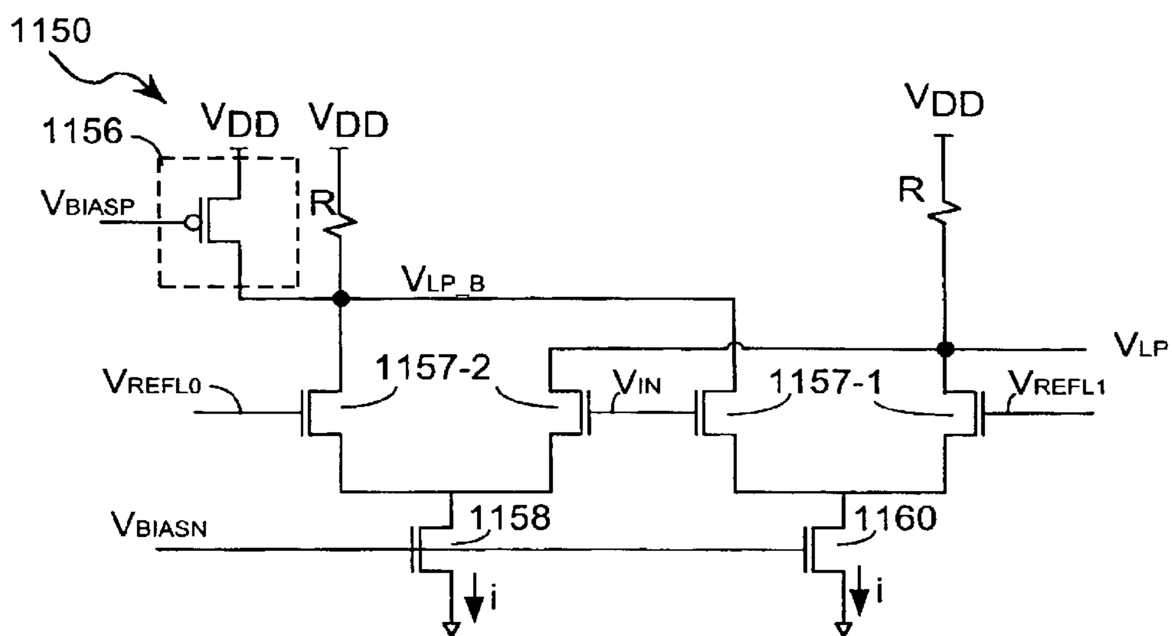
Multi-PAM Pre-Amplifier
