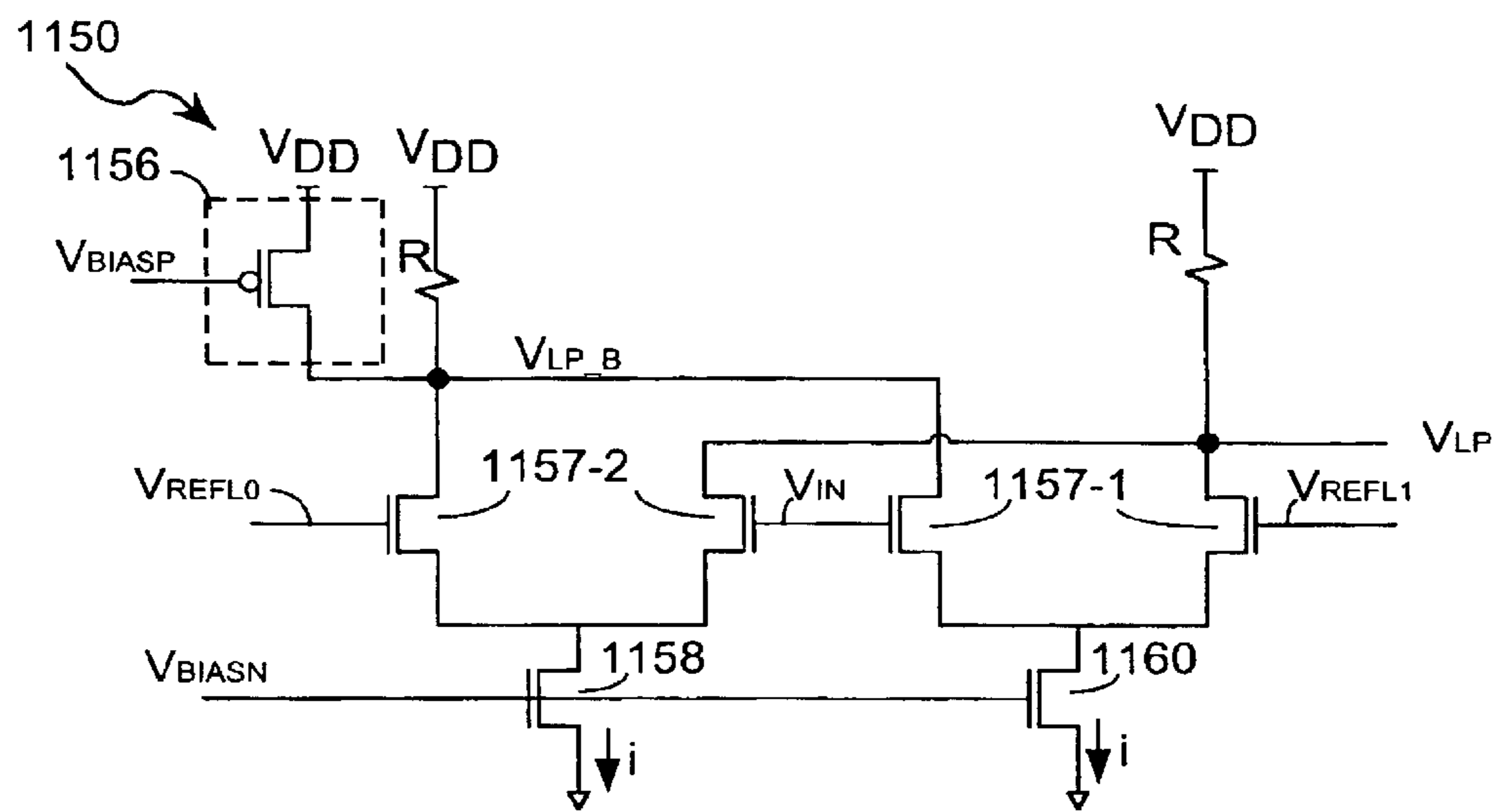
Multi-PAM Pre-Amplifier
