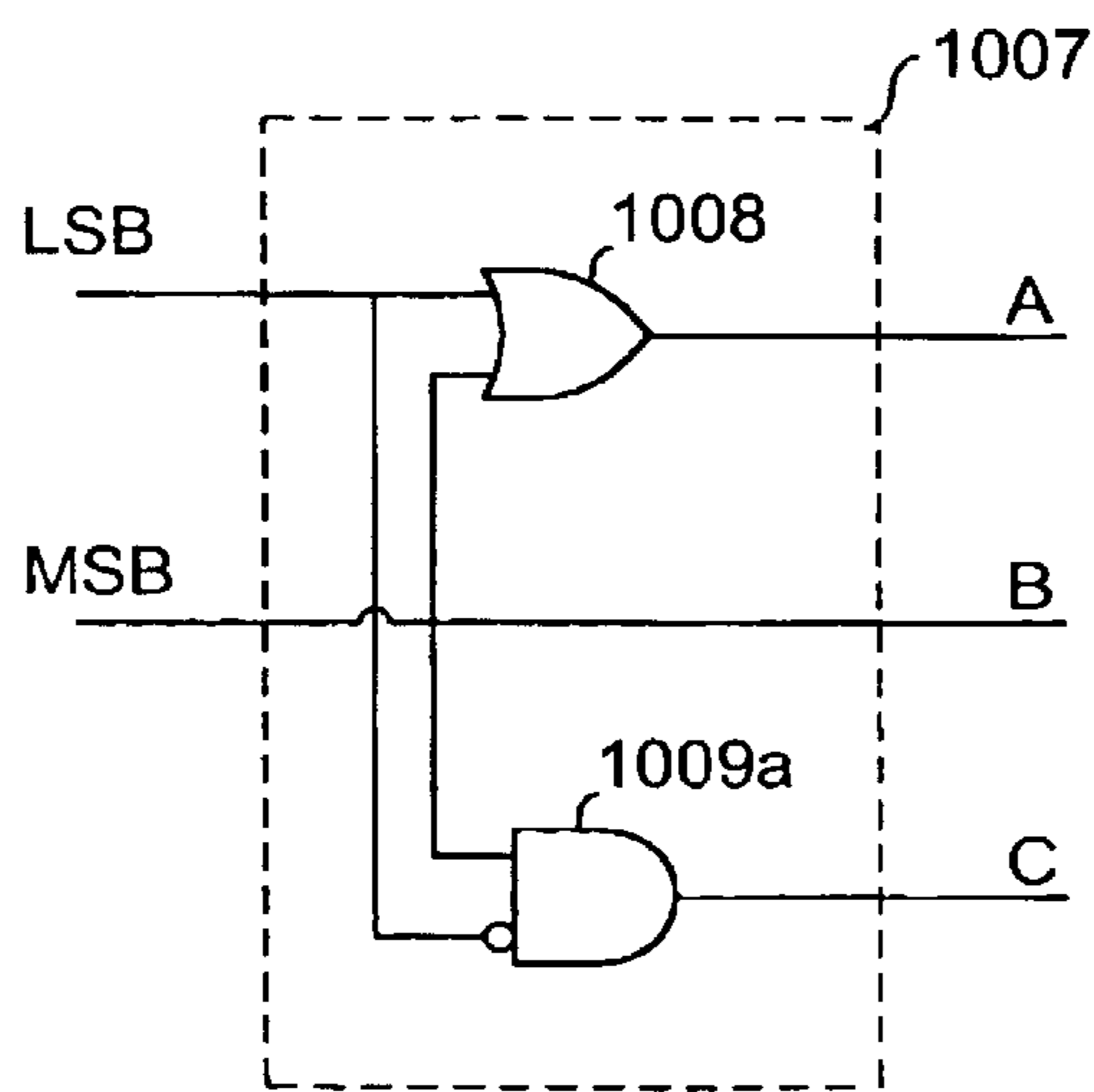
Gray Code Generator
