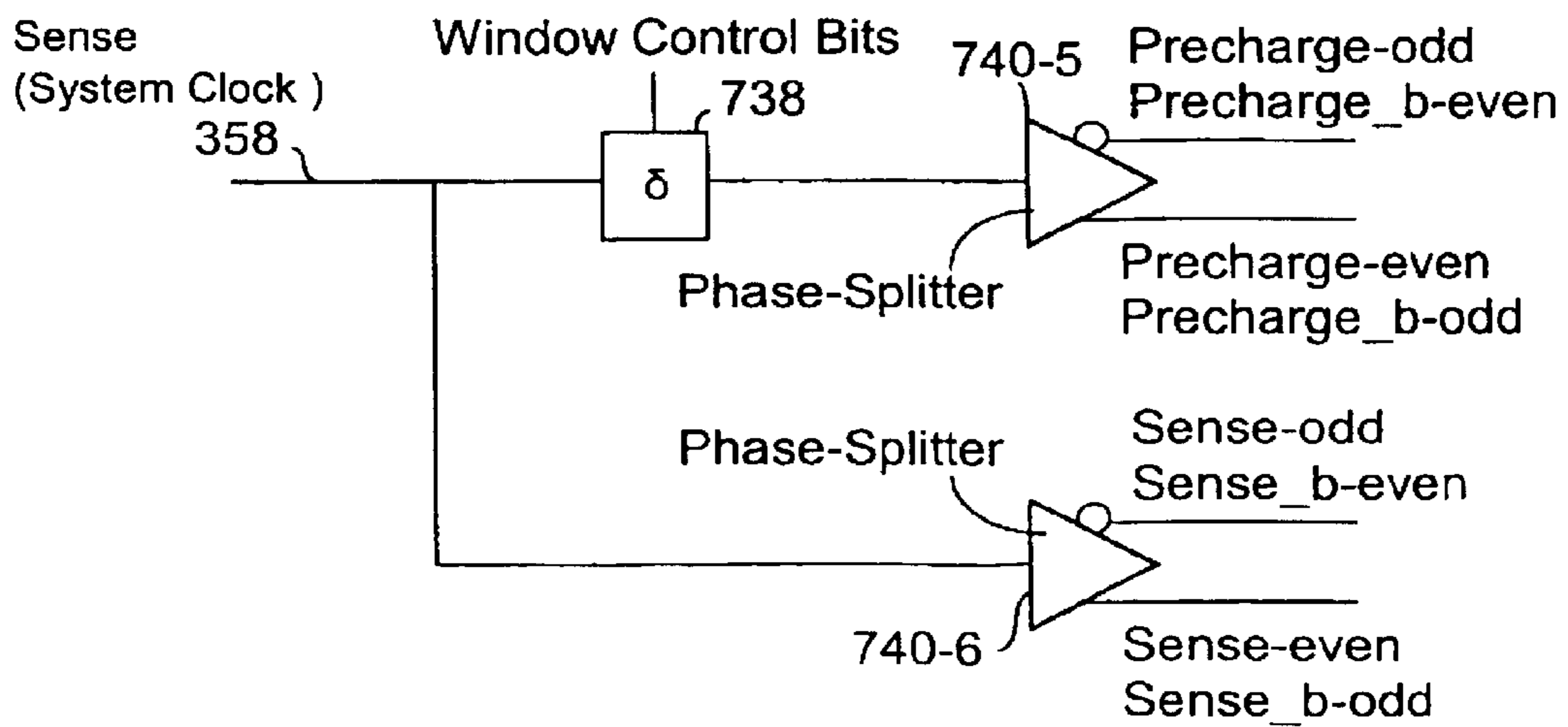
Circuit for Timing Diagram of Fig.17C
