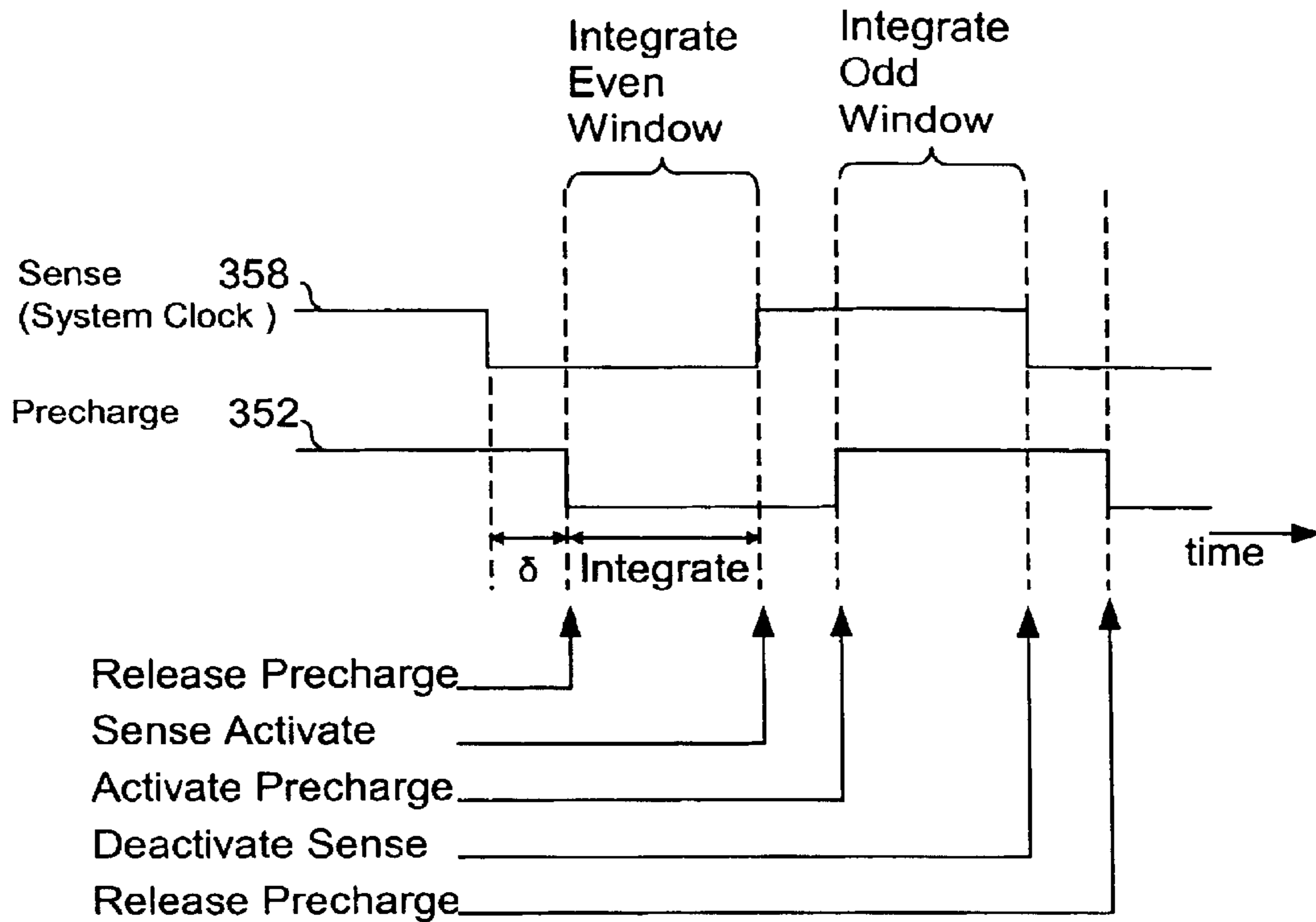
Timing Diagram of Precharge and Sense Signals
