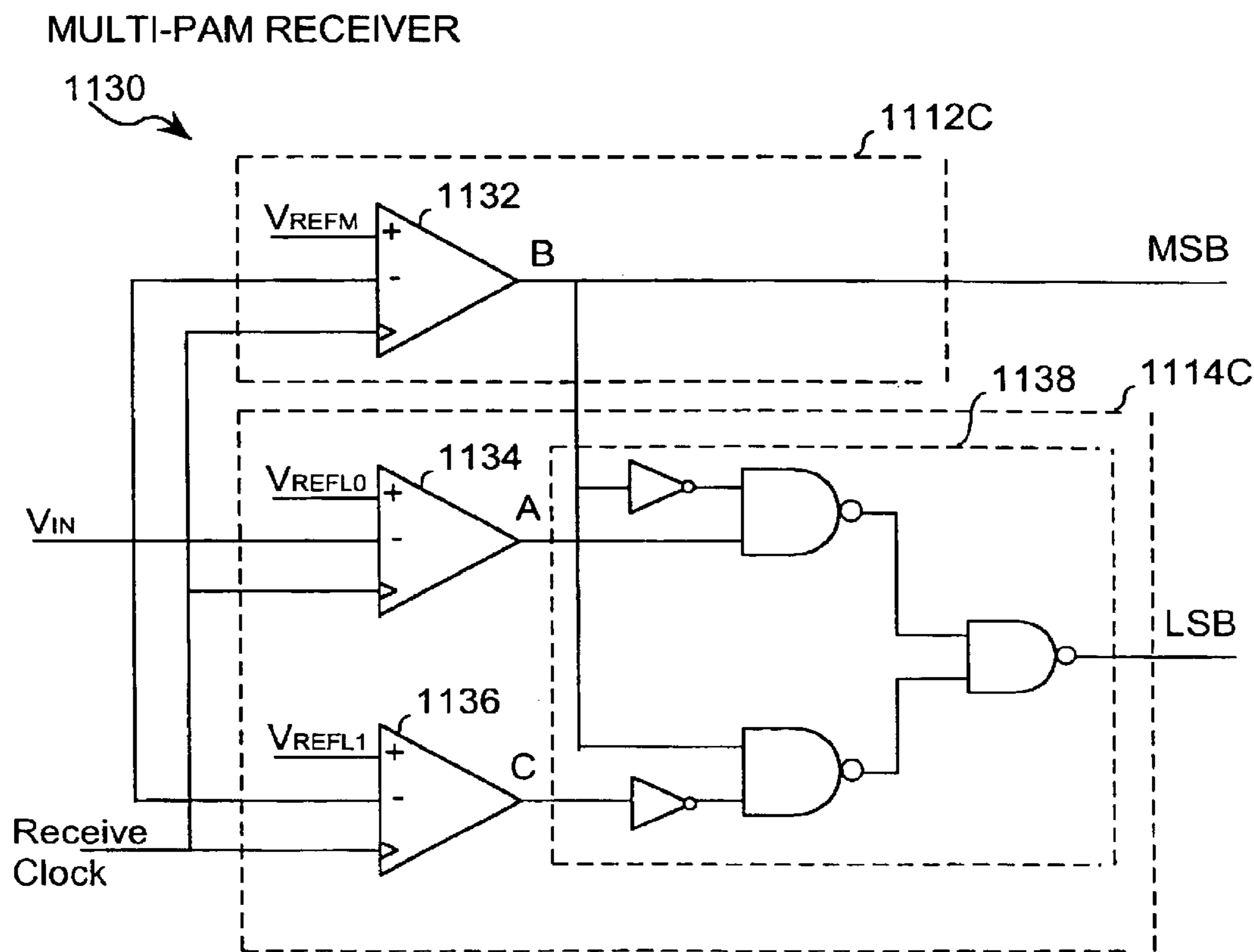
Multi-PAM Receiver FIG. 43
