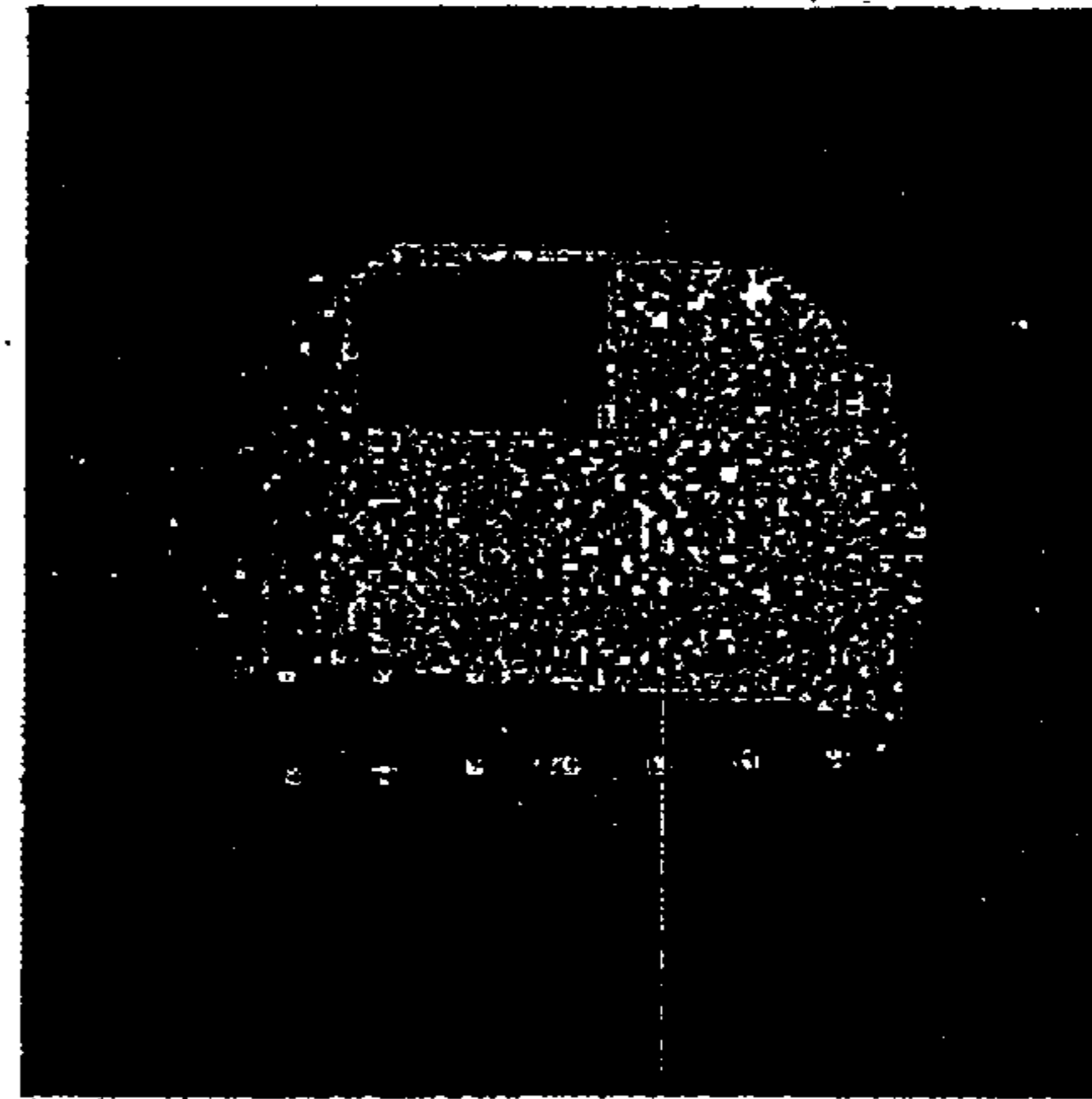
PURE m=(0 -1) HARMONICS
