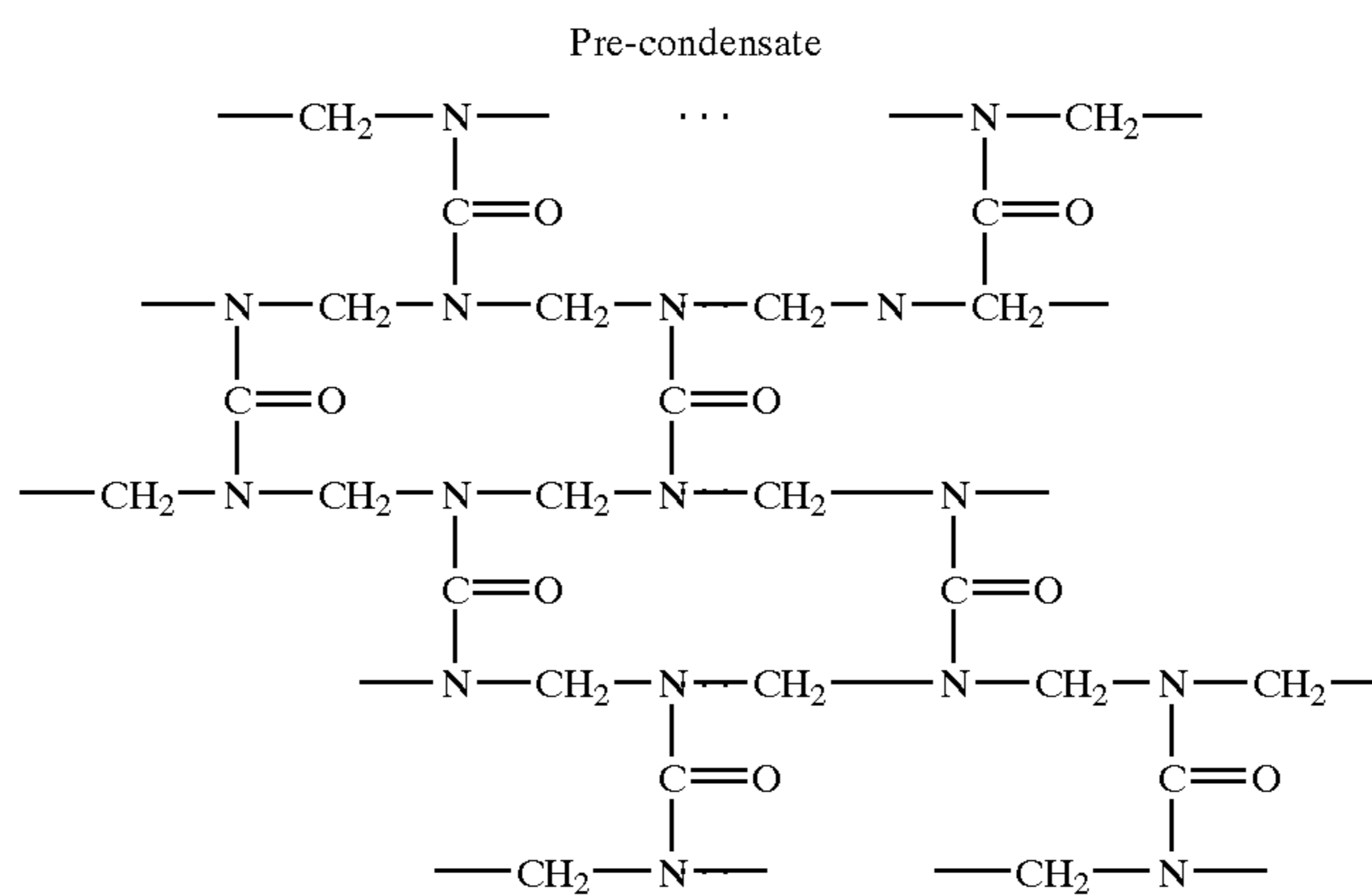
Polymethylene urea
