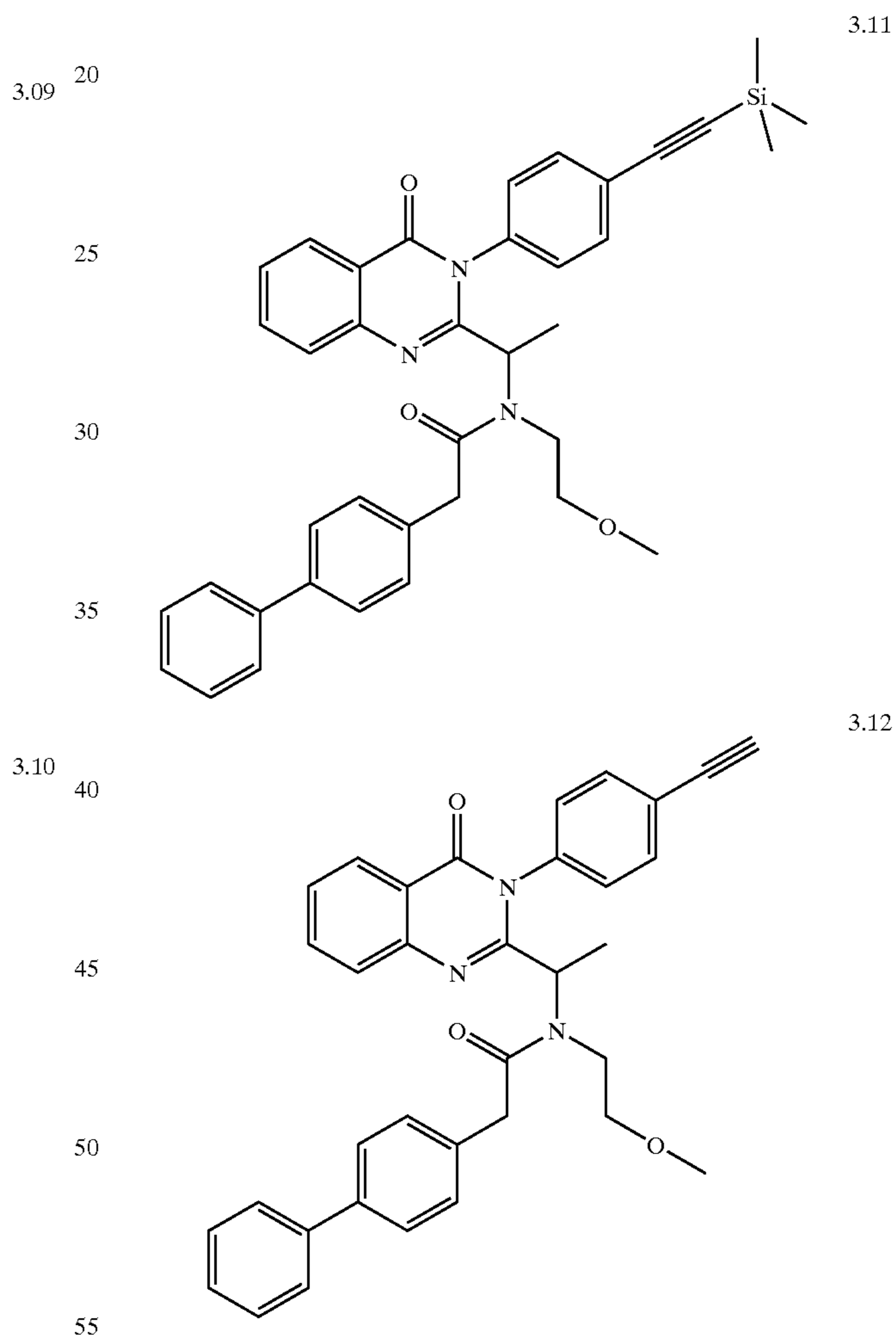
Synthesis of Compounds 3.11 and 3.12
