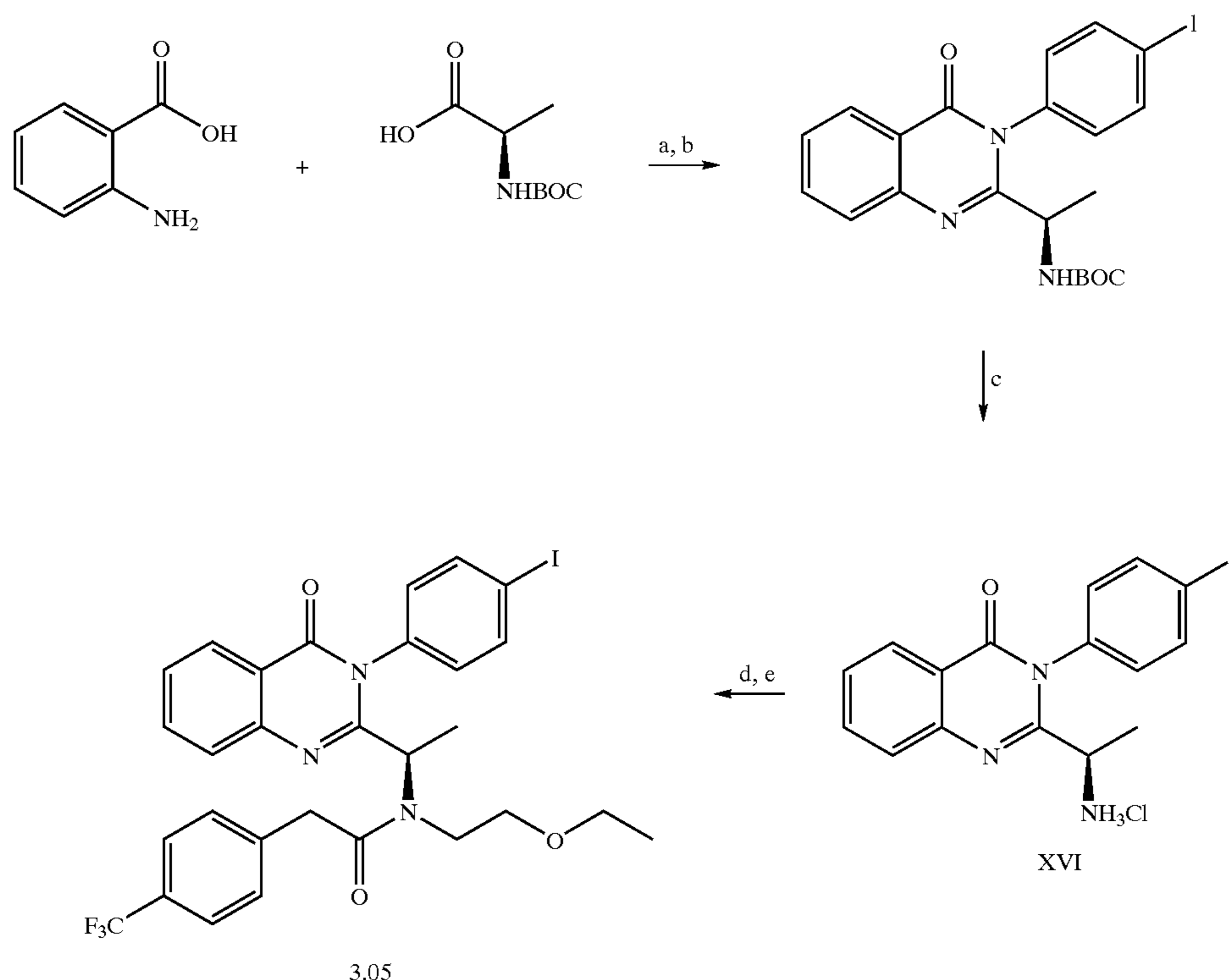
Scheme 5
