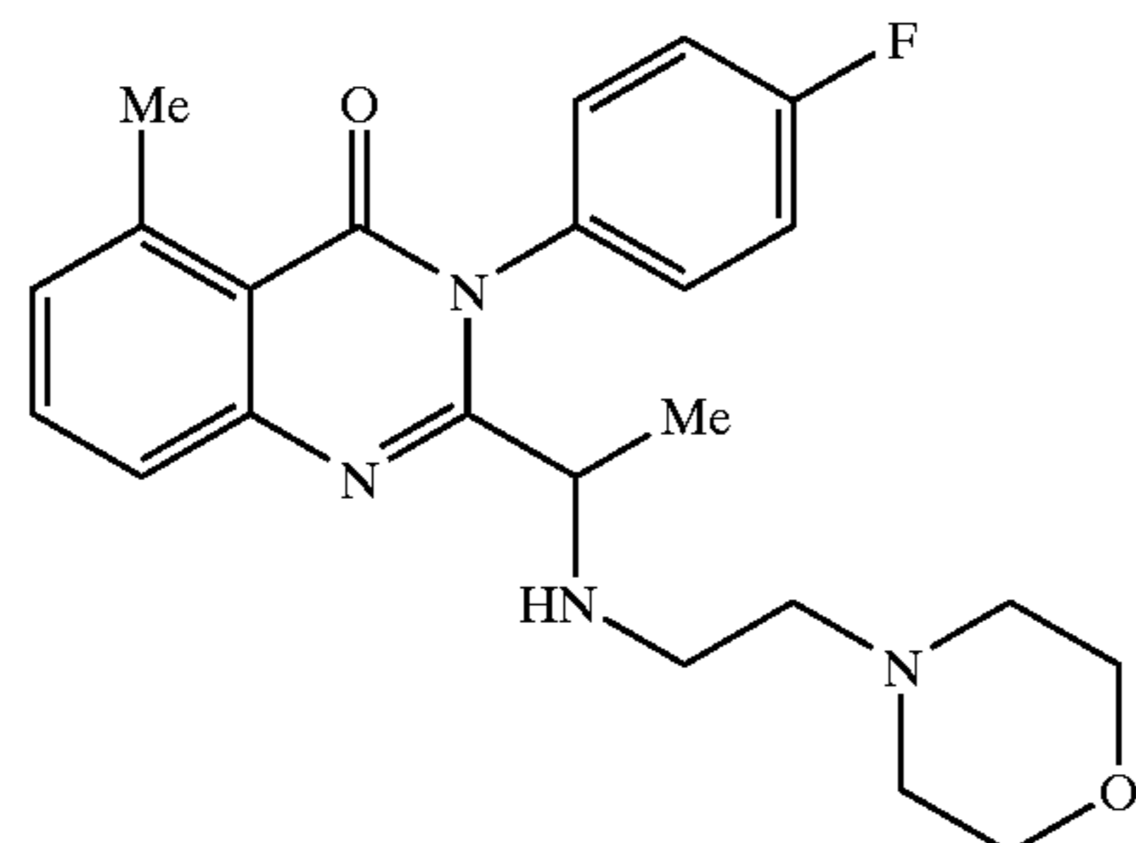
3-(4-Fluoro-phenyl)-5-methyl-2-[1-(2-morpholin-4-yl-ethylamino)-ethyl]-3H-quinazolin-4-one
