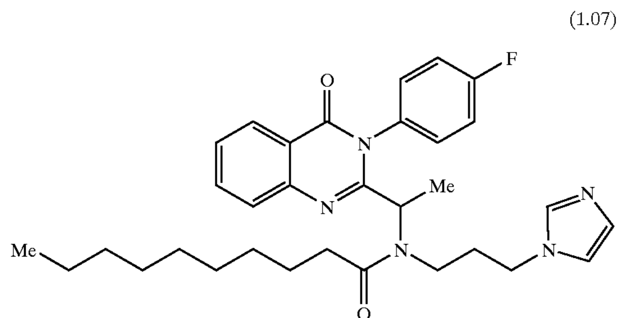
{1-[3-(4-fluoro-phenyl)-4-oxo-3,4-dihydro-quinazolin-2-yl]-ethyl}-(3-imidazol-1-yl)-propyl)-amide
