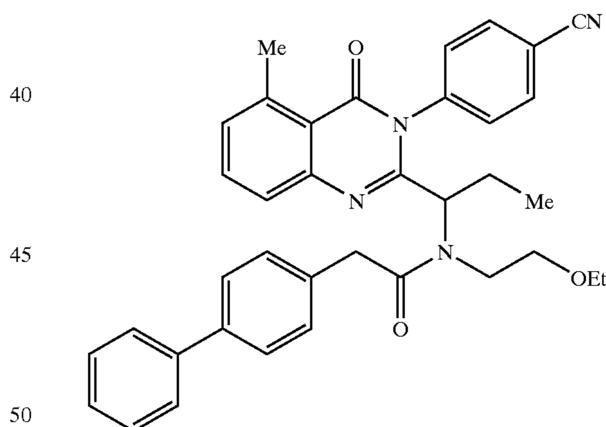
2-Biphenyl-4-yl-N-{1-[3-(4-cyano-phenyl)-5-methyl-4-oxo-3,4-dihydro-quinazolin-2-yl]-propyl}-N-(2-ethoxy-ethyl)-acetamide
