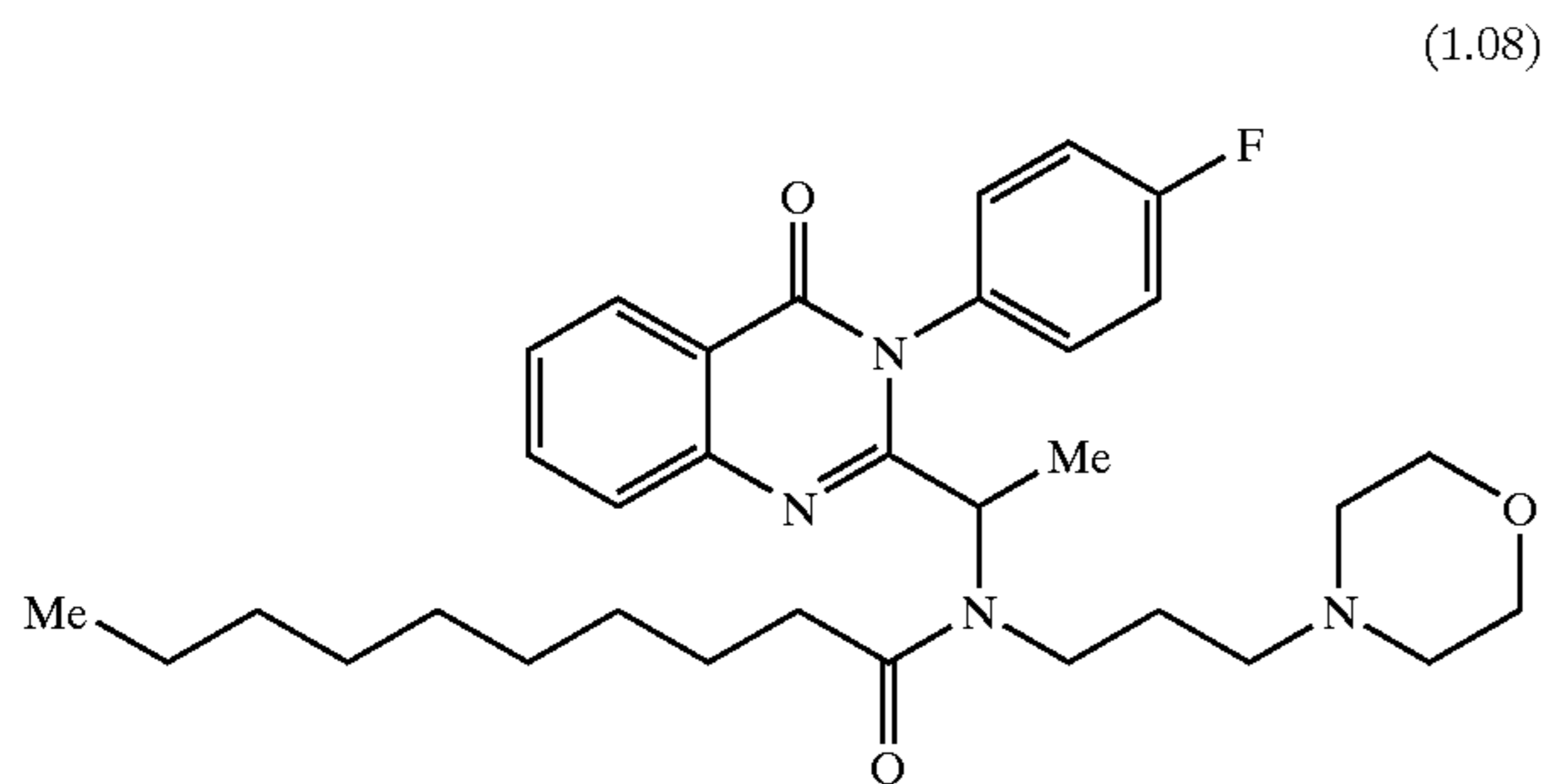
Decanoic acid {1-[3-(4-fluoro-phenyl)-4-oxo-3,4-dihydro-quinazolin-2-yl]-ethyl}-(3-morpholin-4-yl)-propyl)-amide
