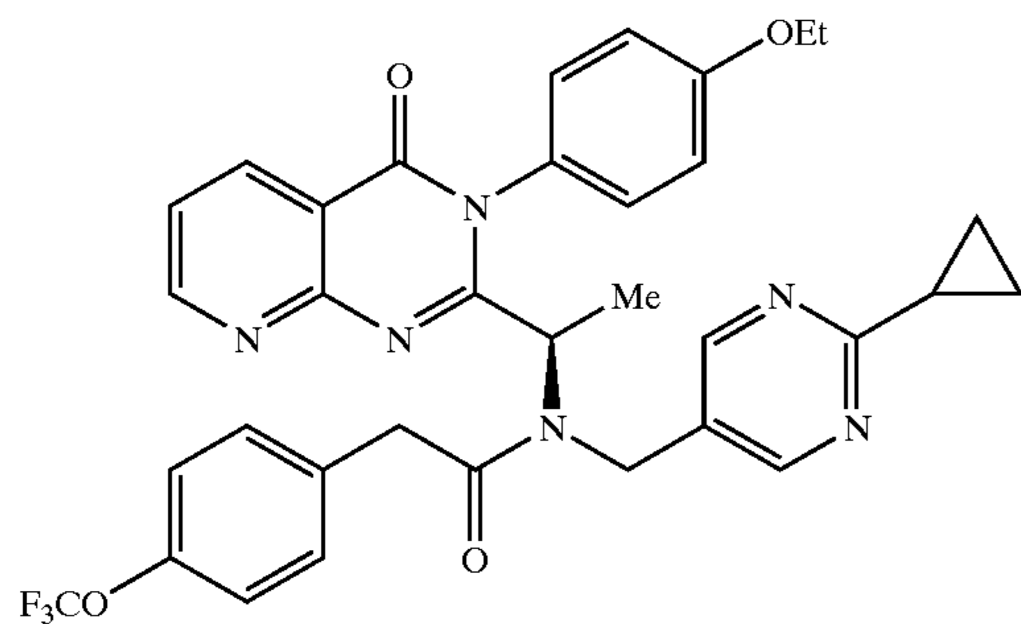
( R )- N -(2-Cyclopropyl-pyrimidin-5-ylmethyl)- N -{1-[3-(4-ethoxyphenyl)-4-oxo-3,4-dihydro-pyrido[2,3- d ]pyrimidin-2-yl]-ethyl}-2-(4-trifluoromethoxy-phenyl)-acetamide
