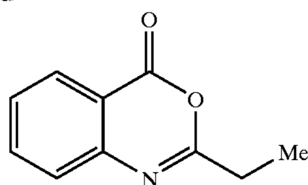
2-Ethyl-benzo[d][1,3]oxazin-4-one (III)
