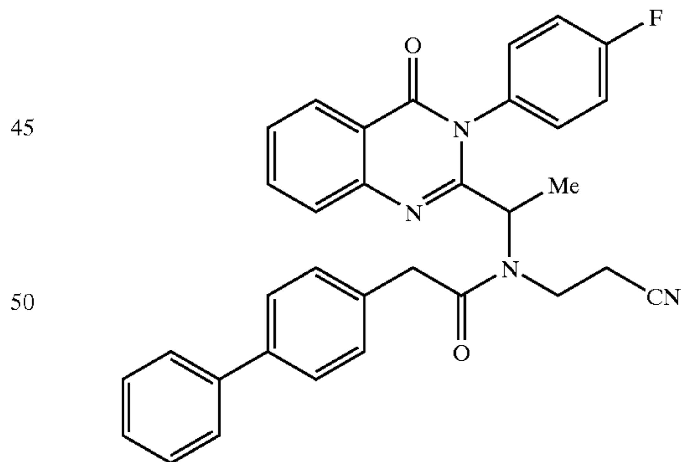
2-Biphenyl-4-yl-N-(2-cyano-ethyl)-N-(1-[3-(4-fluoro-phenyl)-4-oxo-3,4-dihydro-quinazolin-2-yl]-ethyl)-acetamide
