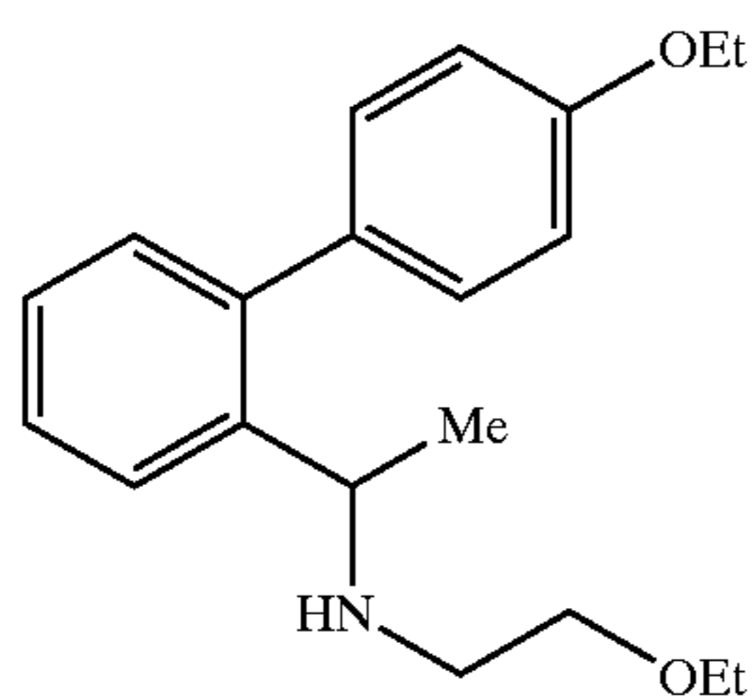
[1-(4'-Ethoxy-biphenyl-2-yl)-ethyl]-(2-ethoxy-ethyl)-amine
