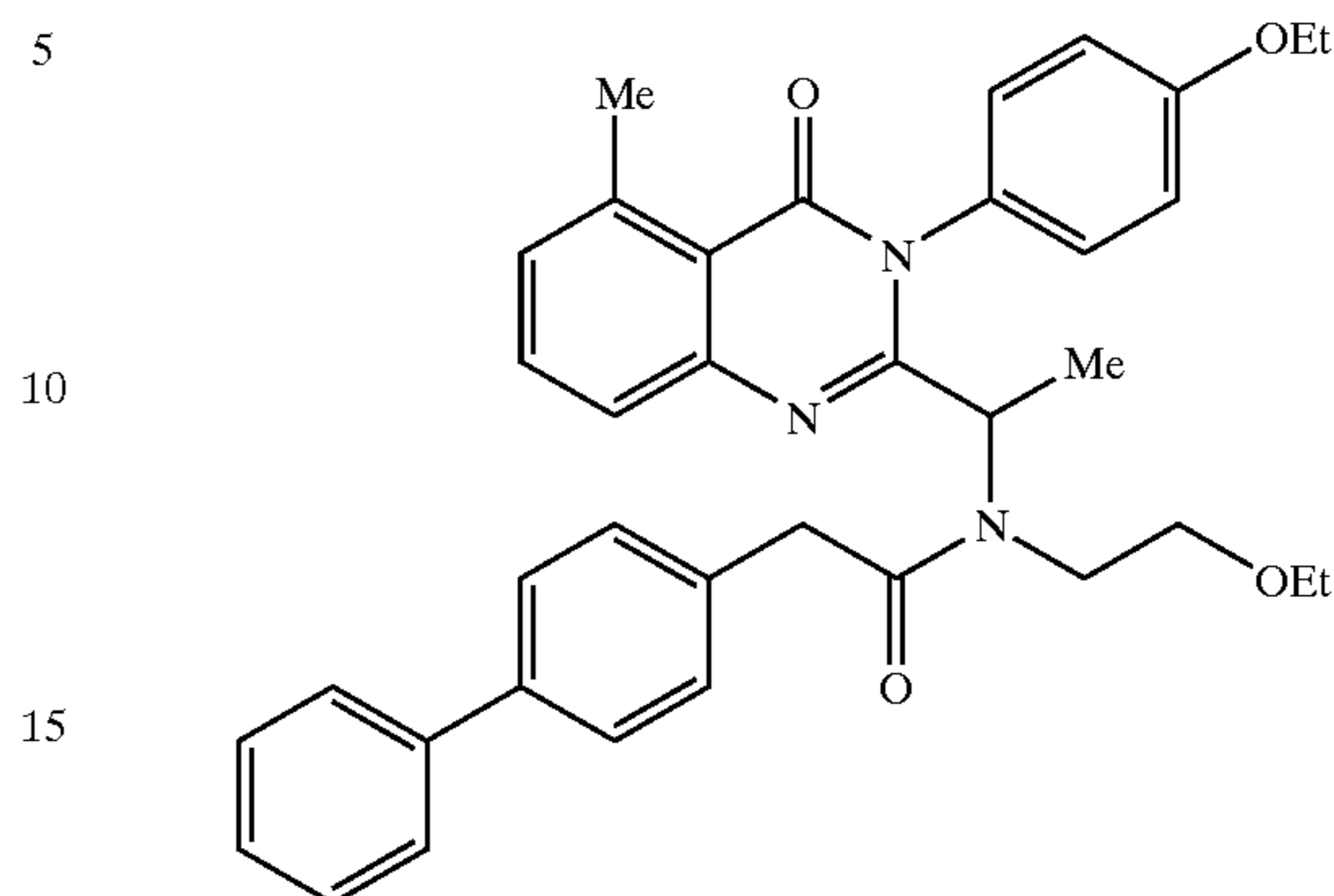
2-Biphenyl-4-yl-N-(2-ethoxy-ethyl)-N-{1-[3-(4-ethoxy-phenyl)-5-methyl-4-oxo-3,4-dihydro-quinazolin-2-yl]-ethyl}-acetamide
