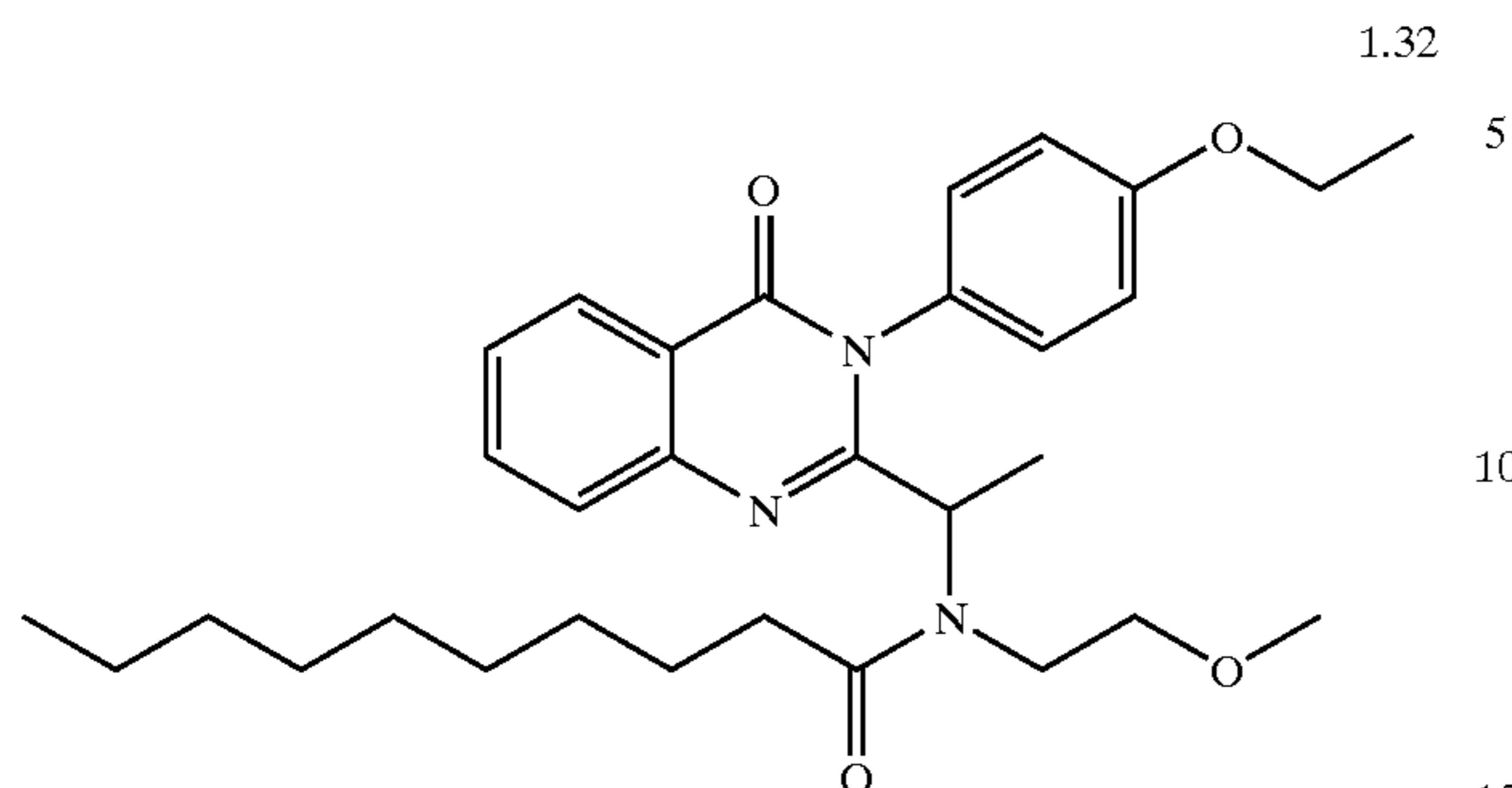
Decanoic acid {1-[3-(4-ethoxy-phenyl)4-oxo-3,4-dihydro-quinazolin-2-yl]-ethyl}-(2-methoxy-ethyl)-amide
