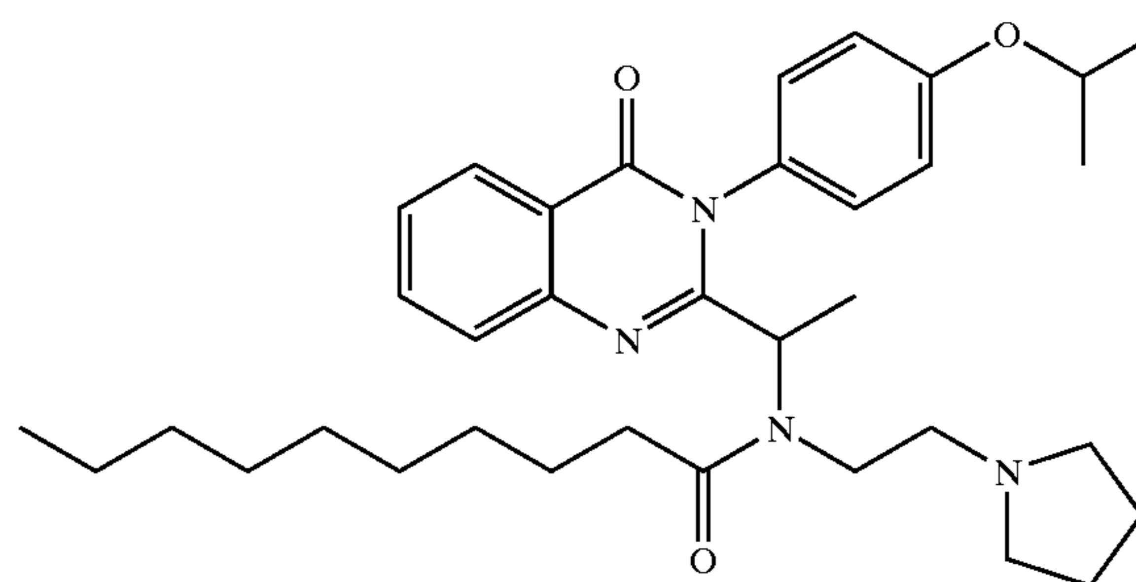
Decanoic acid {1-[3-(4-isopropoxy-phenyl)4-oxo-3,4-dihydro-quinazolin-2-yl]-ethyl}-(2-pyrrolidin-1-yl-ethyl)-amide
