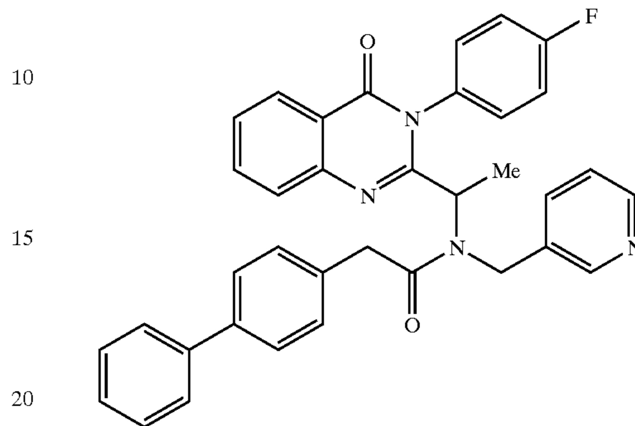
2-Biphenyl-4-yl-N-(1-[3-[(4-fluoro-phenyl)-4-oxo-3,4-dihydro-quinazolin-2-yl]-ethyl]-ethyl)-N-pyridin-3-ylmethylacetamide
