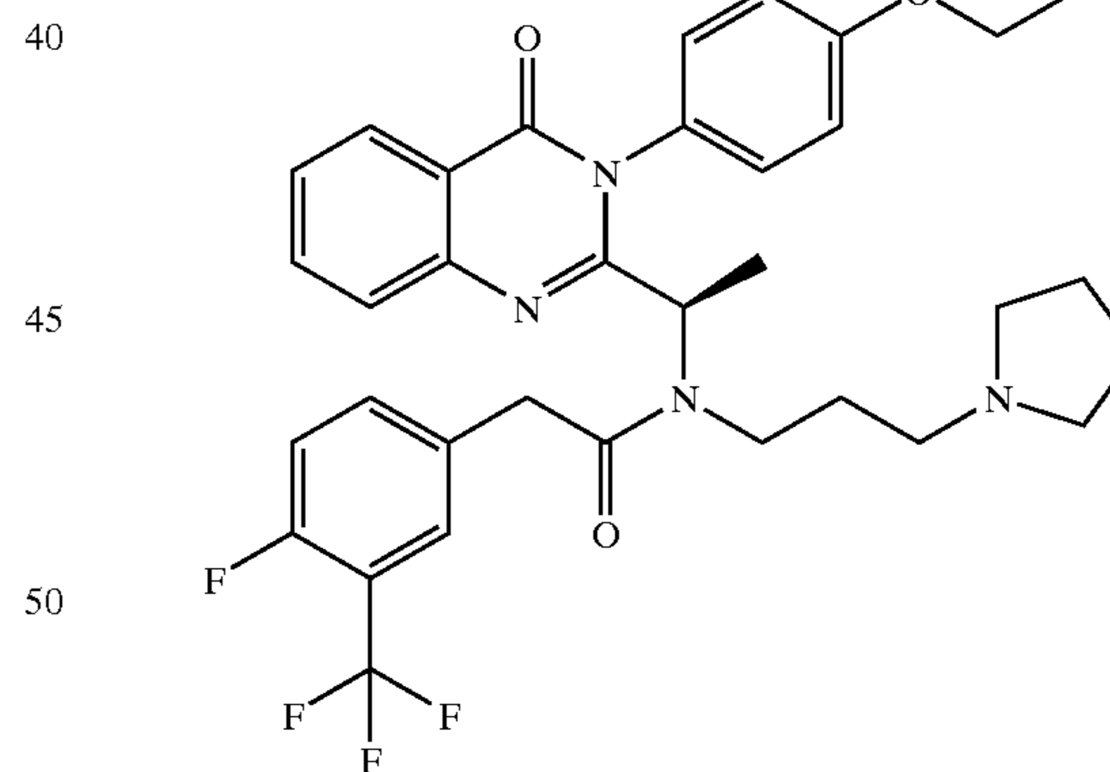
N -{1-[3-(4-Ethoxy-phenyl)-4-oxo-3,4-dihydro-quinazolin-2-yl]-ethyl}-2-(4-fluoro-3-trifluoromethyl-phenyl)- N -(3-pyrrolidin-1-yl-propyl)-acetamide
