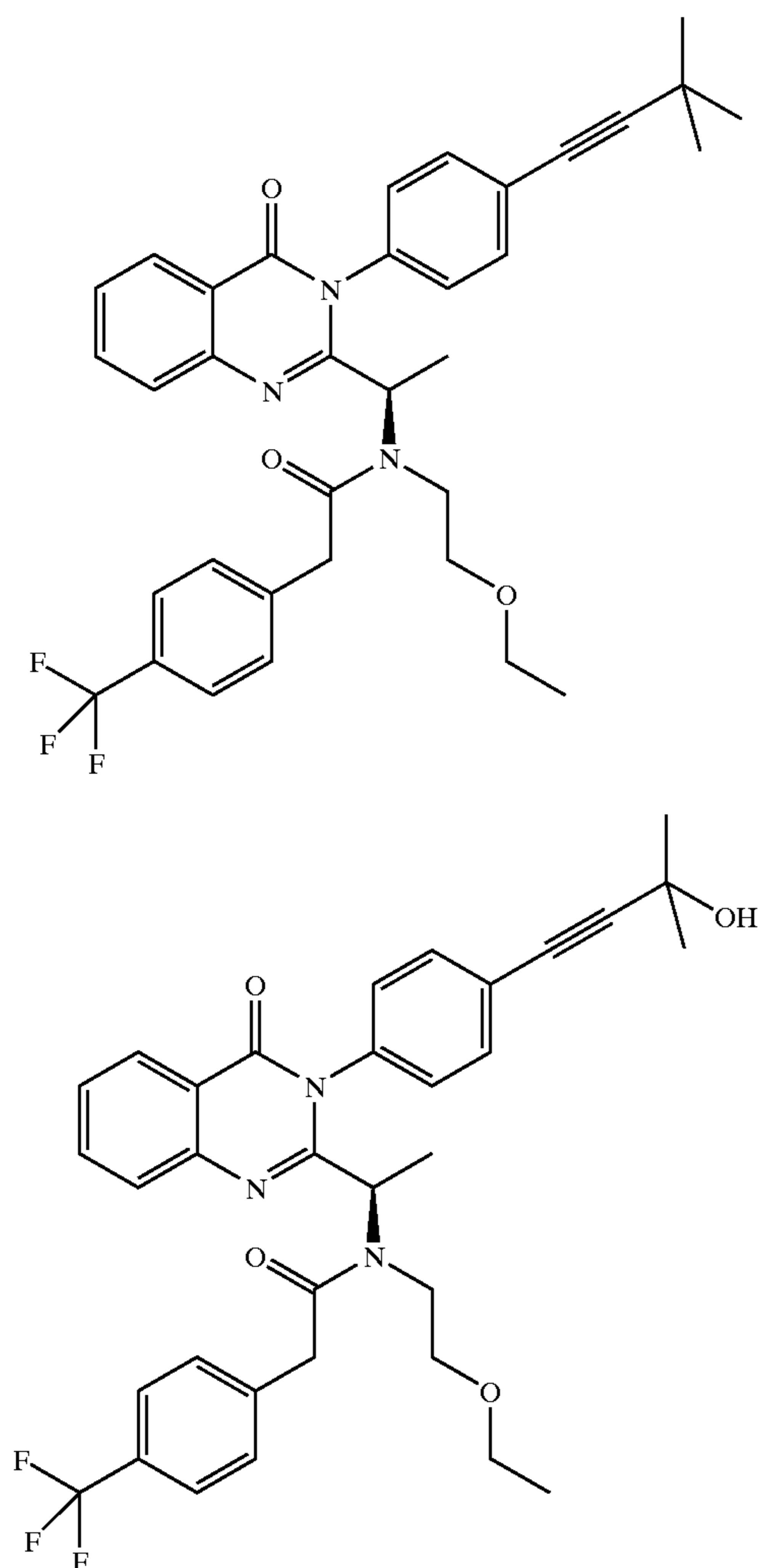
Synthesis of Compounds 3.09 and 3.10
