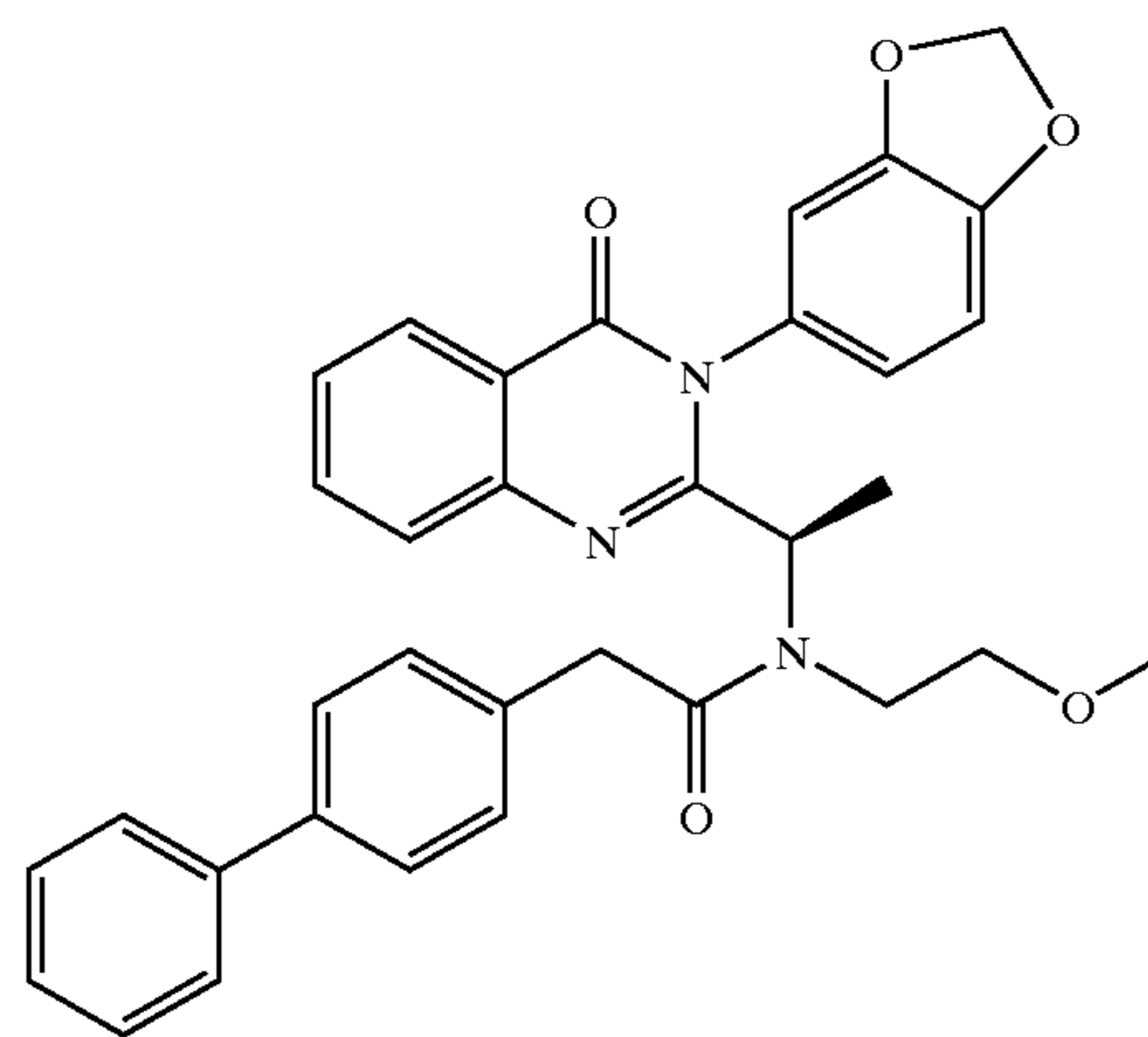
N-[1-(3-benzo[1,3]dioxol-5-yl-4-oxo-3,4-dihydro-quinazolin-2-2yl)-ethyl]-2-biphenyl-4-yl-N-(2-methoxy-ethyl)-acetamide
