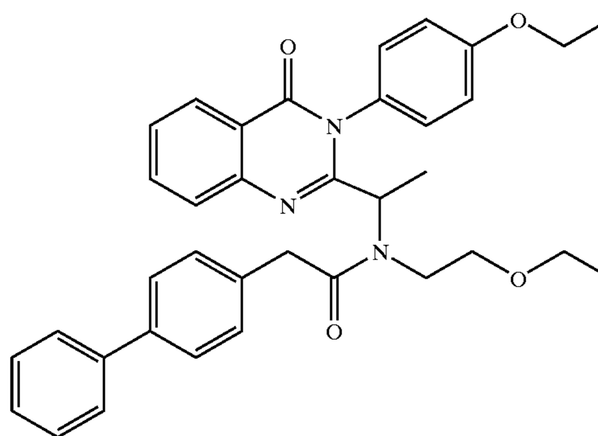
2-Biphenyl-4-yl-N-(2-ethoxy-ethyl)-N-{1-[3-(4-ethoxy-phenyl)-4-oxo-3,4-dihydro-quinazolin-2-yl]-ethyl}-acetamide
