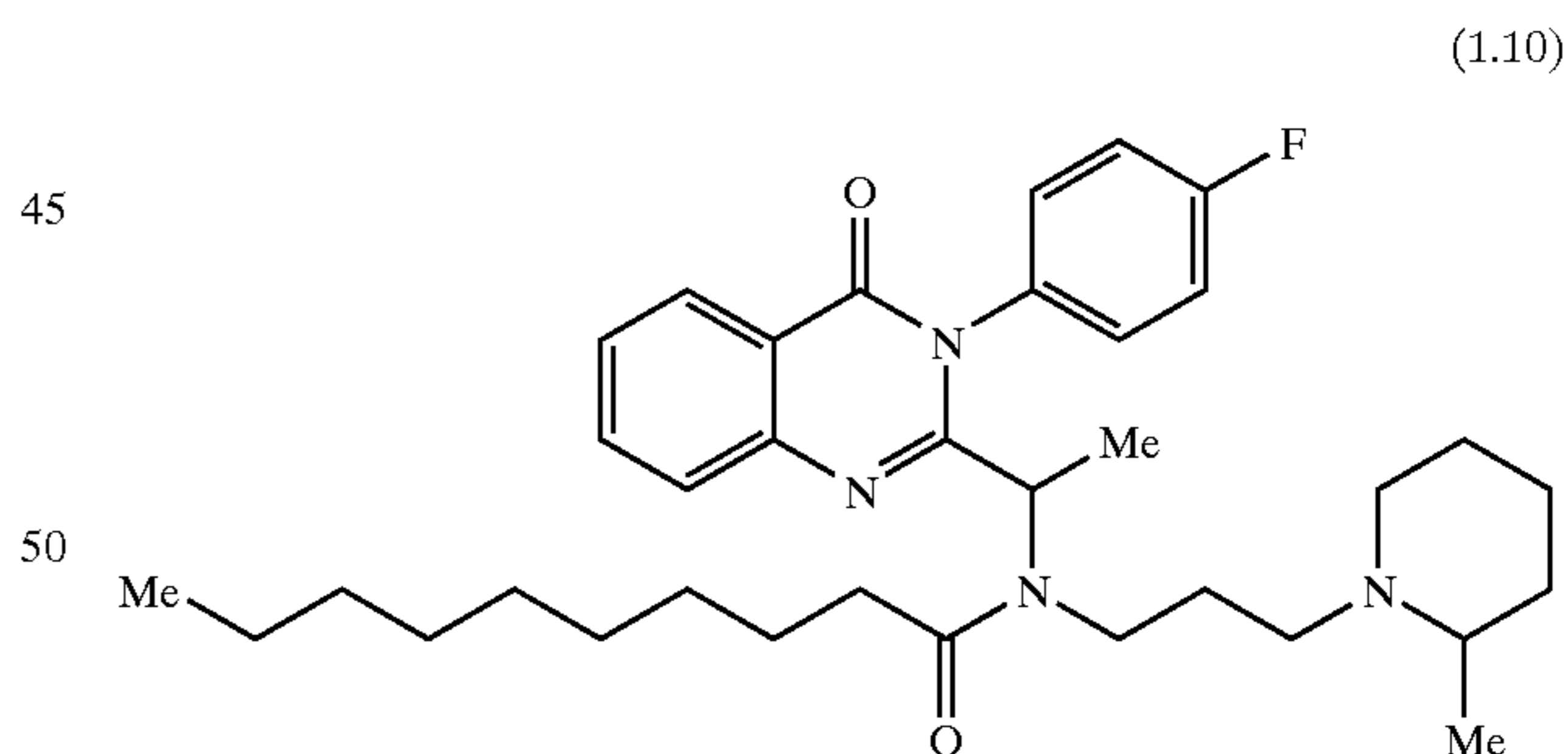
Decanoic acid {1-[3-(4-fluoro-phenyl)-4-oxo-3,4-dihydro-quinazolin-2-yl]-ethyl} [3-(2-methyl-piperidin-1-yl)-propyl]-amide
