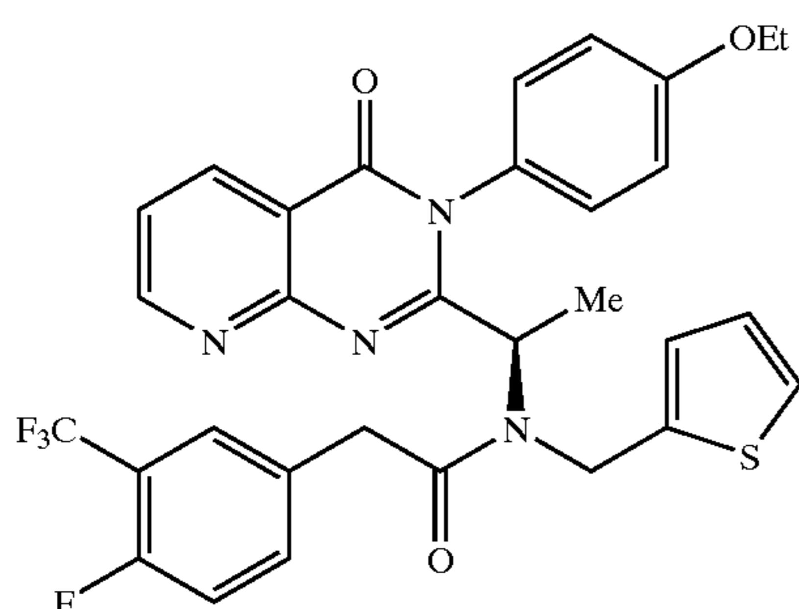
( R )- N -[1-[3-(4-Ethoxy-phenyl)-4-oxo-3,4-dihydro-pyrido[2,3- d ]pyrimidin-2-yl]-ethyl]-2-(4-fluoro-3-trifluoromethyl-phenyl)- N -thiophen-2-ylmethyl-acetamide
