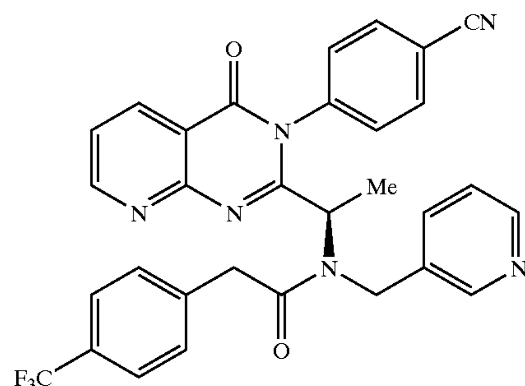
Synthesis of Compound 3.20
