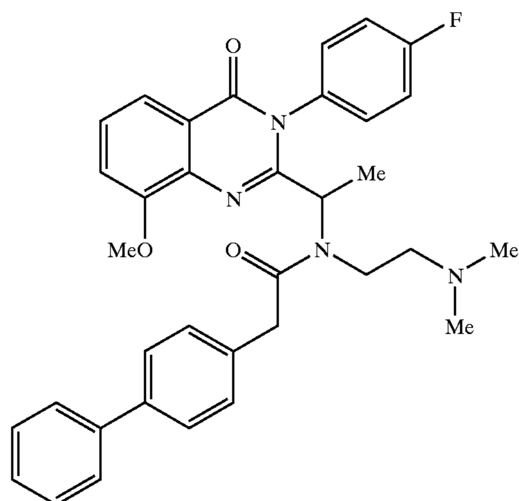
2-Biphenyl-4-yl-N-(2-dimethylamino-ethyl)-N-{1-[3-(4-fluoro-phenyl)-8-methoxy-4-oxo-3,4-dihydro-quinazolin-2-yl]-ethyl}-acetamide
