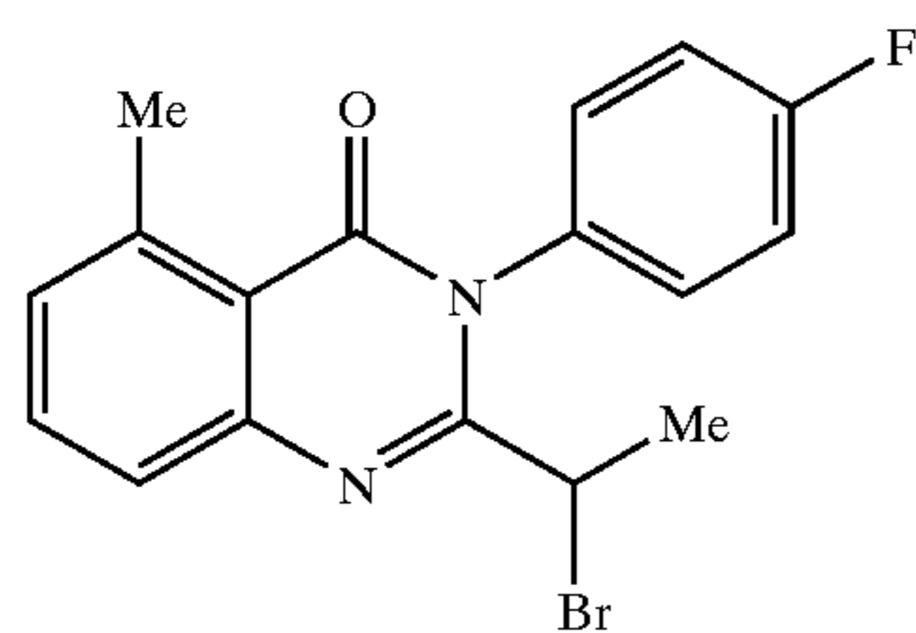
2-(1-Bromo-ethyl)-3-(4-fluoro-phenyl)-5-methyl-3H-quinazolin-4-one
