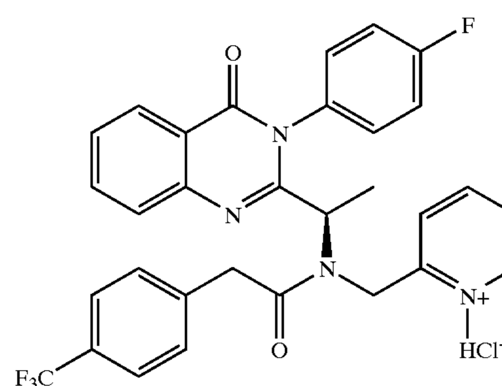
Synthesis of Compound 3.03 and Compound 3.03•HCl
