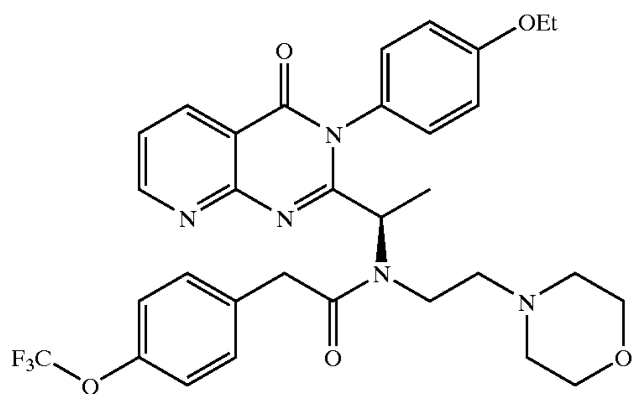
N -{1-[3-(4-Ethoxy-phenyl)-4-oxo-3,4-dihydro-pyridol[2,3- d ]pyrimidin-2-yl]-ethyl}- N -(2-morpholin-4-yl-ethyl)-2-(4-trifluoromethoxy-phenyl)-acetamide
