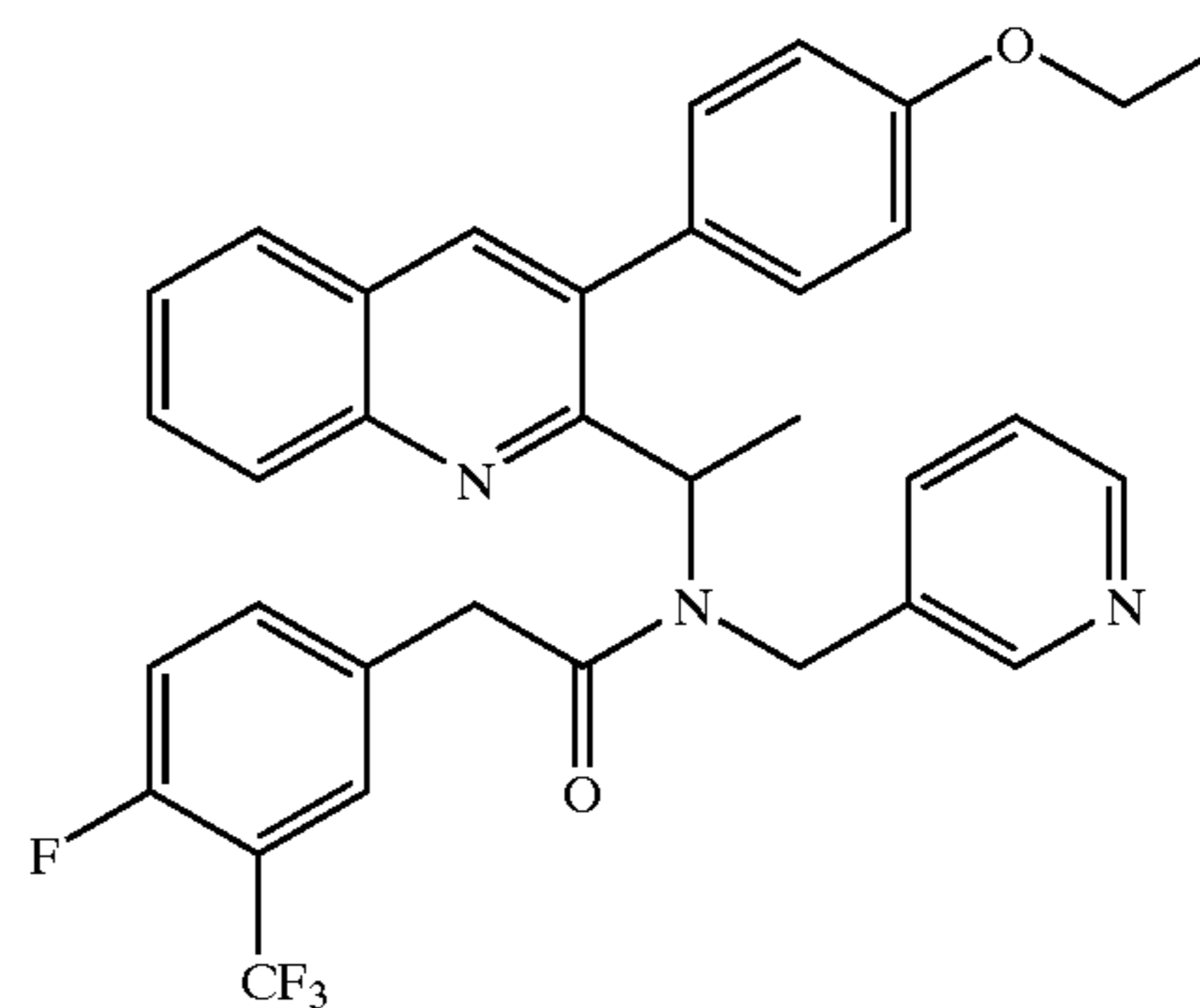
N -{1-[3-(4-Ethoxy-phenyl)-quinolin-2-yl]-ethyl}-2-(4-fluoro-3-trifluoromethyl-phenyl)- N -pyridin-3-ylmethyl-acetamide
