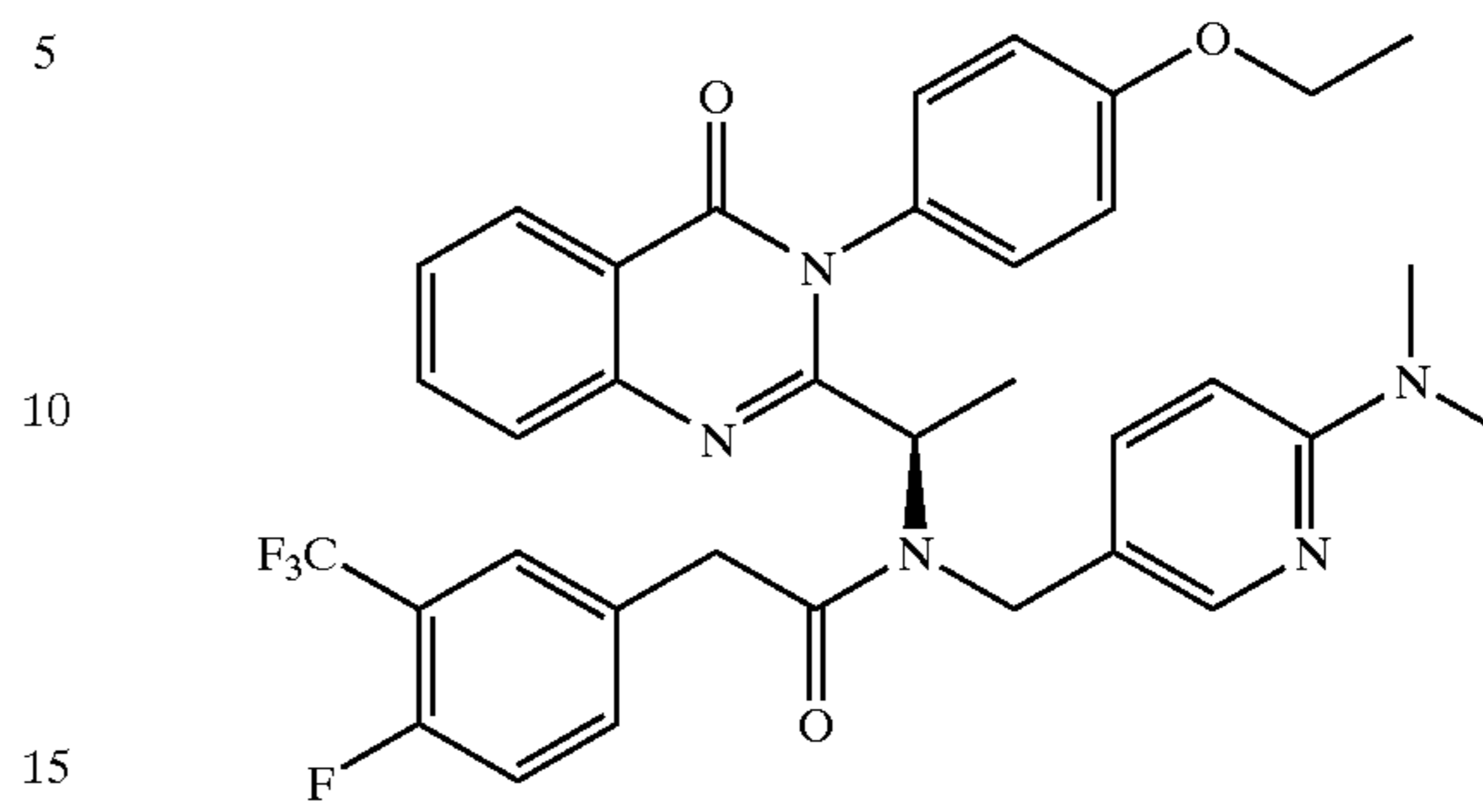
(-)-( R )- N -(6-Dimethylamino-pyridin-3-ylmethyl)- N -(1-(3-(4-ethoxyphenyl)-4-oxo-3,4-dihydro-quinazolin-2-yl)-ethyl)-2-(4-fluoro-3-trifluoromethyl-phenyl)-acetamide
