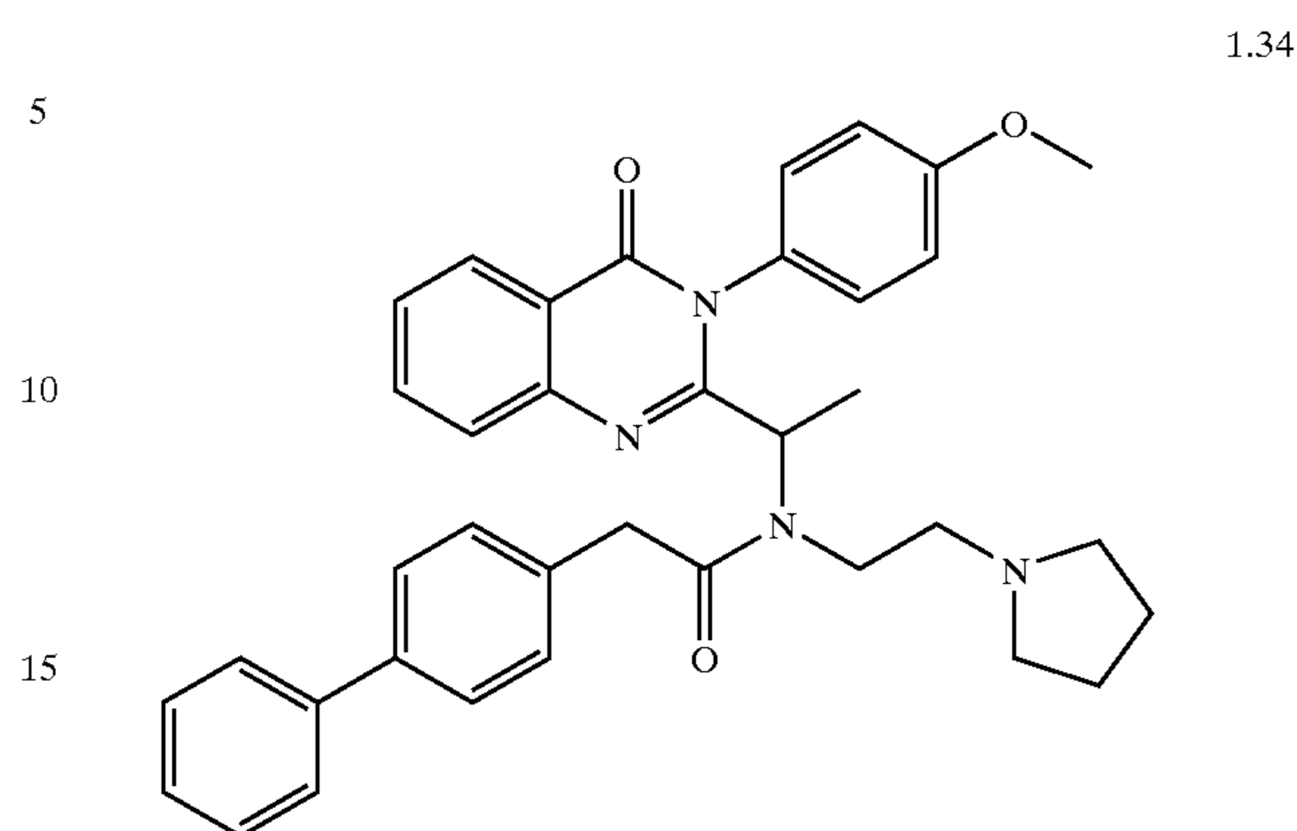
2-Biphenyl-4-yl- N -{1-[3-(4-methoxy-phenyl)4-oxo-3,4-dihydro-quinazolin-2-yl]-ethyl}- N -(2-pyrrolidin-1-yl-ethyl)-acetamide
