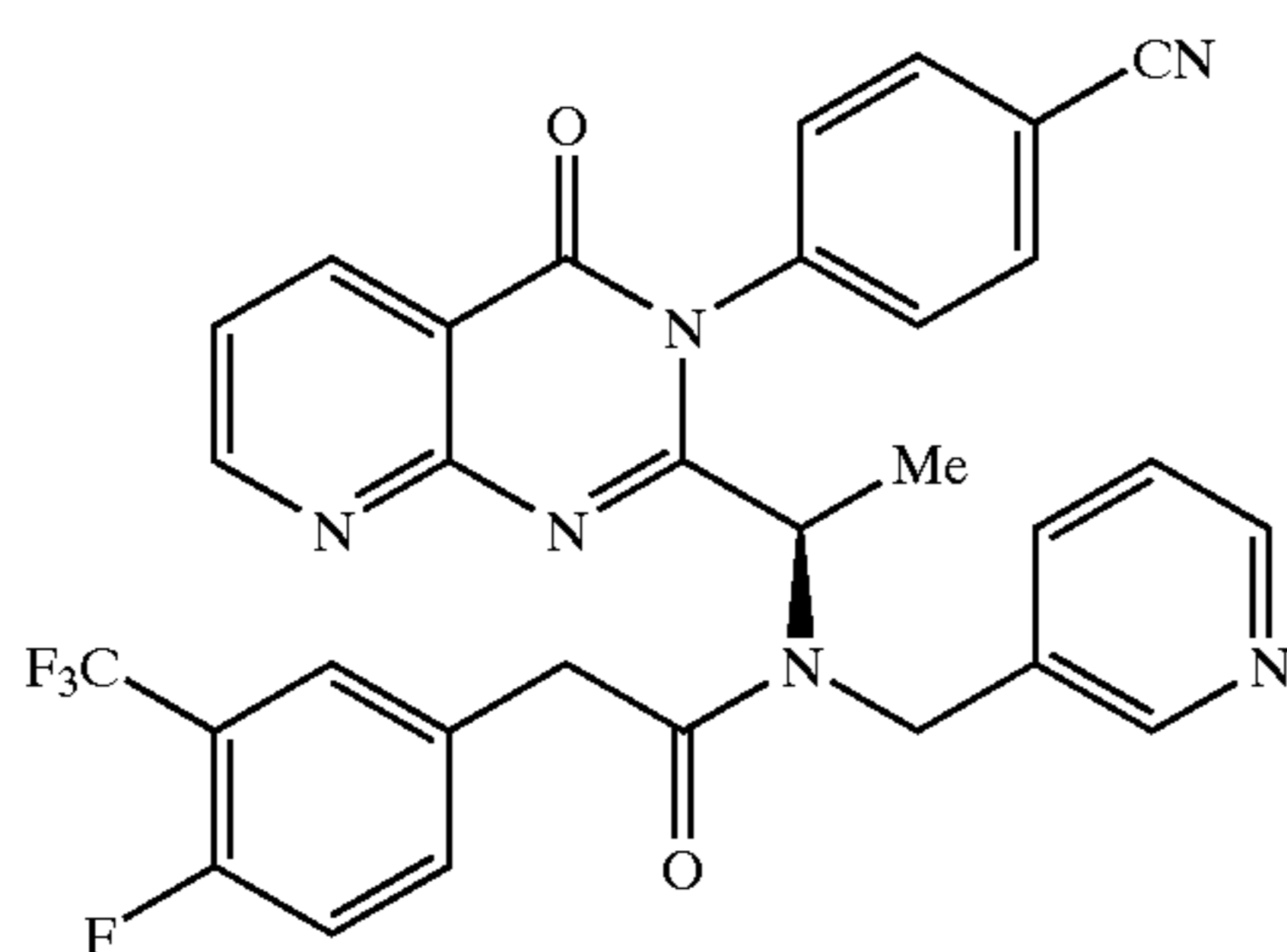
( R )- N -{1-[3-(4-Cyano-phenyl)-4-oxo-3,4-dihydro-pyrido[2,3- d ]pyrimidin-2-yl]-ethyl}-2-(4-fluor-3-trifluoromethyl-phenyl)- N -pyridin-3-ylmethyl-acetamide
