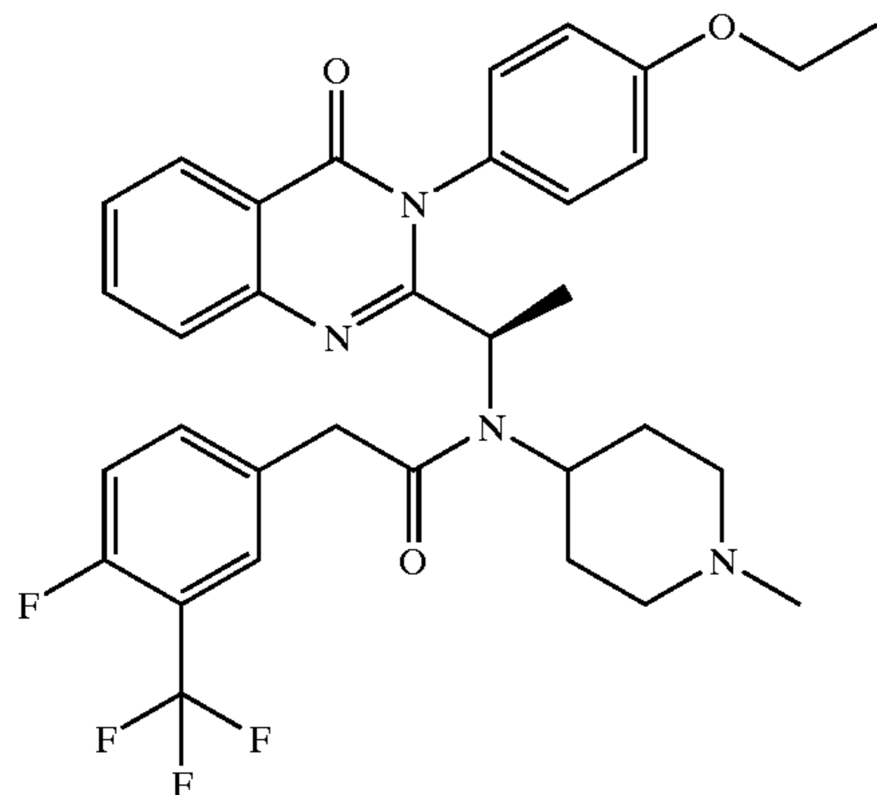
N -{1-[3-(4-Ethoxy-phenyl)-4-oxo-3,4-dihydro-quinazolin-2-yl]-ethyl}-2-(4-fluoro-3-trifluoromethyl-phenyl)- N -(1-methyl-piperidin-4-yl)-acetamide
