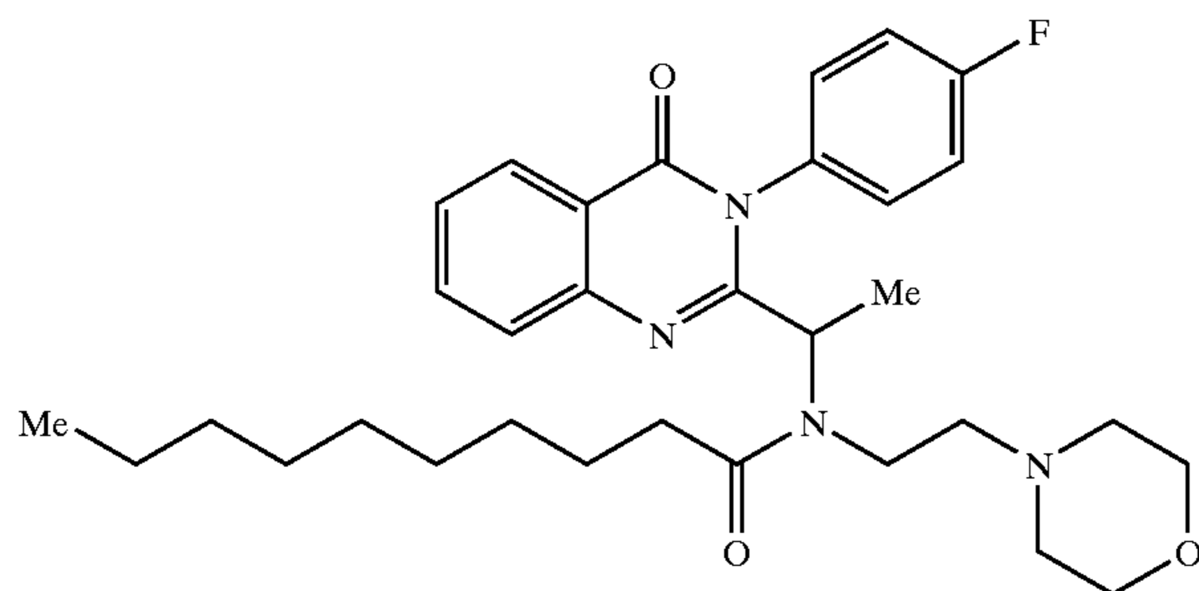
Decanoic acid {1-[3-(4-fluoro-phenyl)-4-oxo-3,4-dihydro-quinazolin-2-yl]-ethyl}-(2-morpholin-4-yl-ethyl)-amide
