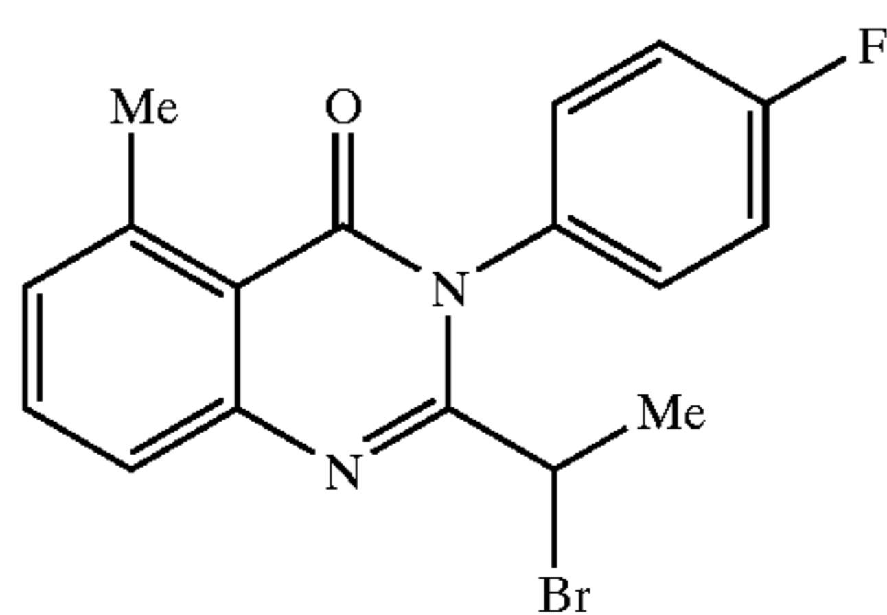
2-(1-Bromo-ethyl)-3-(4-fluoro-phenyl)-5-methyl-3H-quinazolin-4-one
