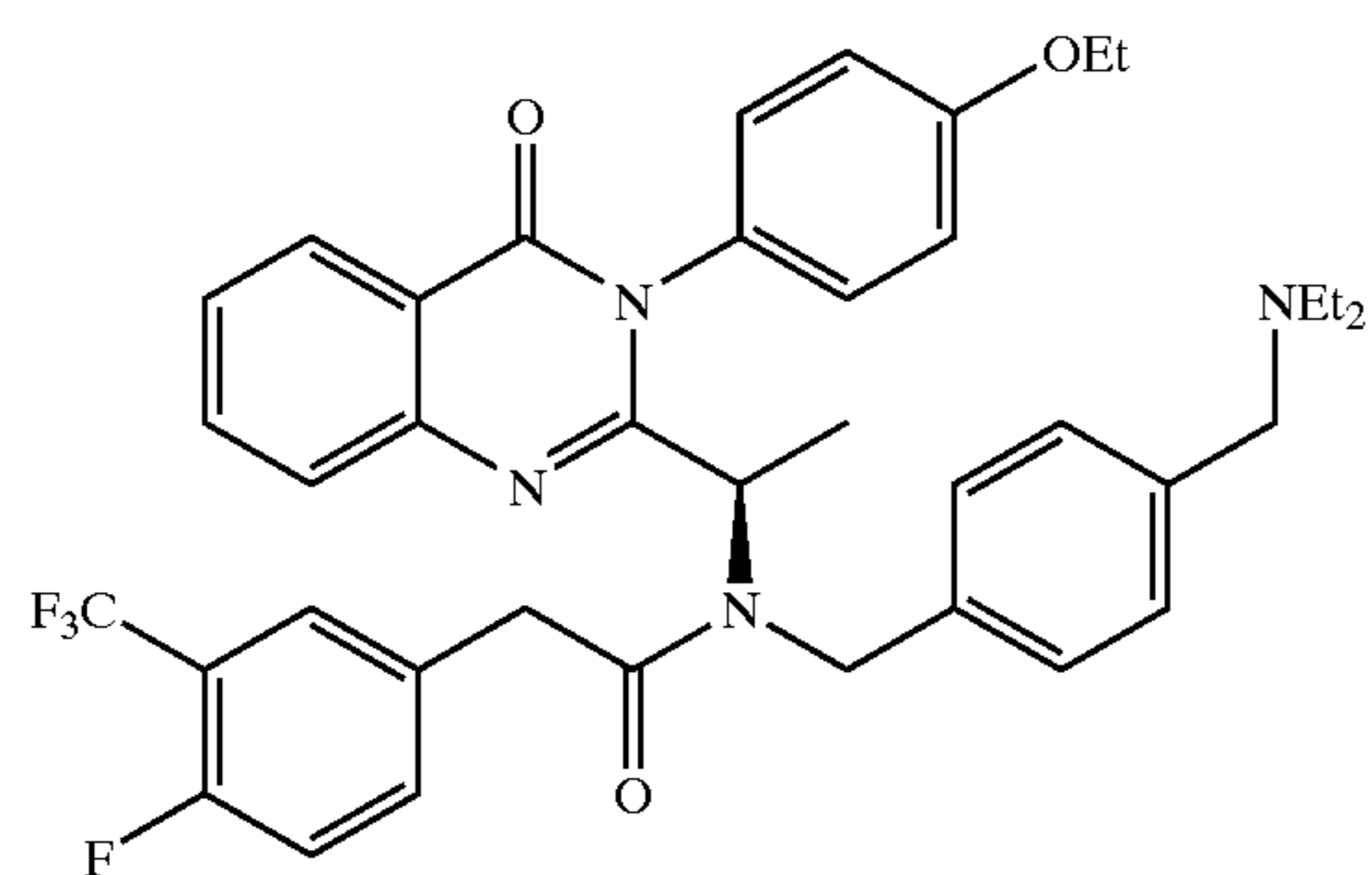
N -(4-Diethylaminomethyl-benzyl)- N -{1-[3-(4-ethoxy-phenyl)-4-oxo-3,4-dihydro-quinazolin-2-yl]-ethyl}-2-(4-fluoro-3-trifluoromethyl-phenyl)-acetamide
