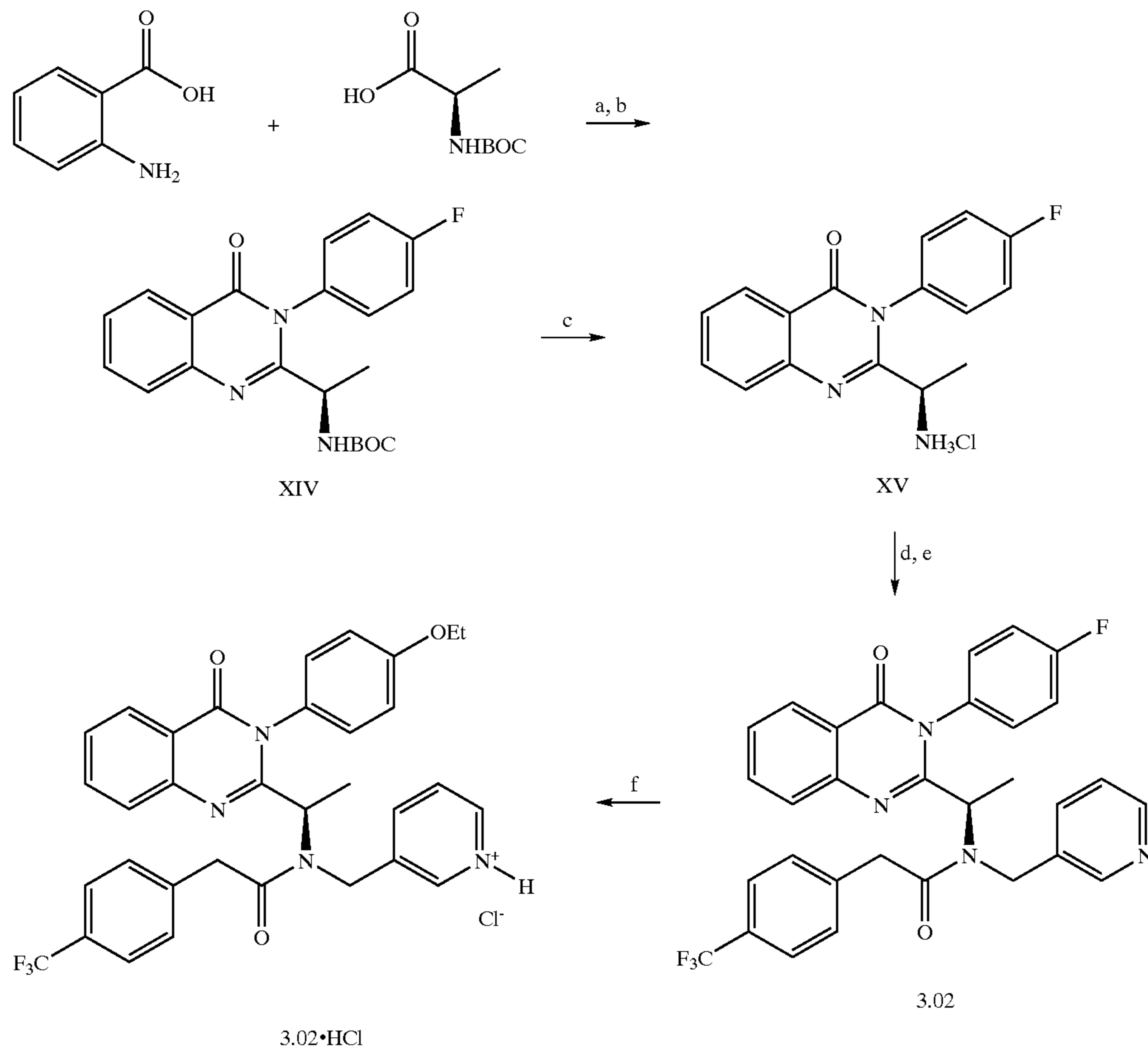
Scheme 4
