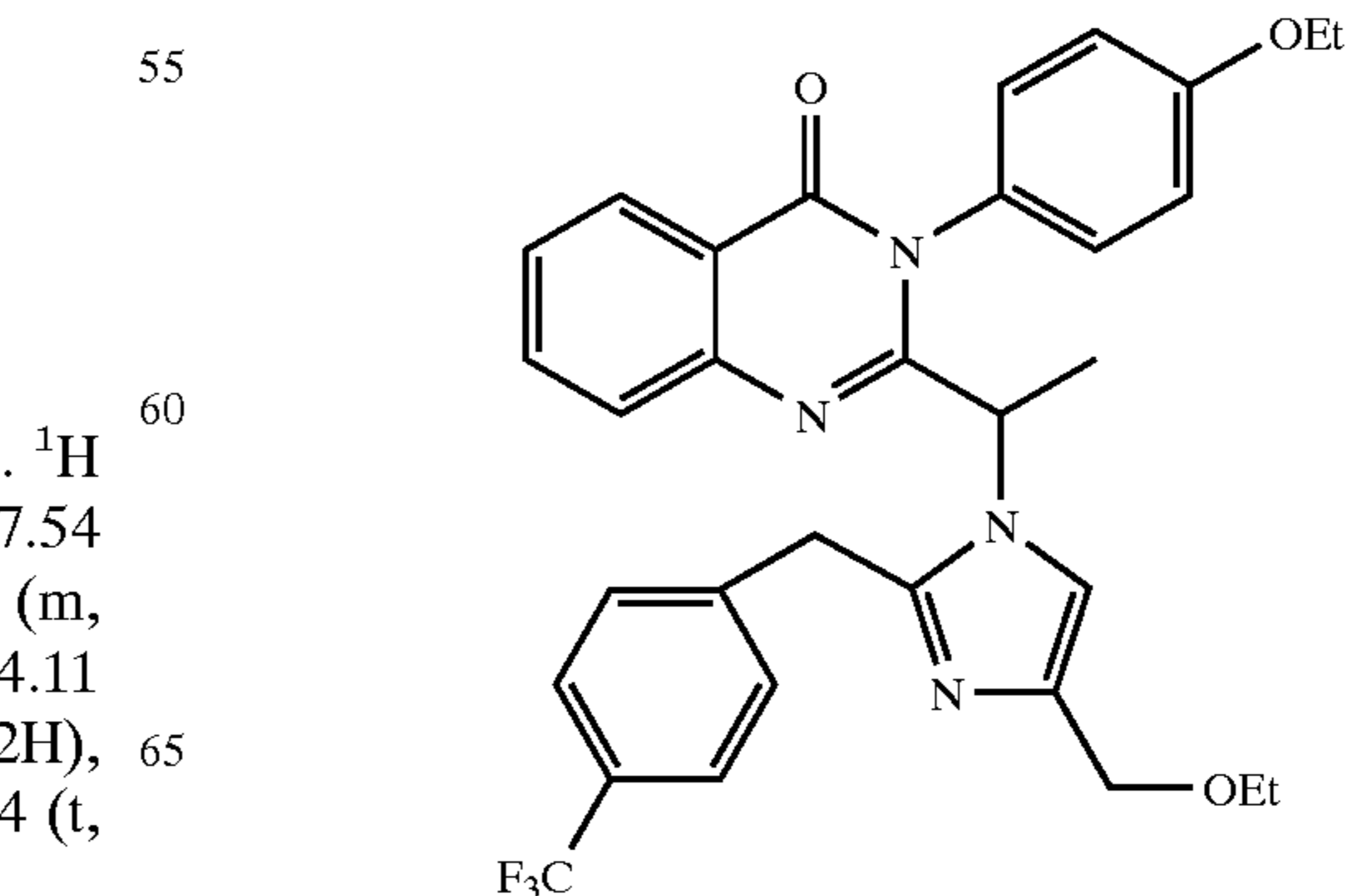
Preparation of Compound 6.10
