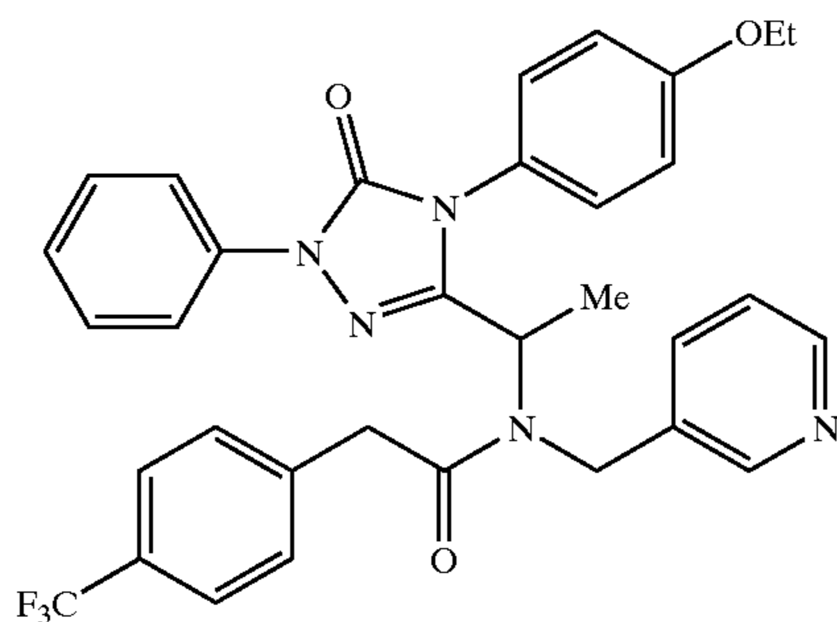
N -{1-[4-(4-Ethoxy-phenyl)-5-oxo-1-phenyl-4,5-dihydro-1 H -[1,2,4]triazol-3-yl]-ethyl}- N -pyridin-3-ylmethyl-2-(4-trifluoromethyl-phenyl)-acetamide
