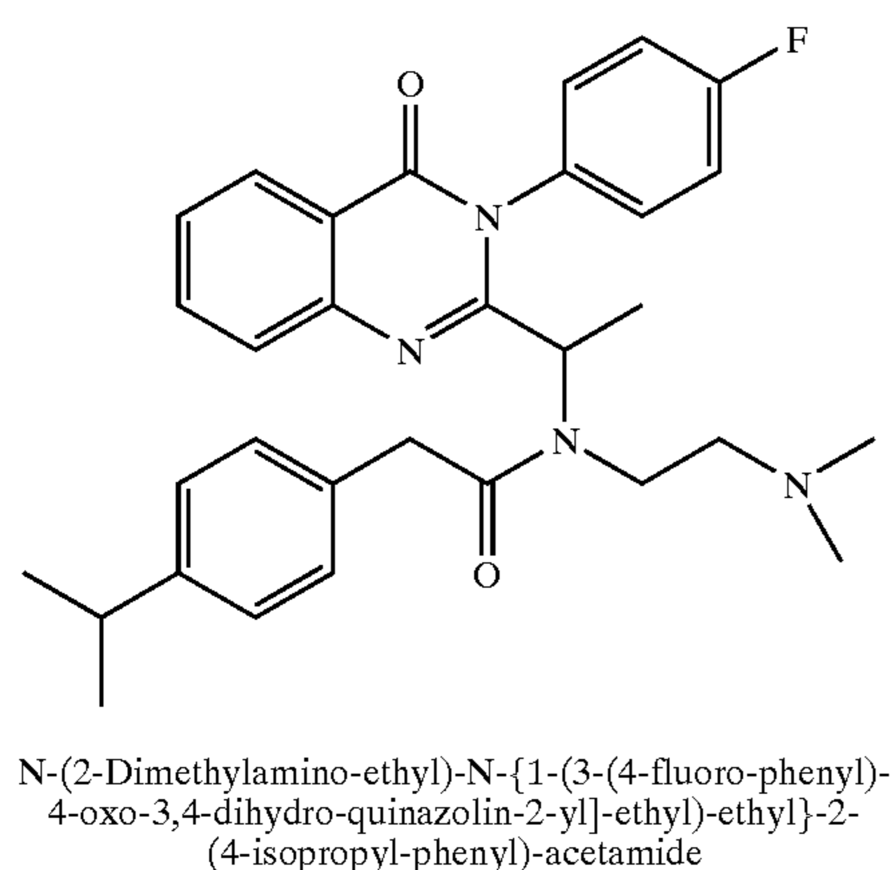
Synthesis of Compound 1.37
