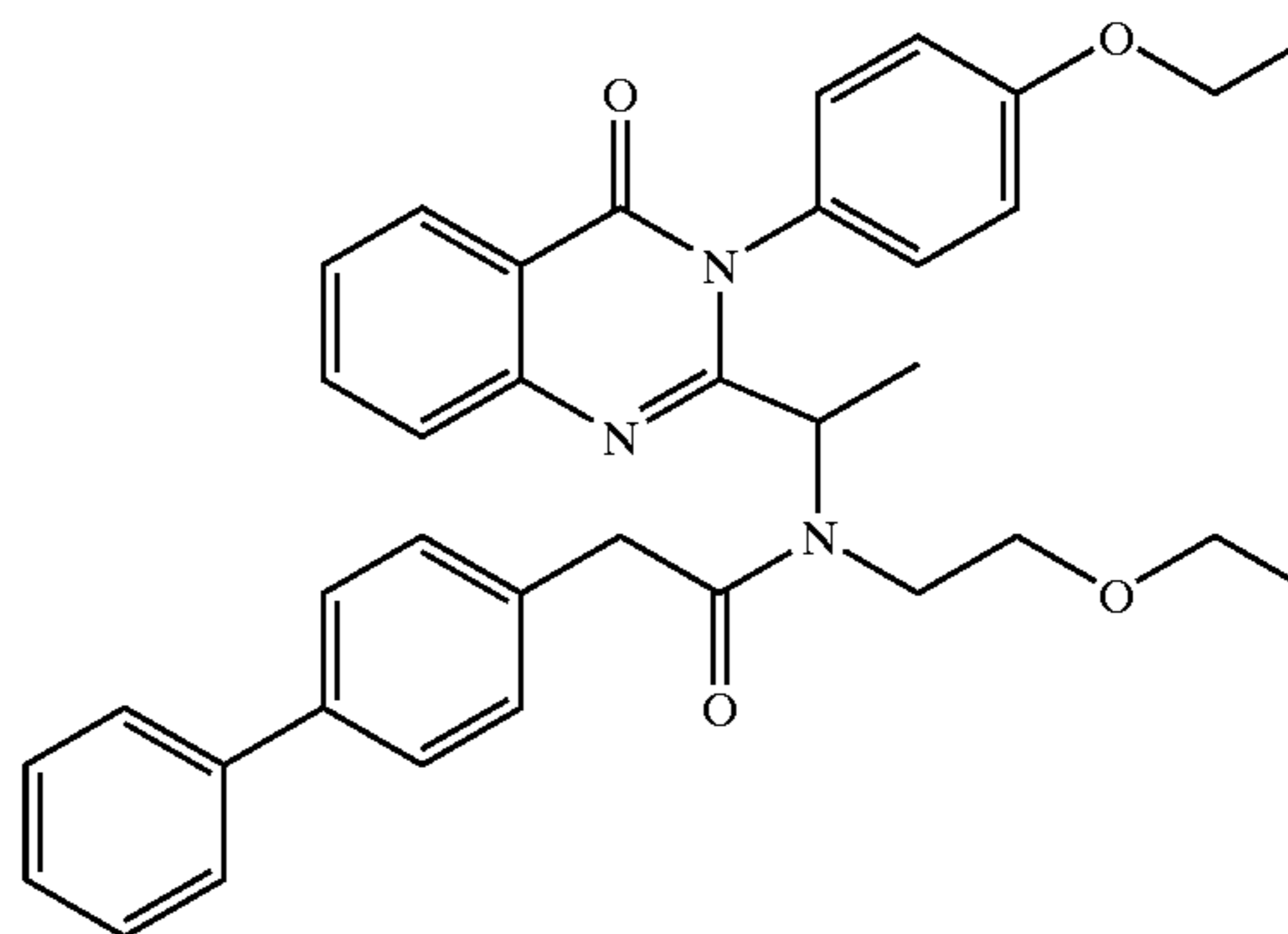
2-Biphenyl-4-yl-N-(2-ethoxy-ethyl)-N-{1-[3-(4-ethoxy-phenyl)-4-oxo-3,4-dihydro-quinazolin-2-yl]-ethyl}-acetamide
