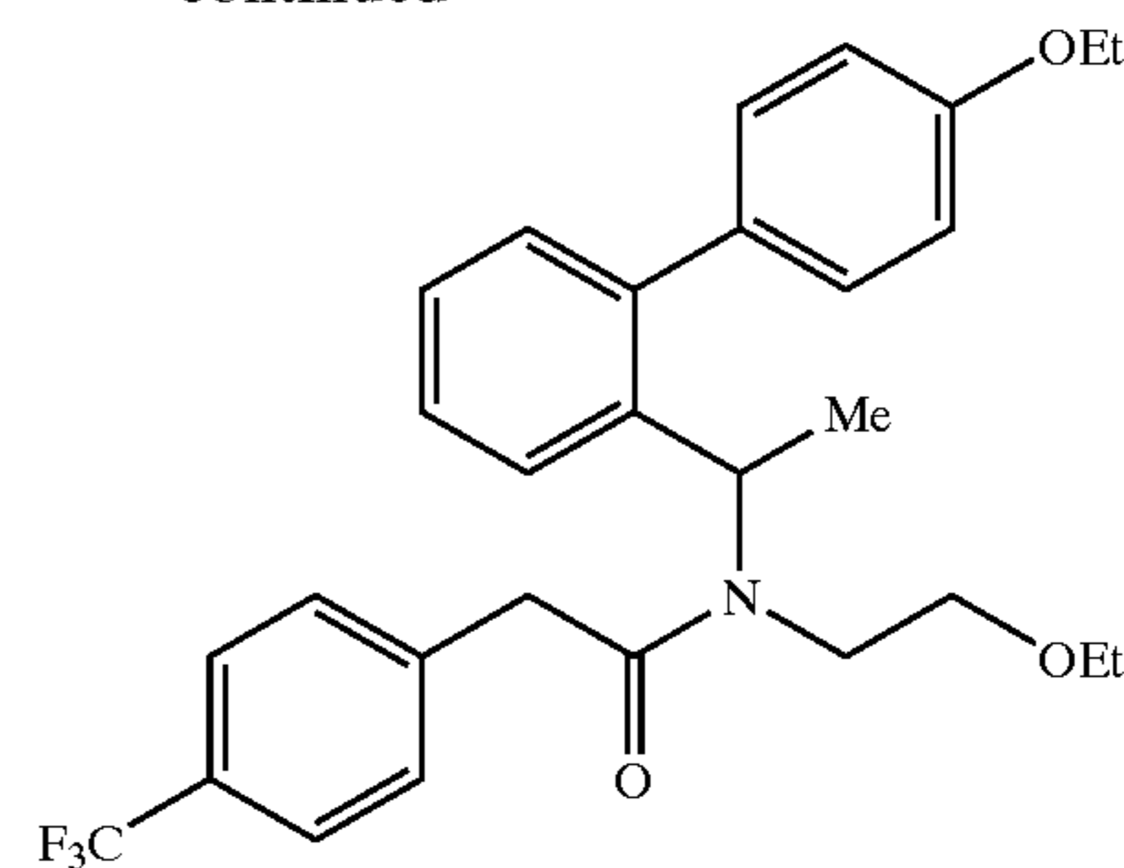
N-[1-(4'-Ethoxy-biphenyl-2-yl)-ethyl]-N-(2-ethoxy-ethyl)-2-(4-trifluoromethyl-phenyl)-acetamide
