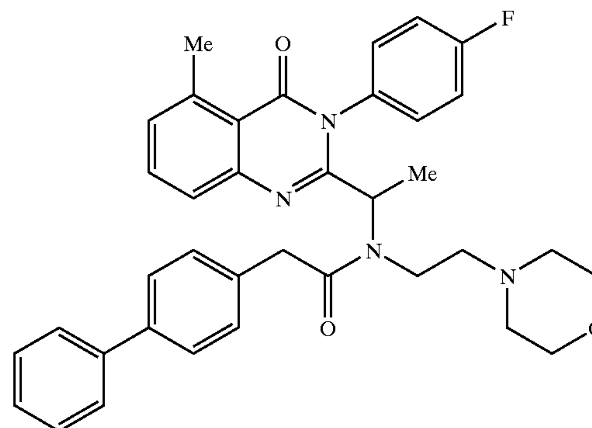
2-Biphenyl-4-yl-N-{1-[3-(4-fluoro-phenyl)-5-methyl-4-oxo-3,4-dihydro-quinazolin-2-yl]-ethyl}-N-(2-morpholin-4-yl-ethyl)-acetamide (2.01)
