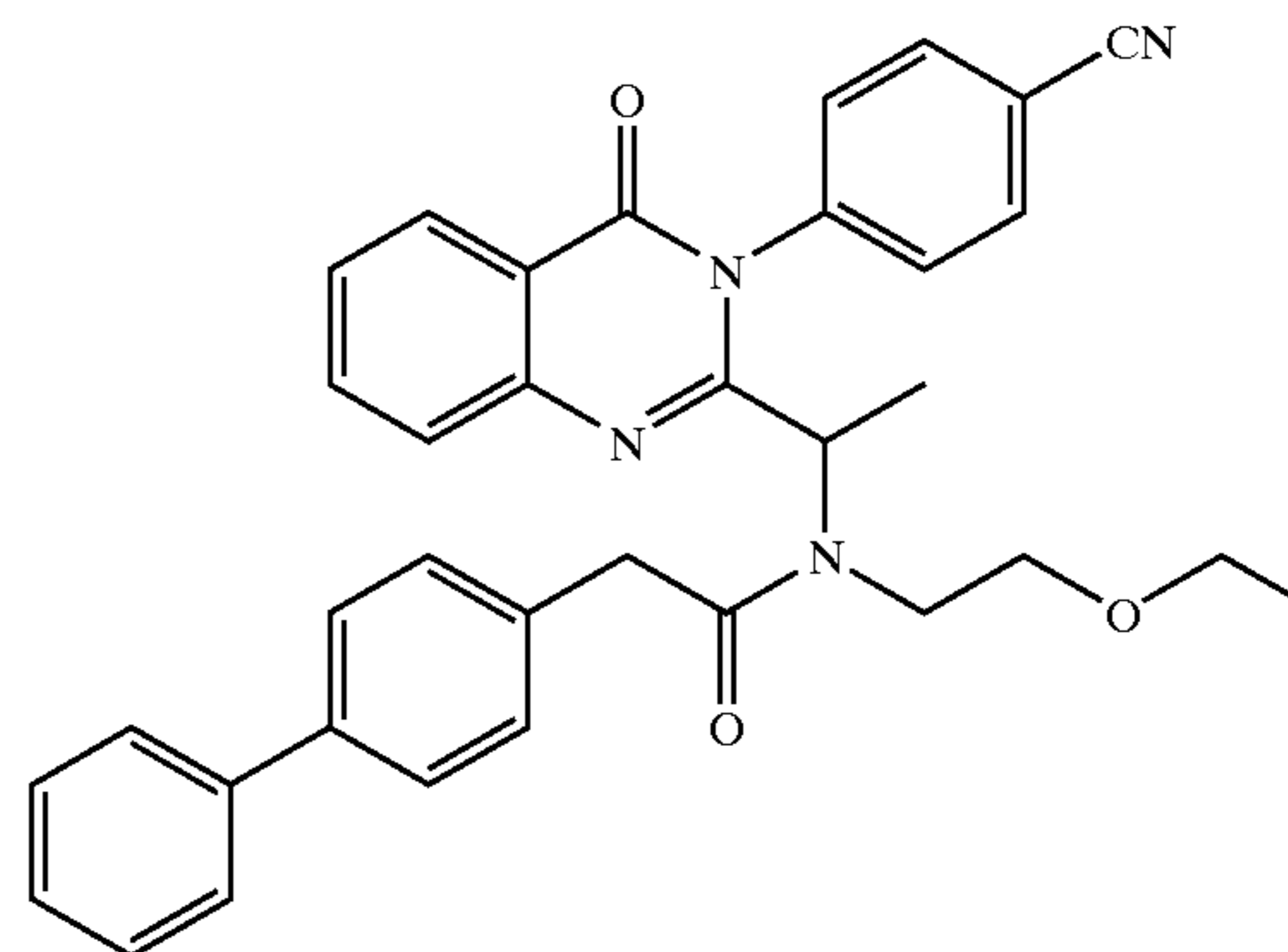
2-Biphenyl-4-yl-N-{1-[3-(4-cyano-phenyl)-4-oxo-3,4-dihydro-quinazolin-2-yl]-ethyl}-N-(2-ethoxy-ethyl)-acetamide
