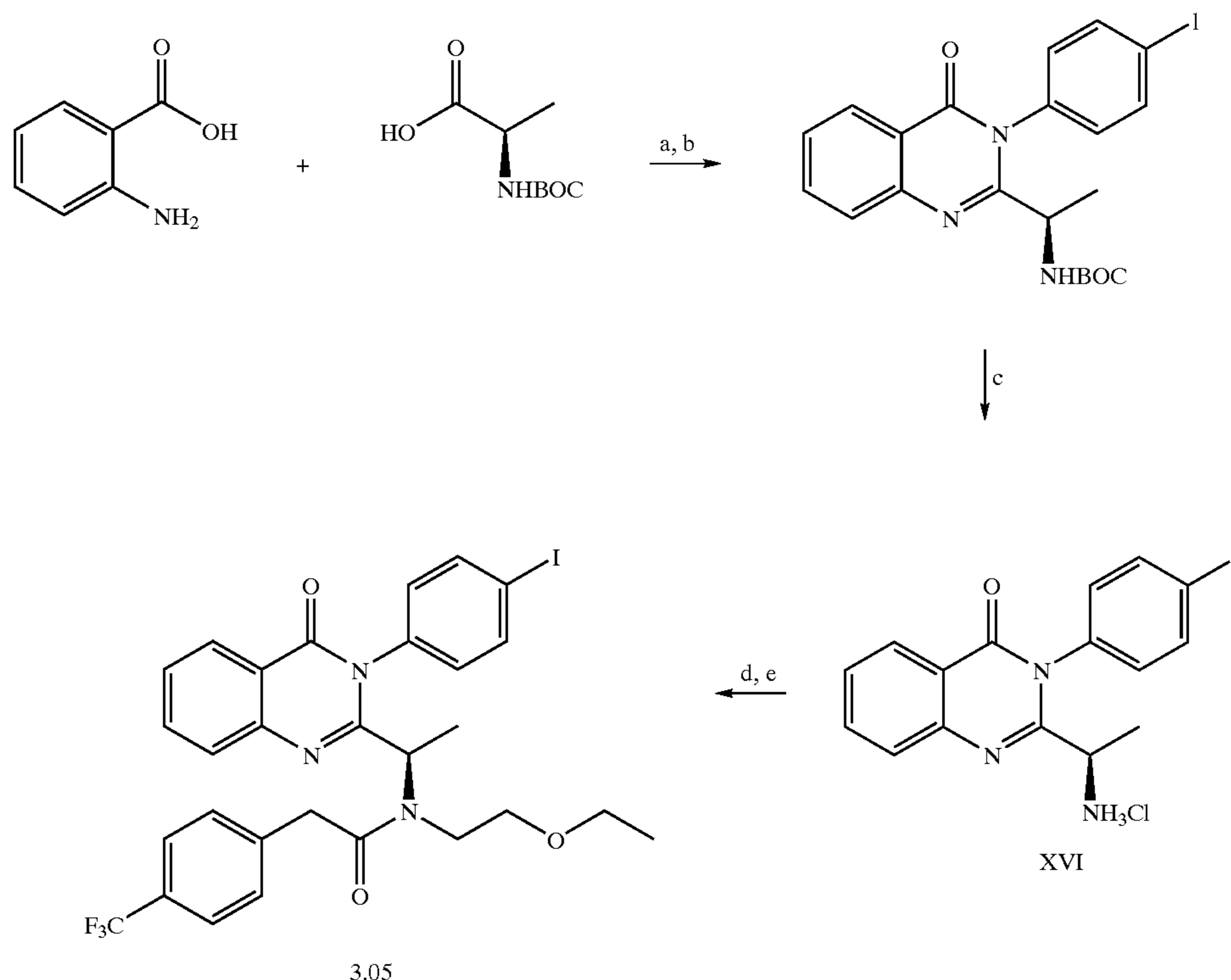
Scheme 5
