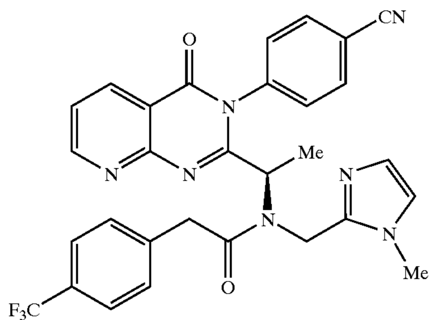
{1R-[3-(4-Cyano-phenyl)-4-oxo-3,4-dihydro-pyrido[2,3-d]rimidin-2-yl]-ethyl}-N-(1-methyl-1H-imidazol-2-ylmethyl)-2-(4-trifluoromethyl-phenyl)-acetamide (3.21)
