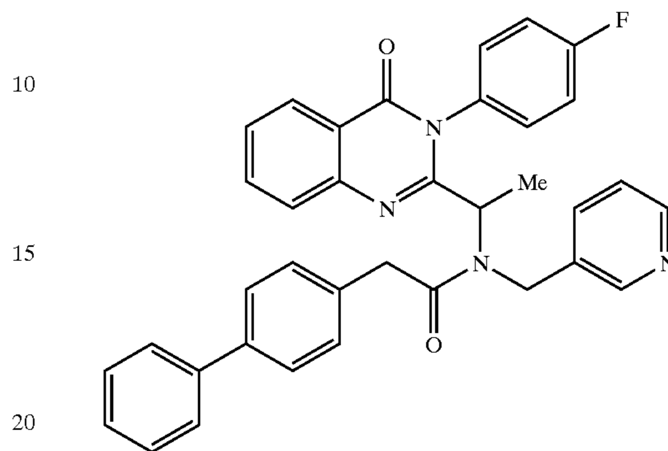
2-Biphenyl-4-yl-N-(1-[3-[(4-fluoro-phenyl)-4-oxo-3,4-dihydro-quinazolin-2-yl]-ethyl]-ethyl)-N-pyridin-3-ylmethylacetamide
