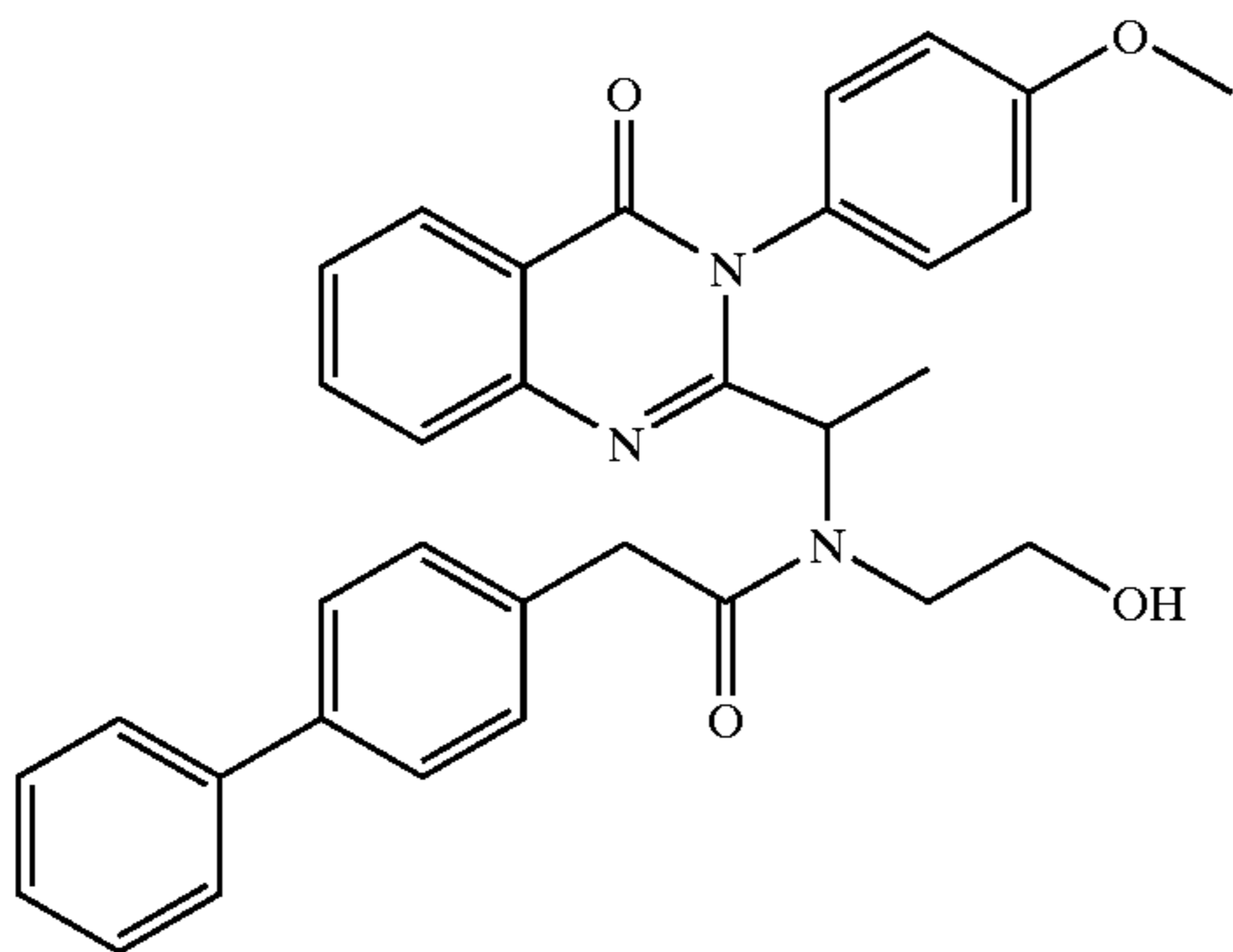
2-Biphenyl-4-yl-N-(2-hydroxy-ethyl)-N-{1-[3-(4-methoxy-phenyl)-4-oxo-3,4-dihydro-quinazolin-2-yl]-ethyl}-acetamide
