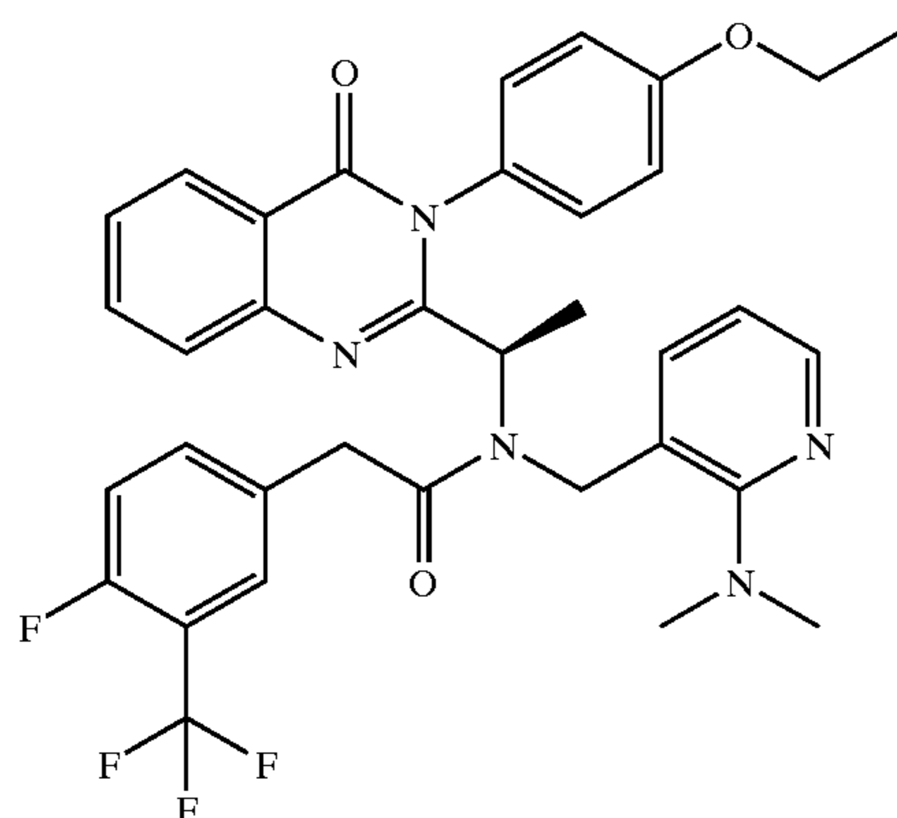
N -(2-Dimethylamino-pyridin-3-ylmethyl)- N -{1-[3-(4-ethoxy-phenyl)-4-oxo-3,4-dihydro-quinazolin-2-yl]-ethyl}-2-(4-fluoro-3-trifluoromethyl-phenyl)-acetamide
