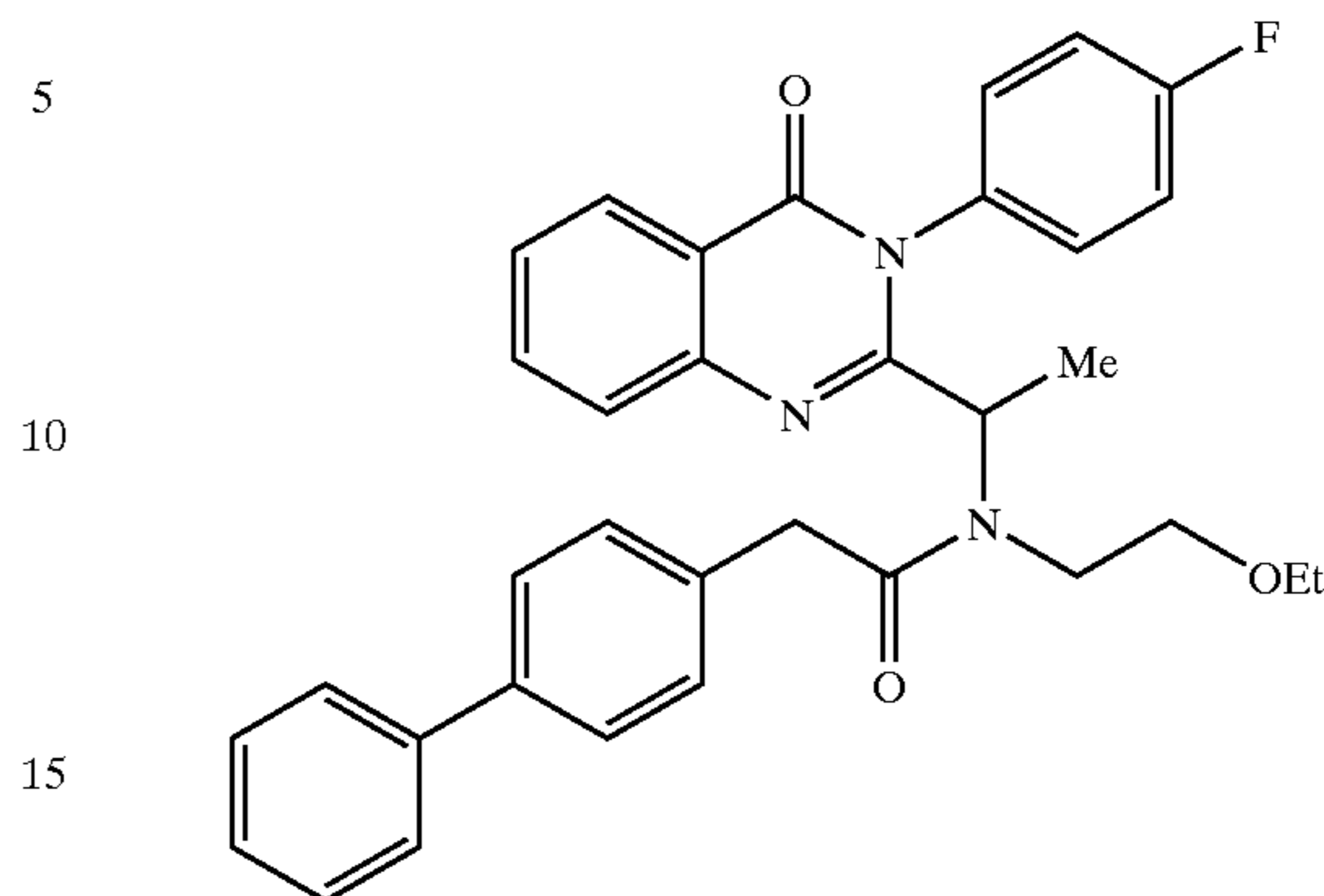
2-Biphenyl-4-yl-N-(1-[3-(4-fluoro-phenyl)-4-oxo-3,4-dihydro-quinazolin-2-yl]-ethyl)-acetamide
