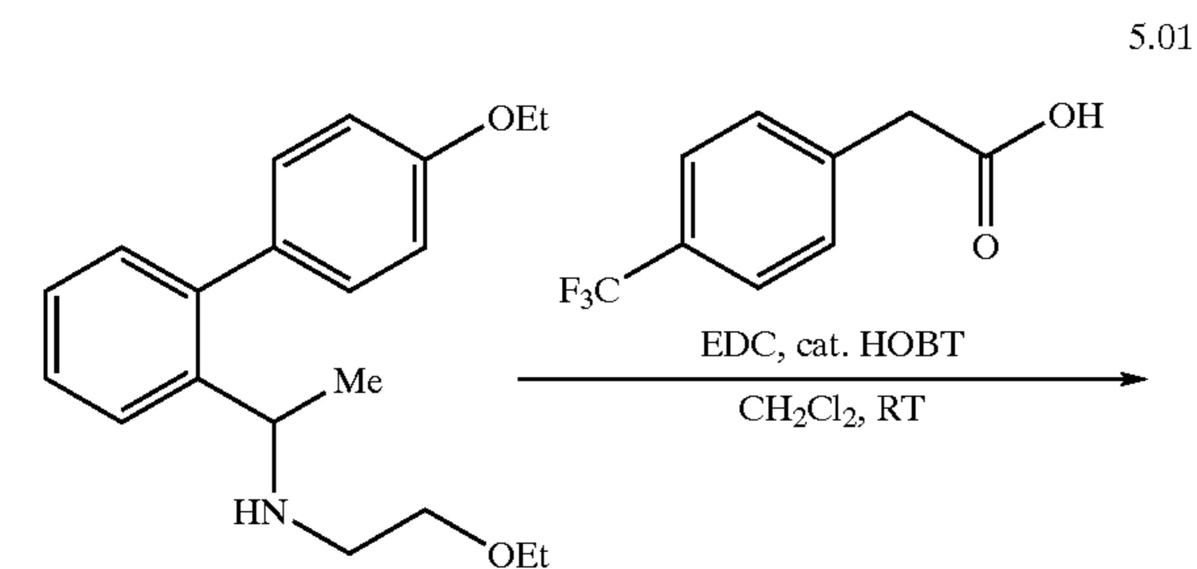
[1-(4'-Ethoxy-biphenyl-2-yl)-ethyl]-(2-ethoxy-ethyl)-amine
