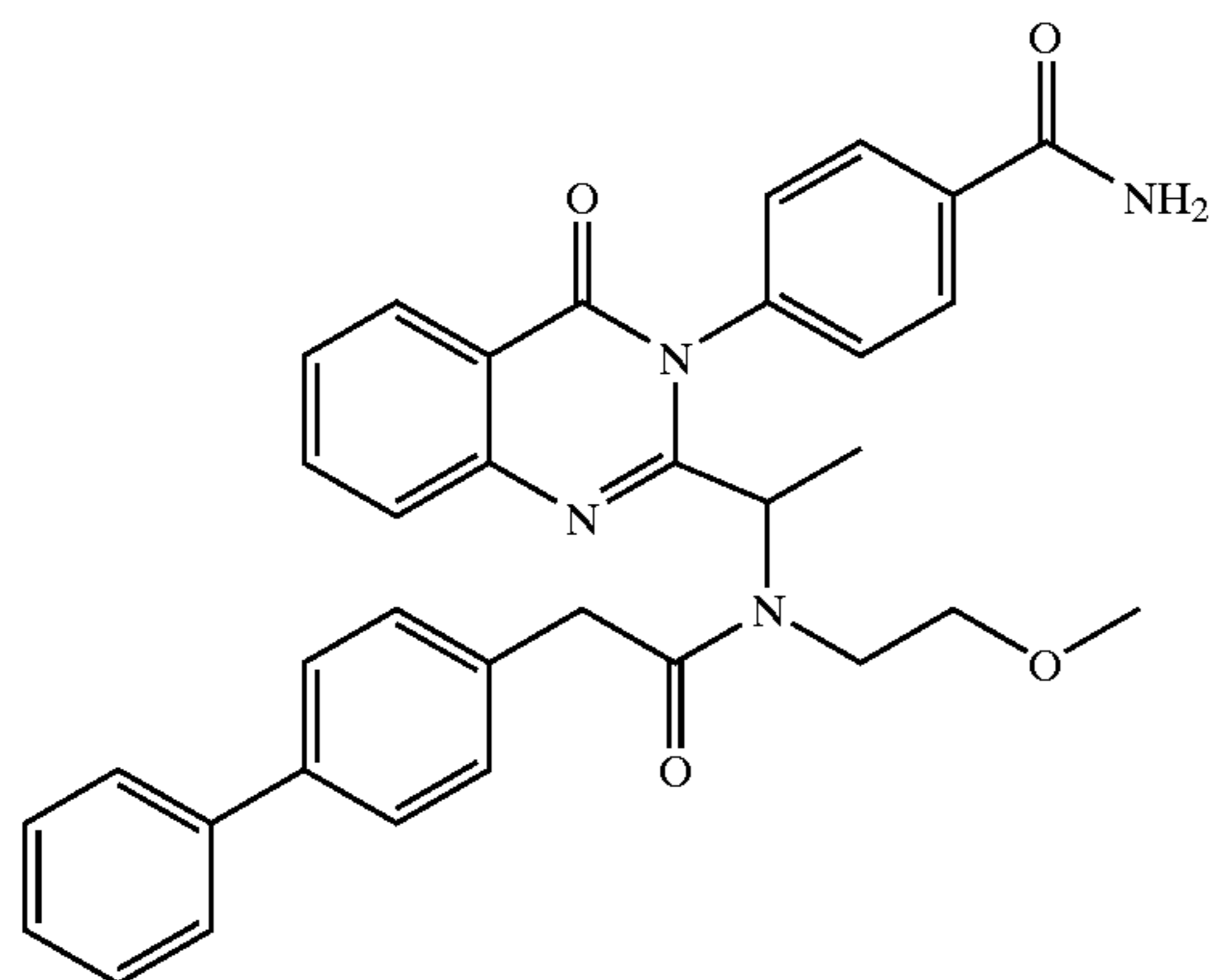
4-(2-{1-[(Biphenyl-4-yl-acetyl)-(2-methoxy-ethyl)-amino]-ethyl}-4-oxo-4H-quinazolin-3-yl)-benzamide
