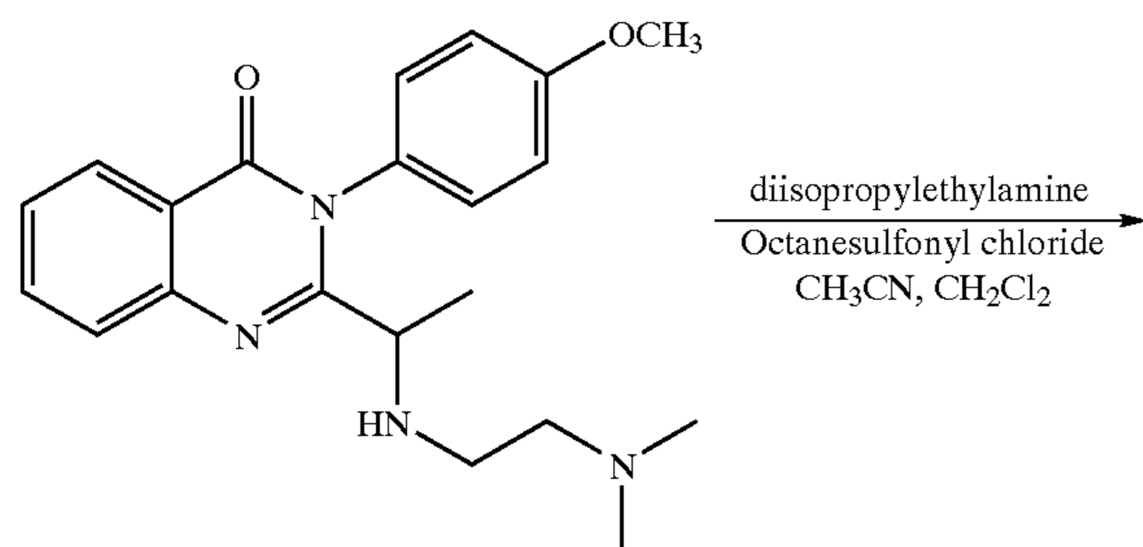
2-[1-(2-Dimethylamino-ethylamino)-ethyl]-3-(4-methoxy-phenyl)-3H-quinazolin-4-one
