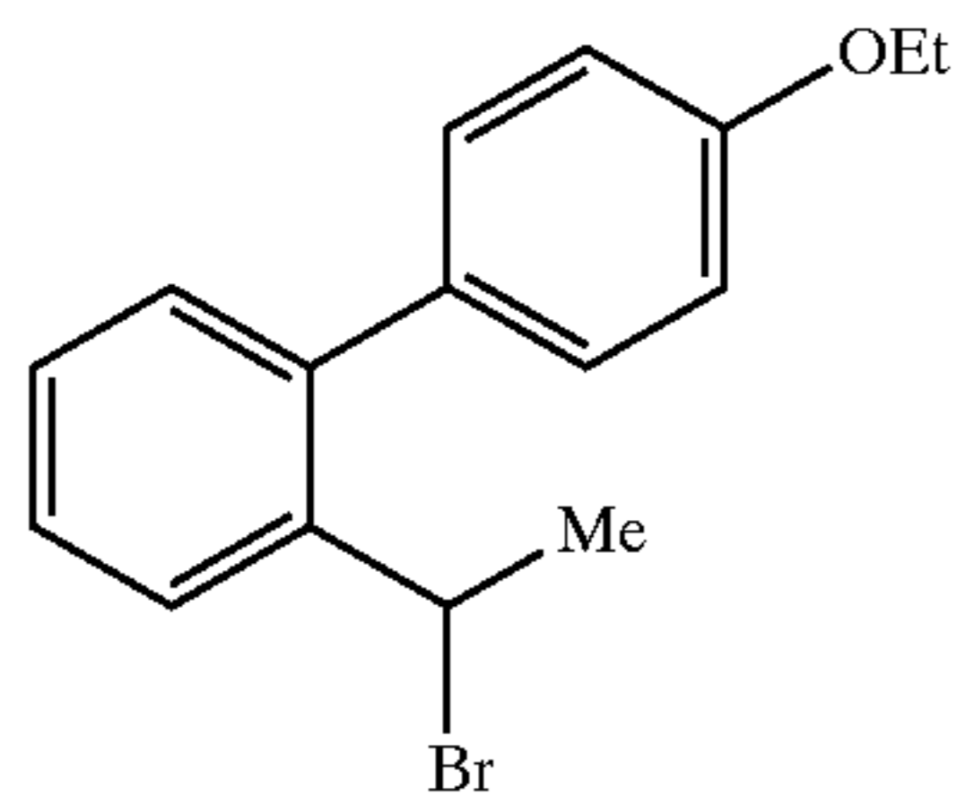
2-(1-Bromo-ethyl)-4'-ethoxy-biphenyl
