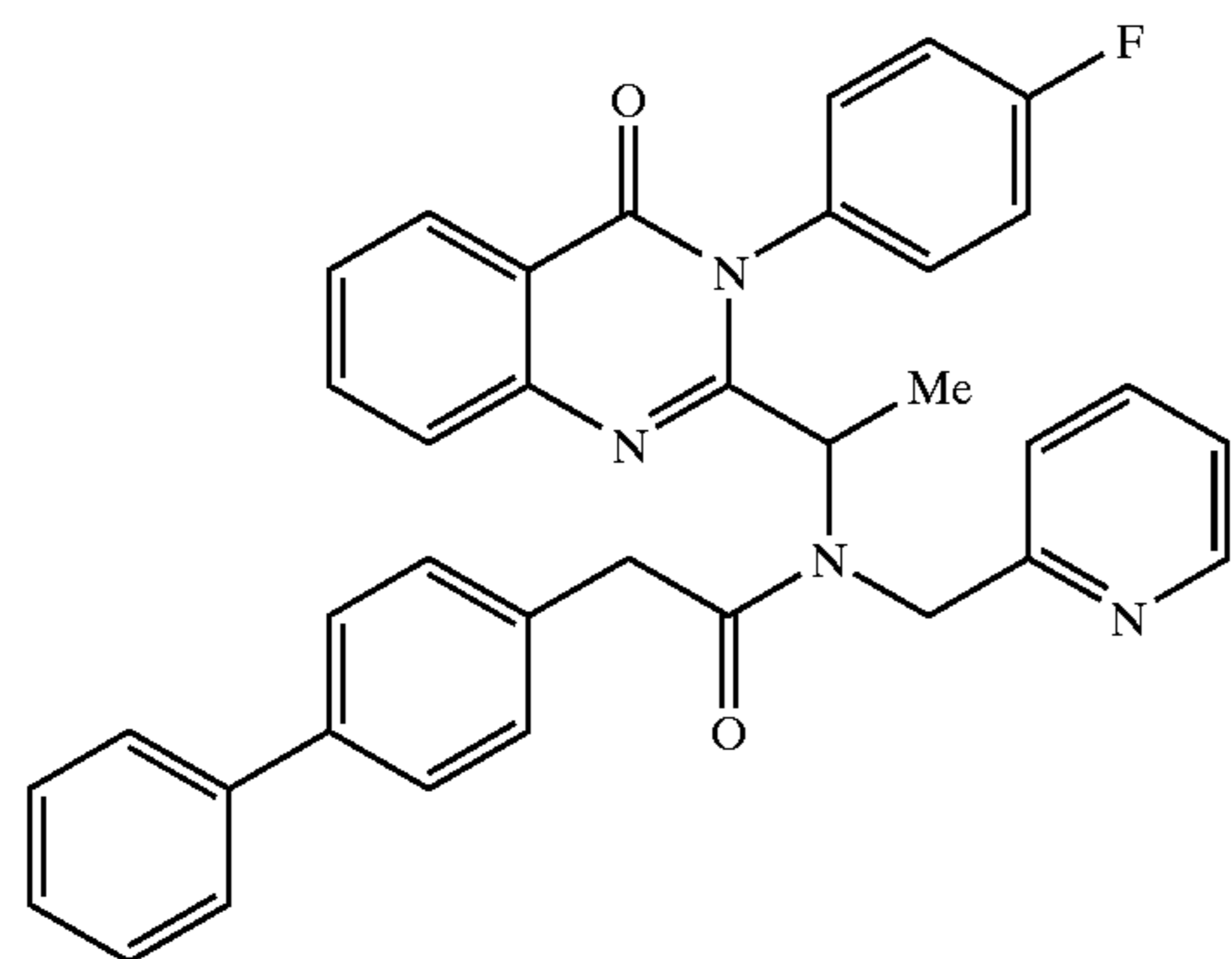
2-Biphenyl-4-yl-N-(1-[3-[(4-fluoro-phenyl)-4-oxo-3,4-dihydro-quinazolin-2-yl]-ethyl]-ethyl)-N-pyridin-2-ylmethylacetamide
