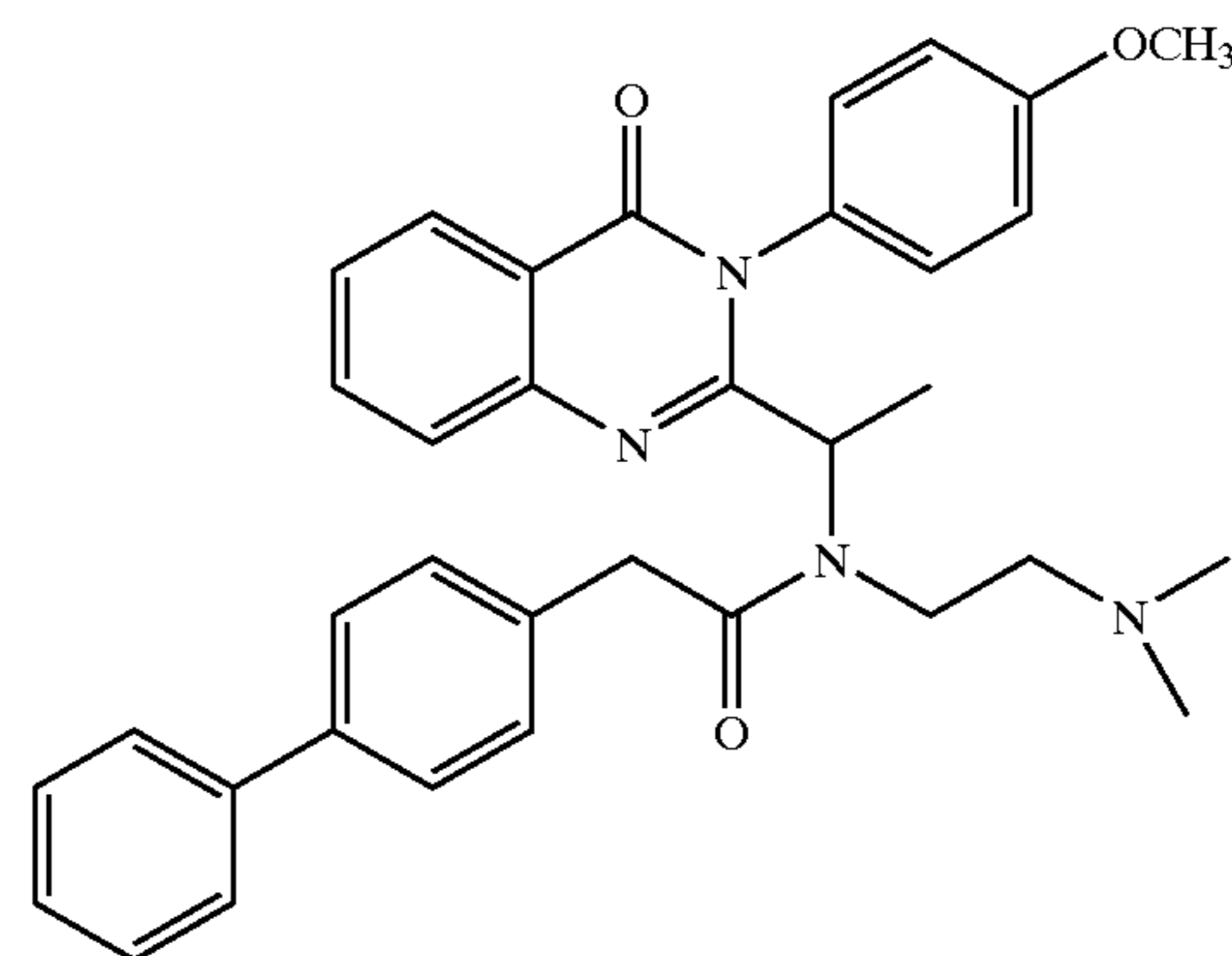
2-Biphenyl-4-yl-N-(2-dimethylamino-ethyl)-N-{1-[3-(4-methoxy-phenyl)-4-oxo-3,4-dihydro-quinazolin-2-yl]-ethyl}-acetamide
