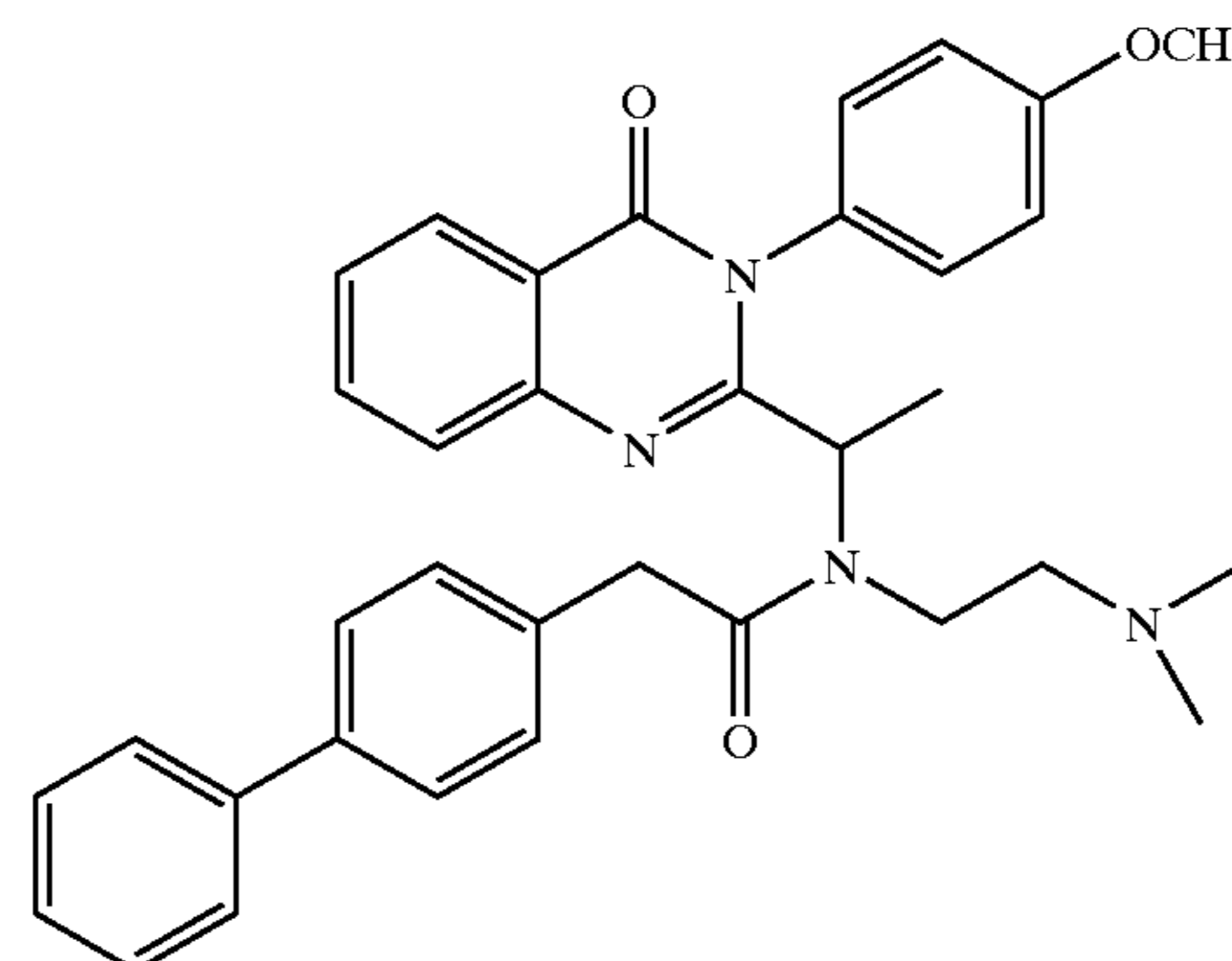
2-Biphenyl-4-yl-N-(2-dimethylamino-ethyl)-N-{1-[3-(4-methoxy-phenyl)-4-oxo-3,4-dihydro-quinazolin-2-yl]-ethyl}-acetamide
