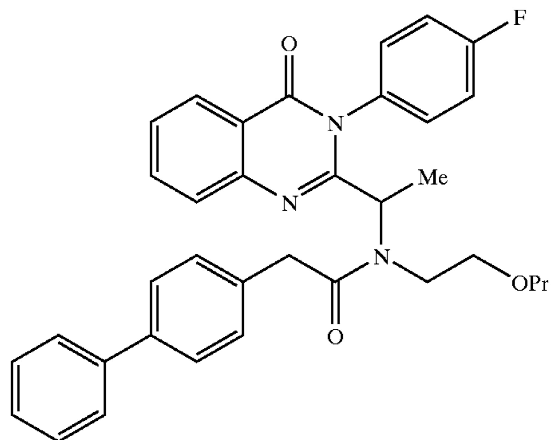
2-Biphenyl-4-yl-N-(1-[3-[(4-fluoro-phenyl)-4-oxo-3,4-dihydro-quinazolin-2-yl]-ethyl]-ethyl)-N-(2-isopropoxyethyl)-acetamide
