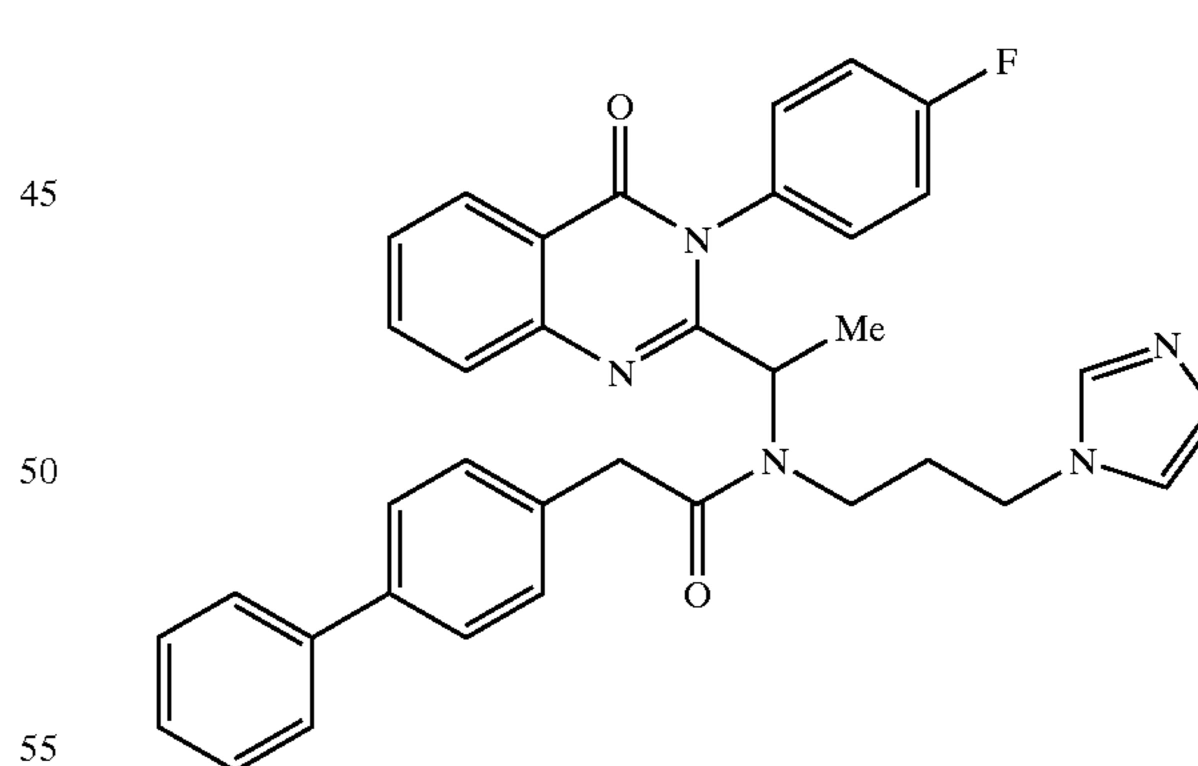
2-Biphenyl-4-yl-N-(1-[3-[(4-fluoro-phenyl)-4-oxo-3,4-dihydro-quinazolin-2-yl]-ethyl]-ethyl)-N-(3-imidazol-1-ylpropyl)acetamide
