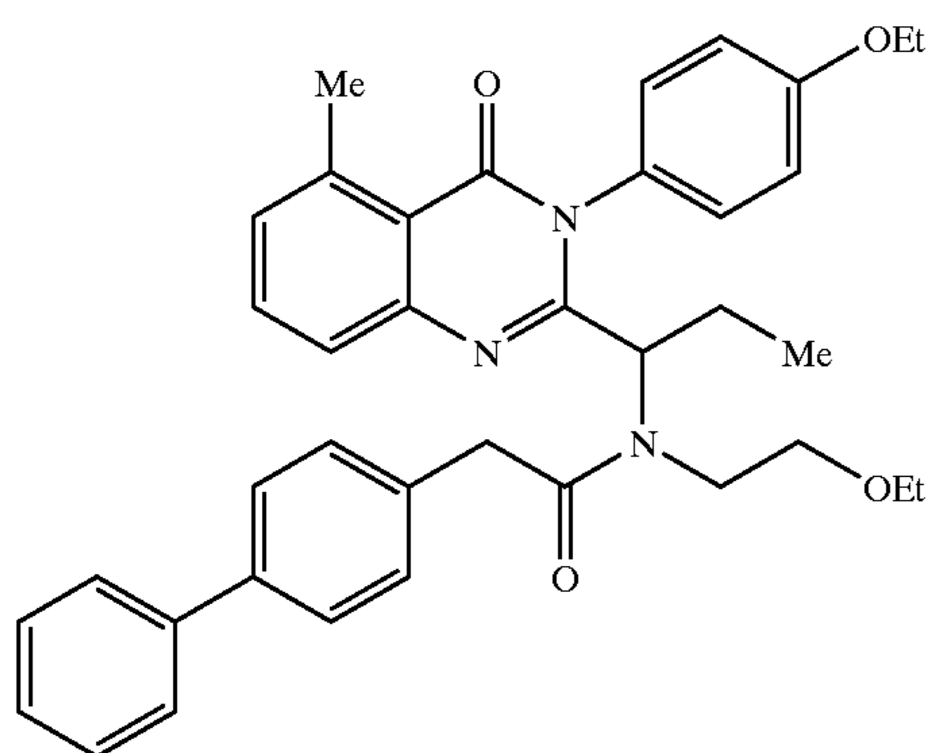
2-Biphenyl-4-yl-N-(2-ethoxy-ethyl)-N-{1-[3-(4-ethoxy-phenyl)-5-methyl-4-oxo-3,4-dihydro-quinazolin-2-yl]-propyl}-acetamide
