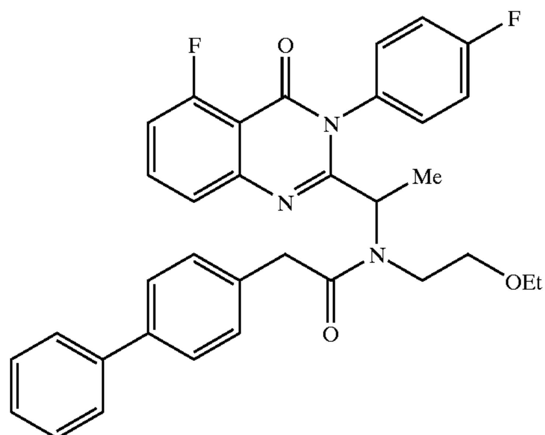
2-Biphenyl-4-yl-N-(2-ethoxy-ethyl)-N-{1-[5-fluoro-3-(4-fluoro-phenyl)-4-oxo-3,4-dihydro-quinazolin-2-yl]-ethyl}-acetamide
