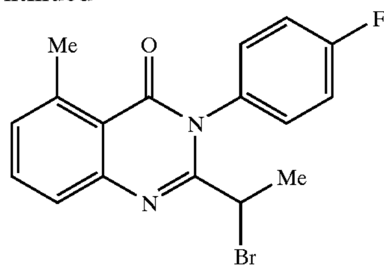
2-(1-Bromo-ethyl)-3-(4-fluoro-phenyl)-5-methyl-3H-quinazolin-4-one (X)
