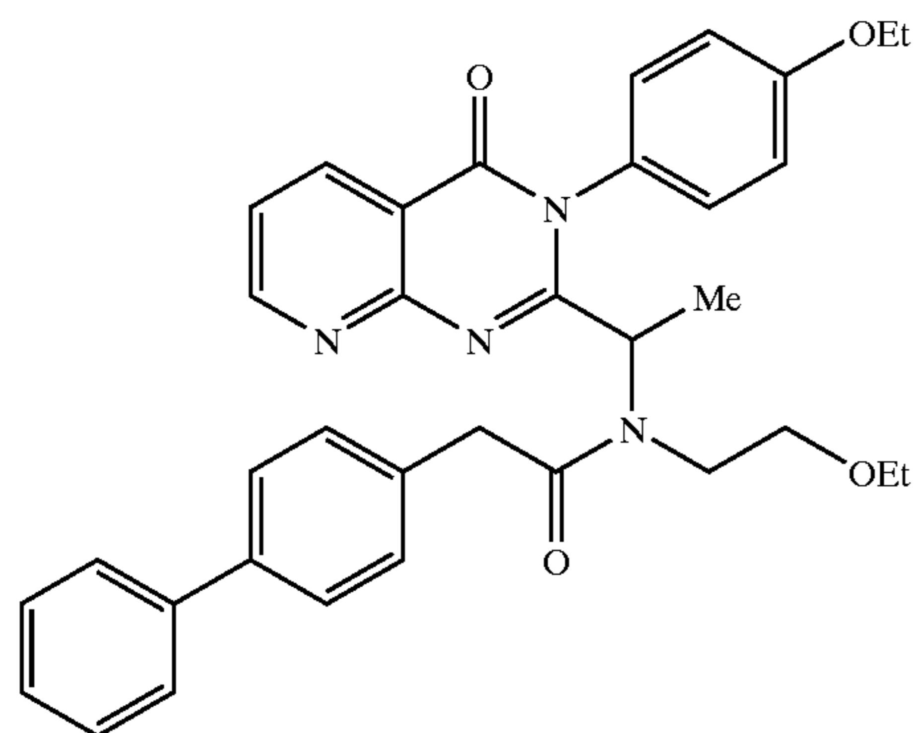
2-Biphenyl-4-yl-N-(2-ethoxy-ethyl)-N-{1-[3-(4-ethoxy-phenyl)-4-oxo-3,4-dihydro-pyrido[2,3-d]pyrimidin-2-yl]-ethyl}-acetamide
