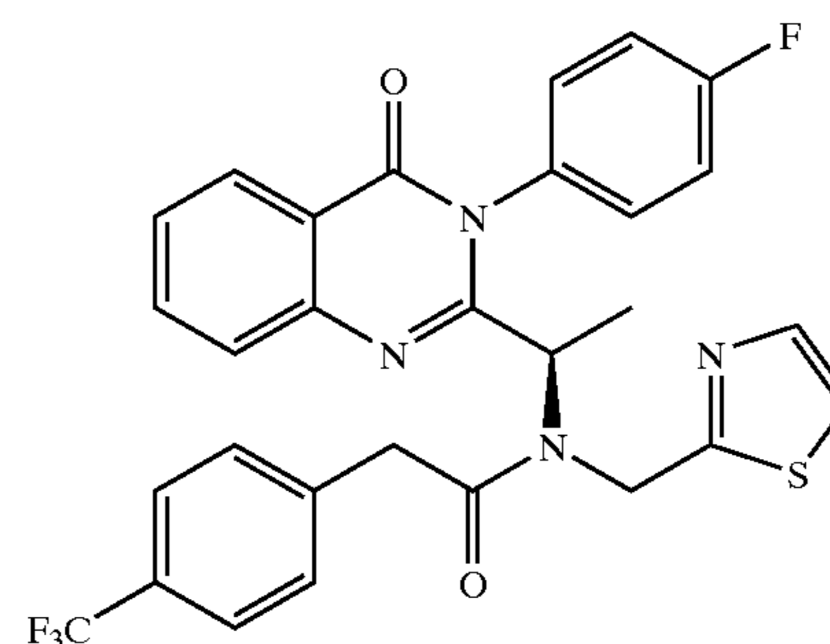
Synthesis of Compound 10.05
