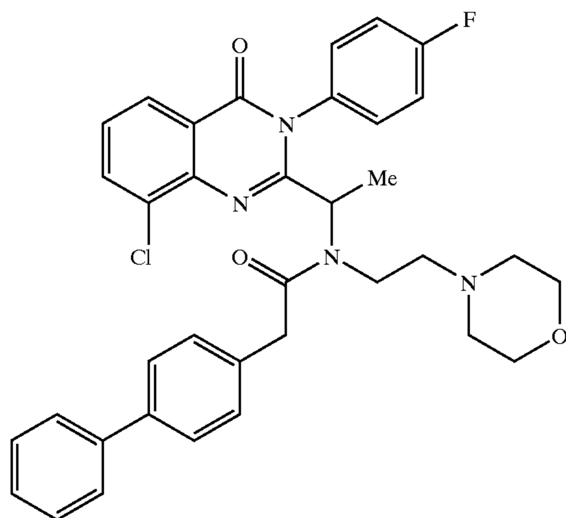
2-Biphenyl-4-yl-N-{1-[8-chloro-3-(4-fluoro-phenyl)-4-oxo-3,4-dihydro-quinazolin-2-yl]-ethyl}-N-(2-morpholin-4-yl-ethyl)-acetamide
