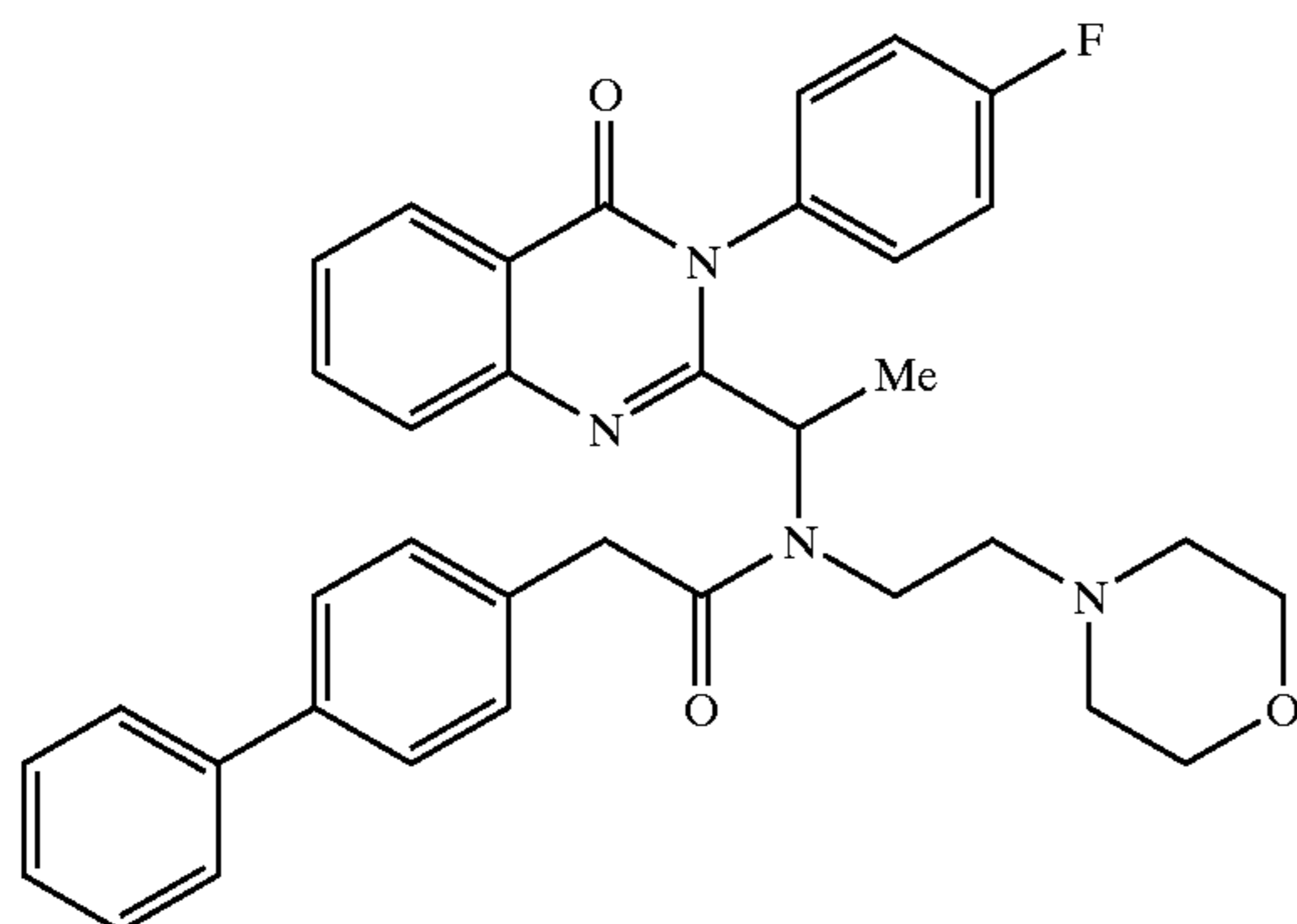
2-Biphenyl-4-yl-N-{1-[3-(4-fluoro-phenyl)-4-oxo-3,4-dihydro-quinazolin-2-yl]-ethyl}-N-(2-morpholin-4-yl-ethyl)-acetamide
