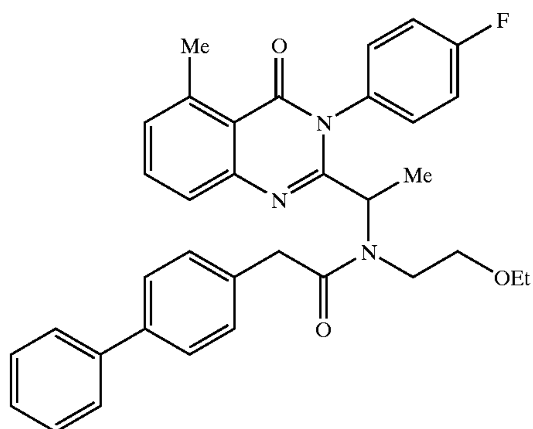
2-Biphenyl-4-yl-N-(2-ethoxy-ethyl)-N-{1-[5-methyl-3-(4-fluoro-phenyl)-4-oxo-3,4-dihydro-quinazolin-2-yl]-ethyl}-acetamide
