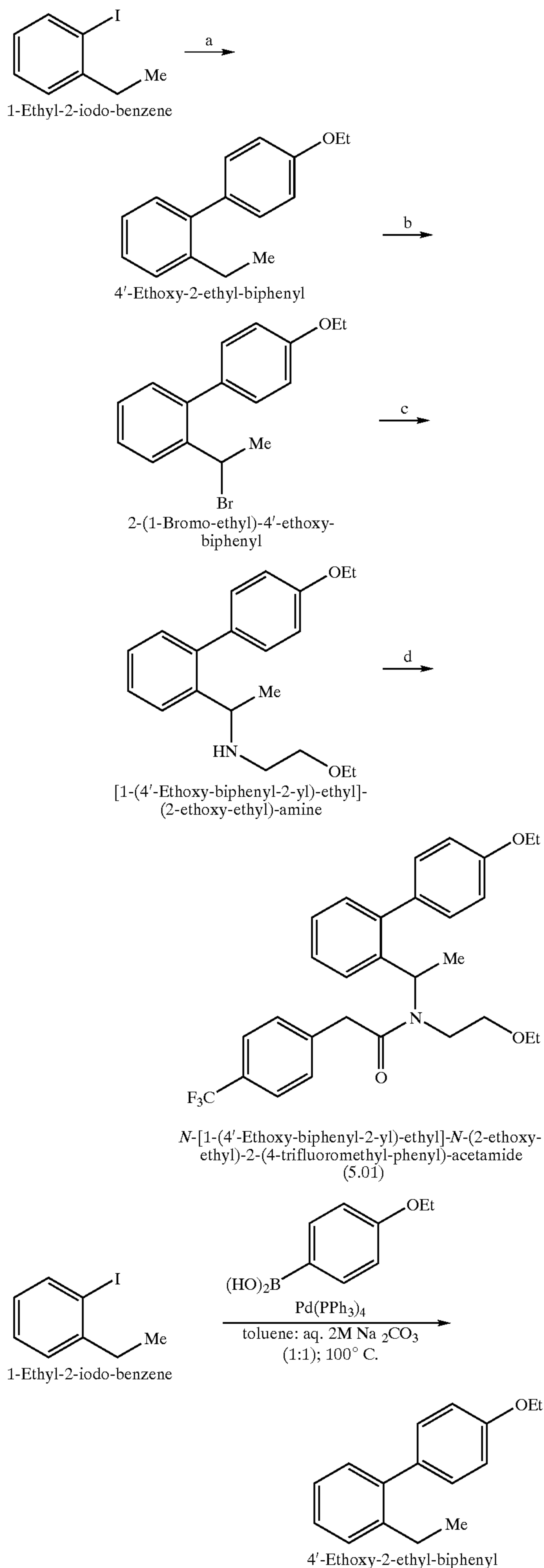
Scheme 13
