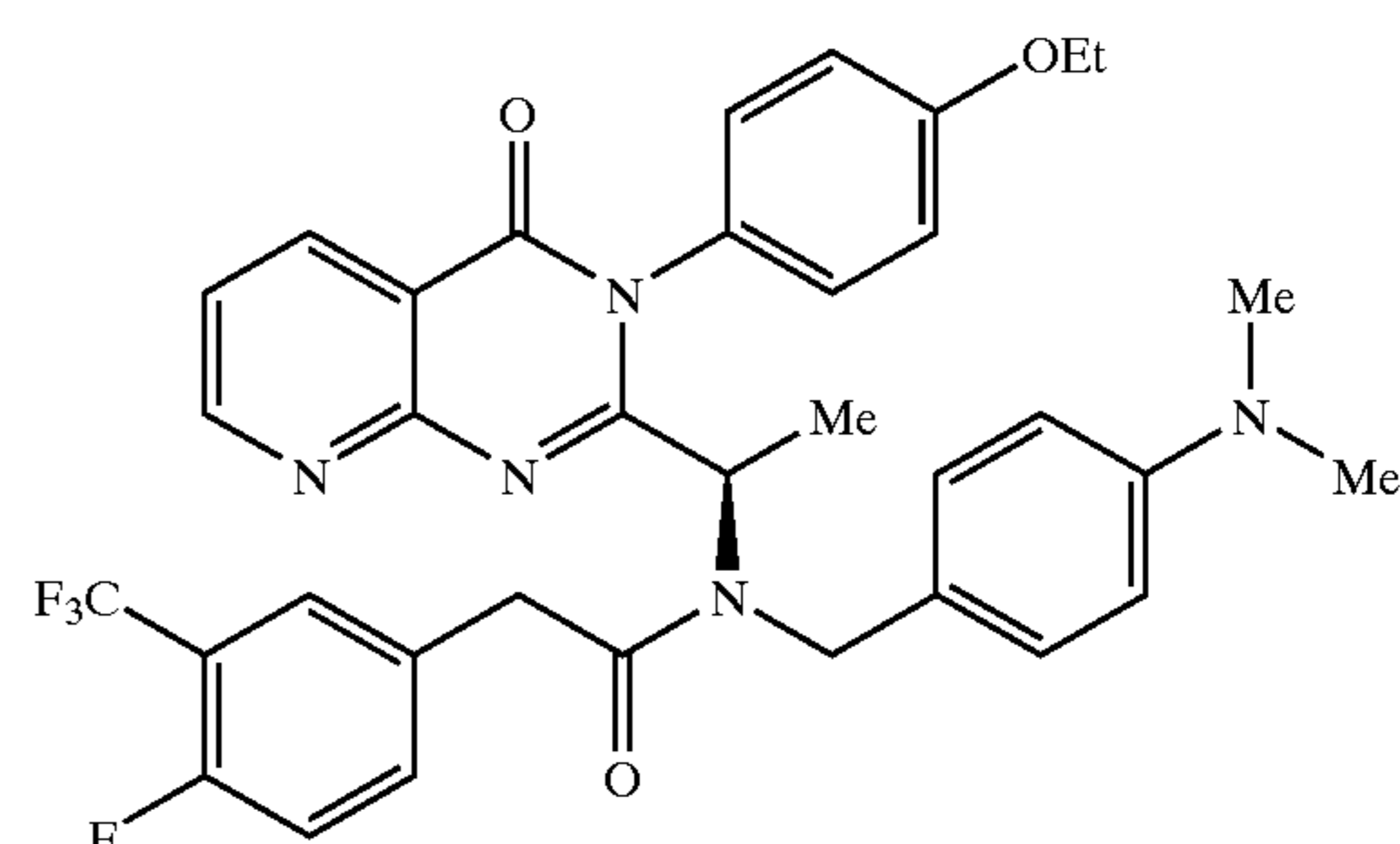
( R )- N -(4-Dimethylamino-benzyl)- N -[1-[3-(4-ethoxy-phenyl)-4-oxo-3,4-dihydro-pyrido[2,3- d ]pyrimidin-2-yl]-ethyl]-2-(4-fluoro-3-trifluoromethyl-phenyl)-acetamide
