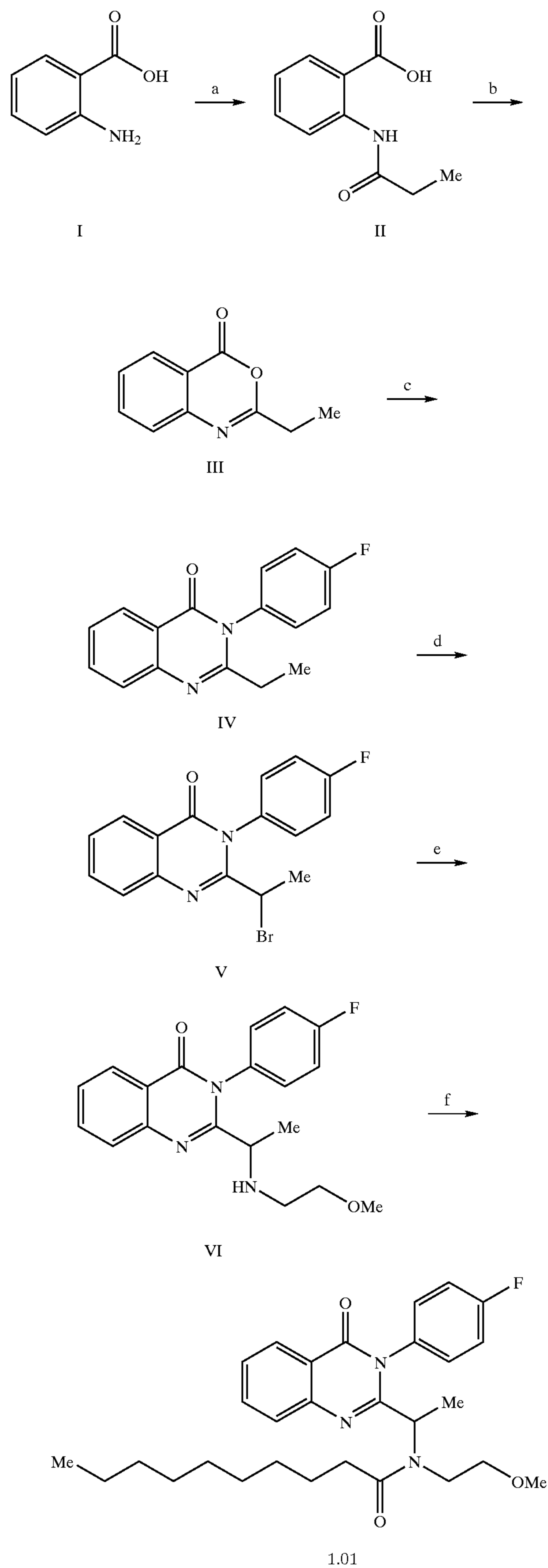
Scheme 1
