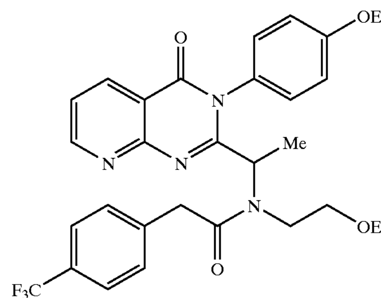
N-(2-Ethoxy-ethyl)-N-{1-[3-(4-ethoxy-phenyl)-4-oxo-3,4-dihydro-pyrido[2,3-d]pyrimidin-2-yl]-ethyl}-2-(4-trifluoromethyl-phenyl)-acetamide
