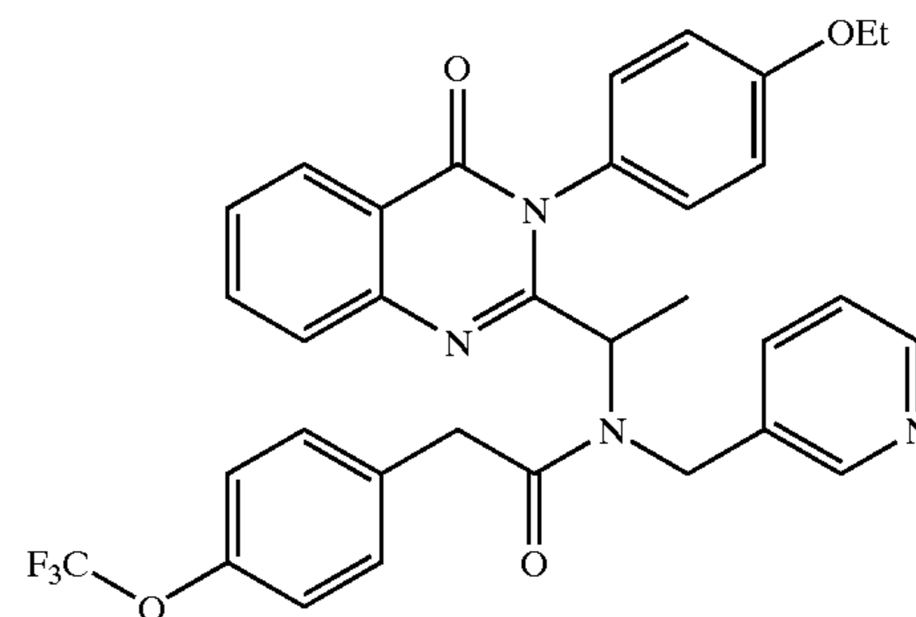
N -{1-[3-(4-Ethoxy-phenyl)-4-oxo-3,4-dihydro-quinazolin-2-yl]-ethyl}- N -pyridin-3-ylmethyl-2-(4-trifluoromethoxy-phenyl)-acetamide
