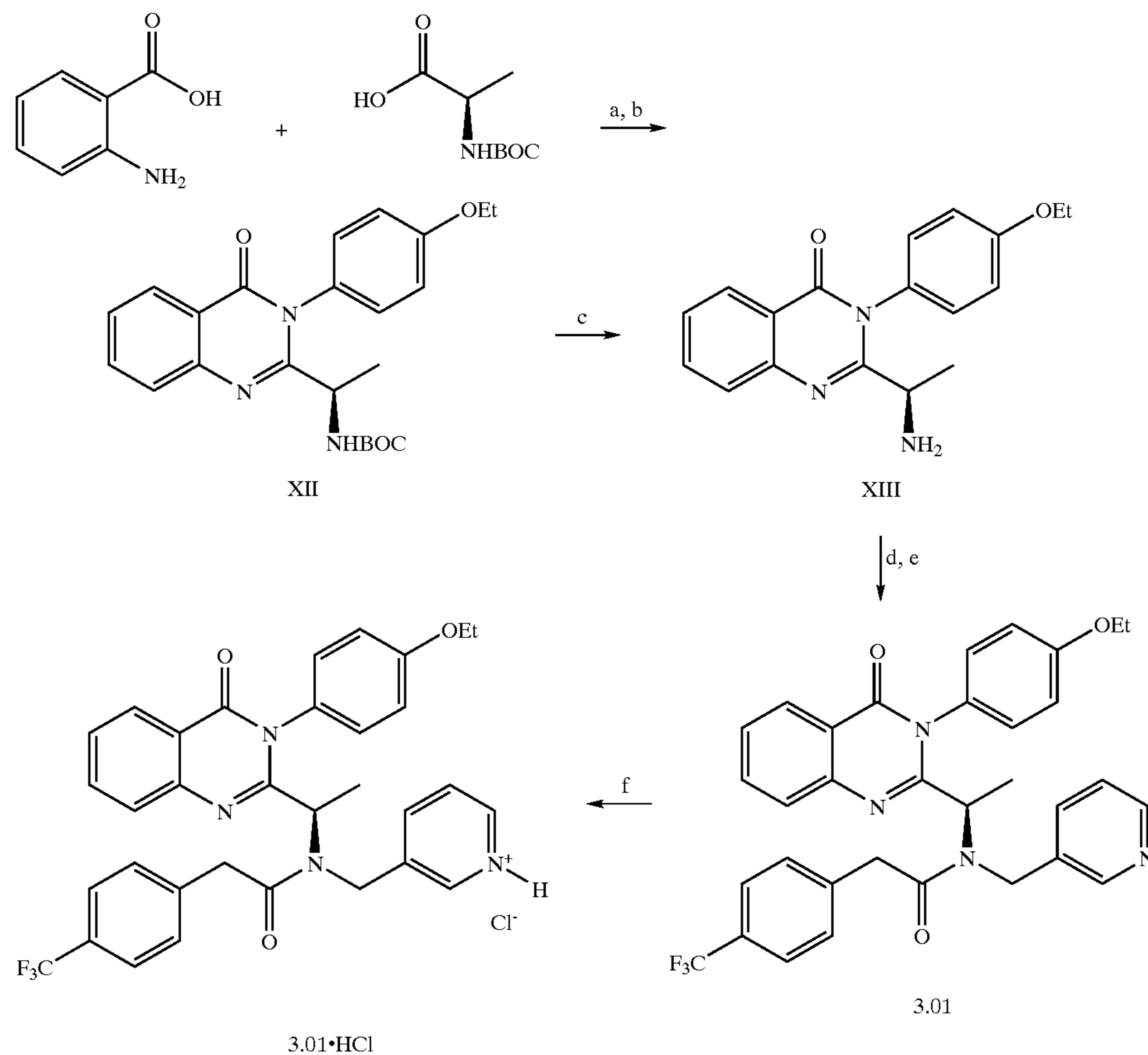
Scheme 3
