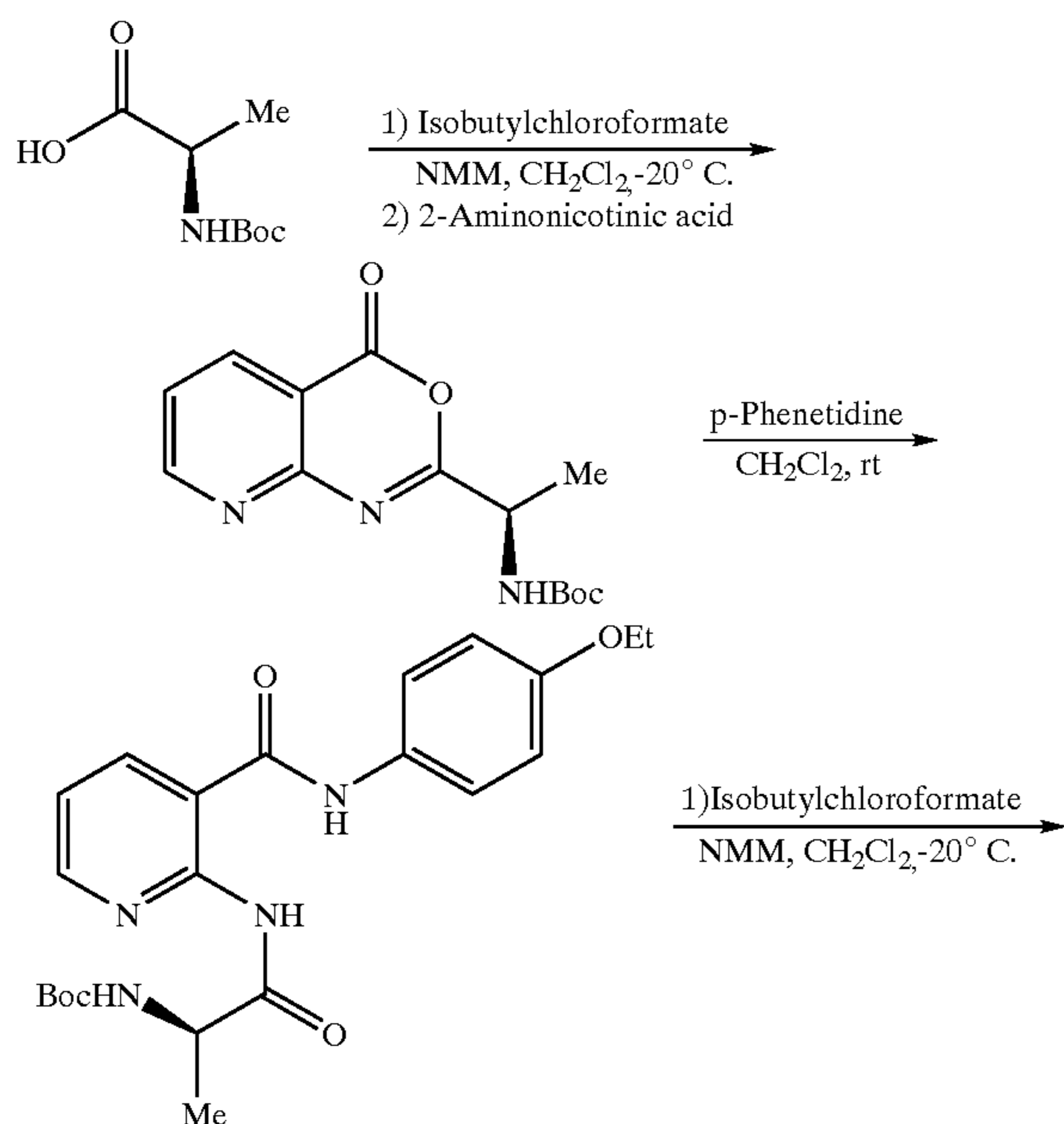
Scheme 9
