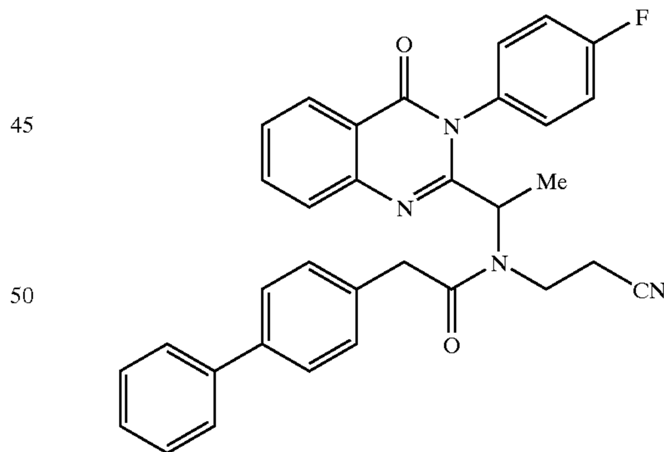
2-Biphenyl-4-yl-N-(2-cyano-ethyl)-N-(1-[3-(4-fluoro-phenyl)-4-oxo-3,4-dihydro-quinazolin-2-yl]-ethyl)-acetamide
