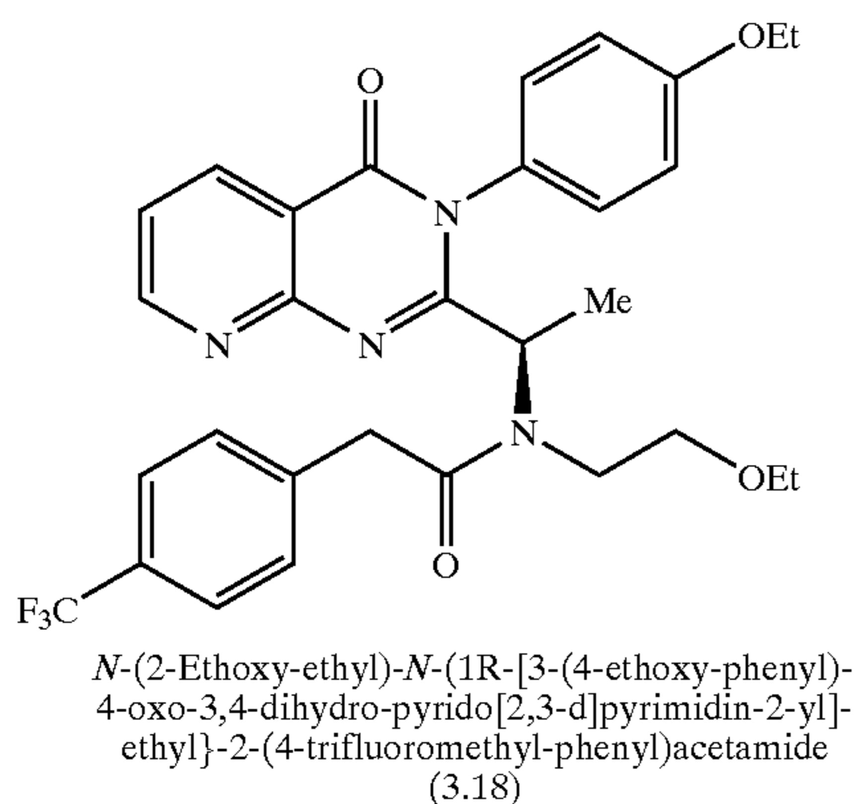
Synthesis of Compound 3.18
