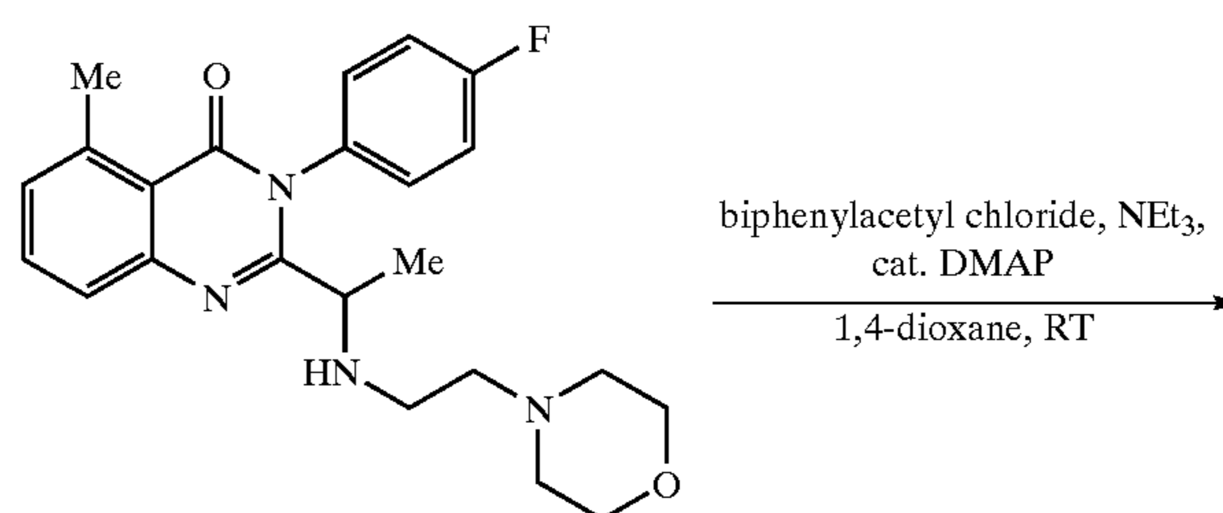
3-(4-Fluoro-phenyl)-5-methyl-2-[1-(2-morpholin-4-yl-ethylamino)-ethyl]-3H-quinazolin-4-one (XI)
