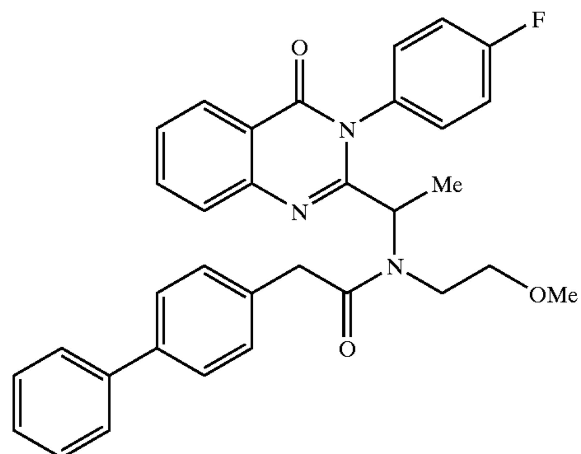
2-Biphenyl-4-yl-N-{1-[3-(4-fluoro-phenyl)-4-oxo-3,4-dihydro-quinazolin-2-yl]-ethyl}-N-(2-methoxy-ethyl)-acetamide
