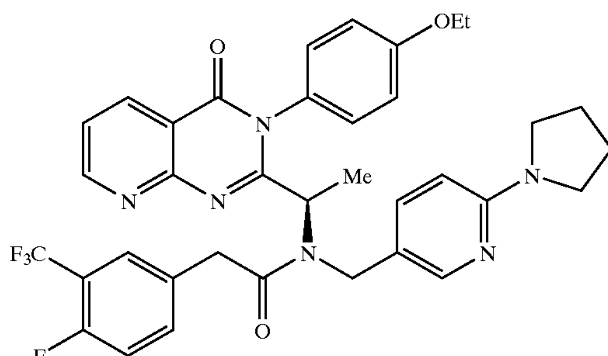
( R )- N -(1-[3-(4-Ethoxy-phenyl)-4-oxo-3,4-dihydro-pyrido[2,3- d ]pyrimidin-2-yl]-ethyl)-2-(4-fluoro-3-trifluoromethyl-phenyl)- N -(6-pyrrolidin-1-yl-3-ylmethyl)-acetamide
