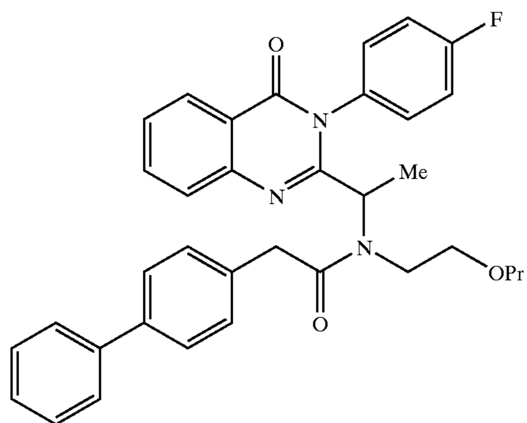
2-Biphenyl-4-yl-N-(1-[3-[(4-fluoro-phenyl)-4-oxo-3,4-dihydro-quinazolin-2-yl]-ethyl]-ethyl)-N-(2-isopropoxyethyl)-acetamide
