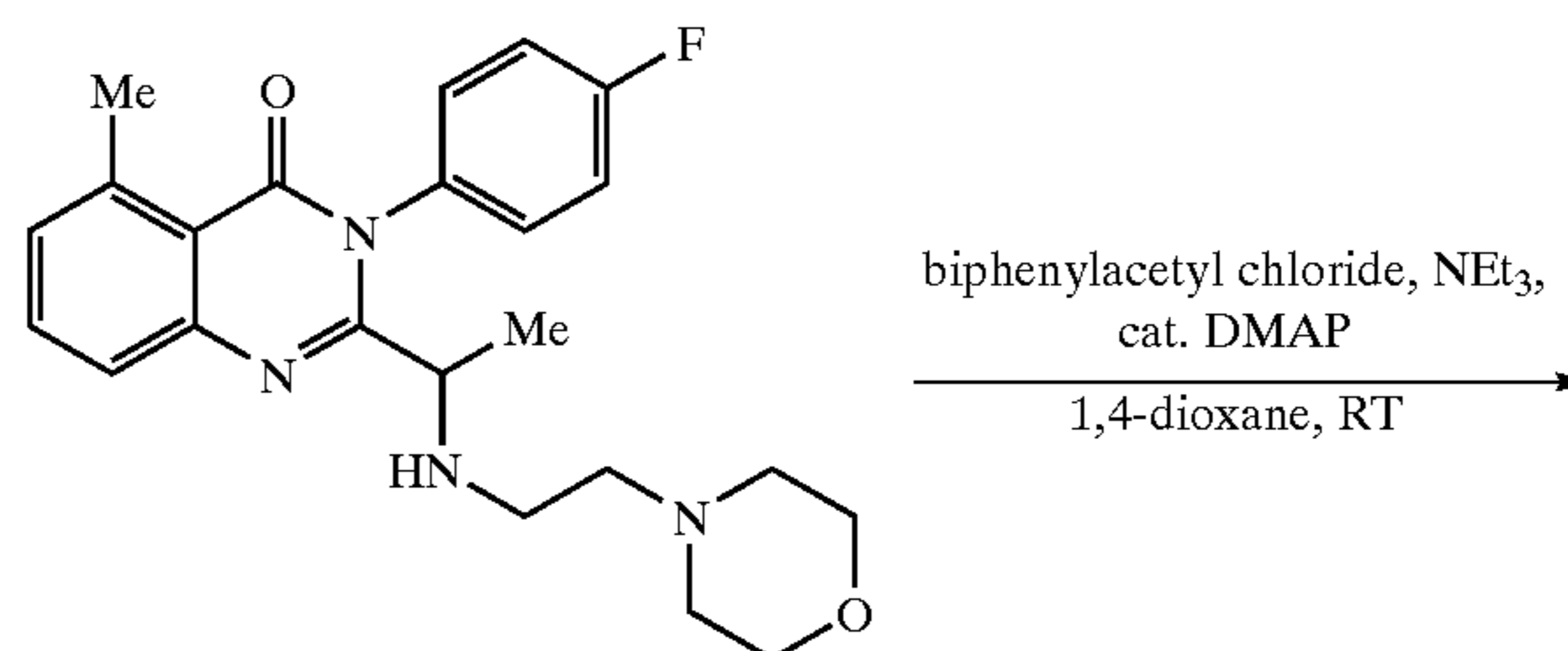
3-(4-Fluoro-phenyl)-5-methyl-2-[1-(2-morpholin-4-yl-ethylamino)-ethyl]-3H-quinazolin-4-one (XI)
