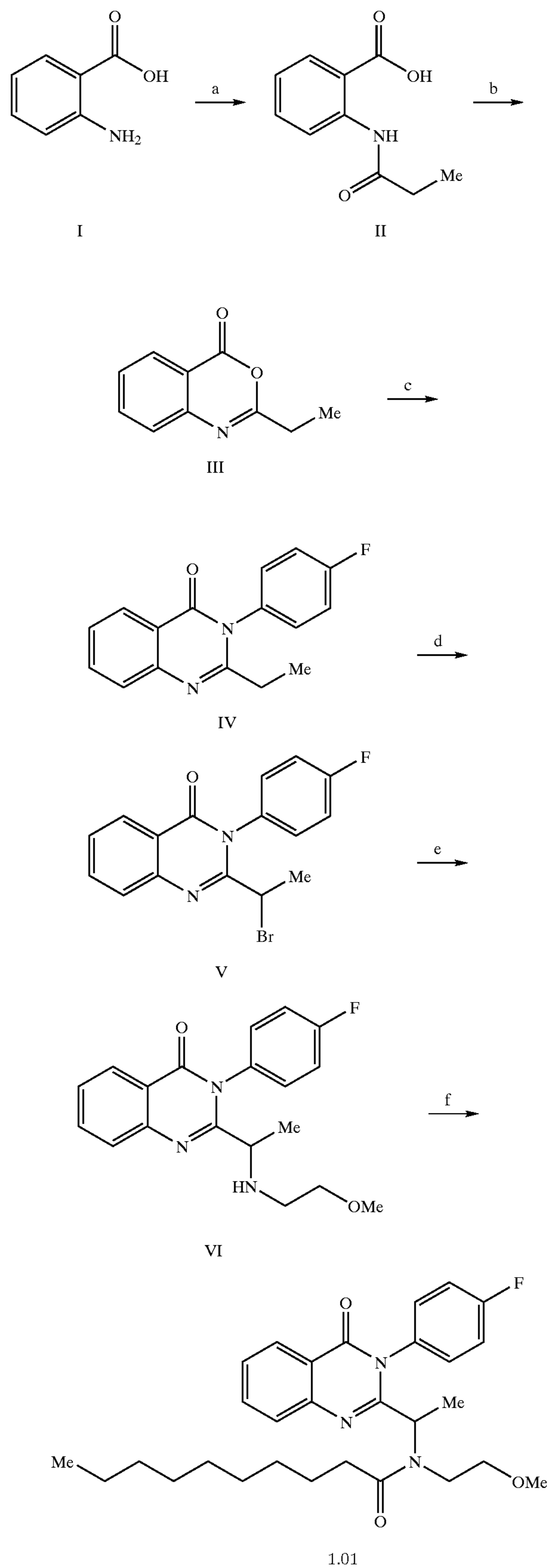
Scheme 1
