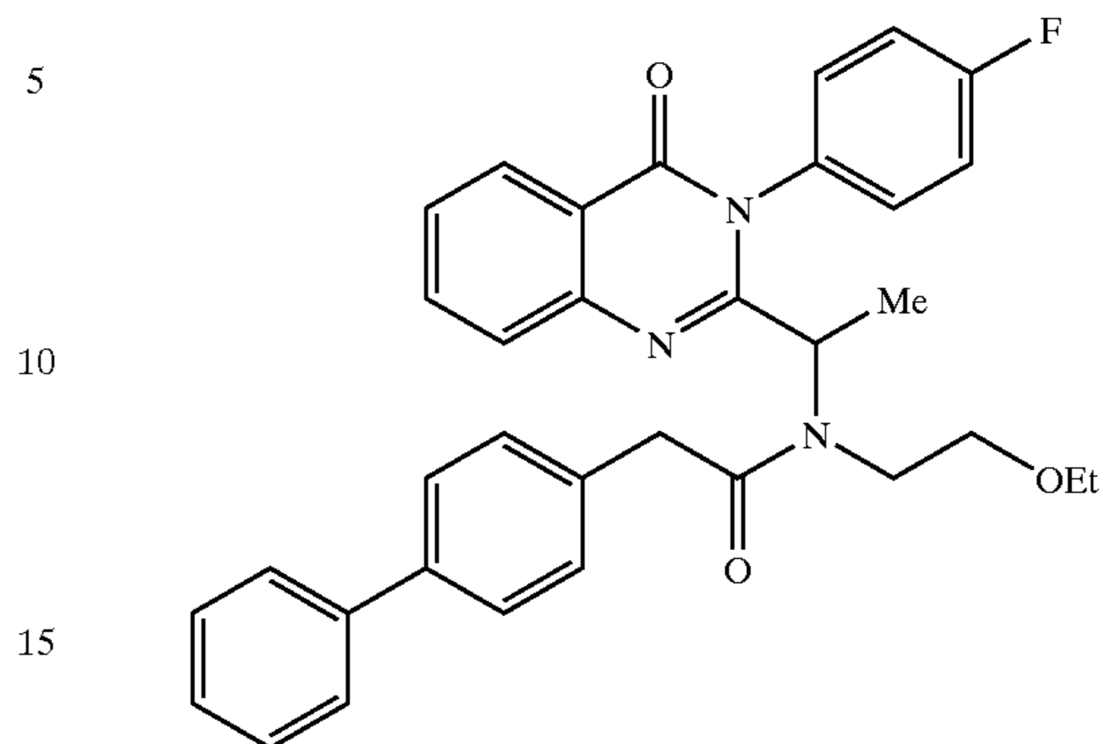
2-Biphenyl-4-yl-N-(1-[3-(4-fluoro-phenyl)-4-oxo-3,4-dihydro-quinazolin-2-yl]-ethyl)-acetamide
