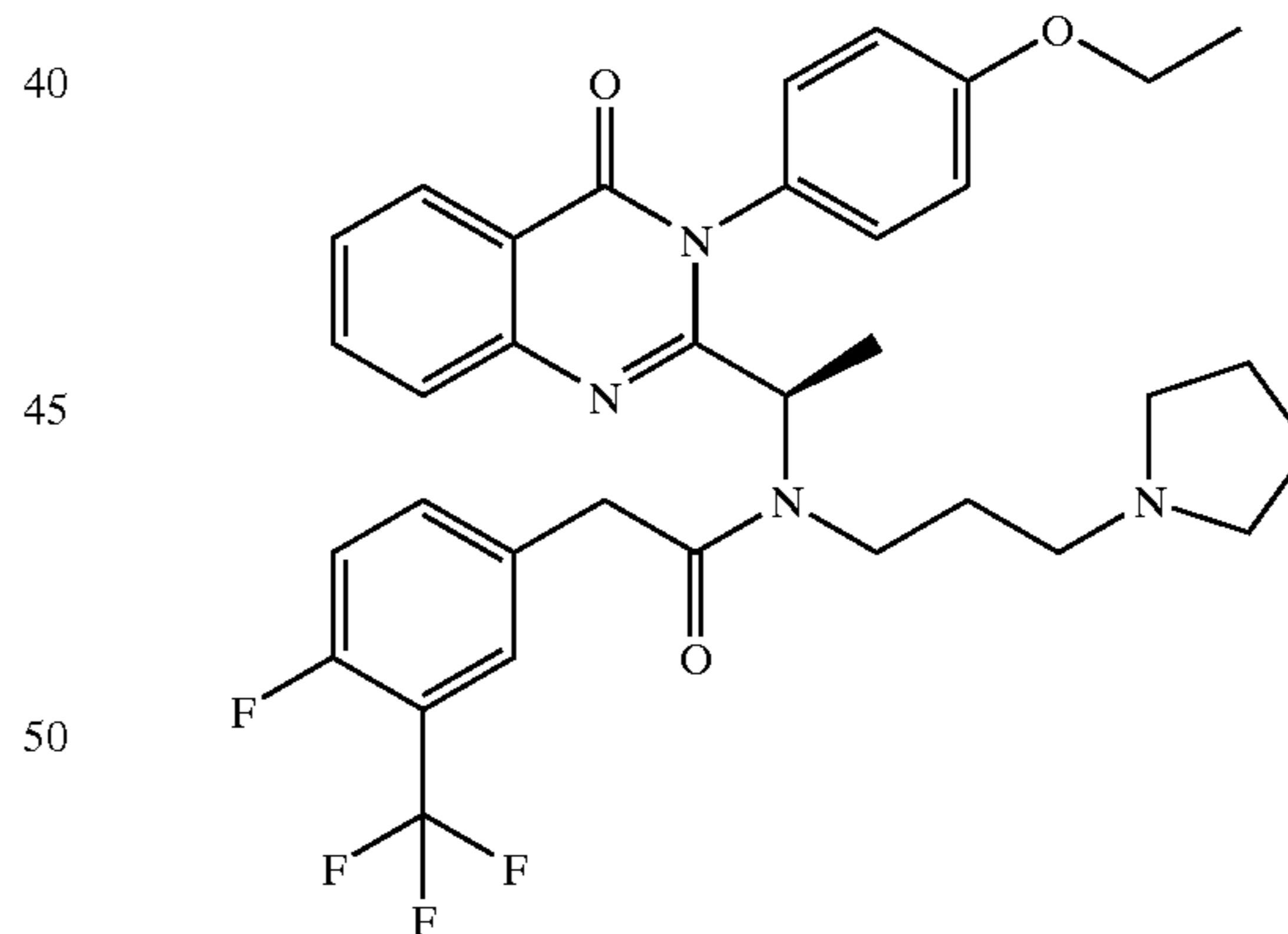
N-{1-[3-(4-Ethoxy-phenyl)-4-oxo-3,4-dihydro-quinazolin-2-yl]-ethyl}-2-(4-fluoro-3-trifluoromethyl-phenyl)-N-(3-pyrrolidin-1-yl-propyl)-acetamide
