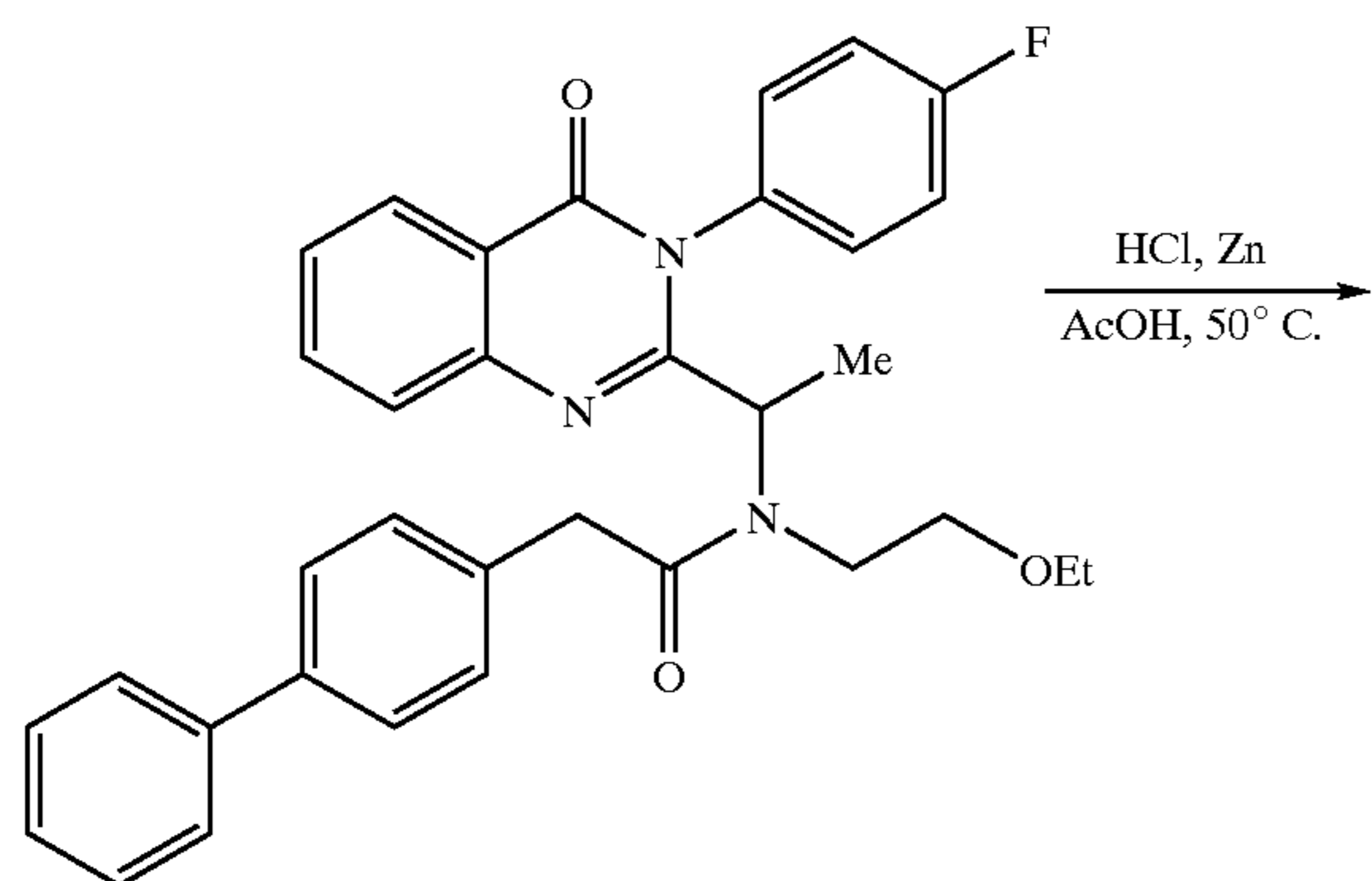
2-Biphenyl-4-yl- N -(2-ethoxy-ethyl)- N -{1-[3-(4-fluoro-phenyl)-4-oxo-3,4-dihydro-quinazolin-2-yl]-ethyl}-acetamide (1.19)
