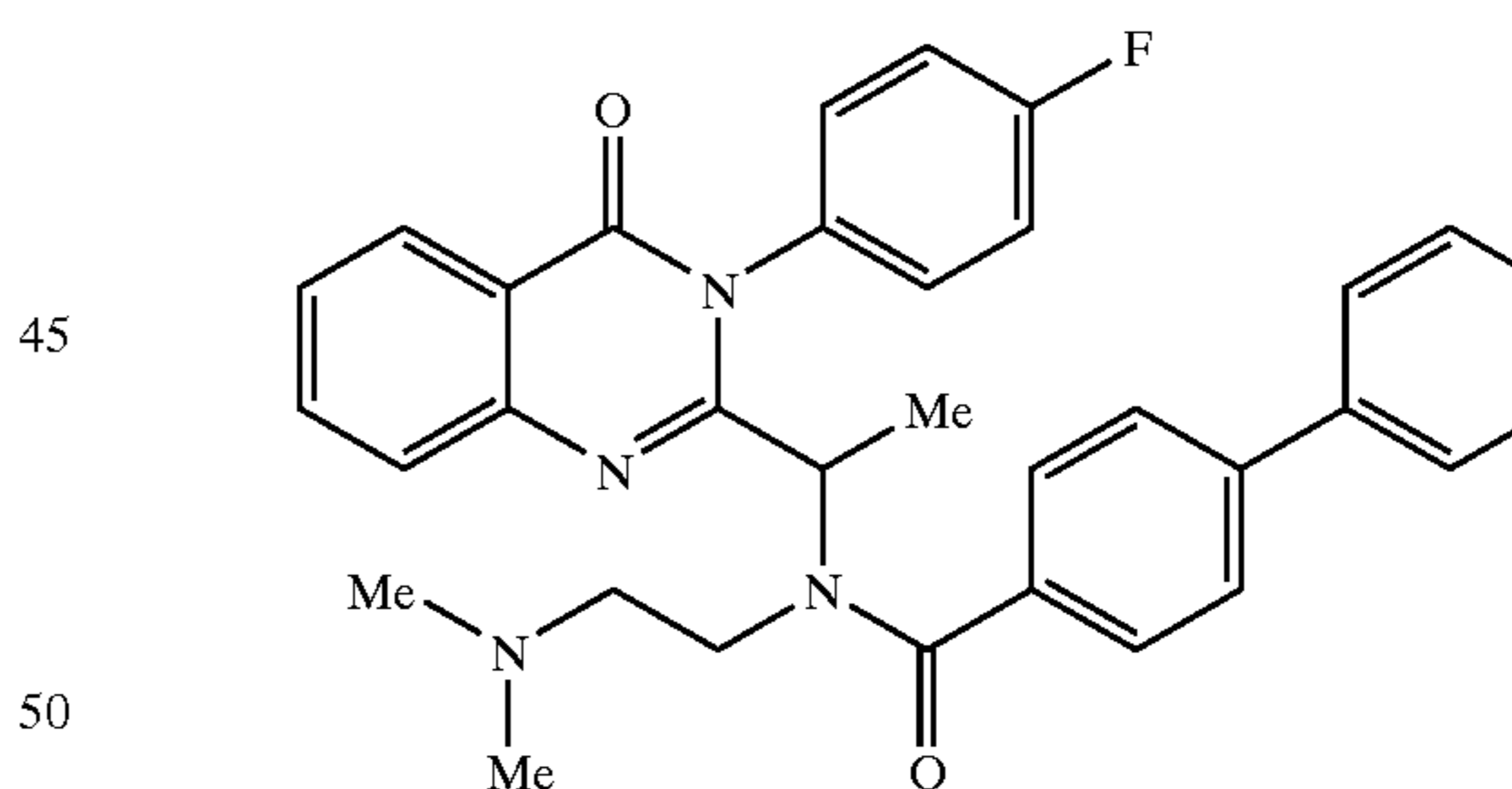
Biphenyl-4-carboxylic acid (2-dimethylamino-ethyl)-{1-[3-(4-fluoro-phenyl)-4-oxo-3,4-dihydro-quinazolin-2-yl]-ethyl}-amide
