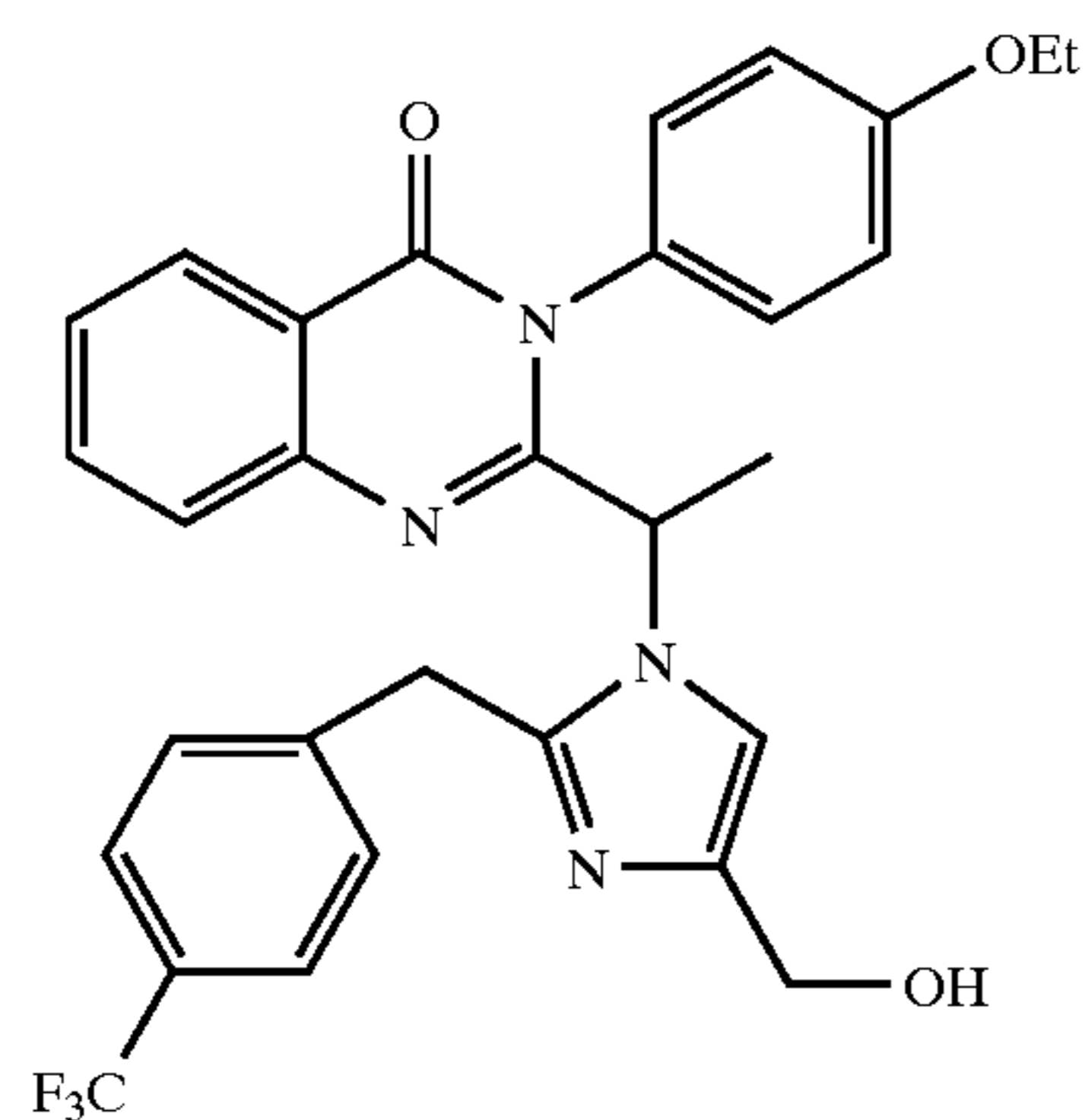
Preparation of Compound 6.11
