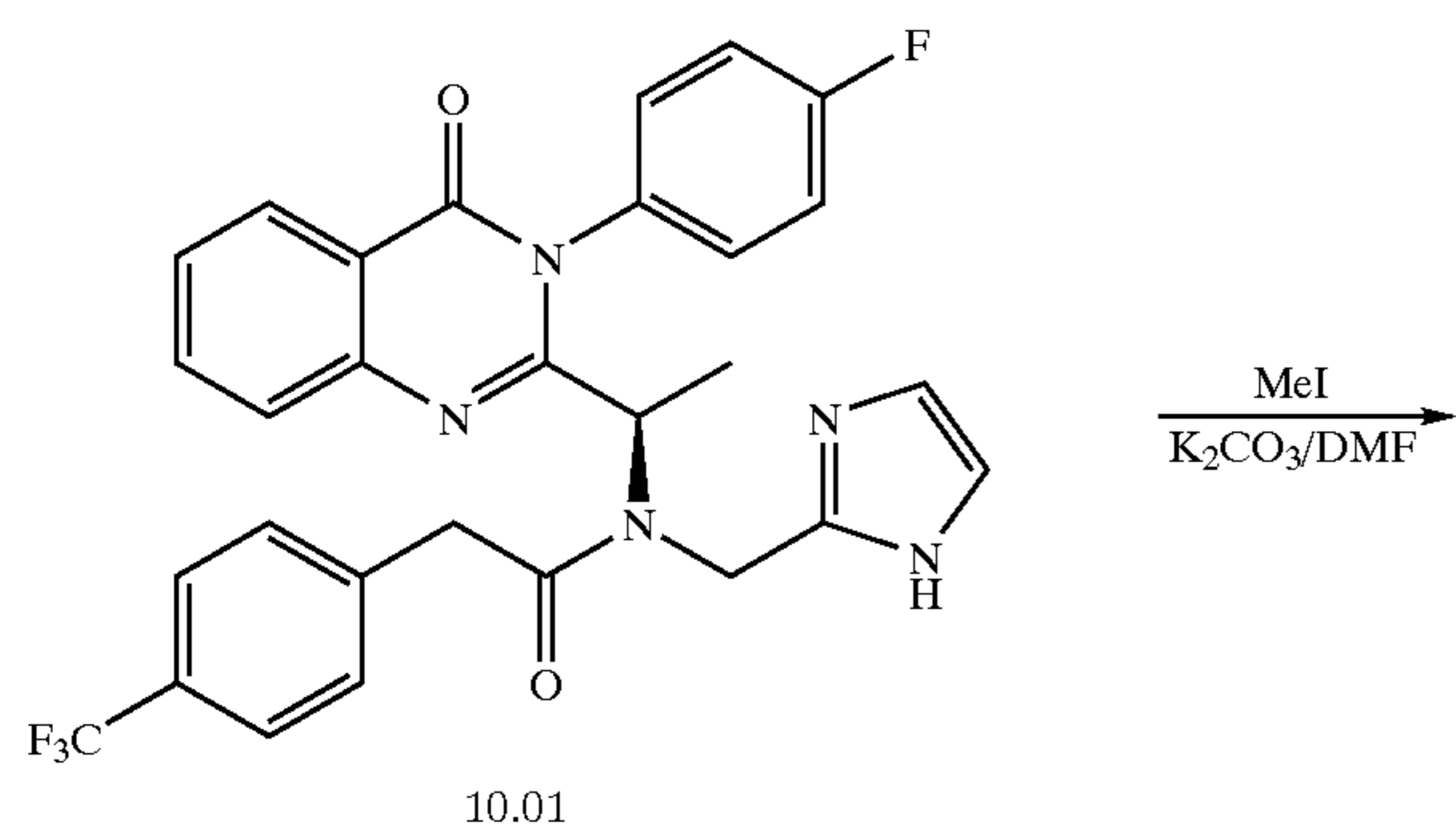
Synthesis of Compound 10.02
