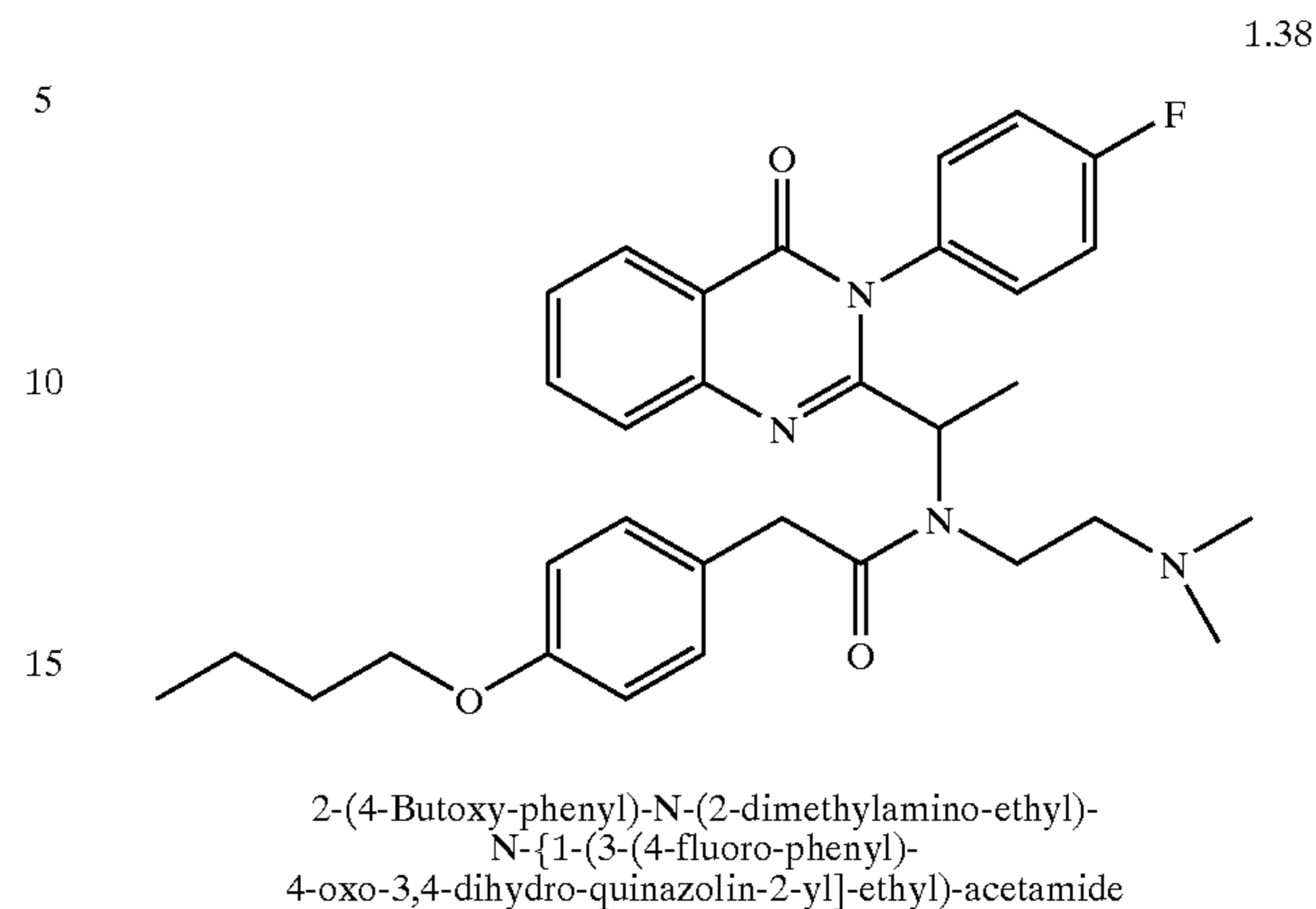
Synthesis of Compound 1.38
