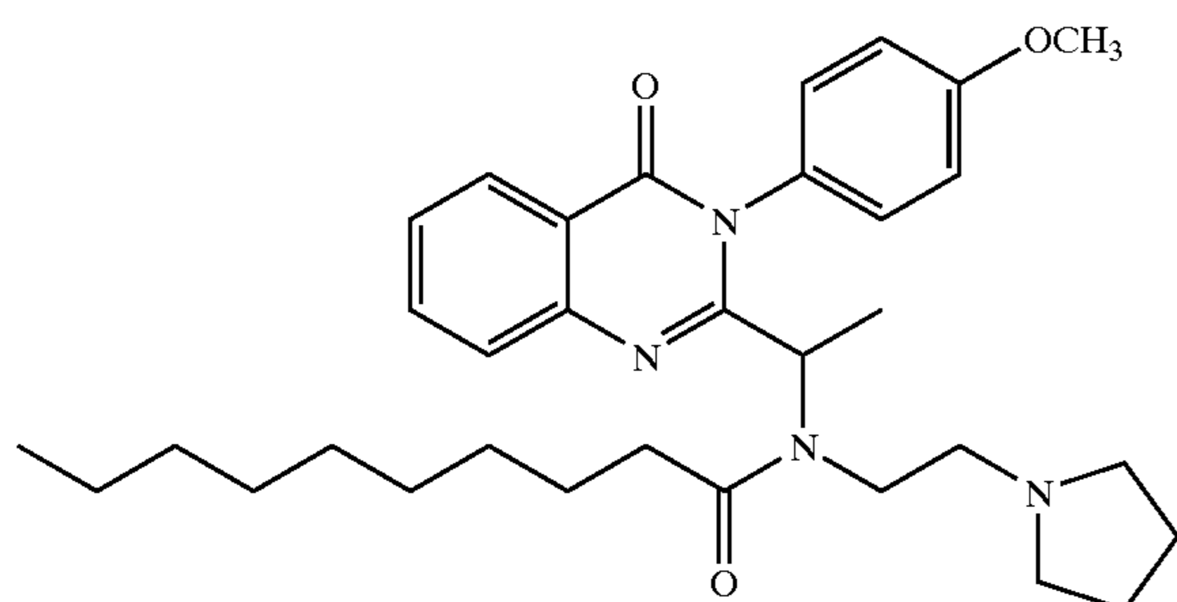
Decanoic acid {1-[3-(4-methoxy-phenyl)4-oxo-3,4-dihydro-quinazolin-2-yl]-ethyl}-(2-pyrrolidin-1-yl-ethyl)-amide
