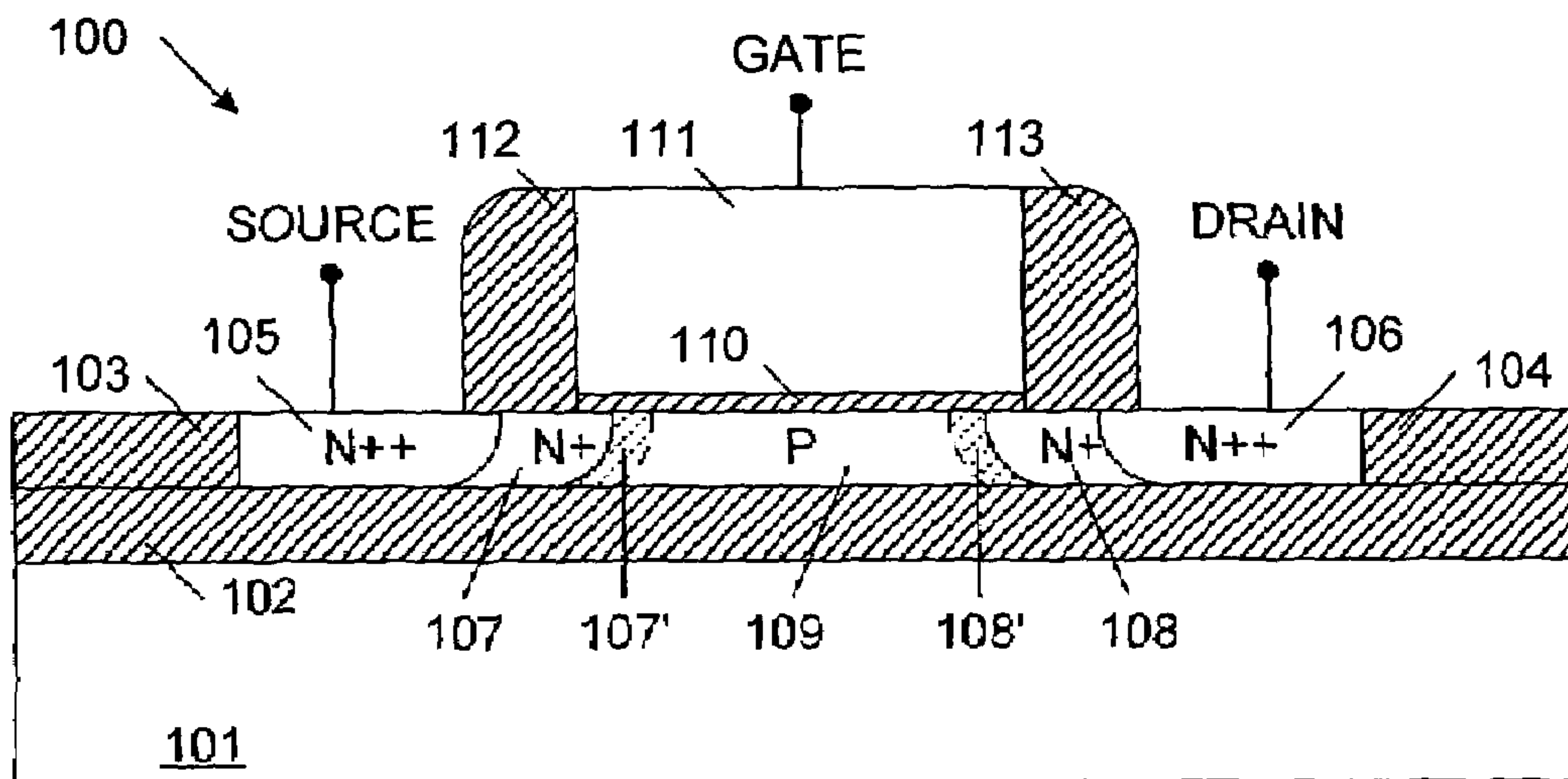
FIG. 1 (PRIOR ART)
