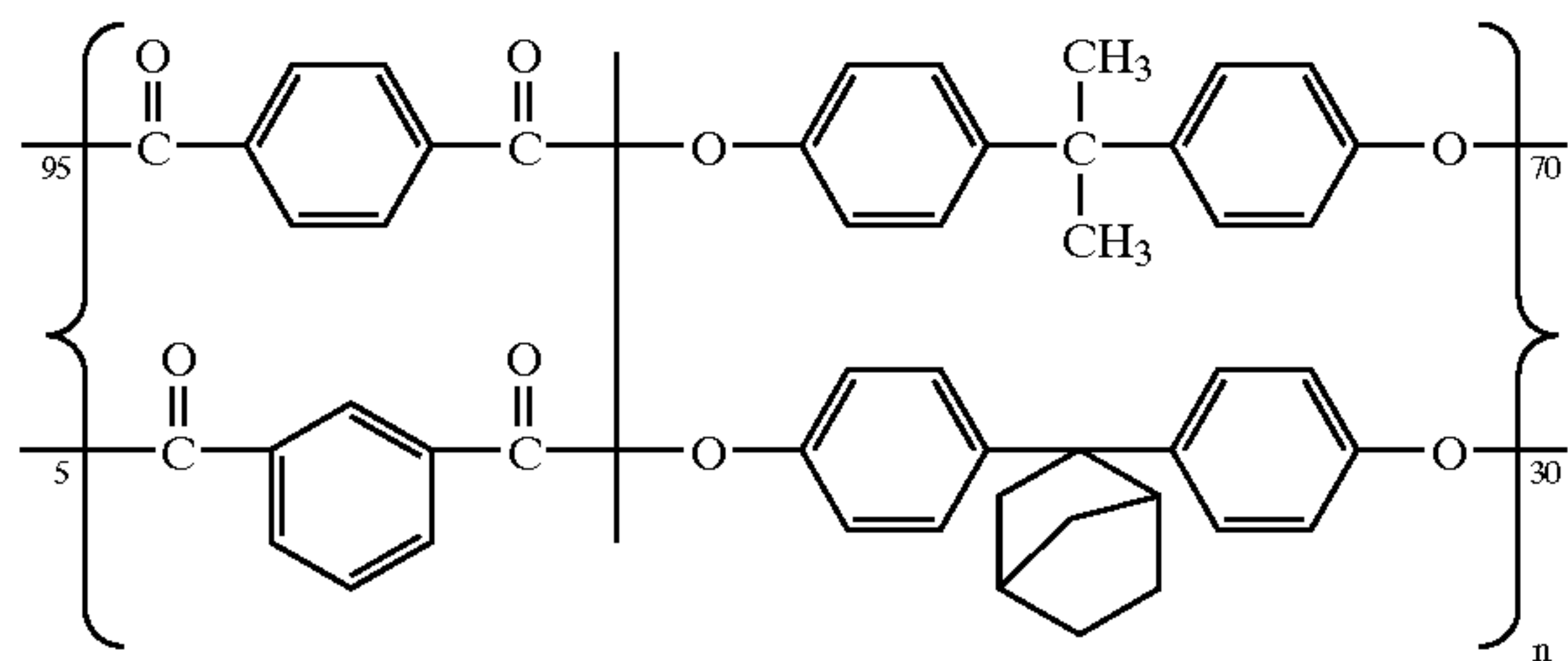
Poly(4,4'-isopropylidene-bisphenol-co-4,4'-(2-norbornylidene) bisphenol) terephthalate-co-isophthalate
