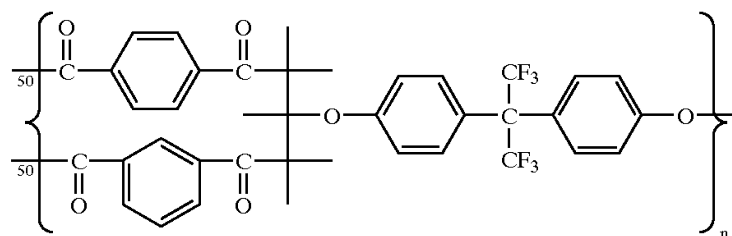
Poly(4,4'-hexafluoroisopropylidene-bisphenol) terephthalate-co-isophthalate
