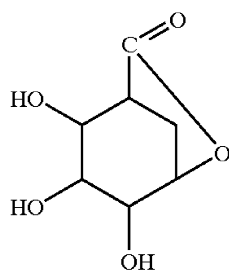
Quinic acid Lactone
