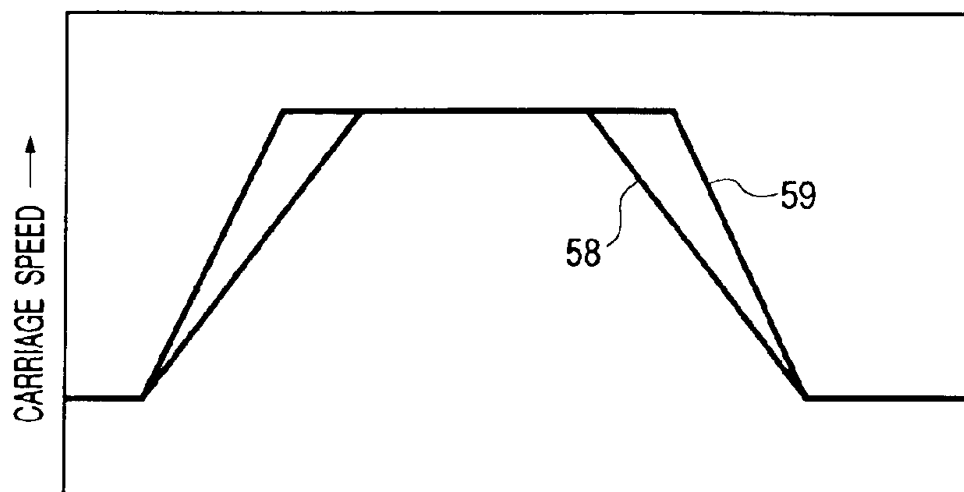
OPERATION RANGE OF CARRIAGE DURING STEP-PRINTING OPERATION
