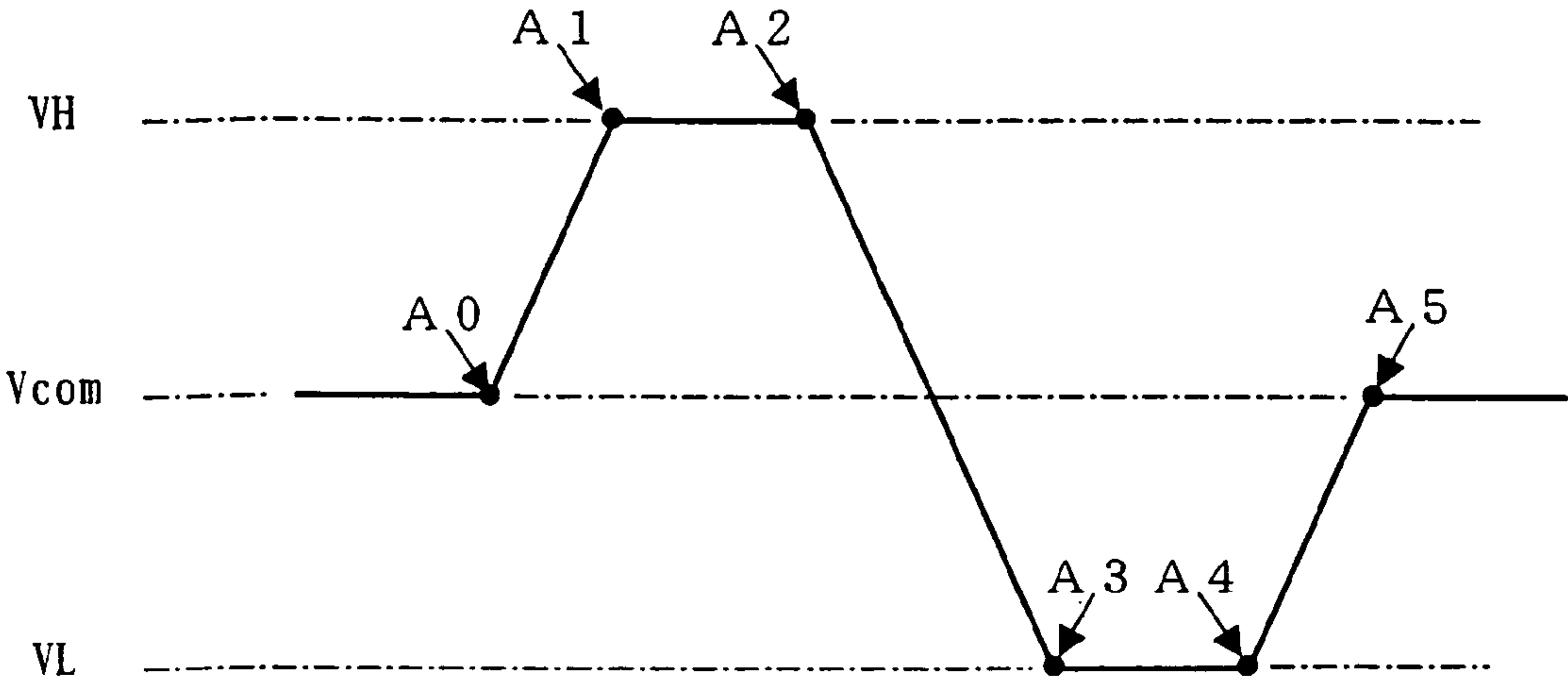
FIG. 16 (Prior Art)
