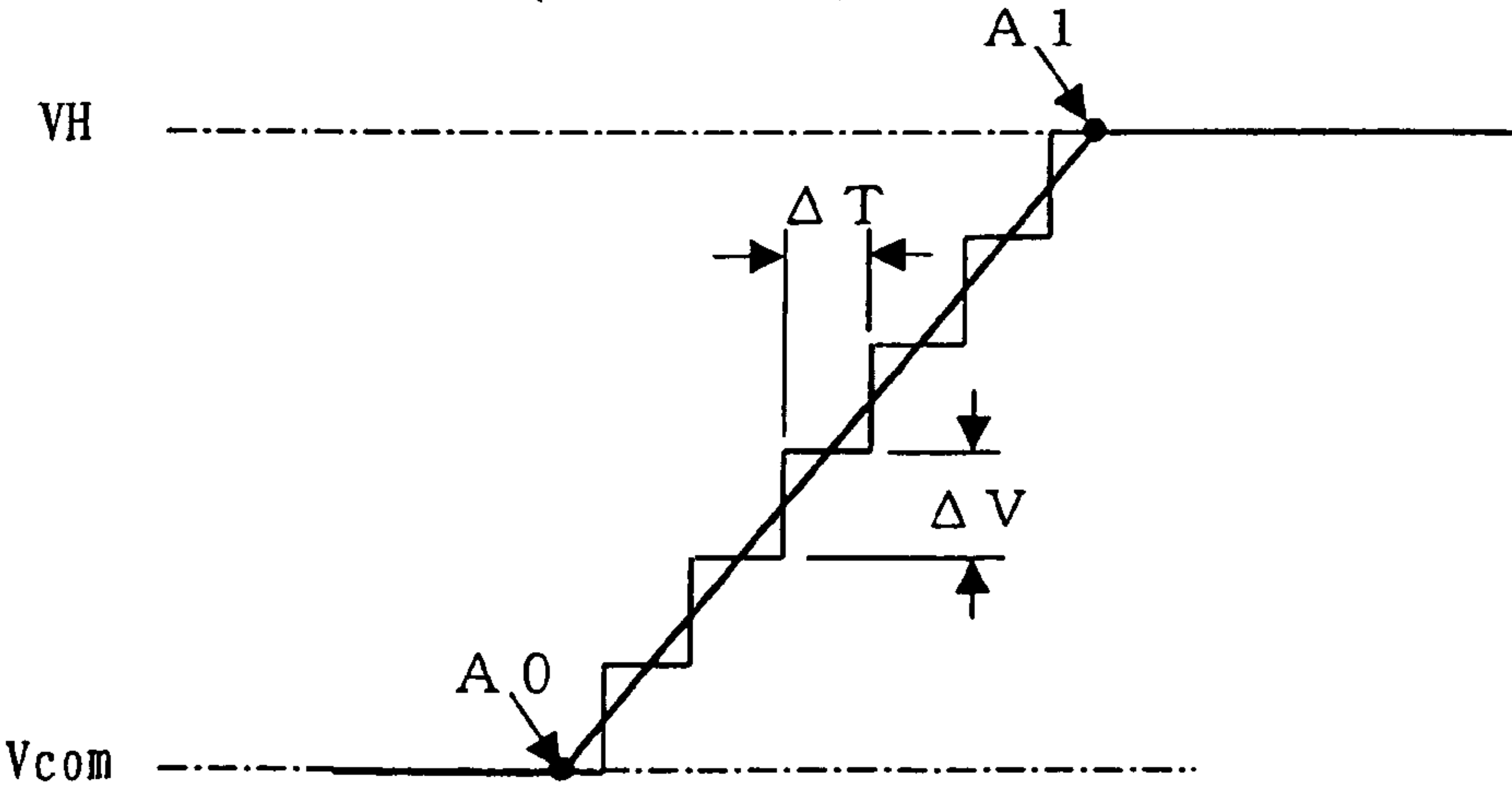
FIG. 17 (Prior Art)
