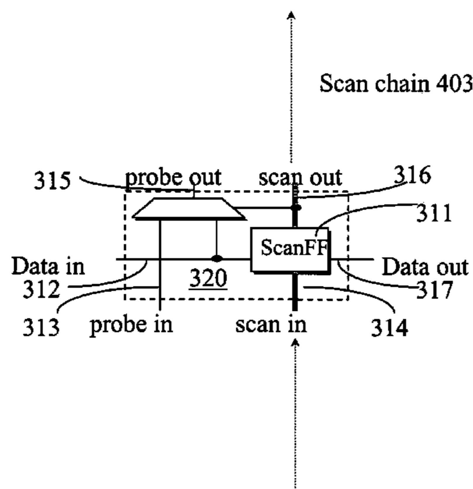
Preferred Embodiment of Block Scan Connector
