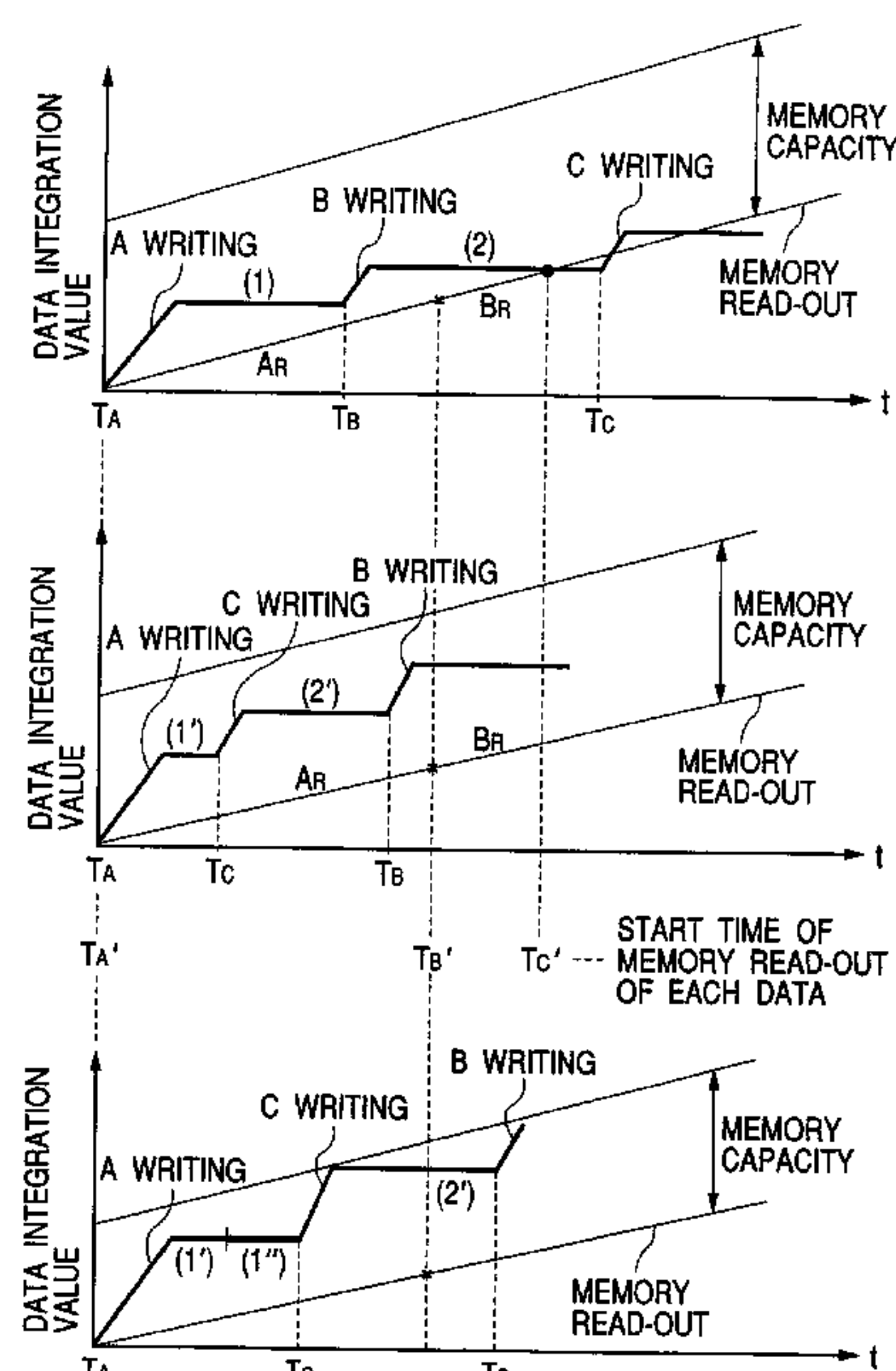
(1'') INDICATES WAITING TIME DUE TO LACK OF SPACE OF MEMORY TA, TB AND TC DENOTE TIME AT WHICH MEMORY READ-OUT OF EACH DATA IS ALLOWED
