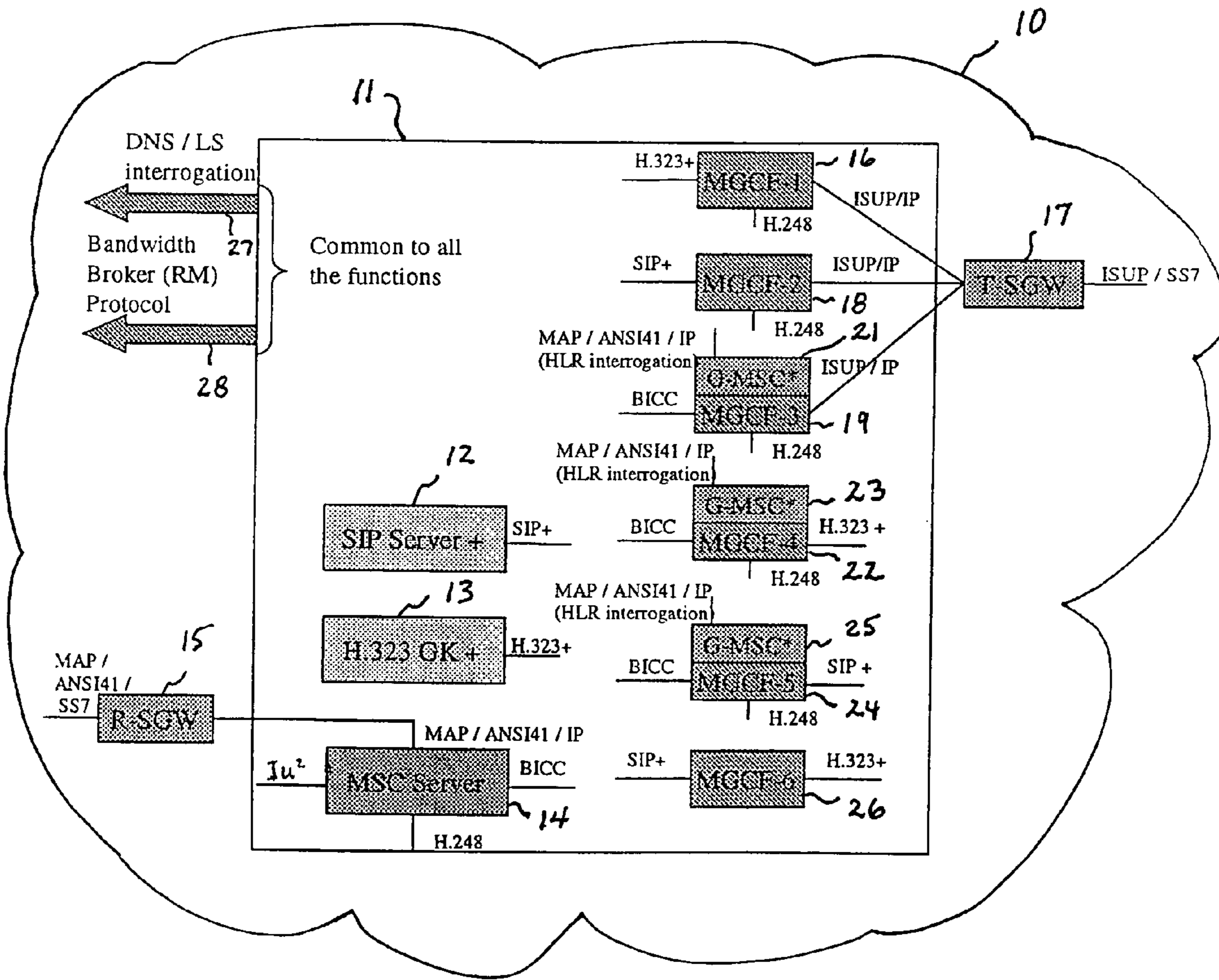
FIG. 1 (PRIOR ART)
