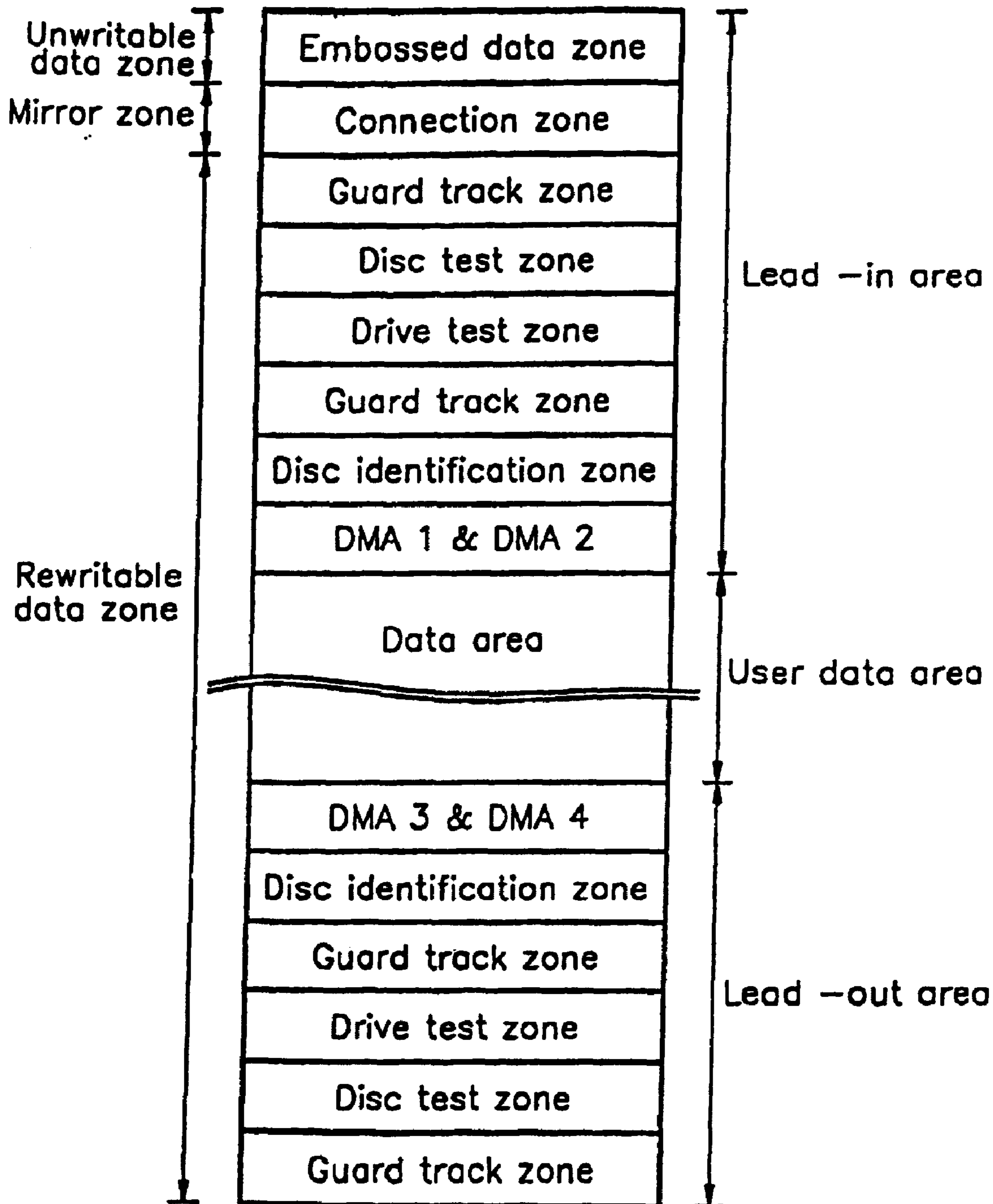
FIG. 2 PRIOR ART
