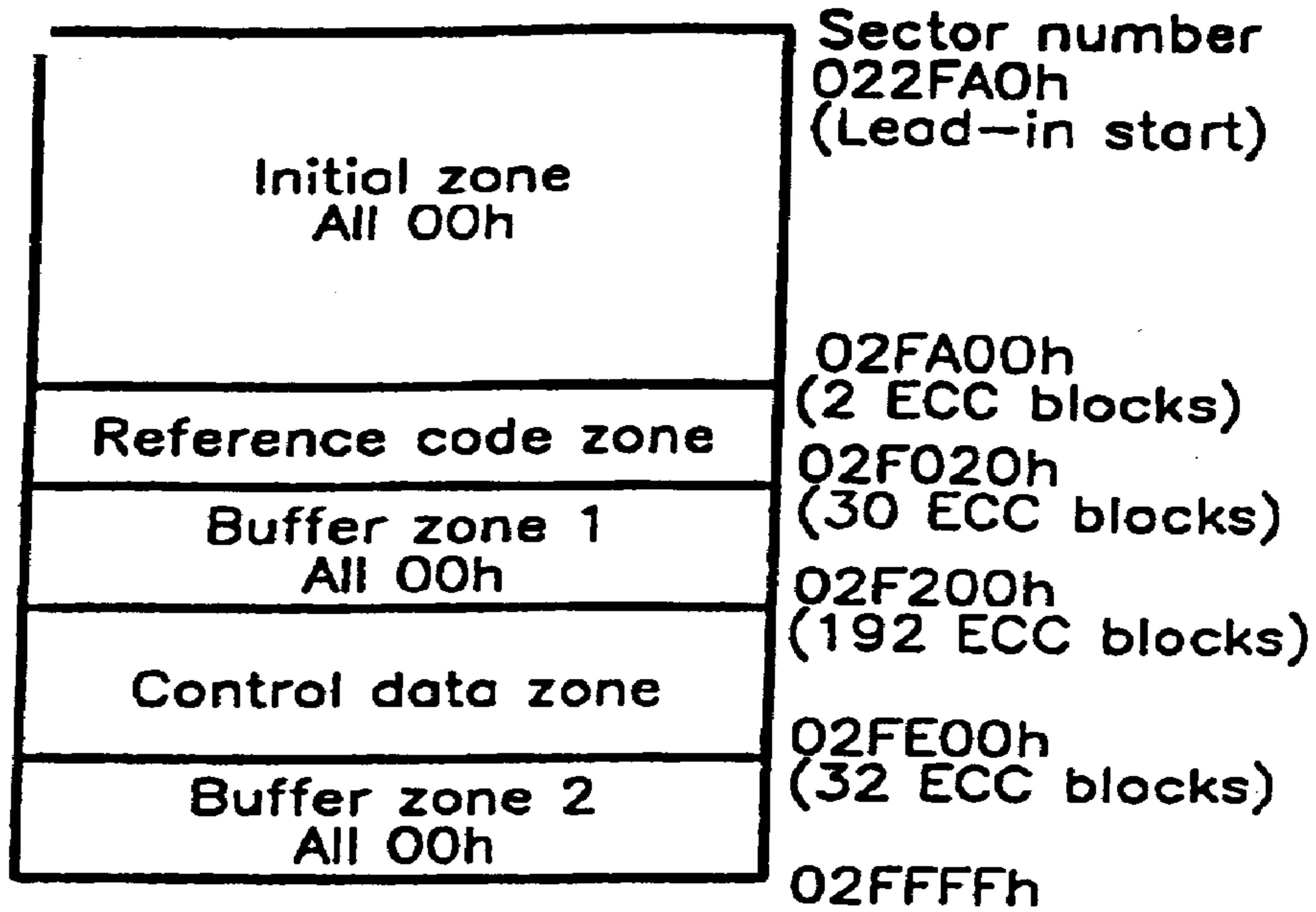
FIG. 11 PRIOR ART
